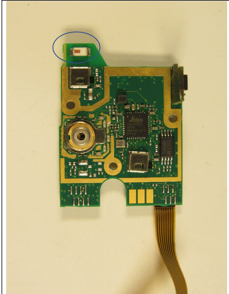
Antenna location ceramic chip antenna
