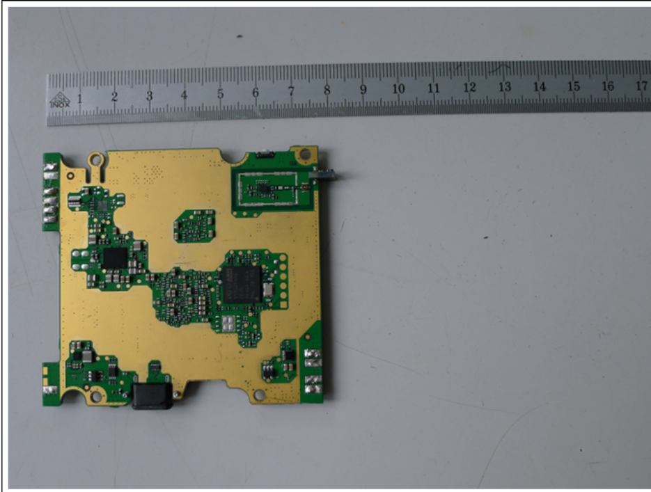
EUT INTERNAL DETAIL (C)
