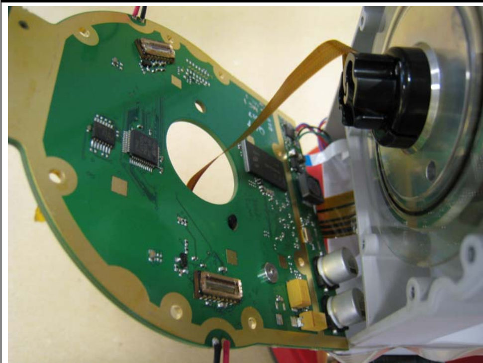
PCB Back
