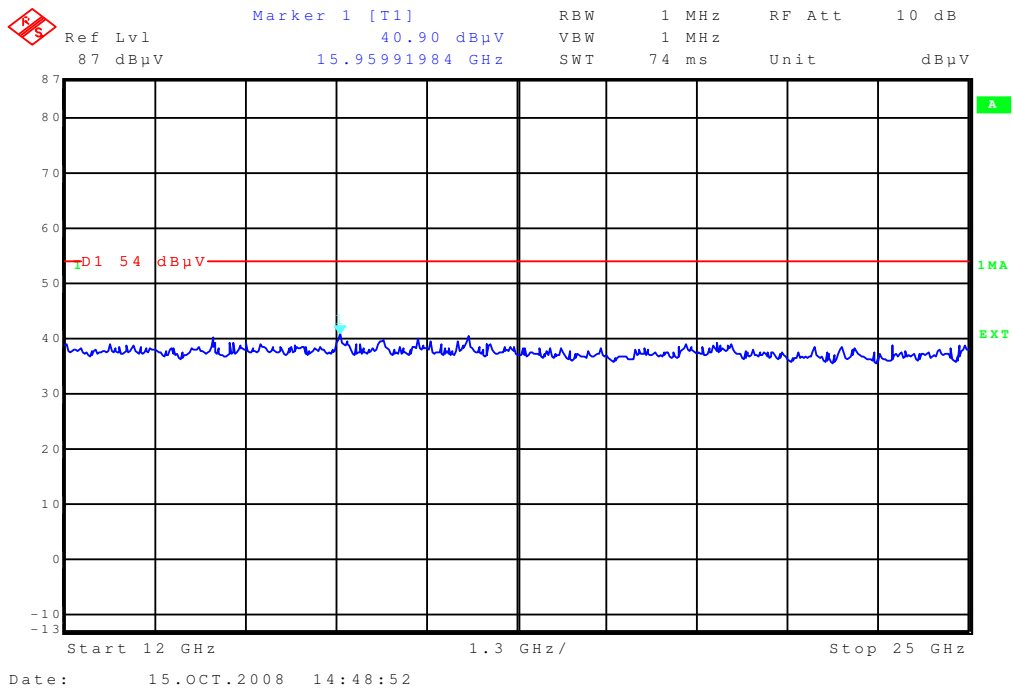
Plot 3: 12 - 25 GHz
