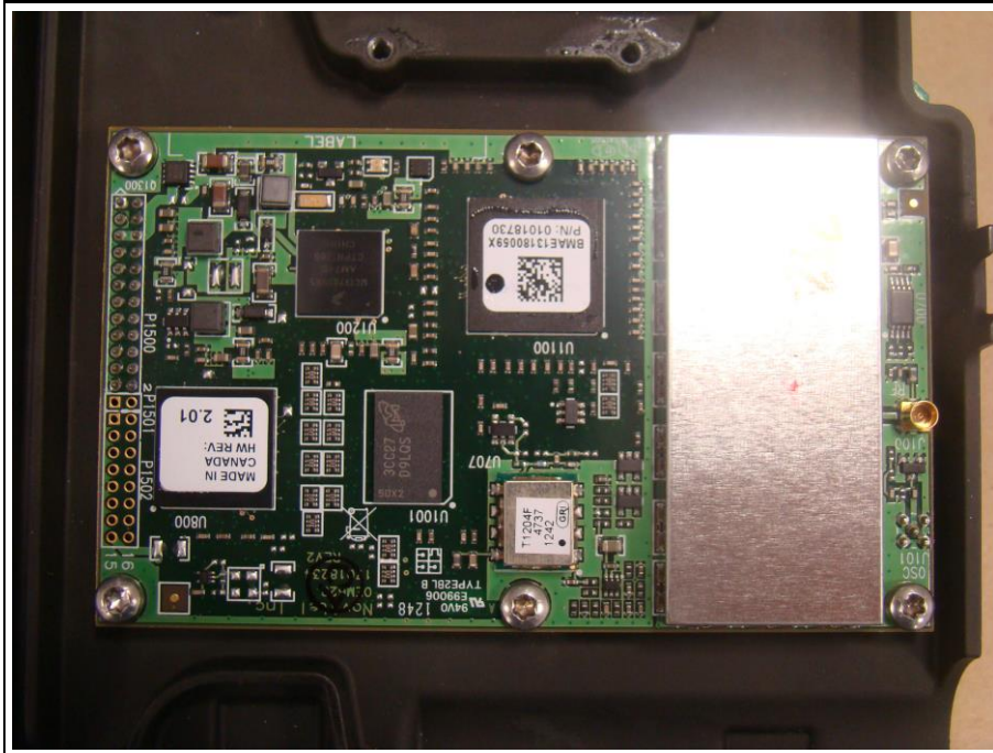
PCB2
