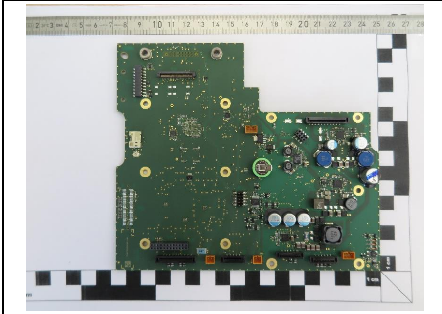
05 PCB 3 TOP SIDE
