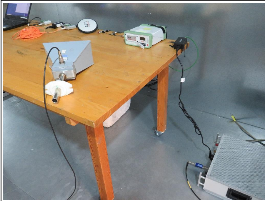
Test Setup PoE Adapter
