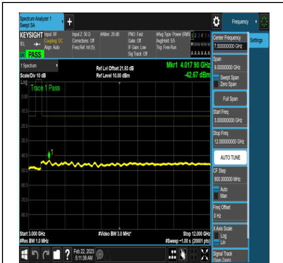
NTNV_N77-3450-3550_PC2_30_100_H_TID4_N/ A_3000_12000_#1
