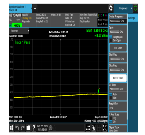
NTNV_N77-3450-3550_PC2_30_100_M_TID4_N/ A_1000_3000_#1
