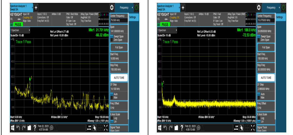
NTNV_N77-3450-3550_PC2_30_100_M_TID6_N/ A_0.009_0.15_#1
