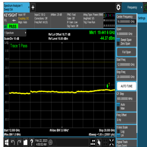
NTNV_N77-3450-3550_PC2_30_100_L_TID18_N /A_12000_20000_#1
