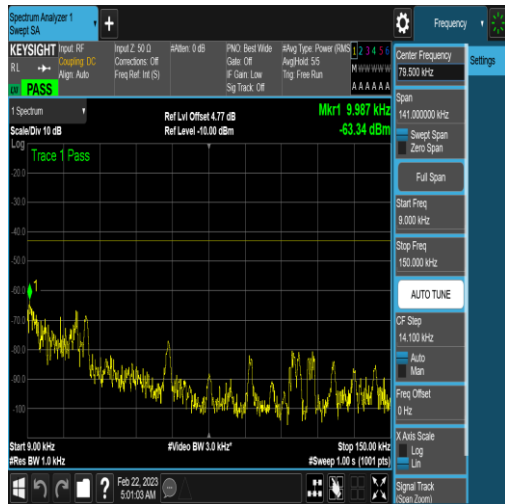
NTNV_N77-3450-3550_PC2_30_100_M_TID16_ N/A_0.009_0.15_#1
