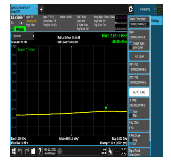
NTNV_N77-3450-3550_PC2_30_100_L_TID16_N /A_0.15_30_#1
