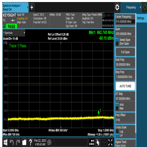
NTNV_N77-3450-3550_PC2_30_100_M_TID5_NV/ A_30_1000_#1
