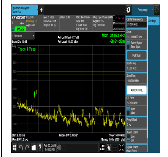
NTNV_N77-3450-3550_PC2_30_100_L_TID17_N /A_3000_12000_#1
