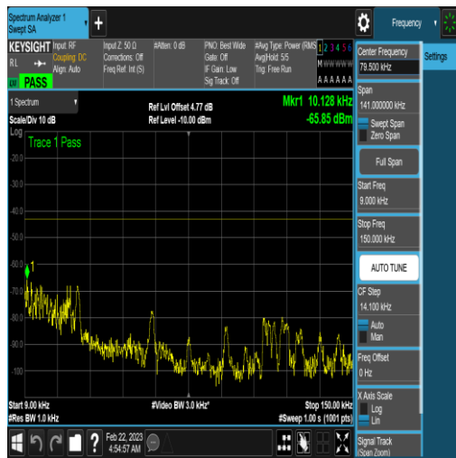
NTNV_N77-3450-3550_PC2_30_100_M_TID5_NV/ A_0.009_0.15_#1
