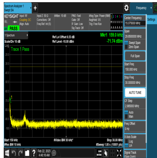
NTNV_N77-3450-3550_PC2_30_100_L_TID17_N /A_0.15_30_#1
