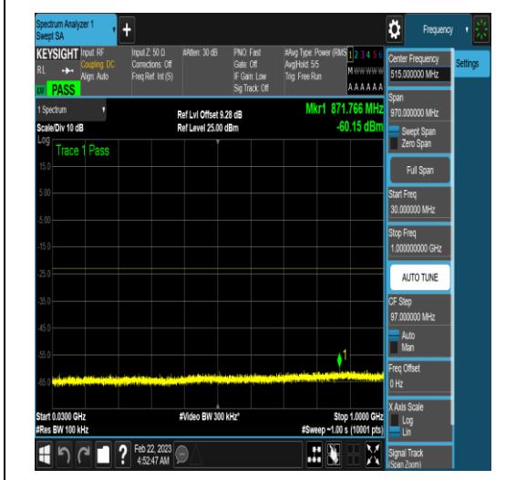
NTNV_N77-3450-3550_PC2_30_100_M_TID4_N/ A_30_1000_#1
