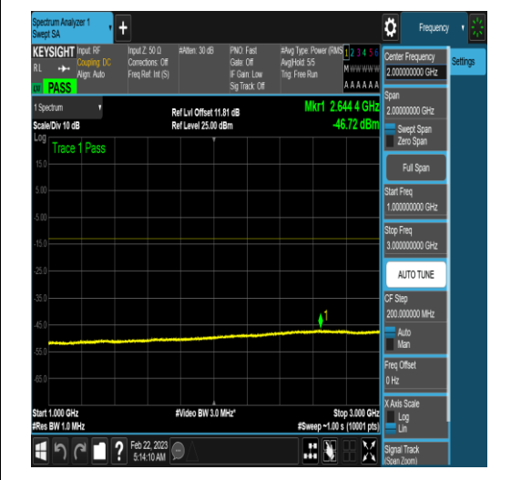
NTNV_N77-3450-3550_PC2_30_100_H_TID5_N/ A_0.15_30_#1
