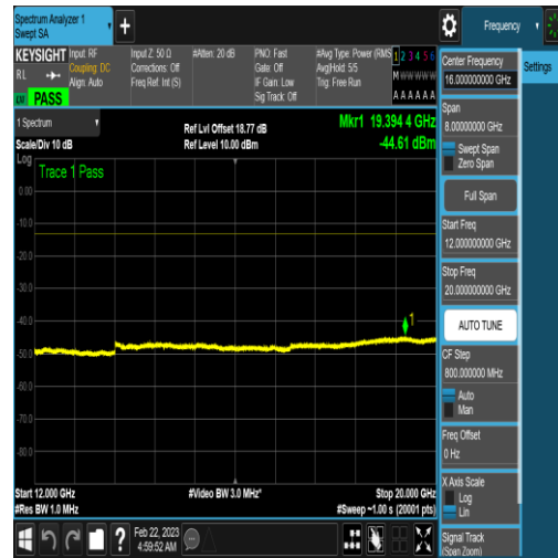
NTNV_N77-3450-3550_PC2_30_100_M_TID6_NV/ A_12000_20000_#1
