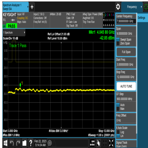
NTNV_N77-3450-3550_PC2_30_100_H_TID5_N/ A_3000_12000_#1
