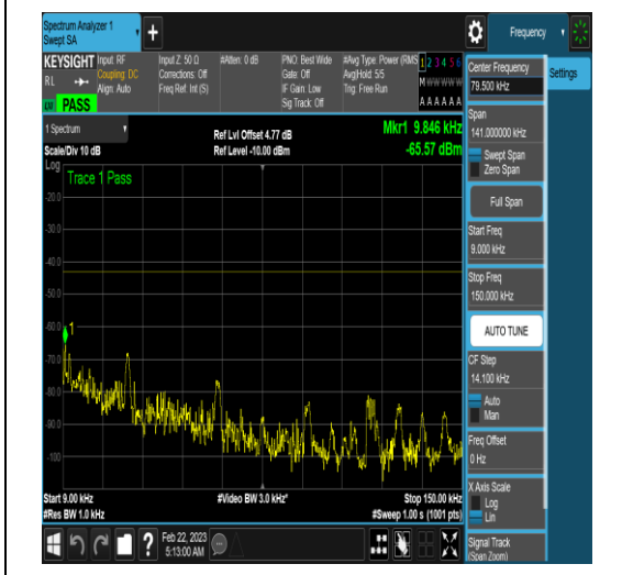
NTNV_N77-3450-3550_PC2_30_100_H_TID5_N/ A_0.009_0.15_#1
