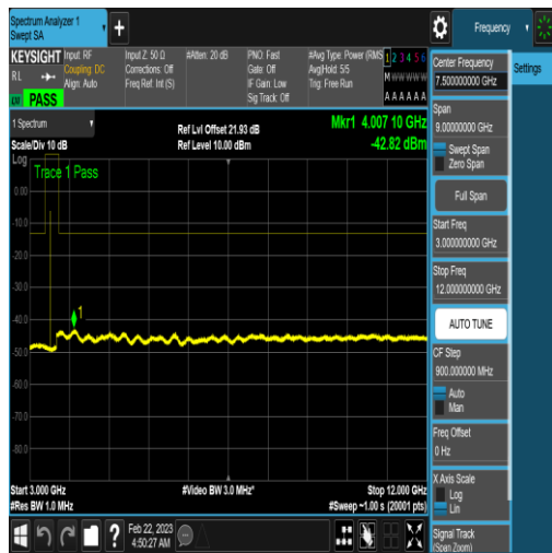
NTNV_N77-3450-3550_PC2_30_100_L_TID18_N /A_3000_12000_#1
