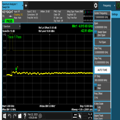
NTNV_N77-3450-3550_PC2_30_100_M_TID6_NV/ A_3000_12000_#1
