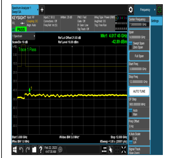
NTNV_N77-3450-3550_PC2_30_100_L_TID17_N /A_3000_12000_#1
