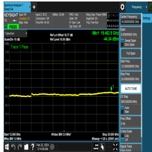
NTNV_N77-3450-3550_PC2_30_100_H_TID5_N/ A_12000_20000_#1
