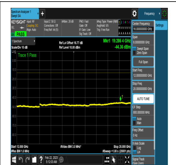
NTNV_N77-3450-3550_PC2_30_100_H_TID4_N/ A_12000_20000_#1
