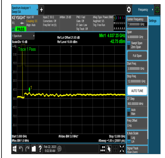
NTNV_N77-3450-3550_PC2_30_100_M_TID16_ N/A_3000_12000_#1
