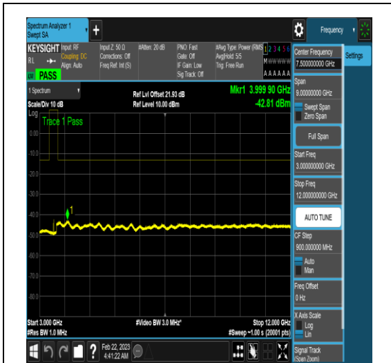
NTNV_N77-3450-3550_PC2_30_100_L_TID6_N/ A_3000_12000_#1
