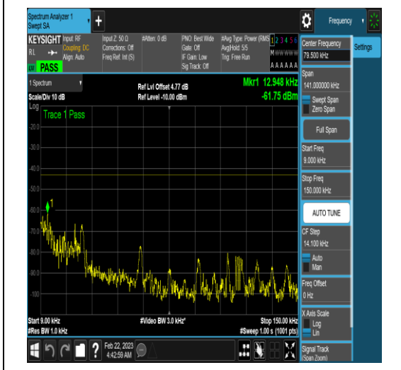
NTNV_N77-3450-3550_PC2_30_100_L_TID16_N /A_0.009_0.15_#1
