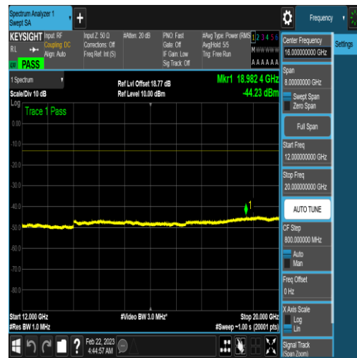
NTNV_N77-3450-3550_PC2_30_100_L_TID16_N /A_12000_20000_#1
