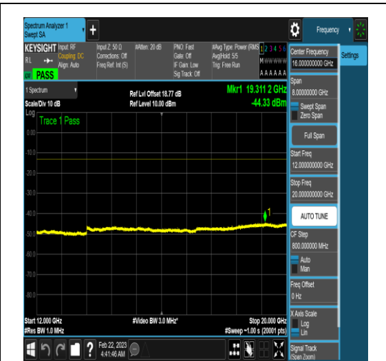
NTNV_N77-3450-3550_PC2_30_100_L_TID6_N/ A_12000_20000_#1
