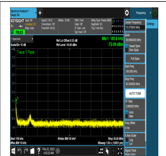
NTNV_N77-3450-3550_PC2_30_100_M_TID4_N/ A_0.15_30_#1
