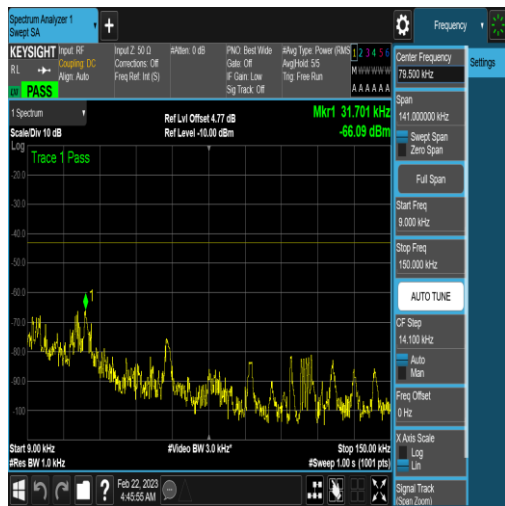
NTNV_N77-3450-3550_PC2_30_100_L_TID17_N /A_0.009_0.15_#1
