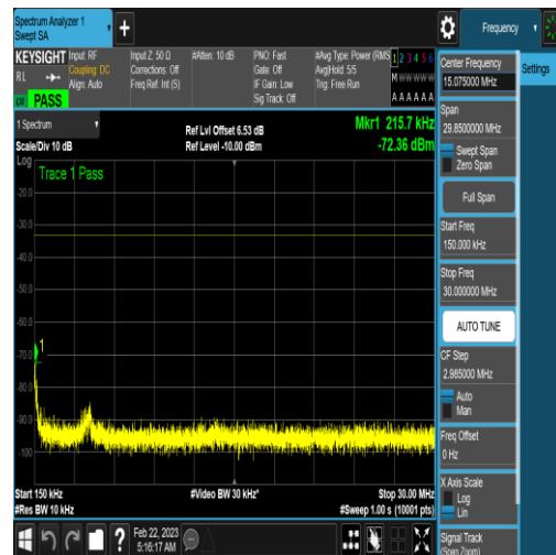
NTNV_N77-3450-3550_PC2_30_100_H_TID6_N/ A_0.15_30_#1
