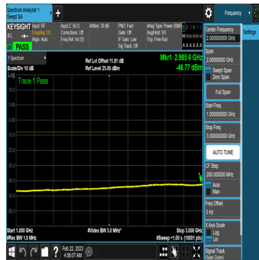
NTNV_N77-3450-3550_PC2_30_100_M_TID5_NV/ A_1000_3000_#1
