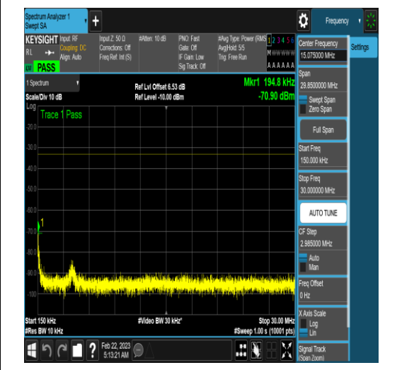
NTNV_N77-3450-3550_PC2_30_100_H_TID5_N/ A_0.15_30_#1
