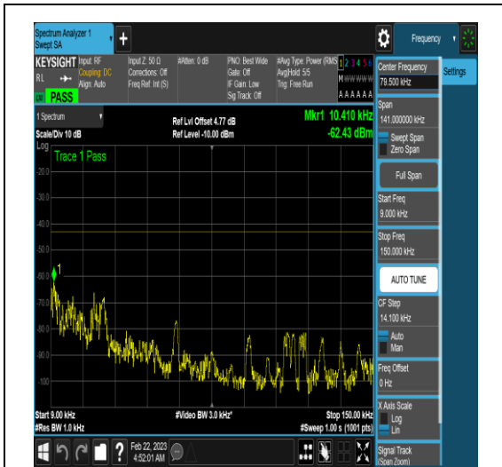
NTNV_N77-3450-3550_PC2_30_100_M_TID4_N/ A_0.009_0.15_#1
