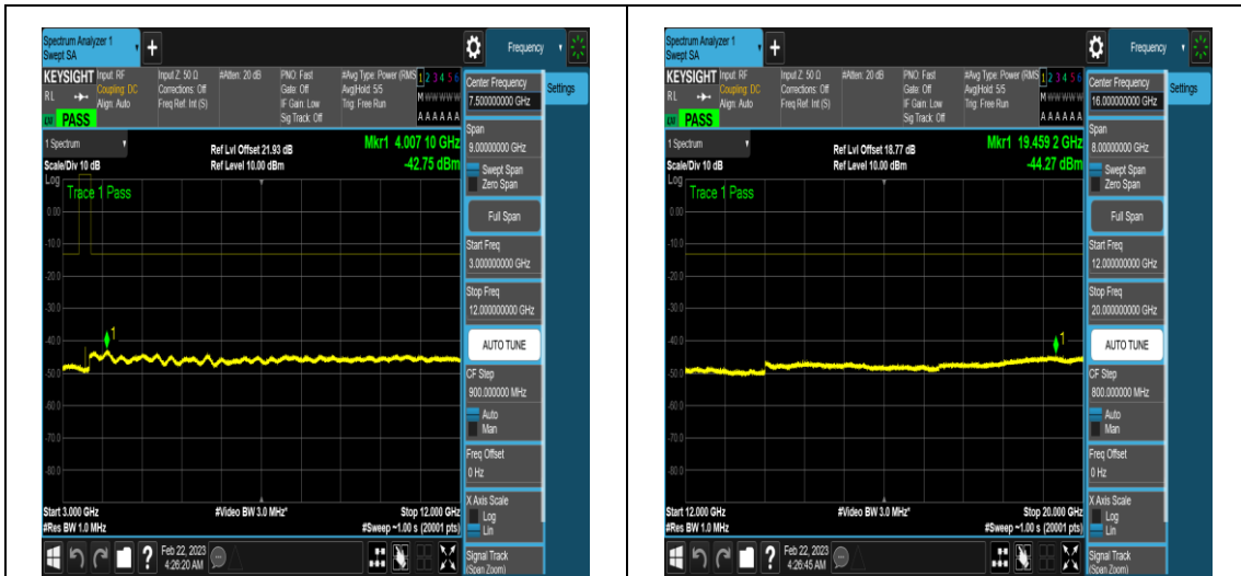
NTNV_N77-3450-3550_PC2_30_90_H_TID16_N/ A_3000_12000_#1
