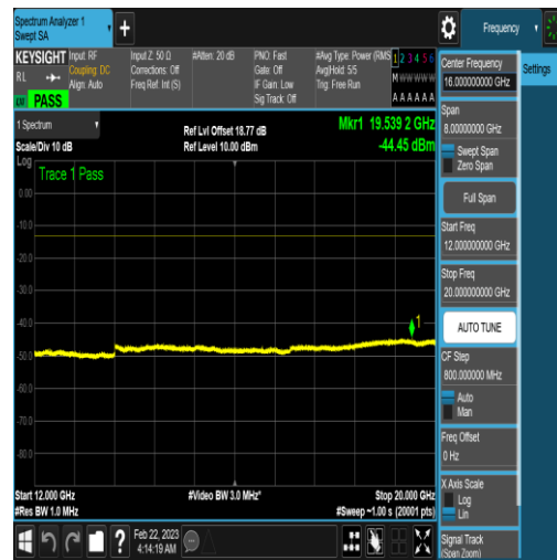
NTNV_N77-3450-3550_PC2_30_90_M_TID18_NV/ A_12000_20000_#1
