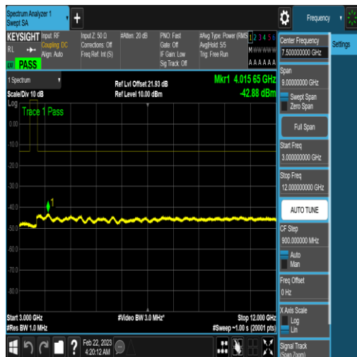
NTNV_N77-3450-3550_PC2_30_90_H_TID5_N/A _3000_12000_#1
