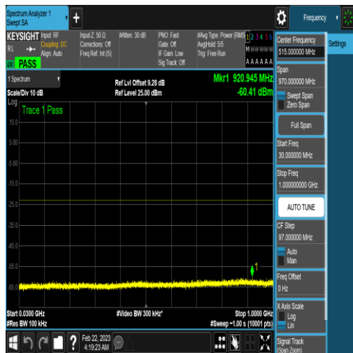
NTNV_N77-3450-3550_PC2_30_90_H_TID5_N/A _30_1000_#1
