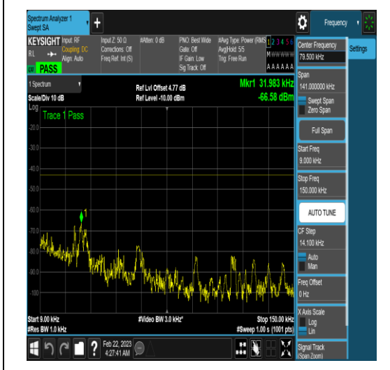
NTNV_N77-3450-3550_PC2_30_90_H_TID17_N/ A_0.009_0.15_#1
