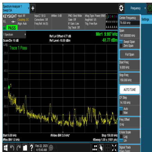
NTNV_N77-3450-3550_PC2_30_90_H_TID4_N/A _0.009_0.15_#1
