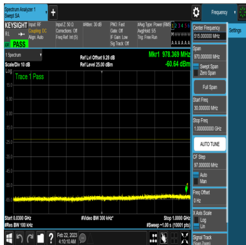
NTNV_N77-3450-3550_PC2_30_90_M_TID17_NV/ A_30_1000_#1
