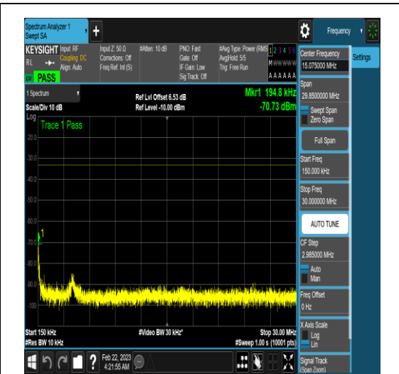
NTNV_N77-3450-3550_PC2_30_90_H_TID6_N/A _0.15_30_#1
