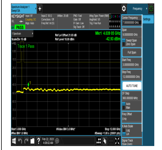
NTNV_N77-3450-3550_PC2_30_90_M_TID16_N/ A_30_1000_#1
