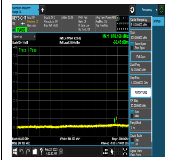
NTNV_N77-3450-3550_PC2_30_90_H_TID6_N/A _30_1000_#1
