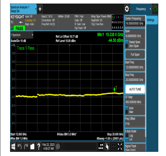
NTNV_N77-3450-3550_PC2_30_90_M_TID16_N/ A_1000_3000_#1
