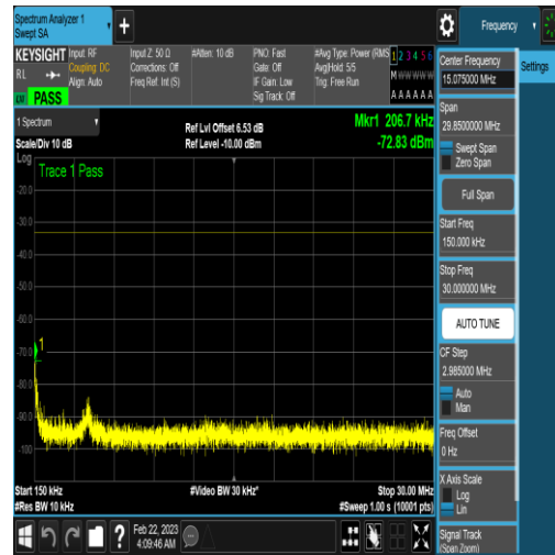
NTNV_N77-3450-3550_PC2_30_90_M_TID17_NV/ A_0.15_30_#1
