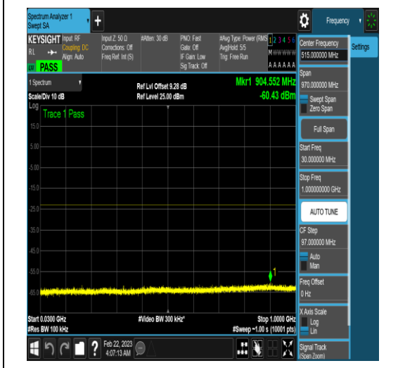
NTNV_N77-3450-3550_PC2_30_90_M_TID16_N/ A_30_1000_#1
