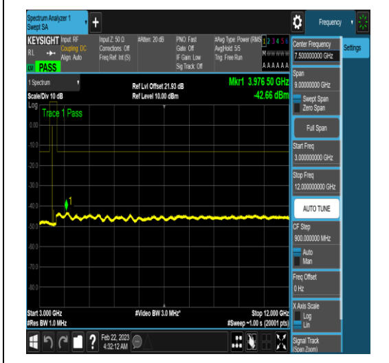
NTNV_N77-3450-3550_PC2_30_90_H_TID18_N/A_3000_12000_#1
