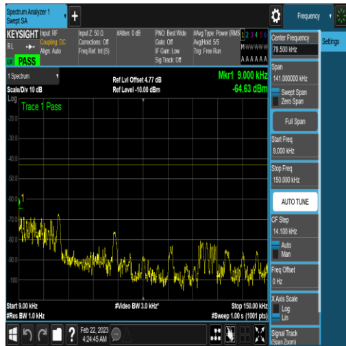
NTNV_N77-3450-3550_PC2_30_90_H_TID16_N/ A_0.009_0.15_#1
