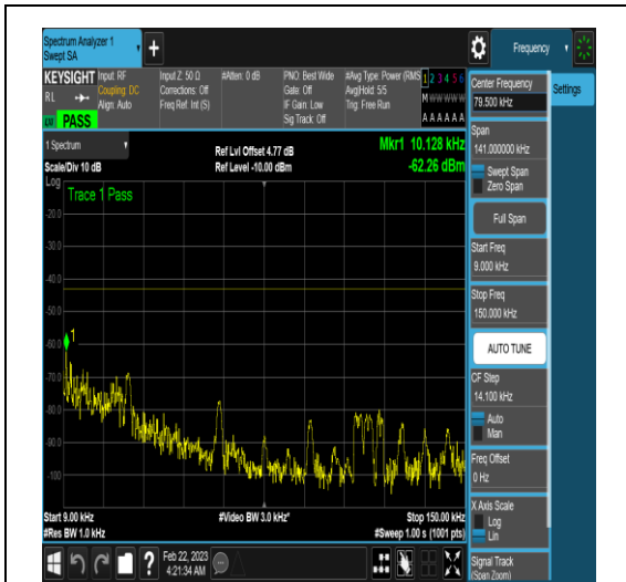
NTNV_N77-3450-3550_PC2_30_90_H_TID6_N/A _0.009_0.15_#1
