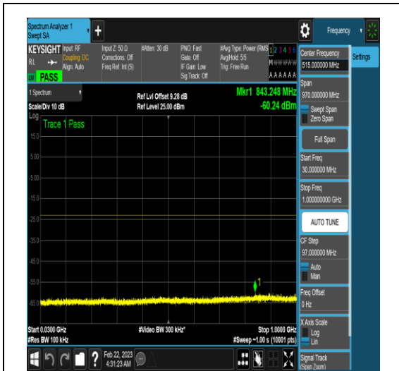
NTNV_N77-3450-3550_PC2_30_90_H_TID18_N/A_30_1000_#1
