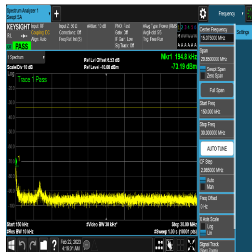
NTNV_N77-3450-3550_PC2_30_90_H_TID4_N/A _0.15_30_#1
