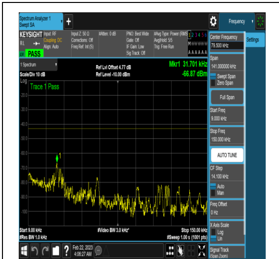
NTNV_N77-3450-3550_PC2_30_90_M_TID16_N/ A_0.009_0.15_#1
