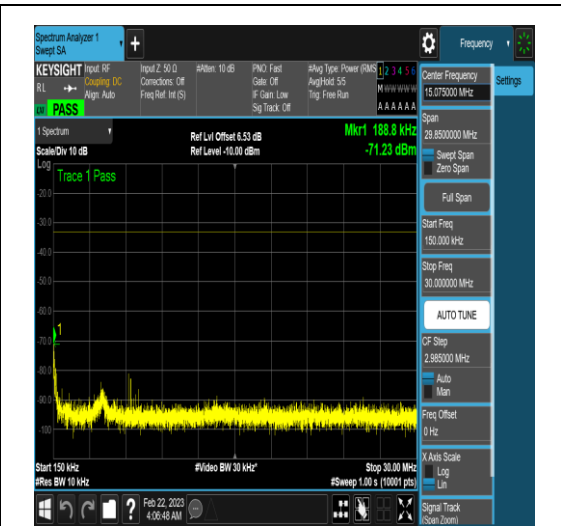
NTNV_N77-3450-3550_PC2_30_90_M_TID16_N/ A_0.15_30_#1
