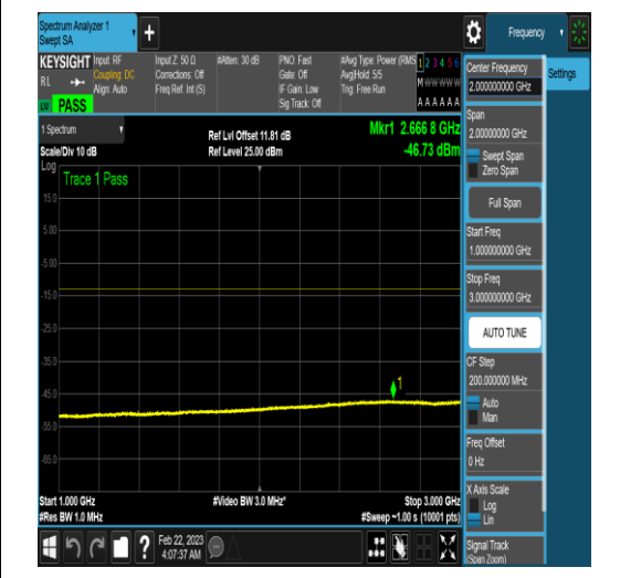
NTNV_N77-3450-3550_PC2_30_90_M_TID16_N/ A_1000_3000_#1
