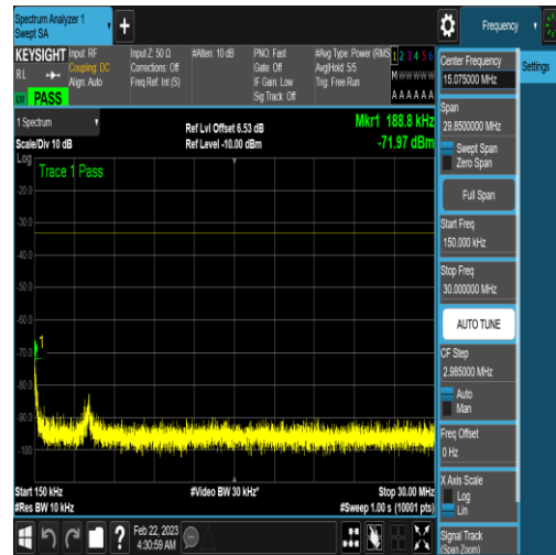
NTNV_N77-3450-3550_PC2_30_90_H_TID18_N/ A_0.15_30_#1
