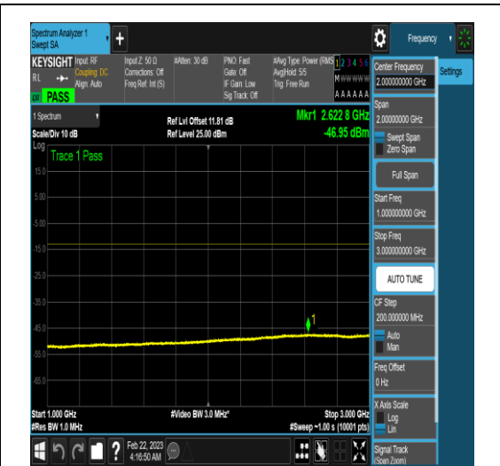
NTNV_N77-3450-3550_PC2_30_90_H_TID4_N/A _1000_3000_#1
