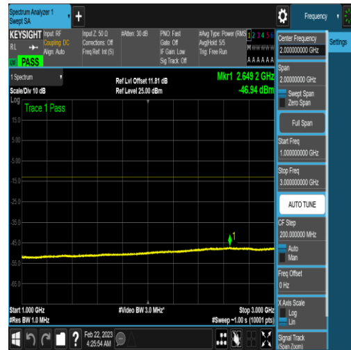
NTNV_N77-3450-3550_PC2_30_90_H_TID16_N/ A_1000_3000_#1
