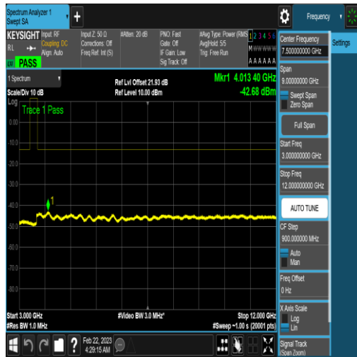
NTNV_N77-3450-3550_PC2_30_90_H_TID17_N/ A_3000_12000_#1
