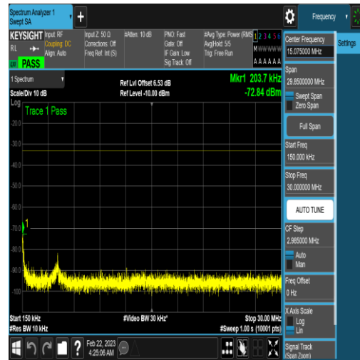
NTNV_N77-3450-3550_PC2_30_90_H_TID16_N/ A_0.15_30_#1
