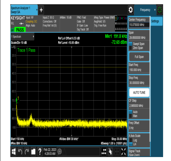
NTNV_N77-3450-3550_PC2_30_90_H_TID17_N/ A_0.15_30_#1
