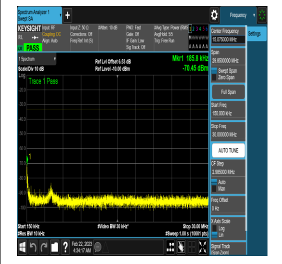
NTNV_N77-3450-3550_PC2_30_90_H_TID18_N/A_12000_20000_#1
