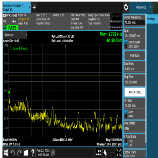
NTNV_N77-3450-3550_PC2_30_90_M_TID17_NV/ A_0.009_0.15_#1
