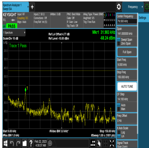
NTNV_N77-3450-3550_PC2_30_90_H_TID18_N/ A_0.009_0.15_#1
