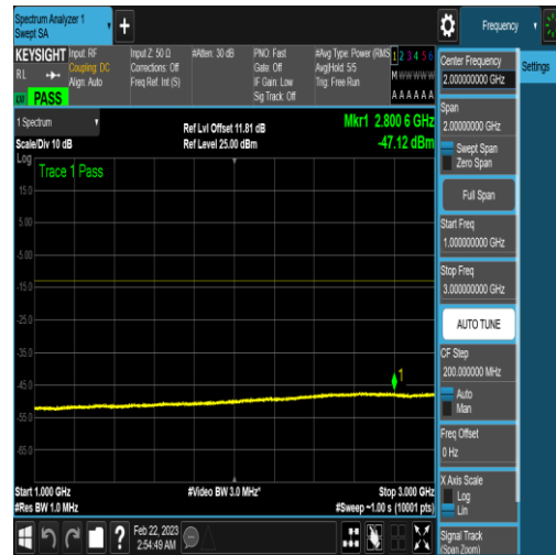
NTNV_N77-3450-3550_PC2_30_80_L_TID16_N/ A_1000_3000_#1
