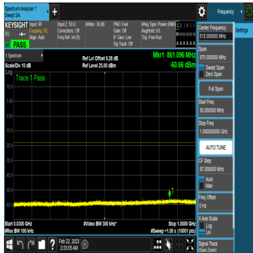
NTNV_N77-3450-3550_PC2_30_60_H_TID6_N/A _30_1000_#1
