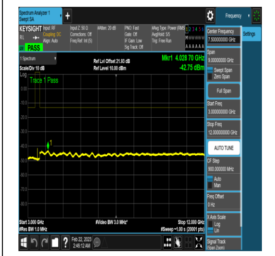
NTNV_N77-3450-3550_PC2_30_80_L_TID4_N/A _3000_12000_#1
