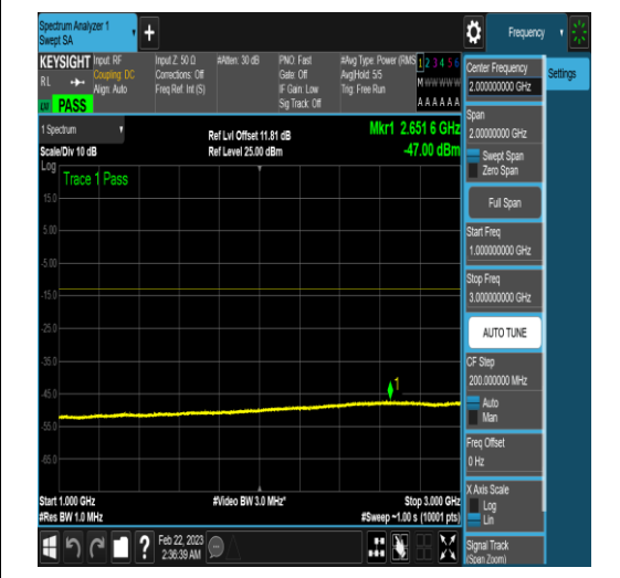
NTNV_N77-3450-3550_PC2_30_60_H_TID16_N/ A_1000_3000_#1
