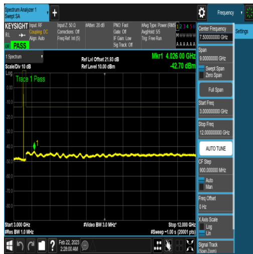
NTNV_N77-3450-3550_PC2_30_60_H_TID4_N/A _3000_12000_#1
