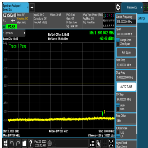
NTNV_N77-3450-3550_PC2_30_60_H_TID17_N/ A_30_1000_#1
