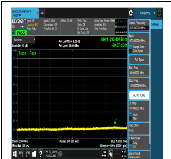
NTNV_N77-3450-3550_PC2_30_80_L_TID4_N/A _30_1000_#1
