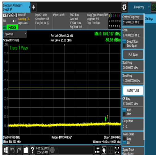
NTNV_N77-3450-3550_PC2_30_80_L_TID16_N/ A_30_1000_#1
