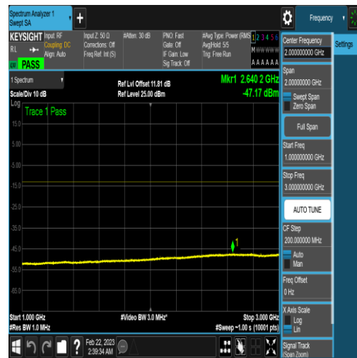
NTNV_N77-3450-3550_PC2_30_60_H_TID17_N/ A_1000_3000_#1
