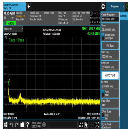
NTNV_N77-3450-3550_PC2_30_60_M_TID18_N/ A_0.15_30_#1
