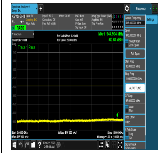
NTNV_N77-3450-3550_PC2_30_60_H_TID16_N/ A_30_1000_#1
