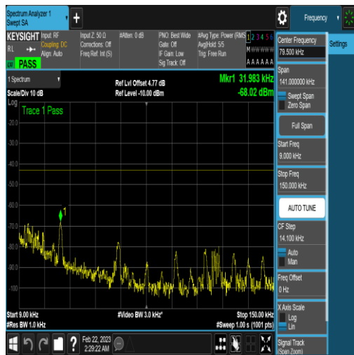
NTNV_N77-3450-3550_PC2_30_60_H_TID5_N/A _0.009_0.15_#1
