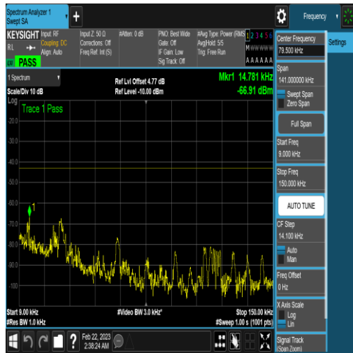
NTNV_N77-3450-3550_PC2_30_60_H_TID17_N/ A_0.009_0.15_#1
