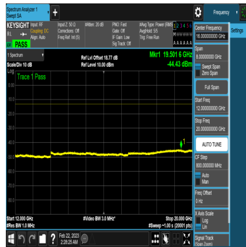
NTNV_N77-3450-3550_PC2_30_60_H_TID4_N/A _12000_20000_#1
