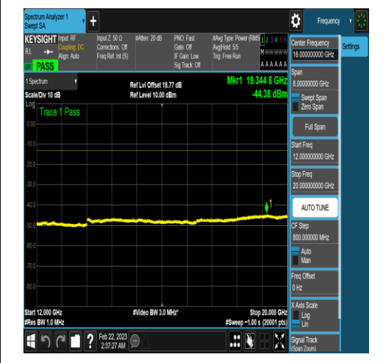
NTNV_N77-3450-3550_PC2_30_60_H_TID16_N/ A_1000_3000_#1
