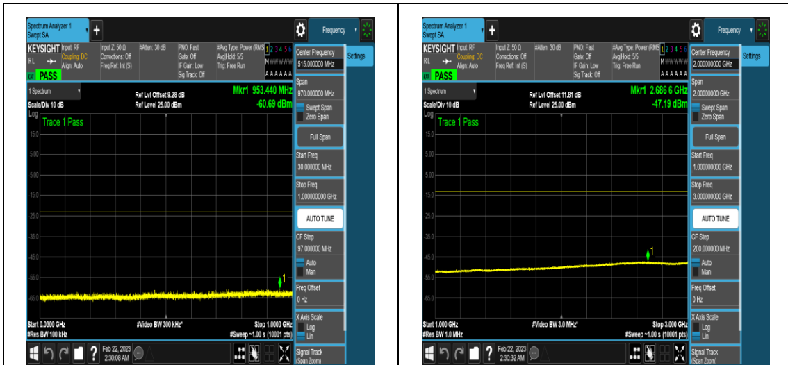
NTNV_N77-3450-3550_PC2_30_60_H_TID5_N/A _30_1000_#1
