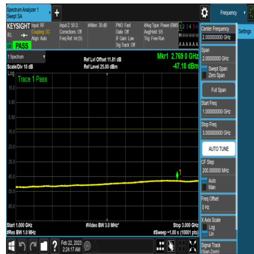
NTNV_N77-3450-3550_PC2_30_60_M_TID18_N/ A_1000_3000_#1
