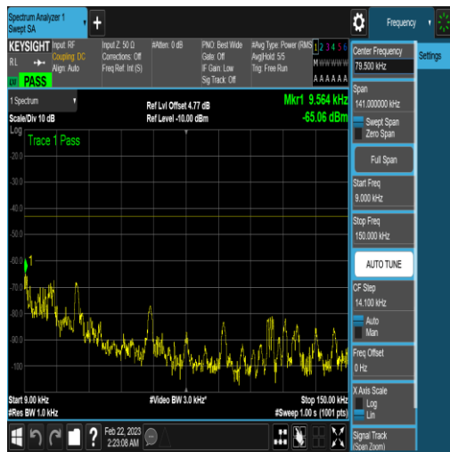
NTNV_N77-3450-3550_PC2_30_60_M_TID18_N/ A_0.009_0.15_#1
