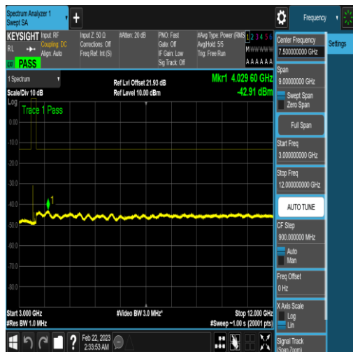
NTNV_N77-3450-3550_PC2_30_60_H_TID6_N/A _3000_12000_#1
