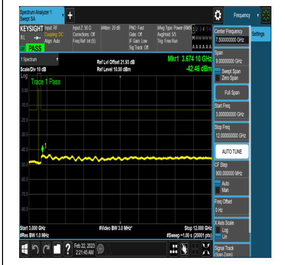
NTNV_N77-3450-3550_PC2_30_60_M_TID17_N/ A_30_1000_#1
