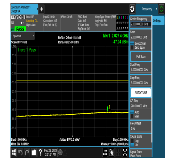
NTNV_N77-3450-3550_PC2_30_60_M_TID17_N/ A_1000_3000_#1
