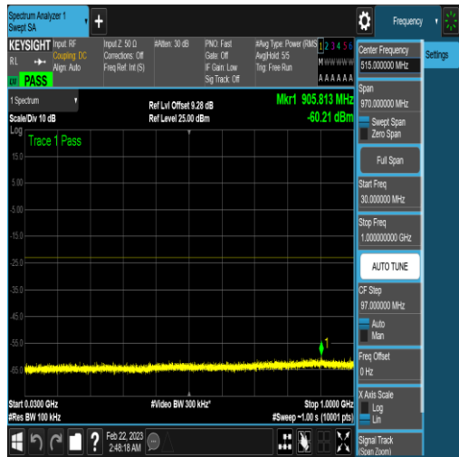
NTNV_N77-3450-3550_PC2_30_80_L_TID5_N/A _30_1000_#1
