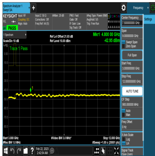
NTNV_N77-3450-3550_PC2_30_60_H_TID18_N/ A_3000_12000_#1
