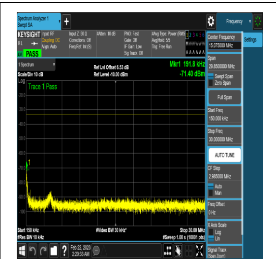
NTNV_N77-3450-3550_PC2_30_60_M_TID17_N/ A_0.15_30_#1
