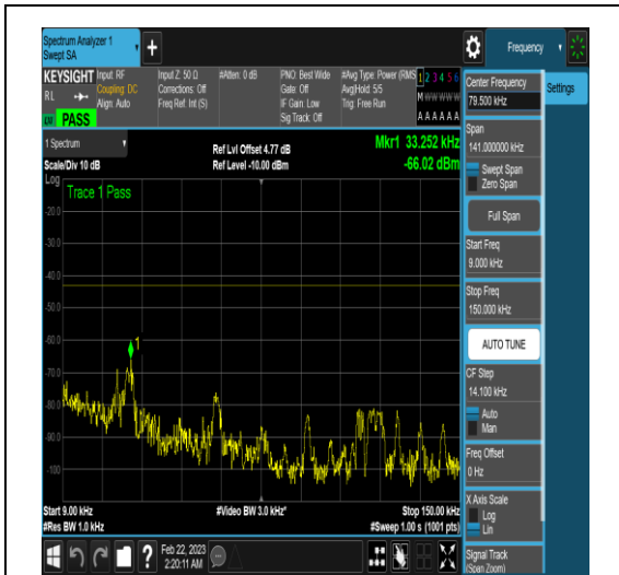
NTNV_N77-3450-3550_PC2_30_60_M_TID17_N/ A_0.009_0.15_#1
