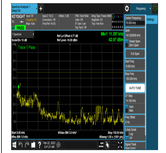
NTNV_N77-3450-3550_PC2_30_60_H_TID18_N/ A_0.009_0.15_#1
