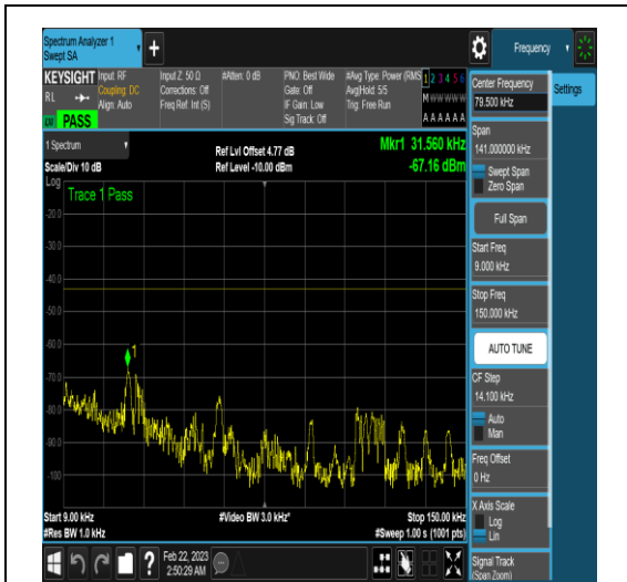
NTNV_N77-3450-3550_PC2_30_80_L_TID6_N/A _0.009_0.15_#1
