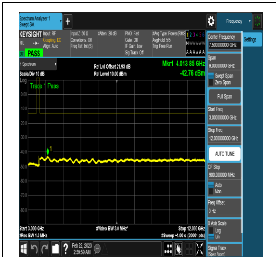
NTNV_N77-3450-3550_PC2_30_60_H_TID17_N/ A_3000_12000_#1
