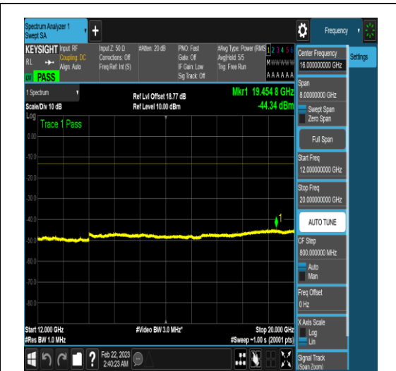
NTNV_N77-3450-3550_PC2_30_60_H_TID17_N/ A_12000_20000_#1
