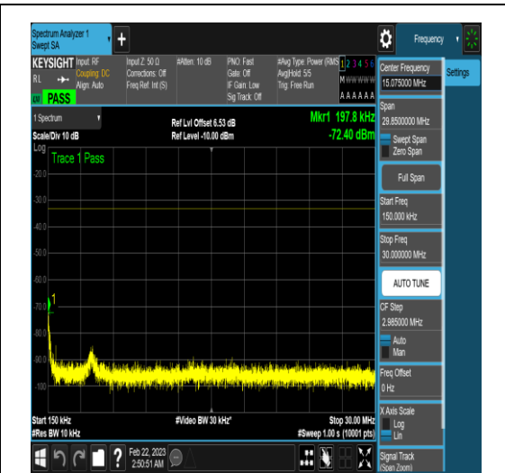
NTNV_N77-3450-3550_PC2_30_80_L_TID6_N/A _0.15_30_#1
