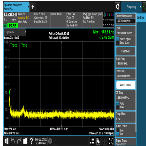
NTNV_N77-3450-3550_PC2_30_80_L_TID16_N/ A_0.15_30_#1
