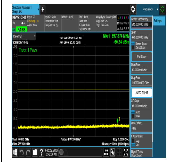
NTNV_N77-3450-3550_PC2_30_60_H_TID18_N/ A_0.009_0.15_#1
