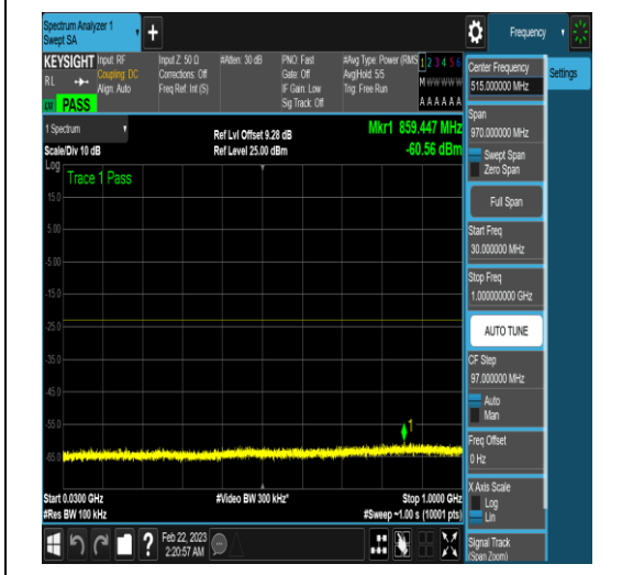
NTNV_N77-3450-3550_PC2_30_60_M_TID17_N/ A_30_1000_#1
