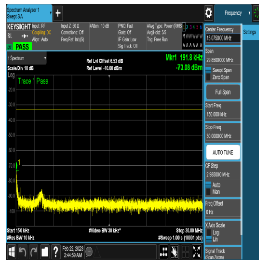
NTNV_N77-3450-3550_PC2_30_80_L_TID4_N/A _0.15_30_#1
