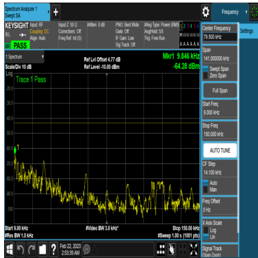
NTNV_N77-3450-3550_PC2_30_80_L_TID16_N/ A_0.009_0.15_#1
