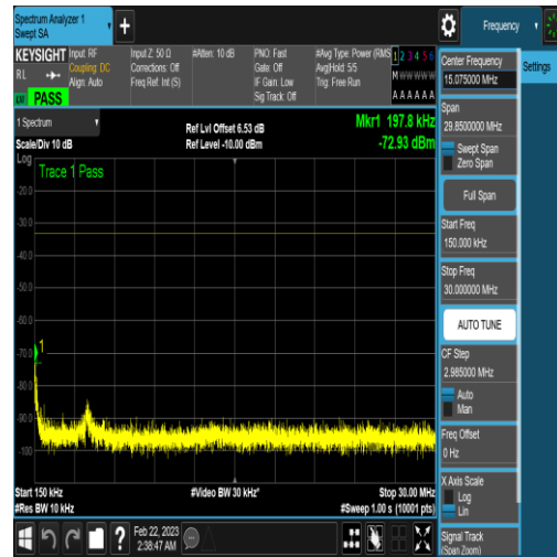
NTNV_N77-3450-3550_PC2_30_60_H_TID17_N/ A_0.15_30_#1
