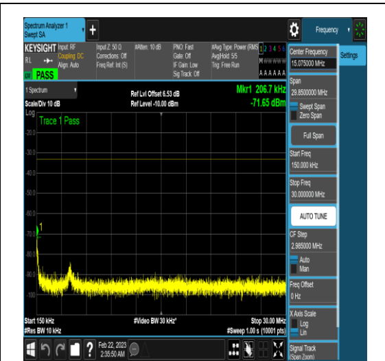
NTNV_N77-3450-3550_PC2_30_60_H_TID16_N/ A_0.15_30_#1
