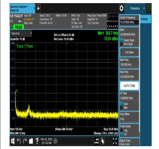
NTNV_N77-3450-3550_PC2_30_60_H_TID18_N/ A_0.15_30_#1
