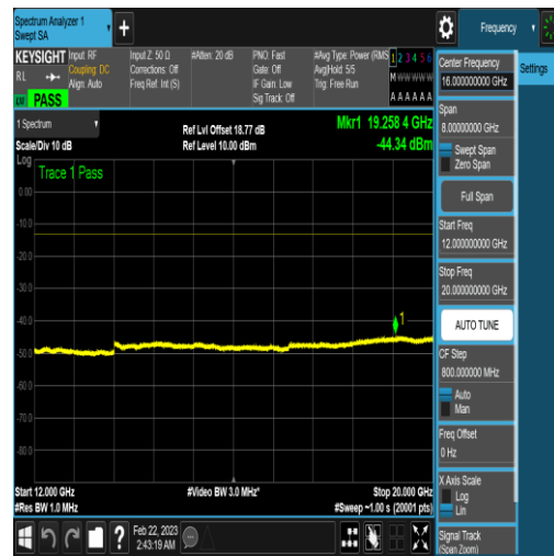
NTNV_N77-3450-3550_PC2_30_60_H_TID18_N/ A_12000_20000_#1
