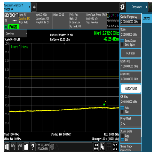
NTNV_N77-3450-3550_PC2_30_60_H_TID6_N/A _1000_3000_#1
