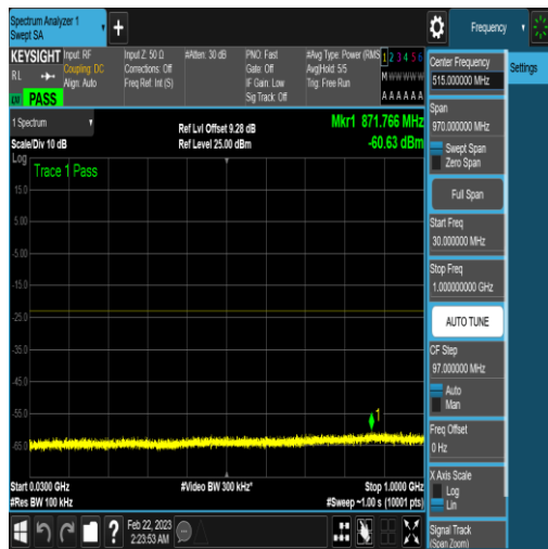
NTNV_N77-3450-3550_PC2_30_60_M_TID18_N/ A_30_1000_#1
