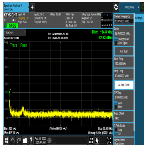
NTNV_N77-3450-3550_PC2_30_60_H_TID5_N/A _0.15_30_#1
