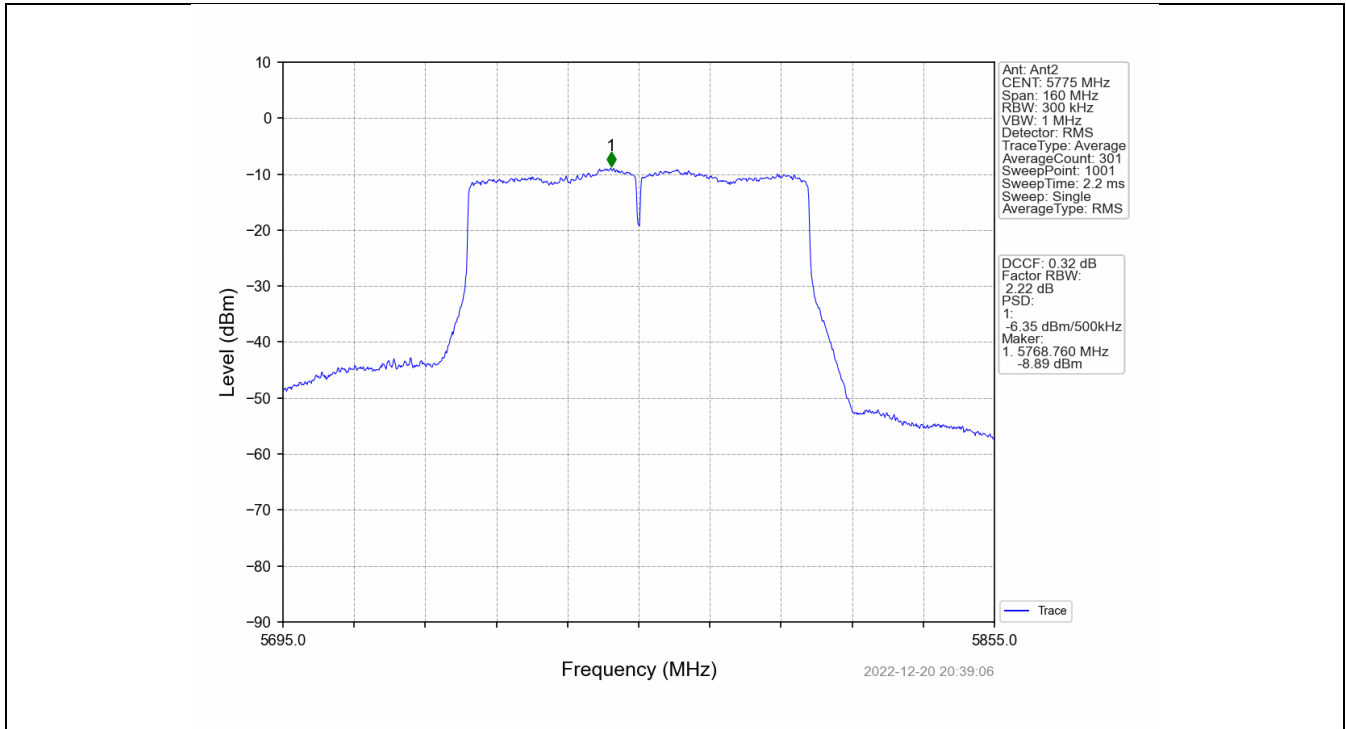
802.11ac(VHT80)_MCH_5775MHz_MIMO_NTNV
