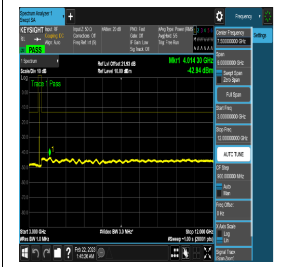
NTNV_N77-3450-3550_PC2_30_50_H_TID17_N/A_3000_12000_#1
