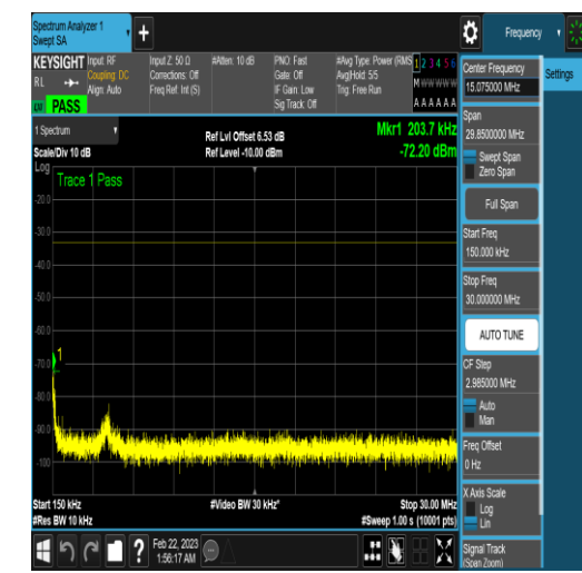
NTNV_N77-3450-3550_PC2_30_60_L_TID6_N/A _0.15_30_#1
