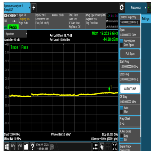
NTNV_N77-3450-3550_PC2_30_50_H_TID18_N/ A_12000_20000_#1
