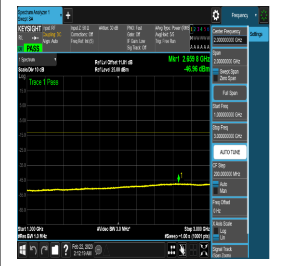
NTNV_N77-3450-3550_PC2_30_60_M_TID5_N/A _0.15_30_#1
