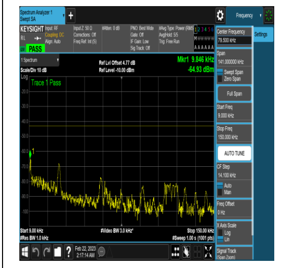
NTNV_N77-3450-3550_PC2_30_60_M_TID6_N/A _3000_12000_#1
