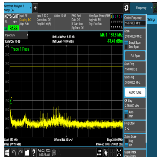
NTNV_N77-3450-3550_PC2_30_60_L_TID16_N/ A_0.15_30_#1
