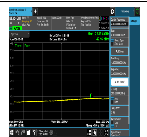
NTNV_N77-3450-3550_PC2_30_60_M_TID6_N/A _1000_3000_#1
