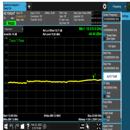
NTNV_N77-3450-3550_PC2_30_60_M_TID16_NV/ A_12000_20000_#1
