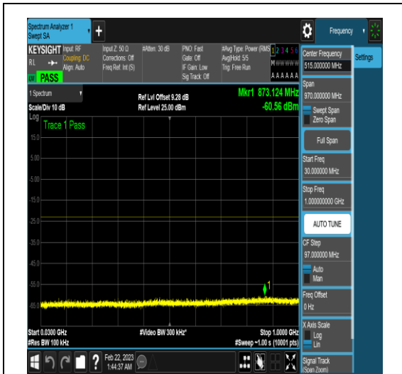
NTNV_N77-3450-3550_PC2_30_50_H_TID17_N/A_30_1000_#1
