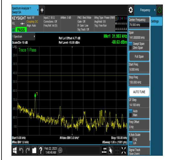
NTNV_N77-3450-3550_PC2_30_50_H_TID17_N/A_3000_12000_#1
