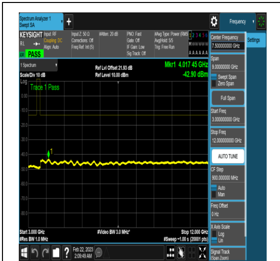
NTNV_N77-3450-3550_PC2_30_60_M_TID4_N/A _3000_12000_#1
