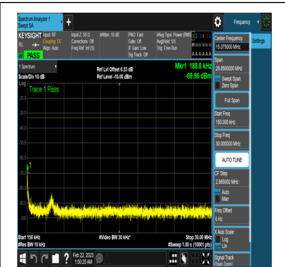
NTNV_N77-3450-3550_PC2_30_60_L_TID4_N/A _0.15_30_#1
