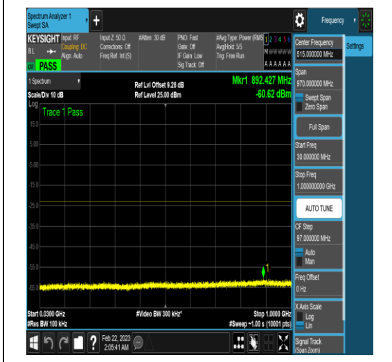
NTNV_N77-3450-3550_PC2_30_60_L_TID18_N/ A_30_1000_#1
