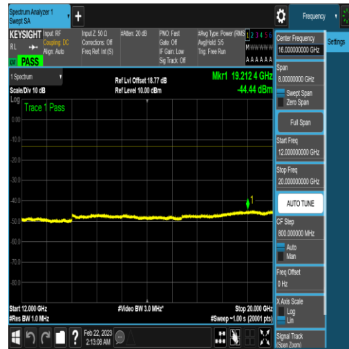
NTNV_N77-3450-3550_PC2_30_60_M_TID5_N/A _12000_20000_#1
