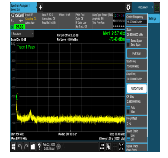
NTNV_N77-3450-3550_PC2_30_60_L_TID16_N/ A_12000_20000_#1
