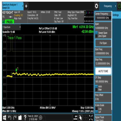
NTNV_N77-3450-3550_PC2_30_60_M_TID16_NV/ A_3000_12000_#1
