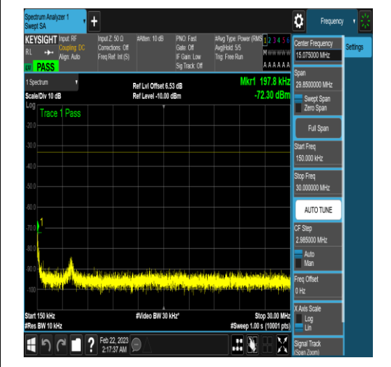
NTNV_N77-3450-3550_PC2_30_60_M_TID6_N/A _12000_20000_#1
