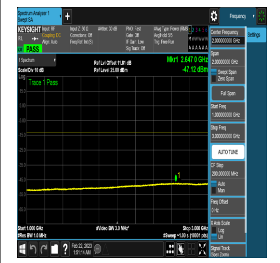
NTNV_N77-3450-3550_PC2_30_60_L_TID4_N/A _1000_3000_#1
