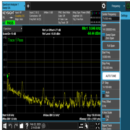
NTNV_N77-3450-3550_PC2_30_60_M_TID6_N/A _0.009_0.15_#1
