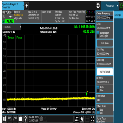
NTNV_N77-3450-3550_PC2_30_60_M_TID16_NV/ A_30_1000_#1
