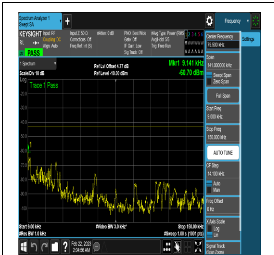
NTNV_N77-3450-3550_PC2_30_60_L_TID18_N/ A_0.009_0.15_#1
