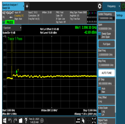
NTNV_N77-3450-3550_PC2_30_50_H_TID18_N/ A_3000_12000_#1
