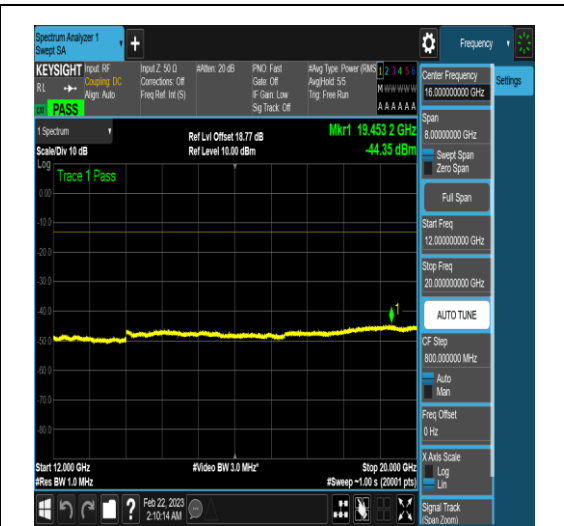
NTNV_N77-3450-3550_PC2_30_60_M_TID4_N/A _12000_20000_#1
