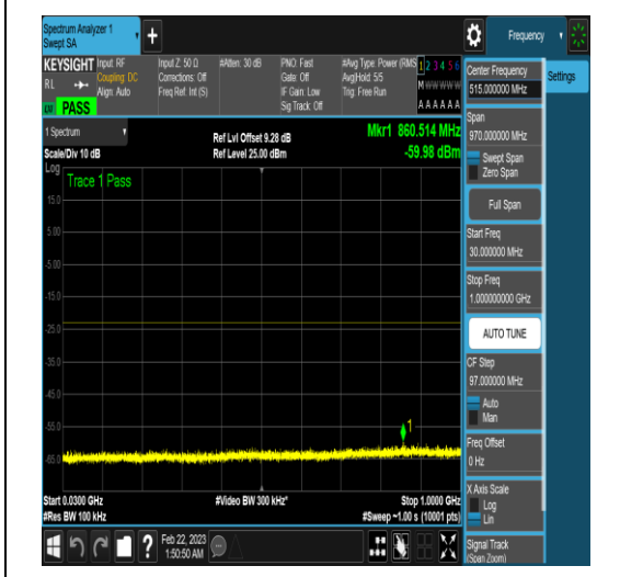
NTNV_N77-3450-3550_PC2_30_60_L_TID4_N/A _30_1000_#1
