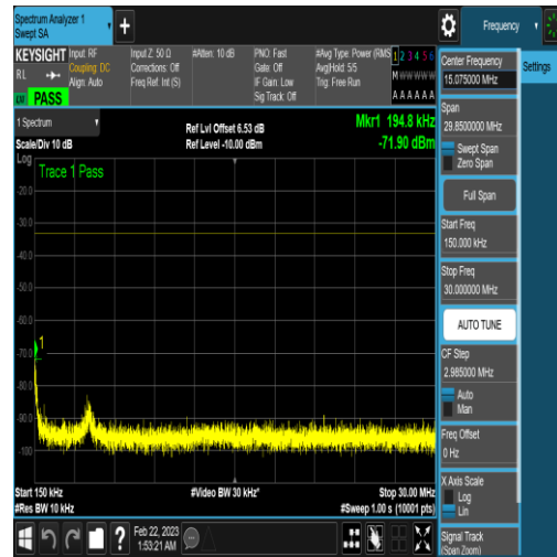
NTNV_N77-3450-3550_PC2_30_60_L_TID5_N/A _0.15_30_#1
