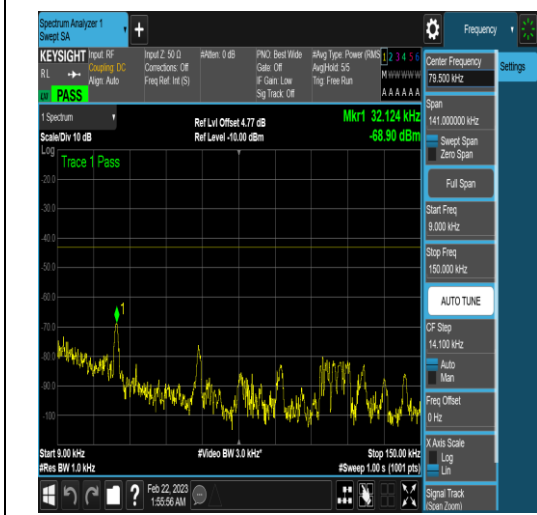
NTNV_N77-3450-3550_PC2_30_60_L_TID6_N/A _0.009_0.15_#1
