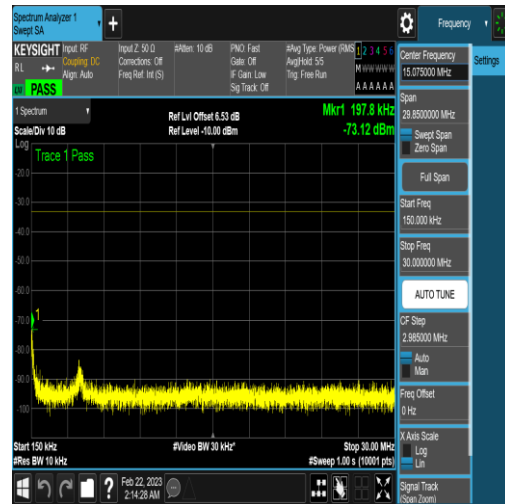
NTNV_N77-3450-3550_PC2_30_60_M_TID6_N/A _0.15_30_#1
