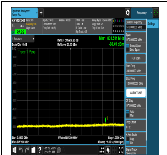
NTNV_N77-3450-3550_PC2_30_60_M_TID6_N/A _30_1000_#1
