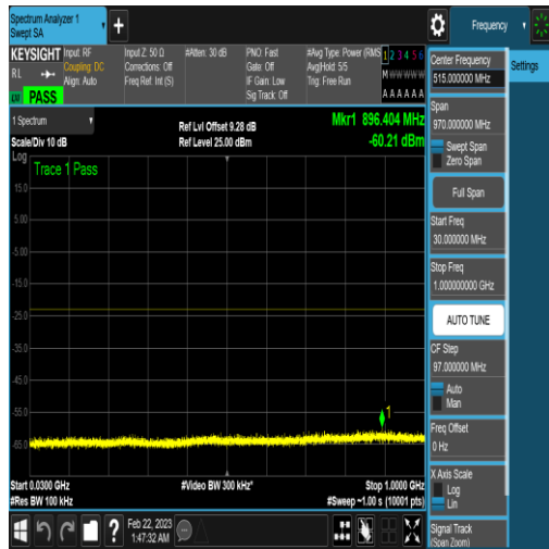
NTNV_N77-3450-3550_PC2_30_50_H_TID18_N/ A_30_1000_#1
