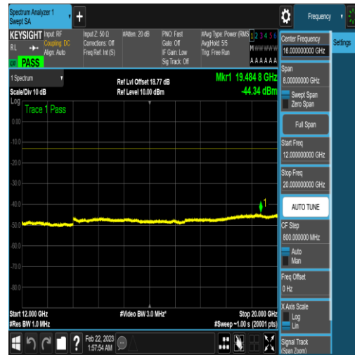
NTNV_N77-3450-3550_PC2_30_60_L_TID6_N/A _12000_20000_#1
