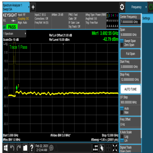
NTNV_N77-3450-3550_PC2_30_60_M_TID5_N/A _3000_12000_#1
