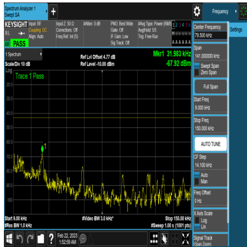
NTNV_N77-3450-3550_PC2_30_60_L_TID5_N/A _0.009_0.15_#1
