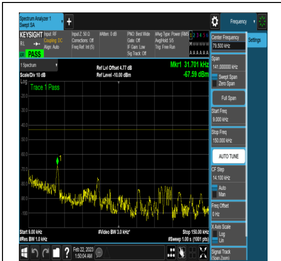
NTNV_N77-3450-3550_PC2_30_60_L_TID4_N/A _0.009_0.15_#1
