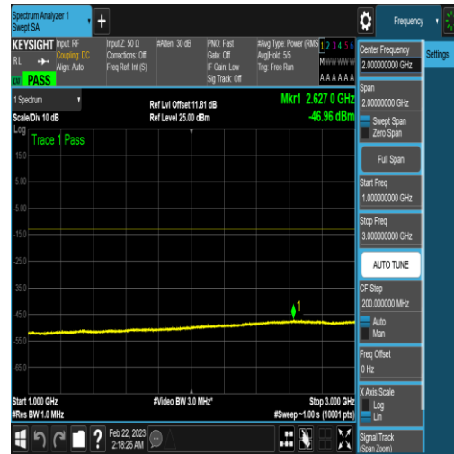
NTNV_N77-3450-3550_PC2_30_60_M_TID16_NV/ A_1000_3000_#1
