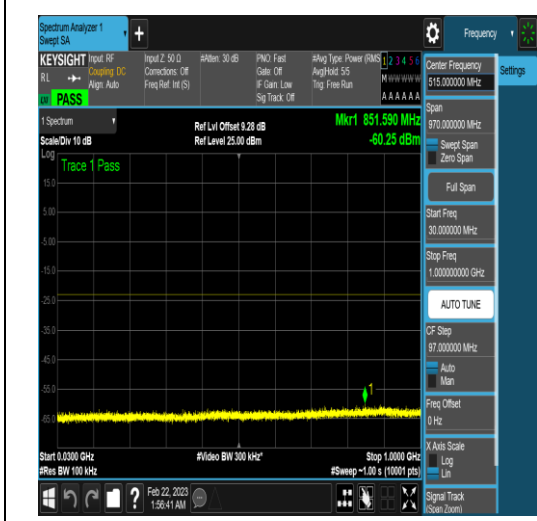
NTNV_N77-3450-3550_PC2_30_60_L_TID6_N/A _0.009_0.15_#1
