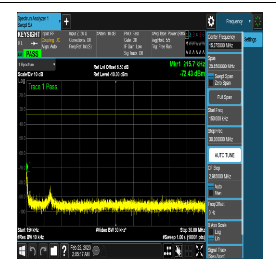
NTNV_N77-3450-3550_PC2_30_60_L_TID18_N/ A_0.15_30_#1
