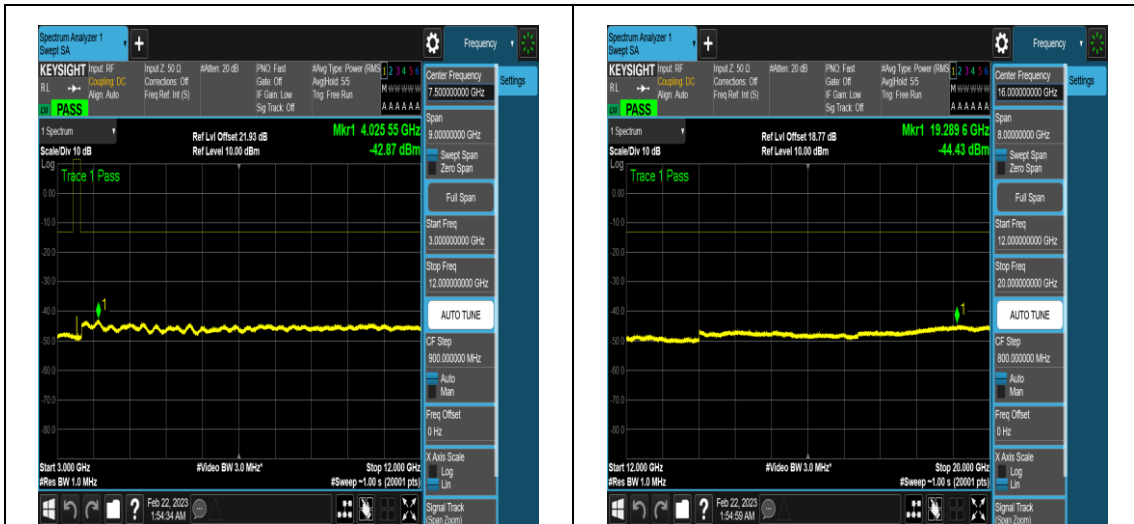
NTNV_N77-3450-3550_PC2_30_60_L_TID5_N/A _3000_12000_#1
