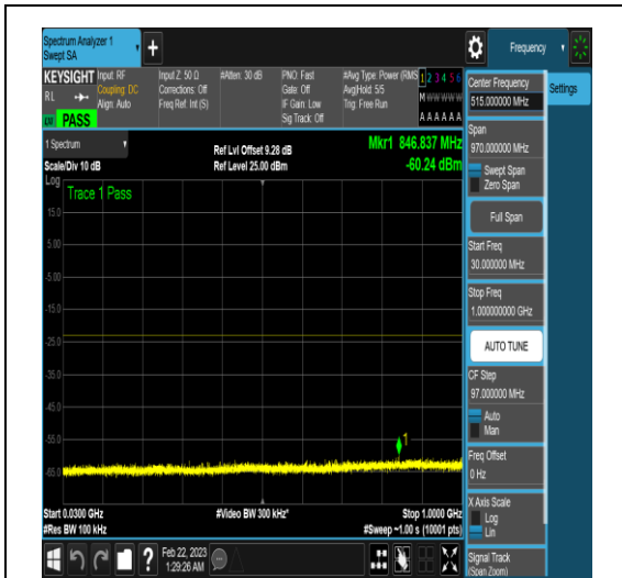
NTNV_N77-3450-3550_PC2_30_50_M_TID18_N/A_30_1000_#1
