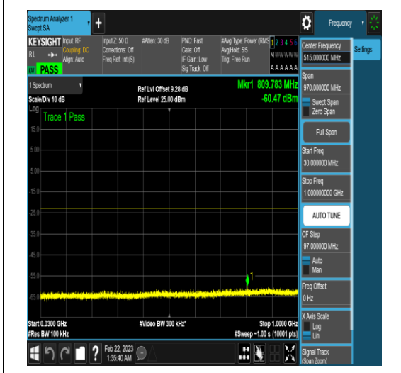
NTNV_N77-3450-3550_PC2_30_50_H_TID5_N/A _30_1000_#1
