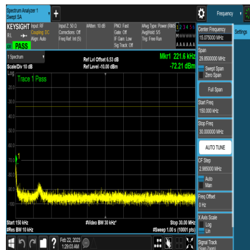
NTNV_N77-3450-3550_PC2_30_50_M_TID18_N/ A_0.15_30_#1
