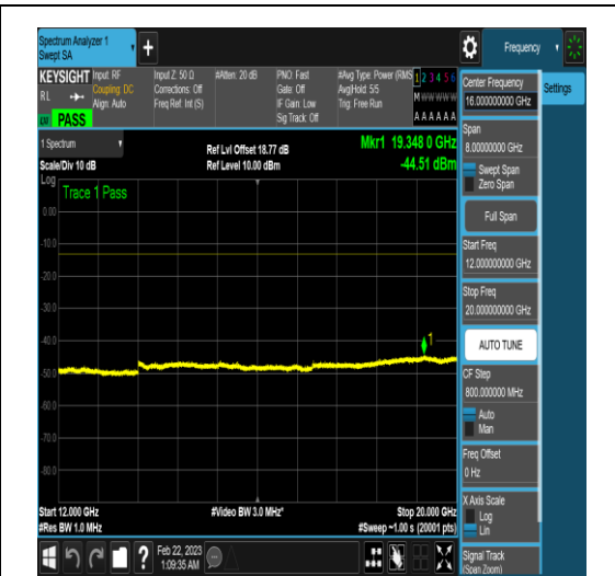
NTNV_N77-3450-3550_PC2_30_50_L_TID17_N/ A_12000_20000_#1
