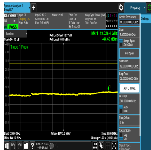
NTNV_N77-3450-3550_PC2_30_50_M_TID5_N/A _12000_20000_#1
