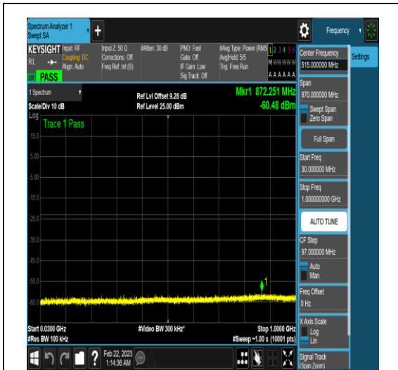
NTNV_N77-3450-3550_PC2_30_50_M_TID4_N/A _30_1000_#1
