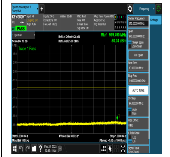
NTNV_N77-3450-3550_PC2_30_40_M_TID18_N/A_30_1000_#1
