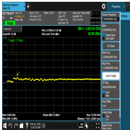
NTNV_N77-3450-3550_PC2_30_40_H_TID5_N/A _3000_12000_#1
