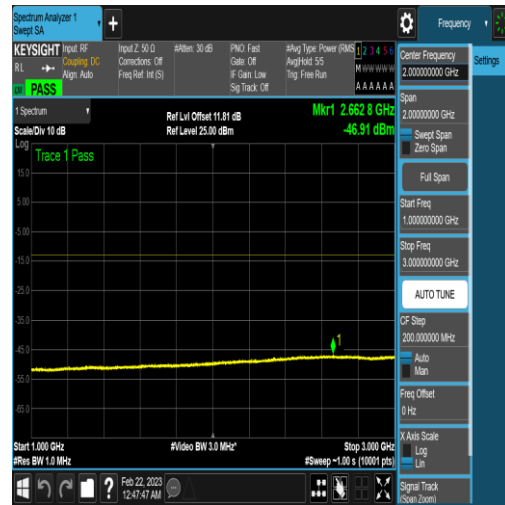
NTNV_N77-3450-3550_PC2_30_40_H_TID16_N/ A_1000_3000_#1
