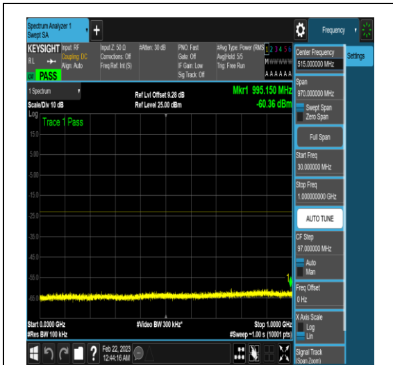
NTNV_N77-3450-3550_PC2_30_40_H_TID6_N/A _30_1000_#1
