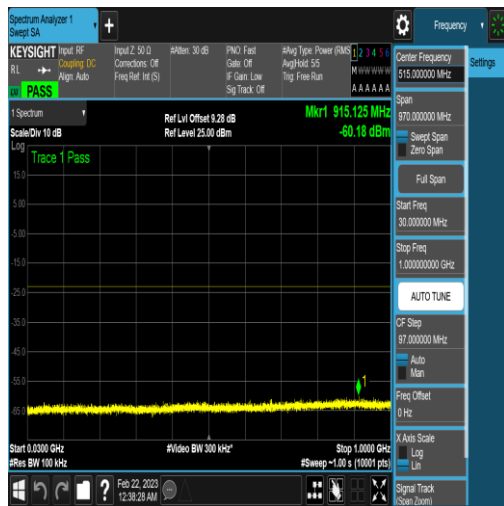
NTNV_N77-3450-3550_PC2_30_40_H_TID4_N/A _30_1000_#1
