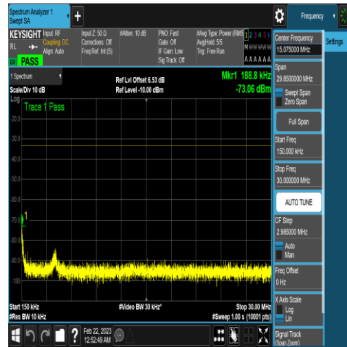
NTNV_N77-3450-3550_PC2_30_40_H_TID18_N/ A_0.15_30_#1
