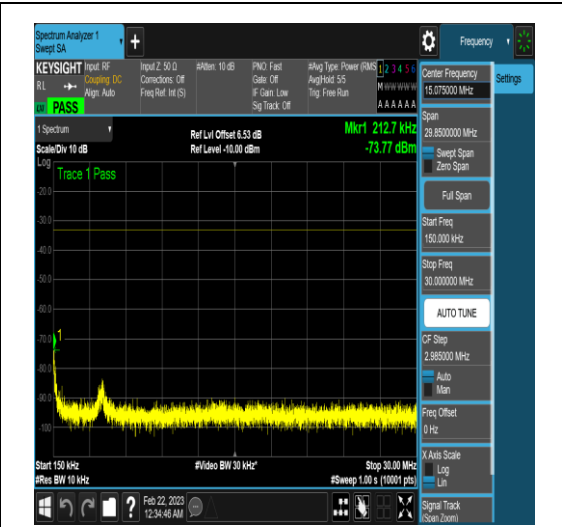
NTNV_N77-3450-3550_PC2_30_40_M_TID18_N/A_0.15_30_#1
