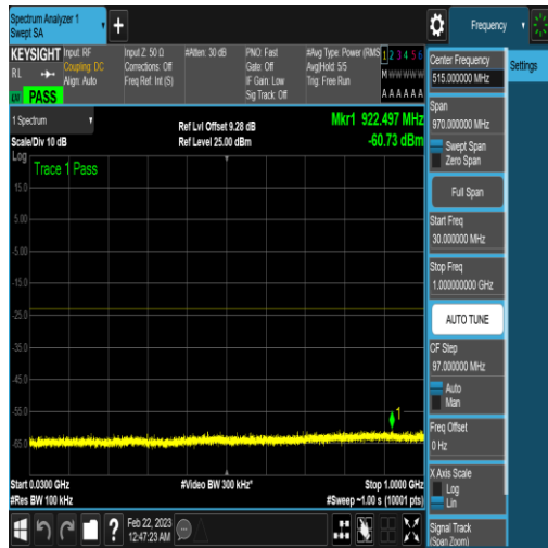
NTNV_N77-3450-3550_PC2_30_40_H_TID16_N/ A_30_1000_#1
