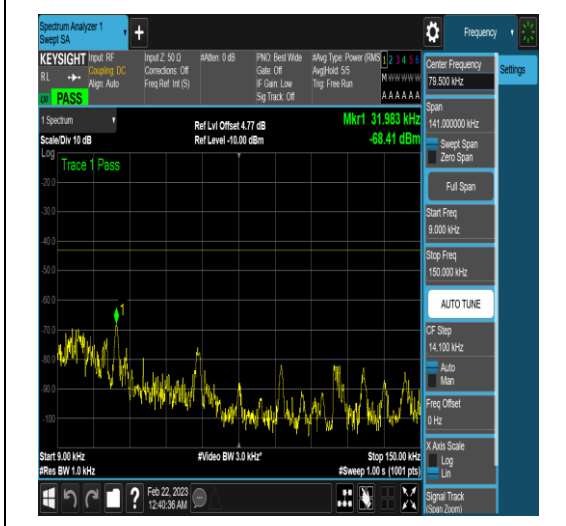
NTNV_N77-3450-3550_PC2_30_40_H_TID5_N/A _0.009_0.15_#1
