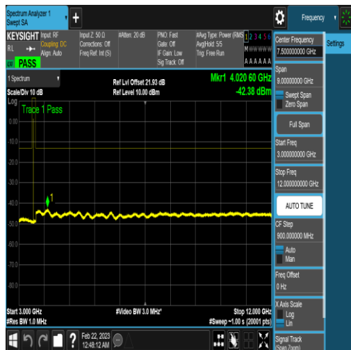
NTNV_N77-3450-3550_PC2_30_40_H_TID16_N/ A_3000_12000_#1
