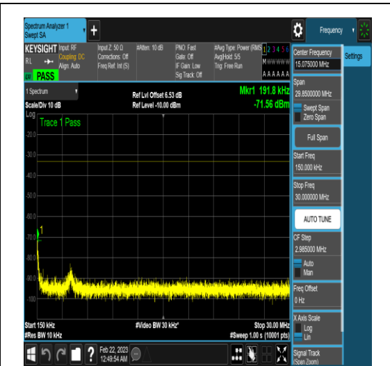
NTNV_N77-3450-3550_PC2_30_40_H_TID17_N/ A_0.15_30_#1
