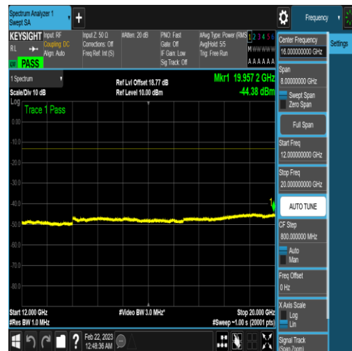
NTNV_N77-3450-3550_PC2_30_40_H_TID16_N/ A_12000_20000_#1
