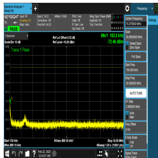
NTNV_N77-3450-3550_PC2_30_40_H_TID6_N/A _0.15_30_#1
