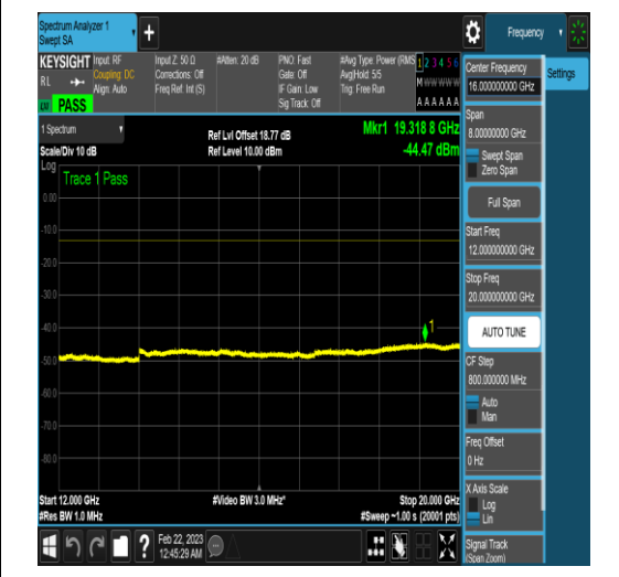
NTNV_N77-3450-3550_PC2_30_40_H_TID6_N/A _12000_20000_#1
