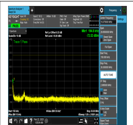
NTNV_N77-3450-3550_PC2_30_50_L_TID16_N/ A_0.15_30_#1
