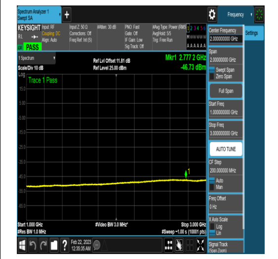
NTNV_N77-3450-3550_PC2_30_40_M_TID18_N/A_1000_3000_#1
