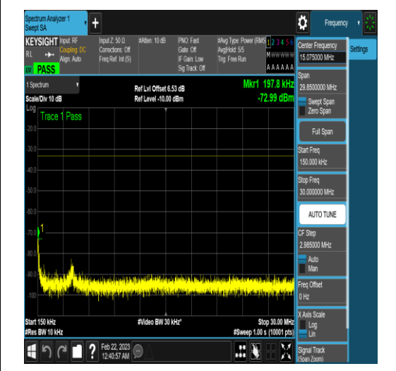
NTNV_N77-3450-3550_PC2_30_40_H_TID5_N/A _0.15_30_#1
