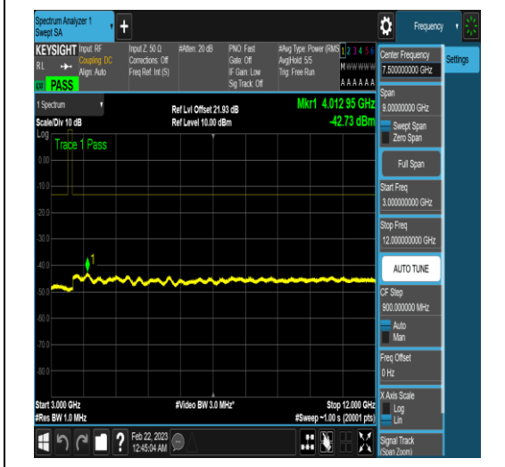
NTNV_N77-3450-3550_PC2_30_40_H_TID6_N/A _3000_12000_#1
