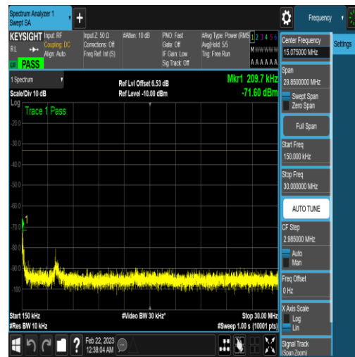
NTNV_N77-3450-3550_PC2_30_40_H_TID4_N/A _0.15_30_#1
