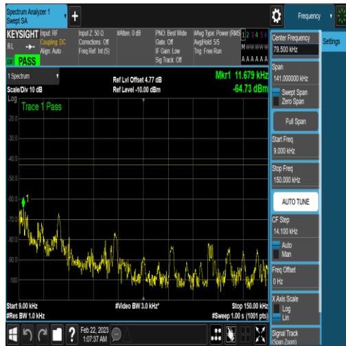
NTNV_N77-3450-3550_PC2_30_50_L_TID17_N/ A_0.009_0.15_#1
