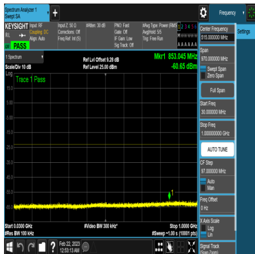
NTNV_N77-3450-3550_PC2_30_40_H_TID18_N/ A_30_1000_#1
