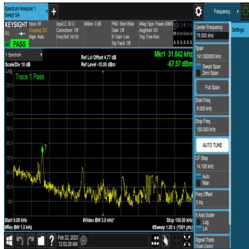
NTNV_N77-3450-3550_PC2_30_40_H_TID18_N/ A_0.009_0.15_#1
