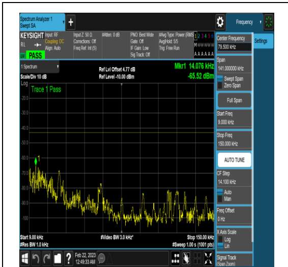
NTNV_N77-3450-3550_PC2_30_40_H_TID17_N/ A_0.009_0.15_#1
