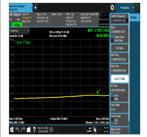
NTNV_N77-3450-3550_PC2_30_40_H_TID17_N/ A_1000_3000_#1
