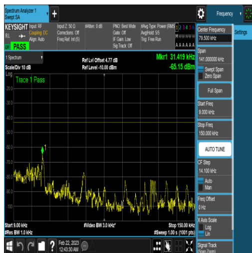
NTNV_N77-3450-3550_PC2_30_40_H_TID6_N/A _0.009_0.15_#1
