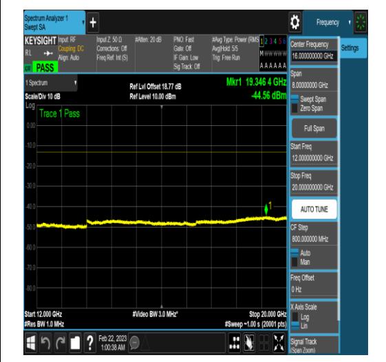
NTNV_N77-3450-3550_PC2_30_50_L_TID5_N/A _12000_20000_#1
