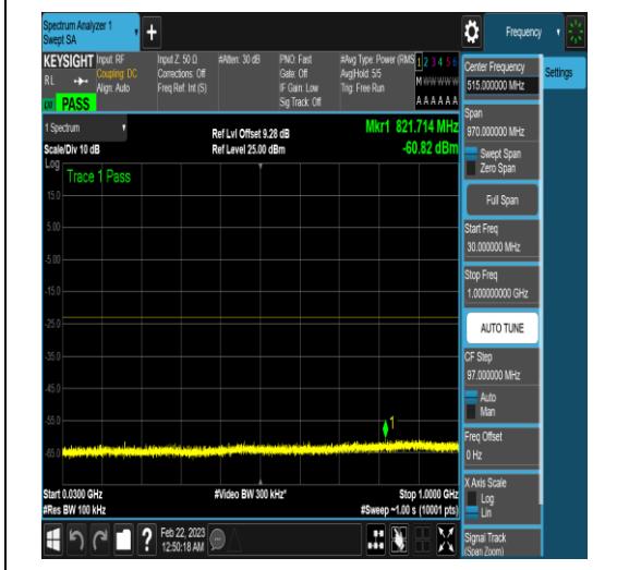
NTNV_N77-3450-3550_PC2_30_40_H_TID17_N/ A_30_1000_#1
