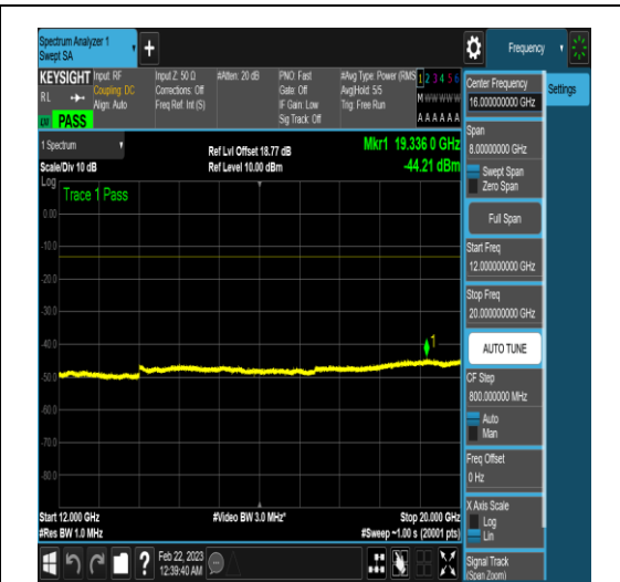
NTNV_N77-3450-3550_PC2_30_40_H_TID4_N/A _12000_20000_#1
