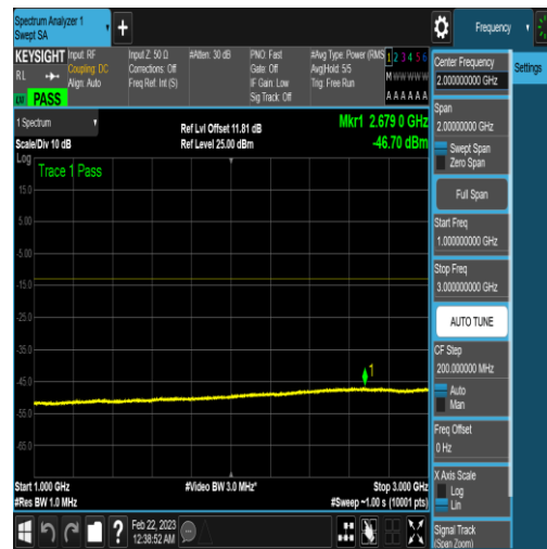
NTNV_N77-3450-3550_PC2_30_40_H_TID4_N/A _1000_3000_#1
