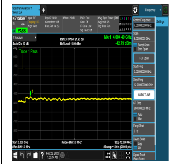
NTNV_N77-3450-3550_PC2_30_50_L_TID5_N/A _3000_12000_#1
