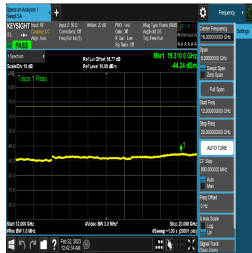
NTNV_N77-3450-3550_PC2_30_40_H_TID5_N/A _12000_20000_#1
