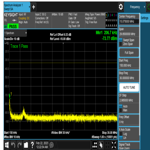
NTNV_N77-3450-3550_PC2_30_40_M_TID5_N/A _0.15_30_#1
