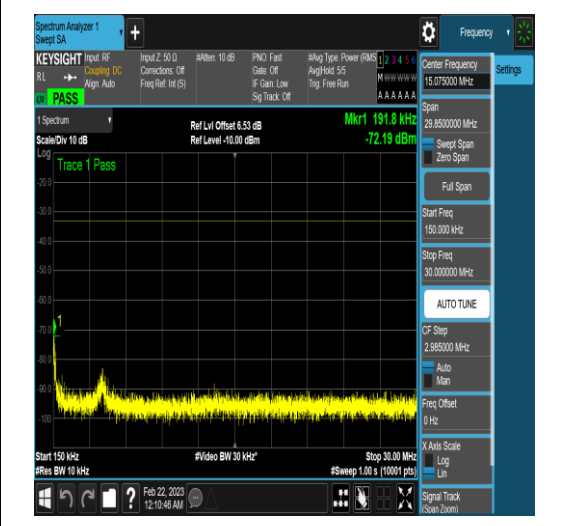
NTNV_N77-3450-3550_PC2_30_40_L_TID16_N/ A_0.15_30_#1
