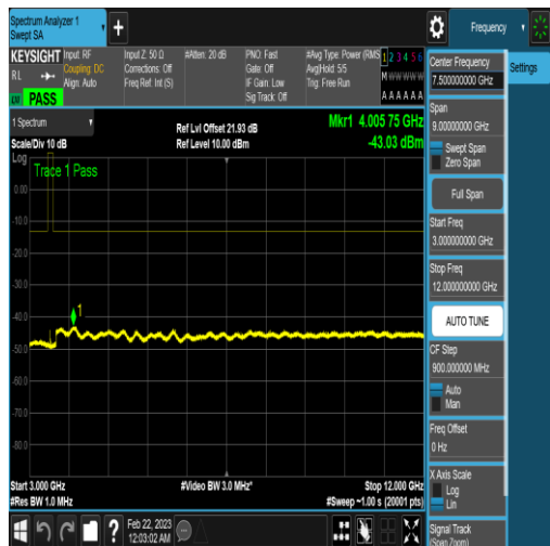
NTNV_N77-3450-3550_PC2_30_40_L_TID4_N/A _3000_12000_#1
