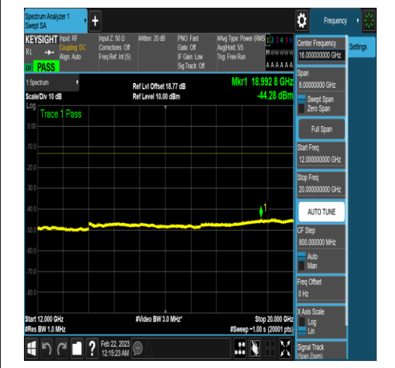
NTNV_N77-3450-3550_PC2_30_40_L_TID17_N/ A_12000_20000_#1
