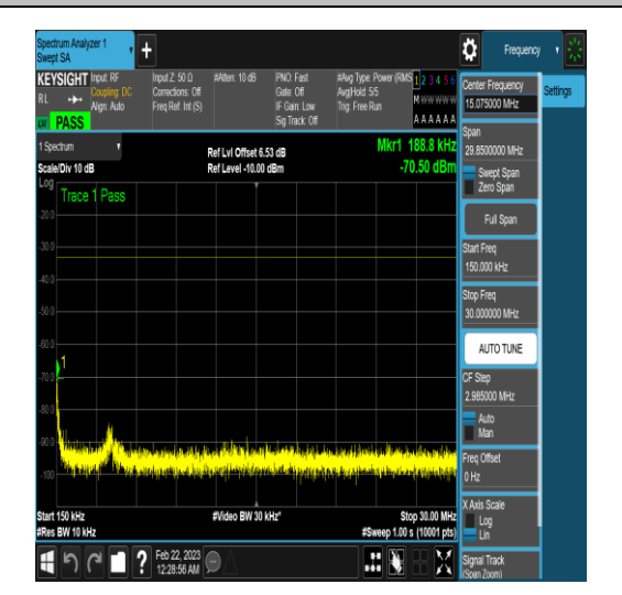
NTNV_N77-3450-3550_PC2_30_40_M_TID16_N/ A_0.15_30_#1
