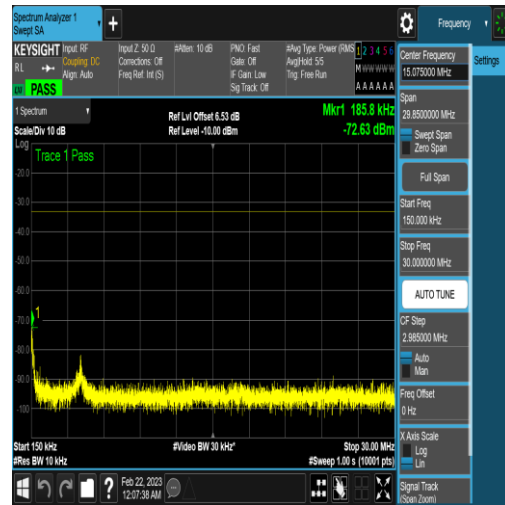
NTNV_N77-3450-3550_PC2_30_40_L_TID6_N/A _0.15_30_#1
