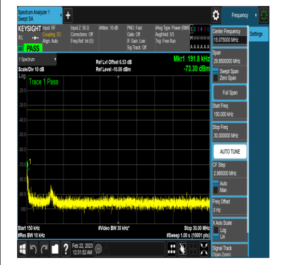
NTNV_N77-3450-3550_PC2_30_40_M_TID16_N/A_12000_20000_#1
