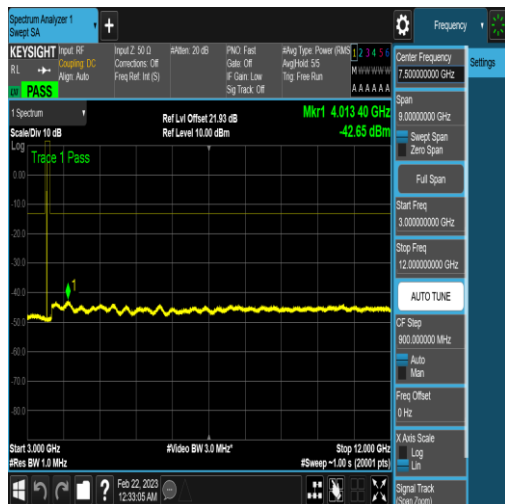
NTNV_N77-3450-3550_PC2_30_40_M_TID17_N/ A_3000_12000_#1
