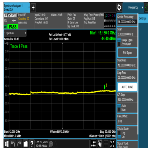
NTNV_N77-3450-3550_PC2_30_40_M_TID17_N/ A_12000_20000_#1
