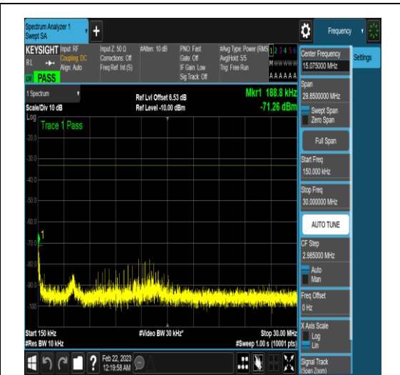
NTNV_N77-3450-3550_PC2_30_40_M_TID4_N/A _0.15_30_#1
