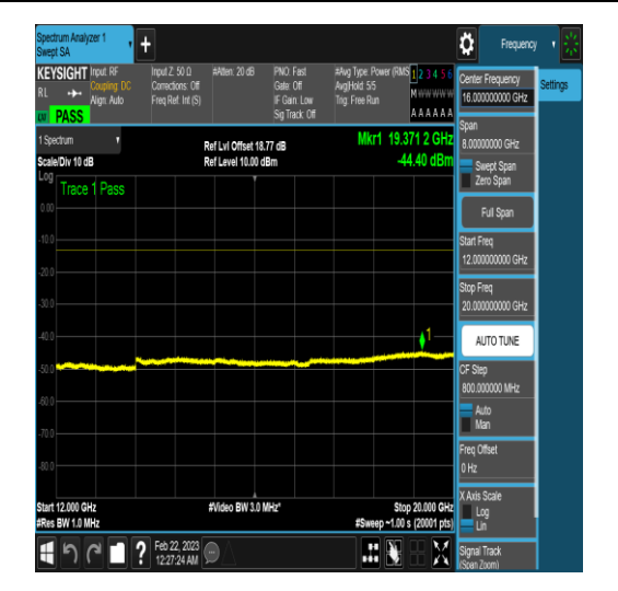
NTNV_N77-3450-3550_PC2_30_40_M_TID6_N/A _12000_20000_#1
