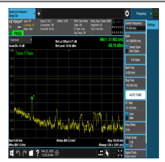
NTNV_N77-3450-3550_PC2_30_40_M_TID16_N/ A_0.009_0.15_#1
