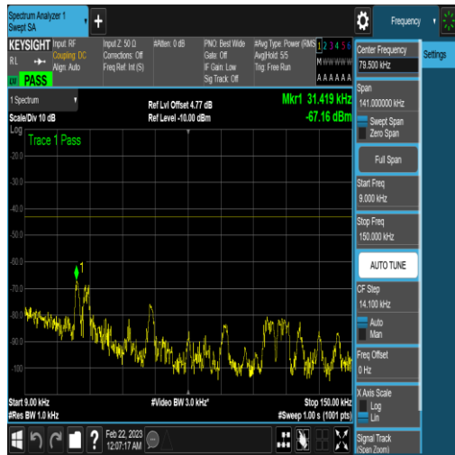
NTNV_N77-3450-3550_PC2_30_40_L_TID6_N/A _0.009_0.15_#1
