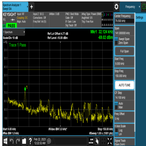
NTNV_N77-3450-3550_PC2_30_40_M_TID5_N/A _0.009_0.15_#1
