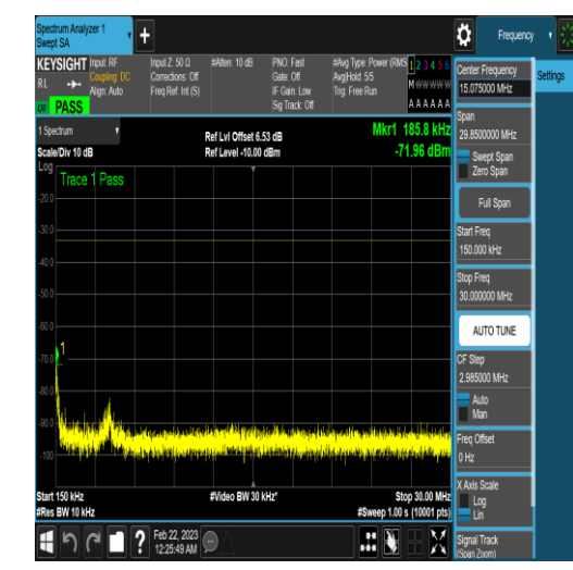
NTNV_N77-3450-3550_PC2_30_40_M_TID6_N/A _0.15_30_#1
