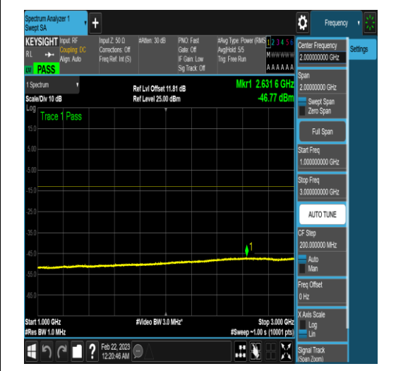
NTNV_N77-3450-3550_PC2_30_40_M_TID4_N/A _1000_3000_#1
