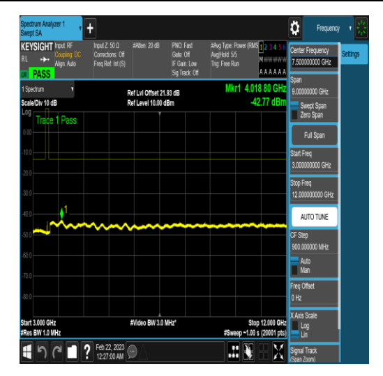
NTNV_N77-3450-3550_PC2_30_40_M_TID6_N/A _3000_12000_#1
