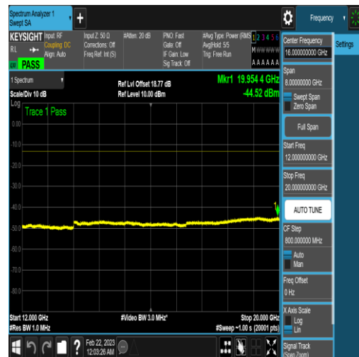
NTNV_N77-3450-3550_PC2_30_40_L_TID4_N/A _12000_20000_#1
