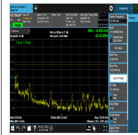
NTNV_N77-3450-3550_PC2_30_40_M_TID6_N/A _0.009_0.15_#1
