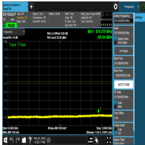
NTNV_N77-3450-3550_PC2_30_40_M_TID17_N/ A_30_1000_#1
