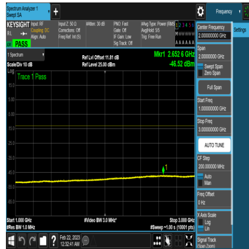
NTNV_N77-3450-3550_PC2_30_40_M_TID17_N/ A_1000_3000_#1
