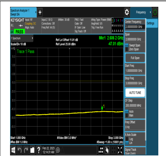
NTNV_N77-3450-3550_PC2_30_40_L_TID17_N/ A_1000_3000_#1
