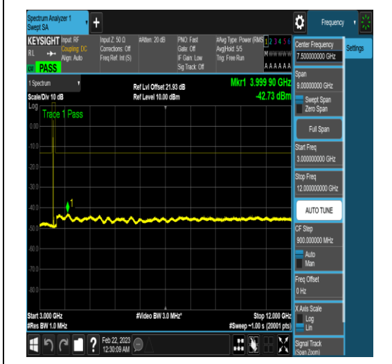
NTNV_N77-3450-3550_PC2_30_40_M_TID16_N/A_3000_12000_#1
