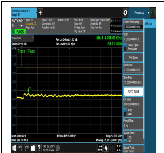
NTNV_N77-3450-3550_PC2_30_40_L_TID6_N/A _3000_12000_#1
