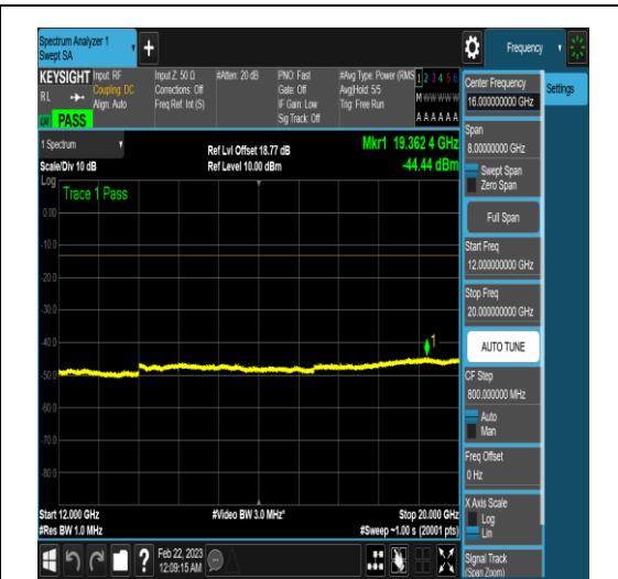
NTNV_N77-3450-3550_PC2_30_40_L_TID6_N/A _12000_20000_#1
