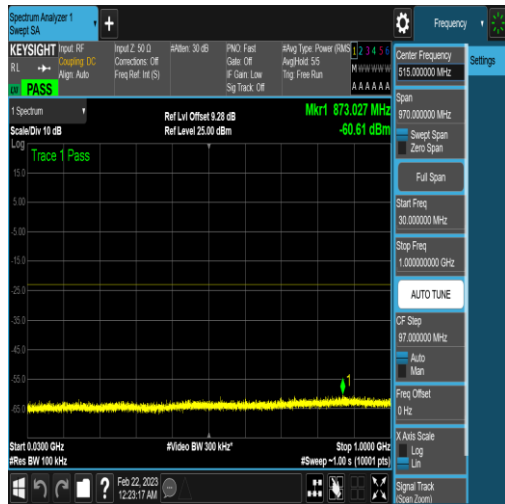
NTNV_N77-3450-3550_PC2_30_40_M_TID5_N/A _30_1000_#1
