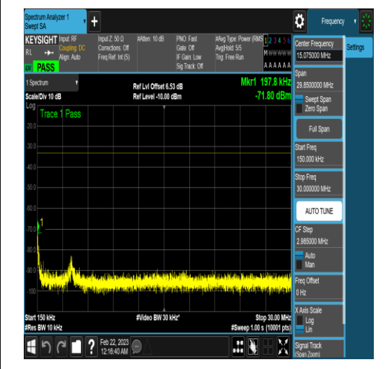
NTNV_N77-3450-3550_PC2_30_40_L_TID17_N/ A_12000_20000_#1
