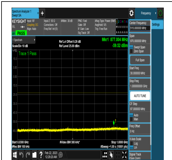
NTNV_N77-3450-3550_PC2_30_40_M_TID16_N/A_30_1000_#1
