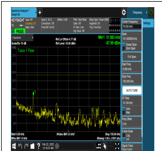
NTNV_N77-3450-3550_PC2_30_40_M_TID4_N/A _0.009_0.15_#1
