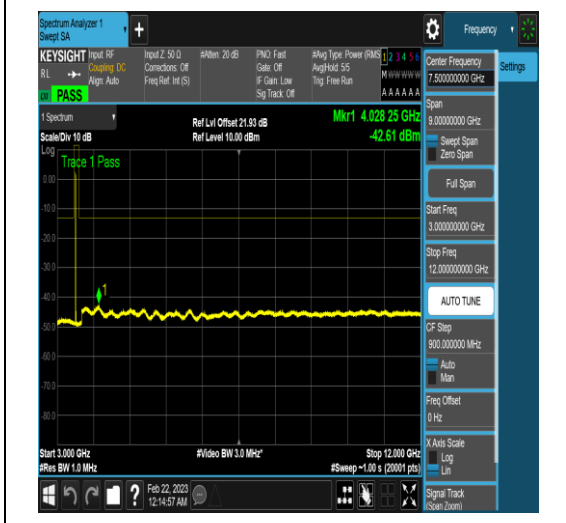
NTNV_N77-3450-3550_PC2_30_40_L_TID17_N/ A_3000_12000_#1
