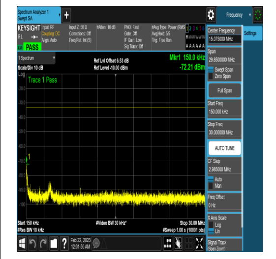
NTNV_N77-3450-3550_PC2_30_20_H_TID18_N/A_12000_20000_#1
