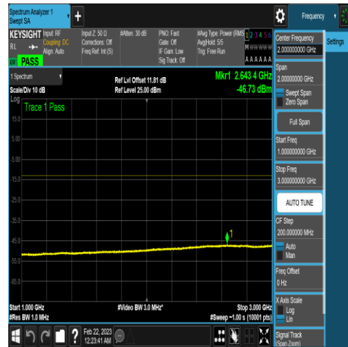
NTNV_N77-3450-3550_PC2_30_40_M_TID5_N/A _1000_3000_#1
