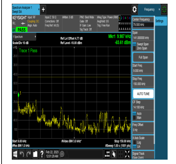
NTNV_N77-3450-3550_PC2_30_20_H_TID18_N/A_3000_12000_#1
