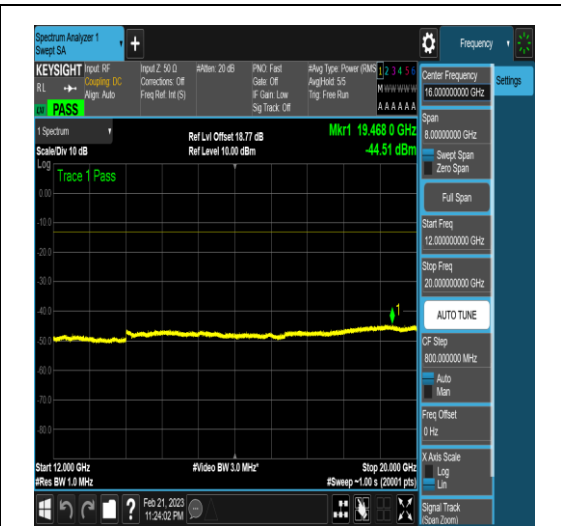
NTNV_N77-3450-3550_PC2_30_20_L_TID18_N/A_12000_20000_#1
