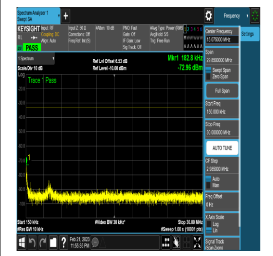
NTNV_N77-3450-3550_PC2_30_20_H_TID17_N/A_0.15_30_#1
