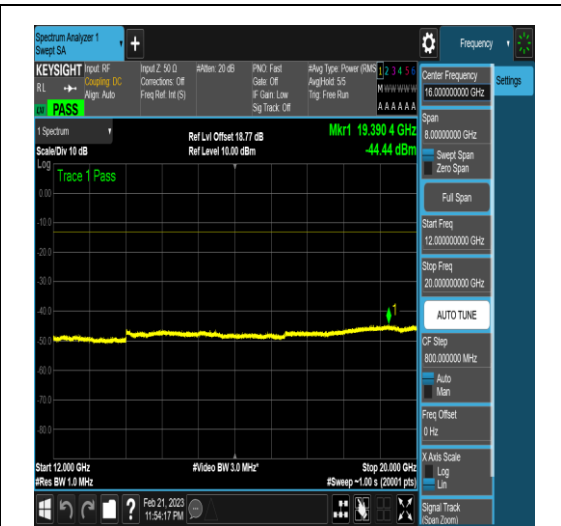
NTNV_N77-3450-3550_PC2_30_20_H_TID16_N/A_12000_20000_#1
