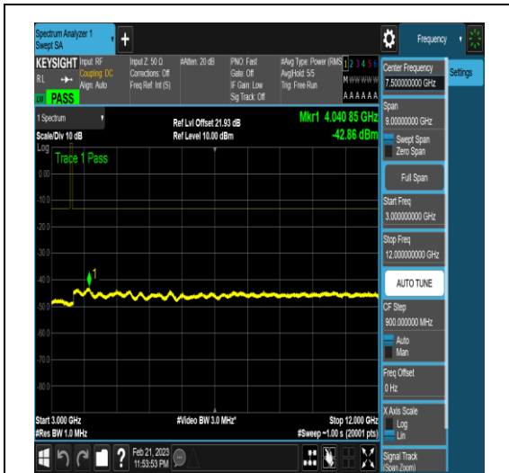
NTNV_N77-3450-3550_PC2_30_20_H_TID16_N/A_3000_12000_#1
