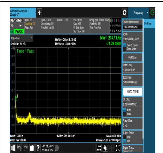
NTNV_N77-3450-3550_PC2_30_20_H_TID6_N/A _0.15_30_#1
