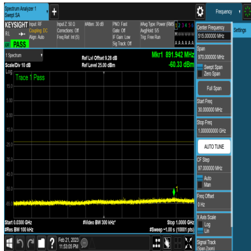
NTNV_N77-3450-3550_PC2_30_20_H_TID16_N/ A_30_1000_#1
