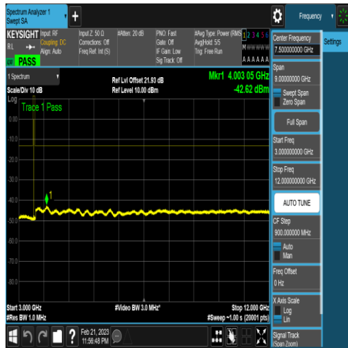
NTNV_N77-3450-3550_PC2_30_20_H_TID17_N/ A_3000_12000_#1
