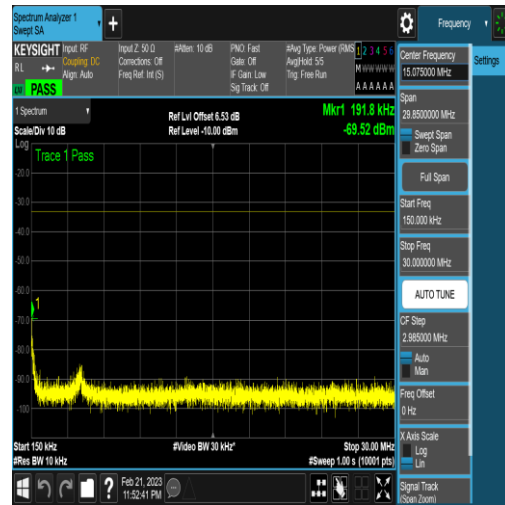
NTNV_N77-3450-3550_PC2_30_20_H_TID16_N/ A_0.15_30_#1
