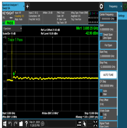
NTNV_N77-3450-3550_PC2_30_20_M_TID4_N/A _3000_12000_#1
