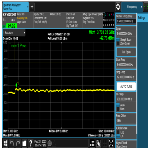
NTNV_N77-3450-3550_PC2_30_20_H_TID5_N/A _3000_12000_#1
