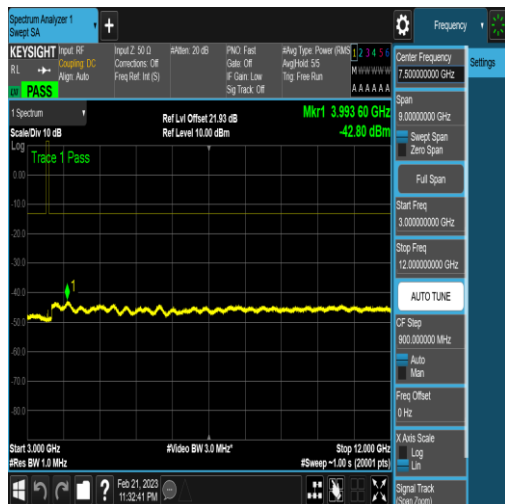
NTNV_N77-3450-3550_PC2_30_20_M_TID6_N/A _3000_12000_#1
