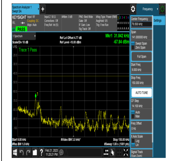
NTNV_N77-3450-3550_PC2_30_20_M_TID4_N/A_0.009_0.15_#1
