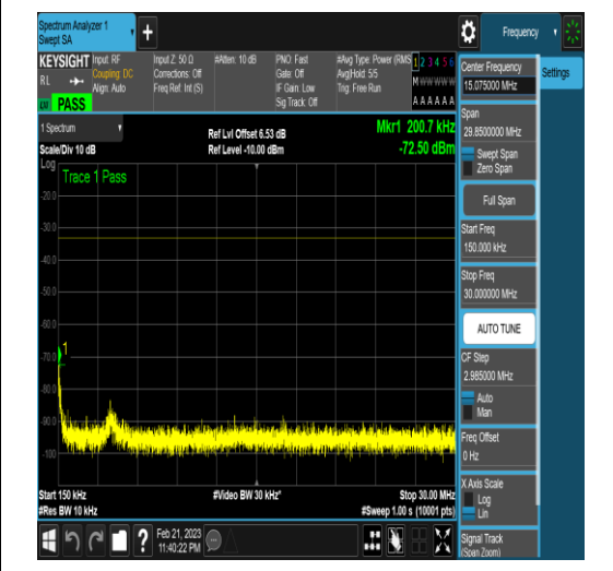
NTNV_N77-3450-3550_PC2_30_20_M_TID18_NV/ A_0.15_30_#1
