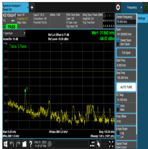
NTNV_N77-3450-3550_PC2_30_20_M_TID17_NV/ A_0.009_0.15_#1
