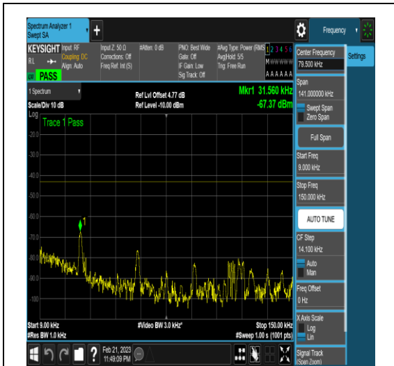
NTNV_N77-3450-3550_PC2_30_20_H_TID6_N/A _0.009_0.15_#1
