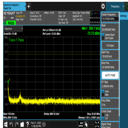
NTNV_N77-3450-3550_PC2_30_20_H_TID18_N/ A_0.15_30_#1
