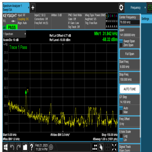
NTNV_N77-3450-3550_PC2_30_20_M_TID5_N/A _0.009_0.15_#1
