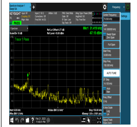
NTNV_N77-3450-3550_PC2_30_20_M_TID18_NV/ A_0.009_0.15_#1
