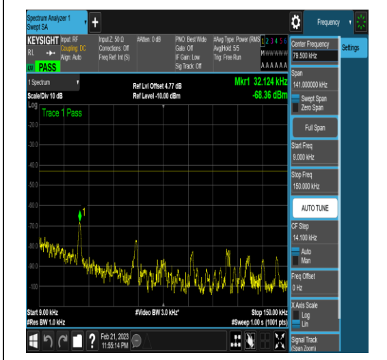
NTNV_N77-3450-3550_PC2_30_20_H_TID17_N/A_0.009_0.15_#1
