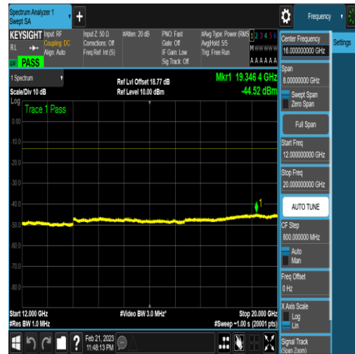
NTNV_N77-3450-3550_PC2_30_20_H_TID5_N/A _12000_20000_#1
