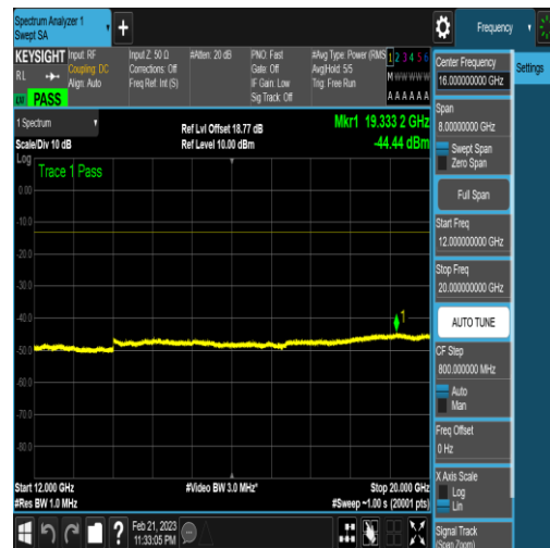
NTNV_N77-3450-3550_PC2_30_20_M_TID6_N/A _12000_20000_#1
