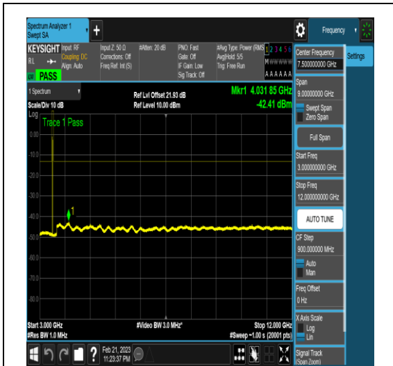
NTNV_N77-3450-3550_PC2_30_20_L_TID18_N/A_3000_12000_#1
