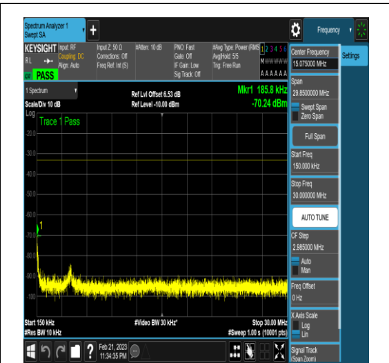
NTNV_N77-3450-3550_PC2_30_20_M_TID16_N/A_0.15_30_#1
