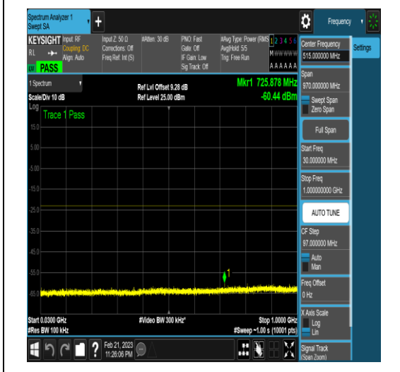
NTNV_N77-3450-3550_PC2_30_20_M_TID4_N/A_0.009_0.15_#1
