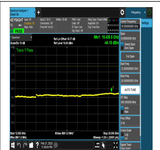
NTNV_N77-3450-3550_PC2_30_20_M_TID17_NV/ A_12000_20000_#1
