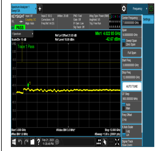
NTNV_N77-3450-3550_PC2_30_20_M_TID16_N/A_30_1000_#1
