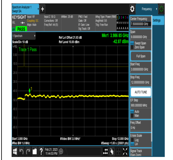
NTNV_N77-3450-3550_PC2_30_20_H_TID4_N/A _3000_12000_#1
