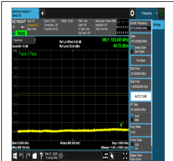
NTNV_N77-3450-3550_PC2_30_20_H_TID4_N/A _30_1000_#1
