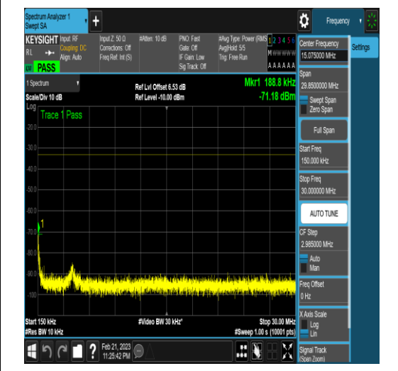
NTNV_N77-3450-3550_PC2_30_20_M_TID4_N/A_0.15_30_#1
