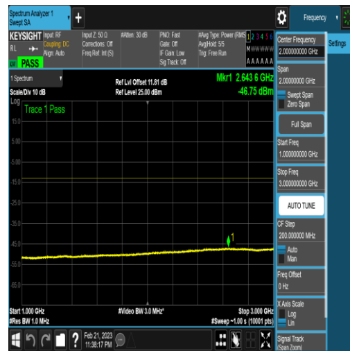
NTNV_N77-3450-3550_PC2_30_20_M_TID17_NV/ A_1000_3000_#1
