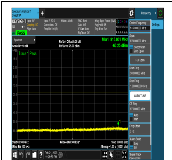
NTNV_N77-3450-3550_PC2_30_20_M_TID5_N/A _30_1000_#1
