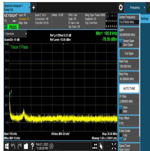
NTNV_N77-3450-3550_PC2_30_20_M_TID5_N/A _0.15_30_#1
