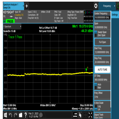
NTNV_N77-3450-3550_PC2_30_20_M_TID4_N/A _12000_20000_#1
