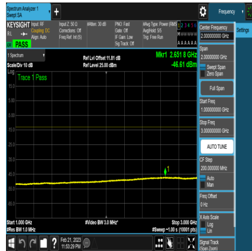
NTNV_N77-3450-3550_PC2_30_20_H_TID16_N/ A_1000_3000_#1
