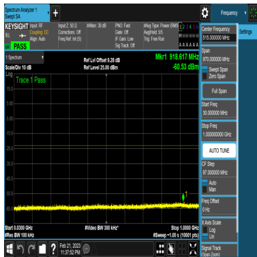
NTNV_N77-3450-3550_PC2_30_20_M_TID17_NV/ A_30_1000_#1
