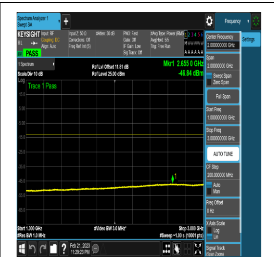
NTNV_N77-3450-3550_PC2_30_20_M_TID5_N/A _1000_3000_#1
