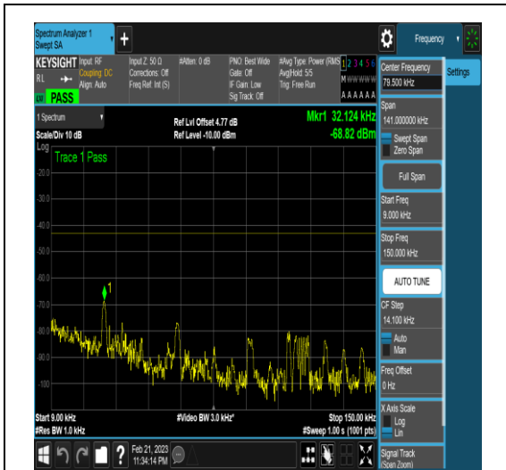
NTNV_N77-3450-3550_PC2_30_20_M_TID16_N/A_0.009_0.15_#1
