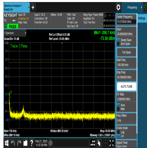
NTNV_N77-3450-3550_PC2_30_20_M_TID17_NV/ A_0.15_30_#1
