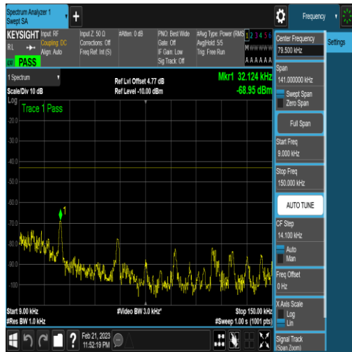
NTNV_N77-3450-3550_PC2_30_20_H_TID16_N/ A_0.009_0.15_#1
