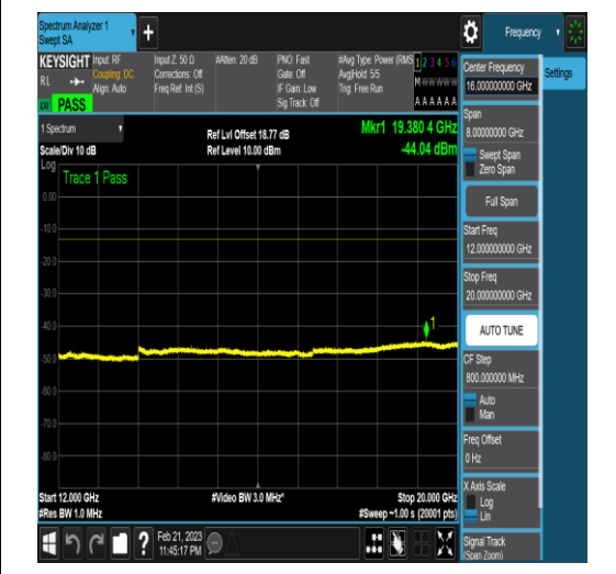
NTNV_N77-3450-3550_PC2_30_20_H_TID4_N/A _12000_20000_#1
