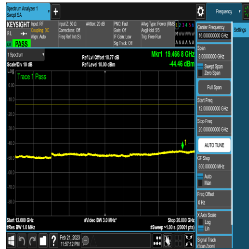
NTNV_N77-3450-3550_PC2_30_20_H_TID17_N/ A_12000_20000_#1
