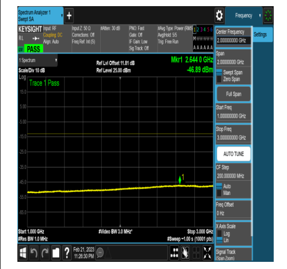
NTNV_N77-3450-3550_PC2_30_20_M_TID4_N/A_0.15_30_#1
