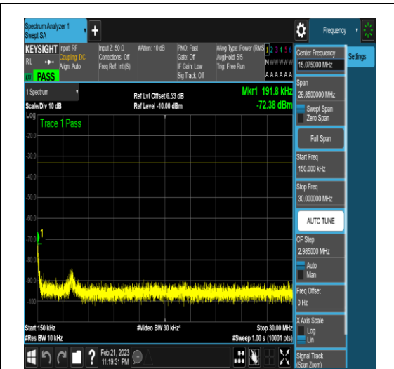
NTNV_N77-3450-3550_PC2_30_20_L_TID17_N/ A_0.15_30_#1
