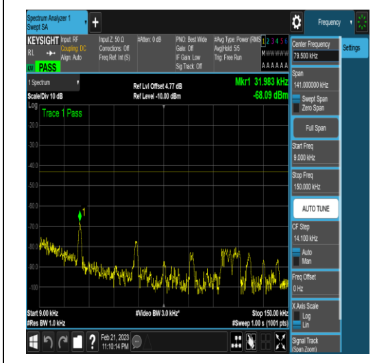
NTNV_N77-3450-3550_PC2_30_20_L_TID5_N/A _0.009_0.15_#1
