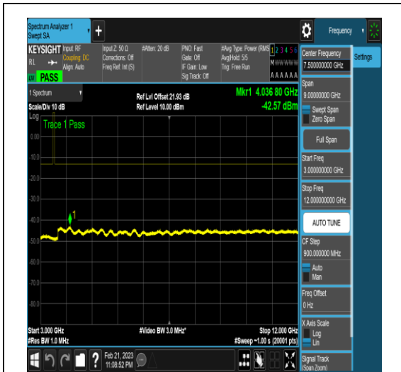
NTNV_N77-3450-3550_PC2_30_20_L_TID4_N/A _3000_12000_#1
