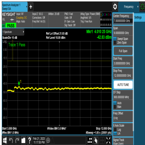
NTNV_N77-3450-3550_PC2_30_20_L_TID16_N/ A_3000_12000_#1
