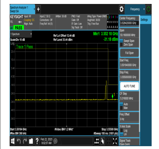
NTNV_N77-3450-3550_PC2_30_40_H_TID6_RID
