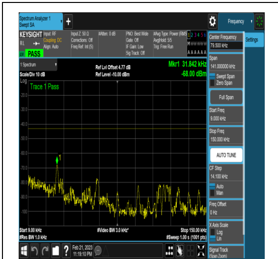
NTNV_N77-3450-3550_PC2_30_20_L_TID17_N/ A_0.009_0.15_#1
