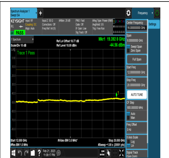
NTNV_N77-3450-3550_PC2_30_20_L_TID4_N/A _12000_20000_#1
