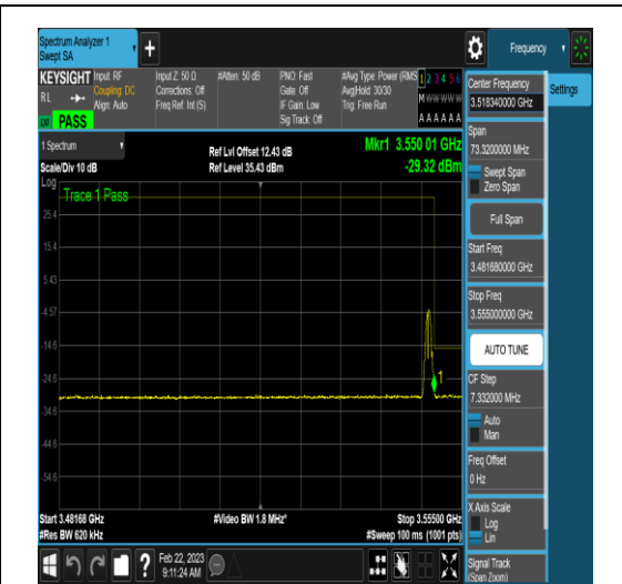
NTNV_N77-3450-3550_PC2_30_60_H_TID6_RID
