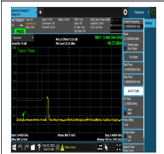
NTNV_N77-3450-3550_PC2_30_40_H_TID5_RID
