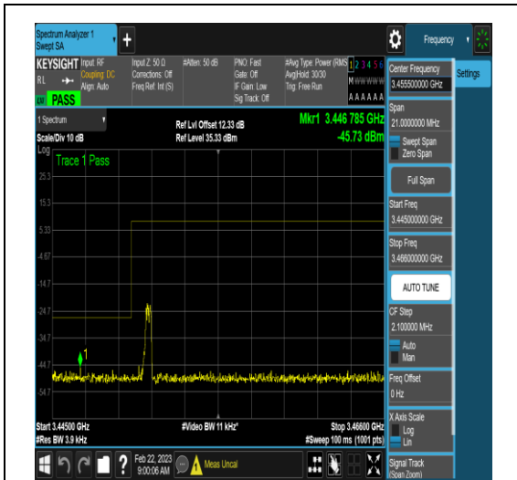
NTNV_N77-3450-3550_PC2_30_40_L_TID4_RID
