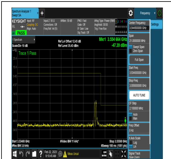
NTNV_N77-3450-3550_PC2_30_60_H_TID5_RID
