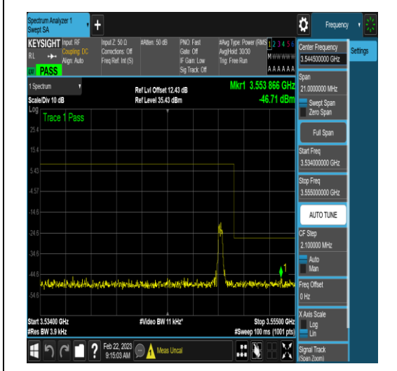
NTNV_N77-3450-3550_PC2_30_80_L_TID4_RID
