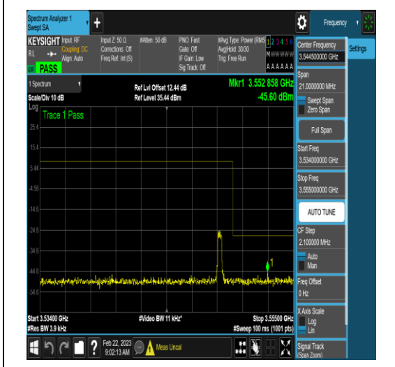
NTNV_N77-3450-3550_PC2_30_40_H_TID5_RID
