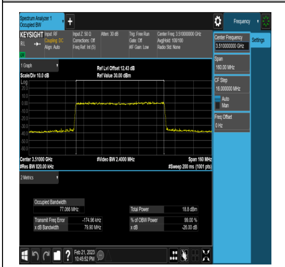
NTNV_N77-3450-3550_PC2_30_80_M_TID1_Ant
