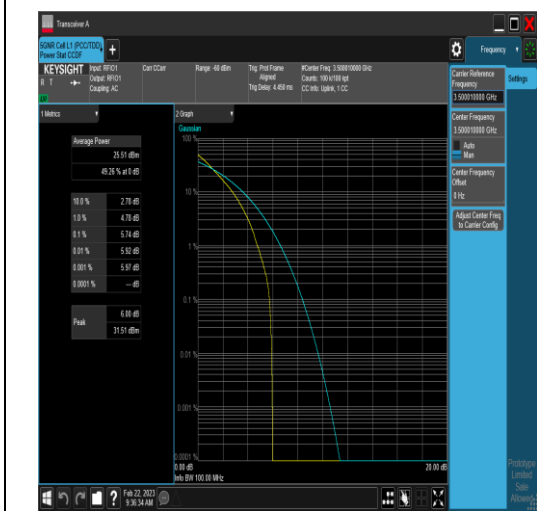
NTNV_N77-3450-3550_PC2_30_90_M_TID2_#1
