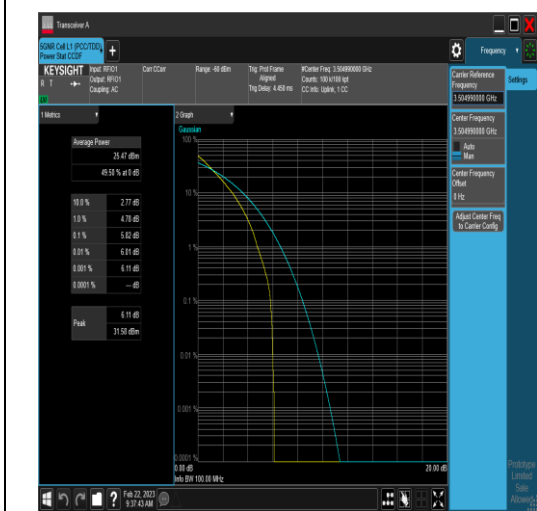
NTNV_N77-3450-3550_PC2_30_90_H_TID2_#1
