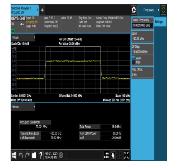
NTNV_N77-3450-3550_PC2_30_80_M_TID5_Ant
