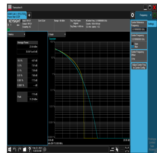
NTNV_N77-3450-3550_PC2_30_60_H_TID6_#1
