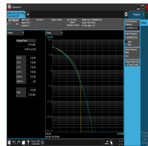
NTNV_N77-3450-3550_PC2_30_90_H_TID6_#1
