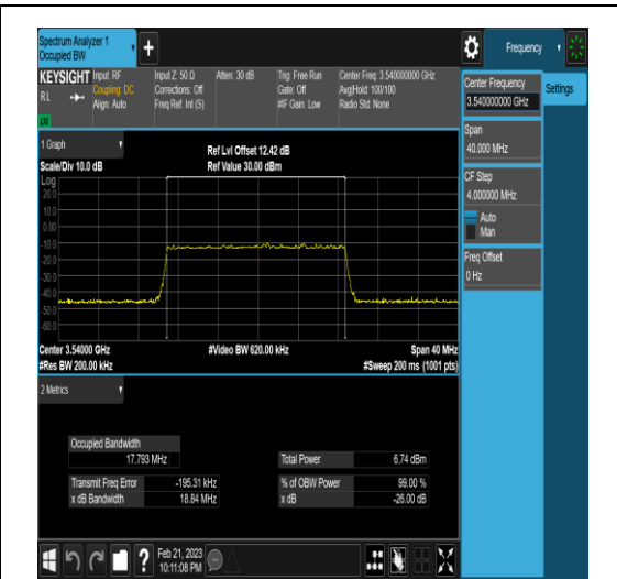
NTNV_N77-3450-3550_PC2_30_20_H_TID5_Ant
