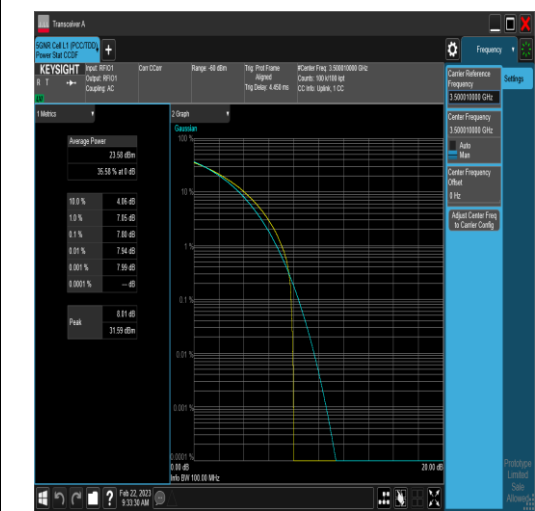
NTNV_N77-3450-3550_PC2_30_80_M_TID6_#1
