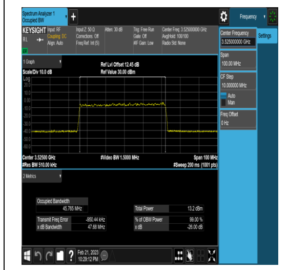
NTNV_N77-3450-3550_PC2_30_50_H_TID5_Ant
