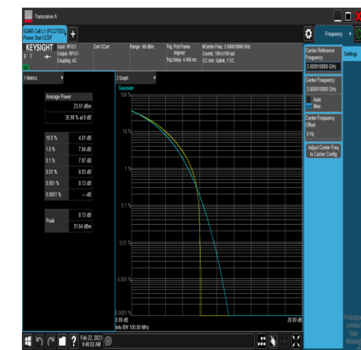
NTNV_N77-3450-3550_PC2_30_100_M_TID6_#1
