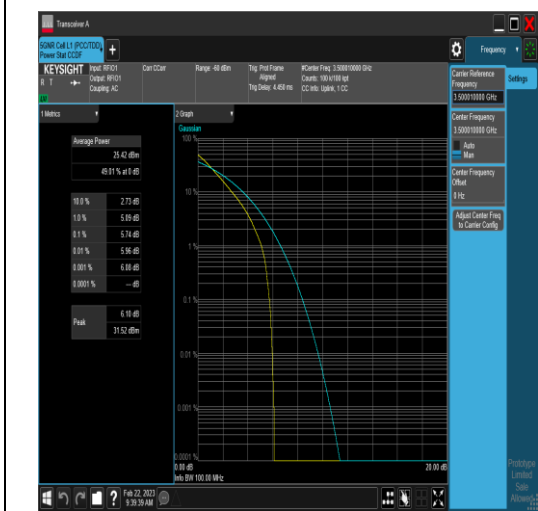
NTNV_N77-3450-3550_PC2_30_100_M_TID2_#1
