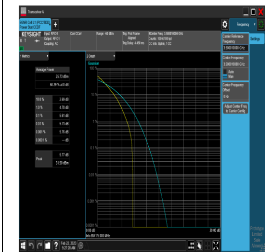
NTNV_N77-3450-3550_PC2_30_60_M_TID2_#1
