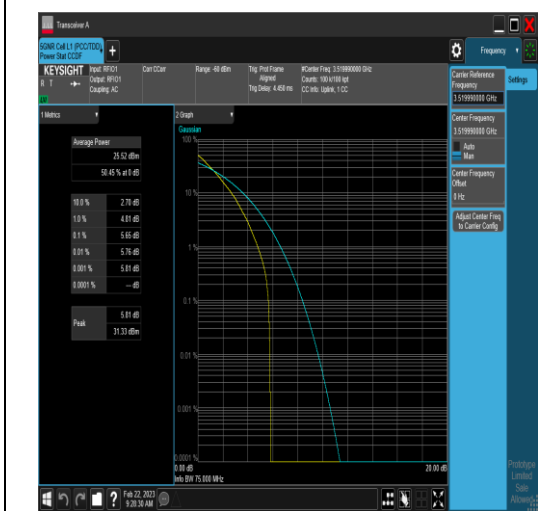
NTNV_N77-3450-3550_PC2_30_60_H_TID2_#1
