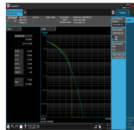
NTNV_N77-3450-3550_PC2_30_60_M_TID6_#1
