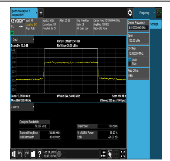
NTNV_N77-3450-3550_PC2_30_80_M_TID5_Ant
