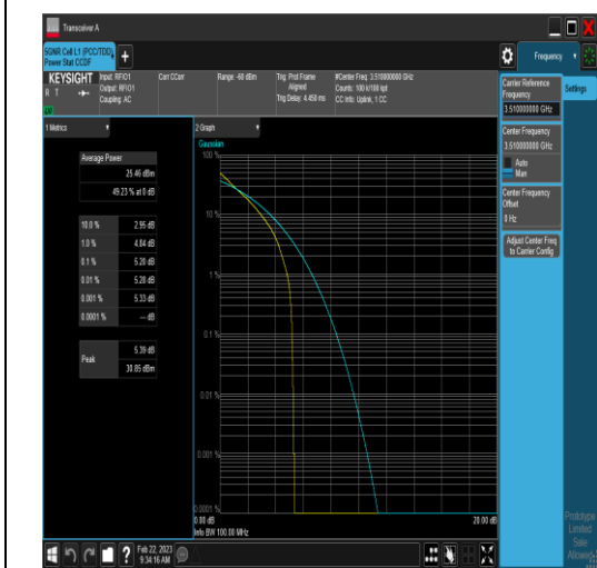
NTNV_N77-3450-3550_PC2_30_80_H_TID2_#1
