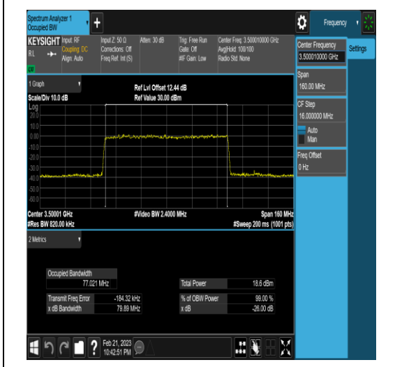
NTNV_N77-3450-3550_PC2_30_80_M_TID1_Ant
