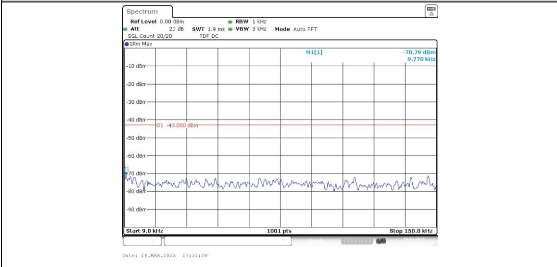
Band2-9400-4-0.009~0.15MHz
