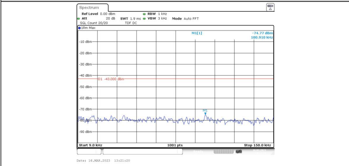
Band2-9400-4-0.009~0.15MHz
