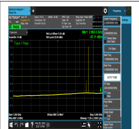
NTNV_DC_5A_n41A_PC3_30_5+100_M+H_TID5 _NS_01_1000_3000_#1
