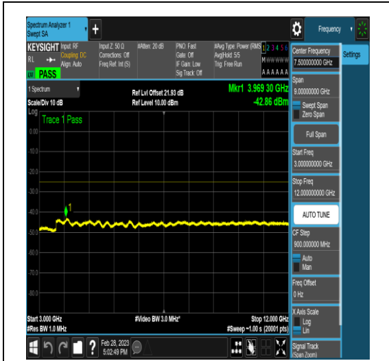
NTNV_DC_5A_n41A_PC3_30_5+100_M+M_TID1 8_NS_01_3000_12000_#1
