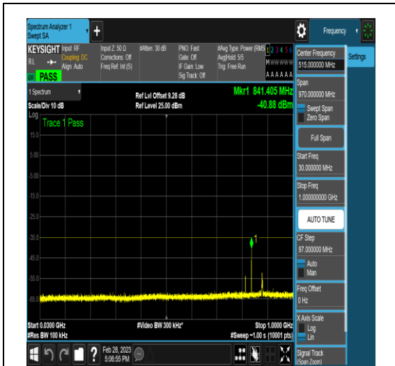
NTNV_DC_5A_n41A_PC3_30_5+100_M+H_TID5 _NS_01_30_1000_#1
