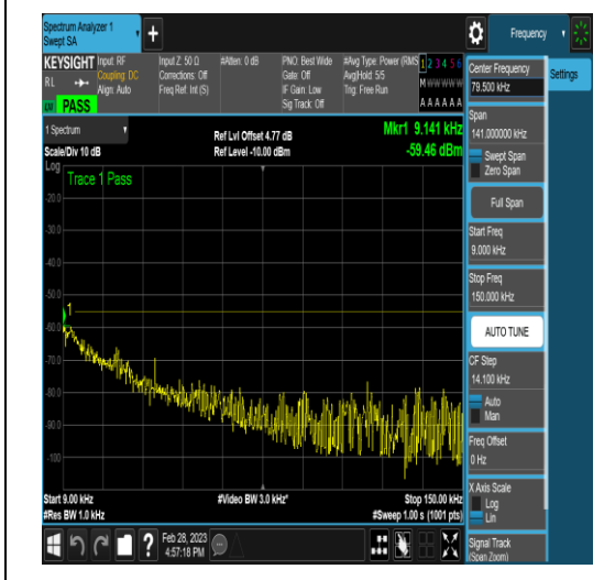
NTNV_DC_5A_n41A_PC3_30_5+100_M+M_TID6 _NS_01_3000_12000_#1
