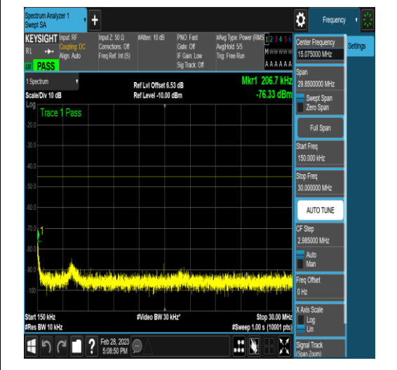
NTNV_DC_5A_n41A_PC3_30_5+100_M+H_TID5 _NS_01_12000_20000_#1
