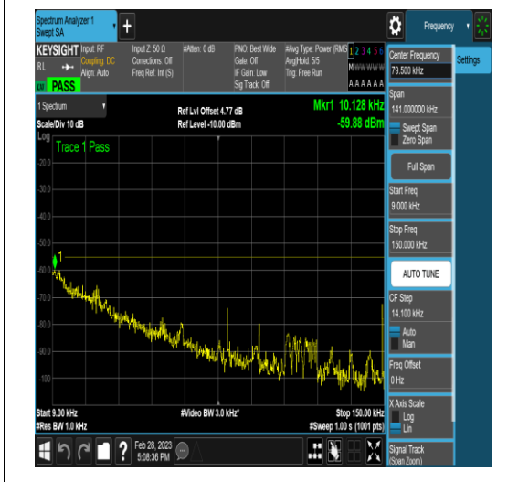
NTNV_DC_5A_n41A_PC3_30_5+100_M+H_TID5 _NS_01_3000_12000_#1
