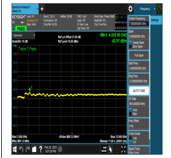
NTNV_DC_5A_n41A_PC3_30_5+100_M+H_TID5 _NS_01_3000_12000_#1
