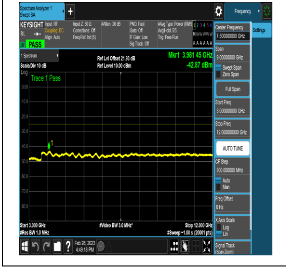
NTNV_DC_5A_n41A_PC3_30_5+100_M+L_TID1 8_NS_01_30_1000_#1
