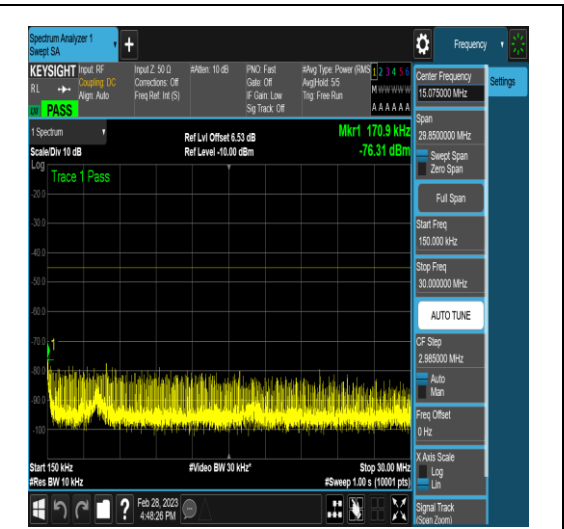
NTNV_DC_5A_n41A_PC3_30_5+100_M+L_TID1 8_NS_01_0.15_30_#1
