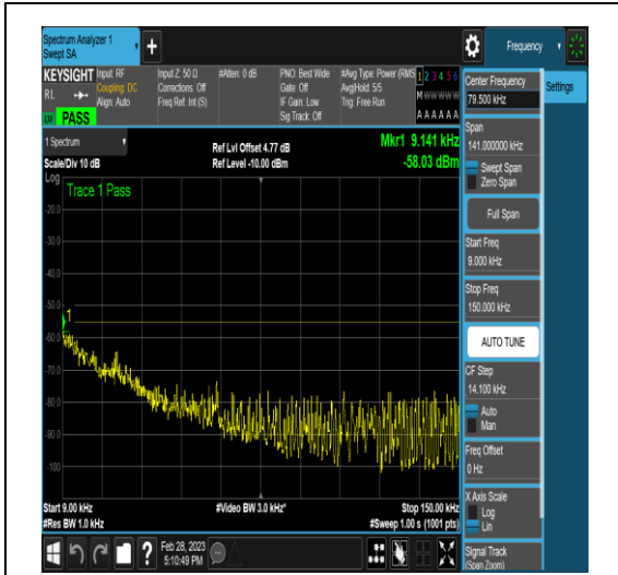
NTNV_DC_5A_n41A_PC3_30_5+100_M+H_TID1 6_NS_01_0.009_0.15_#1
