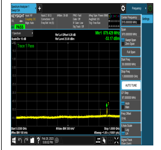
NTNV_DC_5A_n41A_PC3_30_5+100_M+M_TID1 7_NS_01_30_1000_#1
