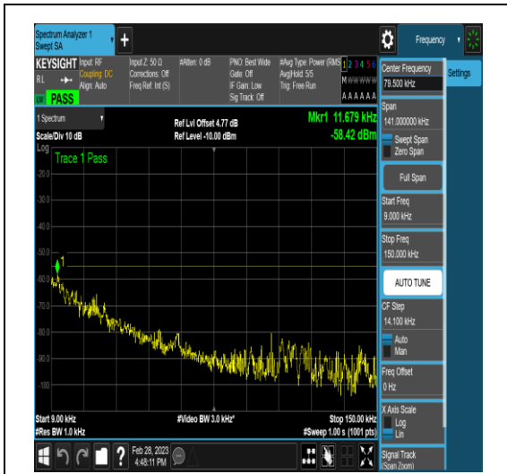
NTNV_DC_5A_n41A_PC3_30_5+100_M+L_TID1 8_NS_01_0.009_0.15_#1
