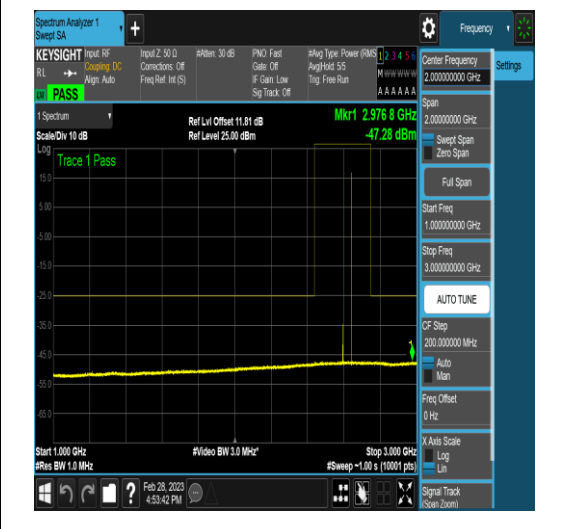
NTNV_DC_5A_n41A_PC3_30_5+100_M+M_TID5 _NS_01_0.15_30_#1
