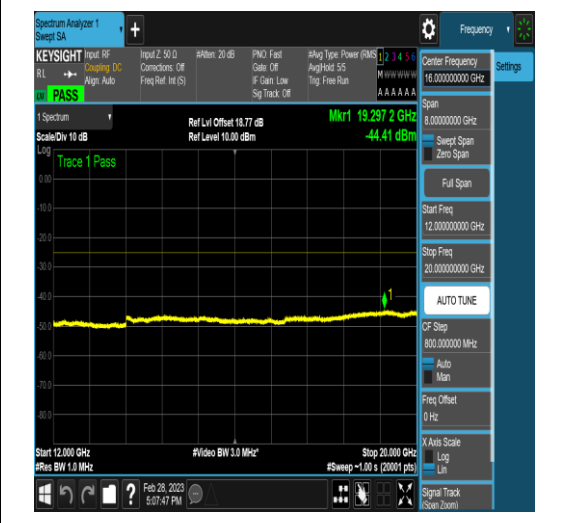
NTNV_DC_5A_n41A_PC3_30_5+100_M+H_TID5 _NS_01_12000_20000_#1
