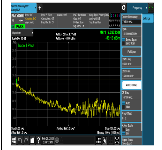
NTNV_DC_5A_n41A_PC3_30_5+100_M+H_TID4 _NS_01_0.009_0.15_#1
