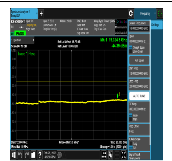
NTNV_DC_5A_n41A_PC3_30_5+100_M+M_TID4 _NS_01_12000_20000_#1
