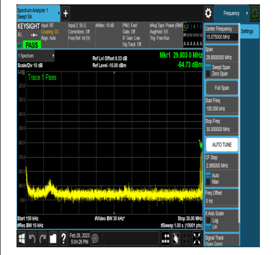
NTNV_DC_5A_n41A_PC3_30_5+100_M+H_TID4 _NS_01_0.15_30_#1
