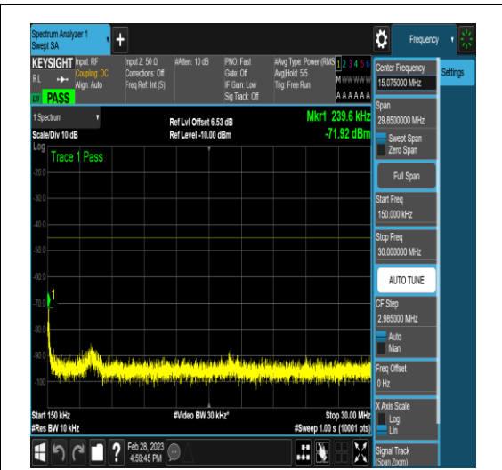
NTNV_DC_5A_n41A_PC3_30_5+100_M+M_TID1 7_NS_01_0.15_30_#1
