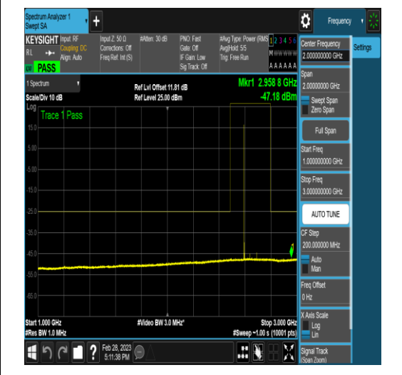
NTNV_DC_5A_n41A_PC3_30_5+100_M+H_TID1 6_NS_01_1000_3000_#1
