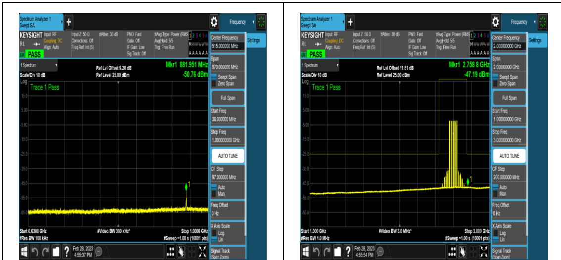
NTNV_DC_5A_n41A_PC3_30_5+100_M+M_TID6 _NS_01_30_1000_#1
