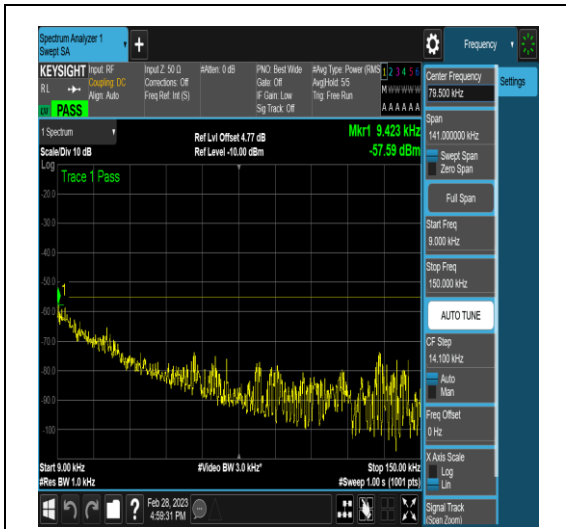
NTNV_DC_5A_n41A_PC3_30_5+100_M+M_TID1 7_NS_01_0.009_0.15_#1
