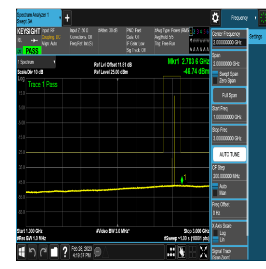
NTNV_DC_5A_n41A_PC3_30_5+60_M+M_TID17 _NS_01_0.15_30_#1
