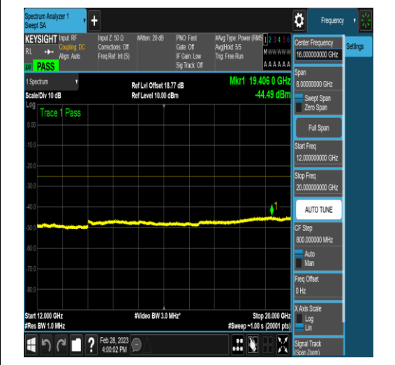
NTNV_DC_5A_n41A_PC3_30_5+60_M+L_TID5_ NS_01_12000_20000_#1
