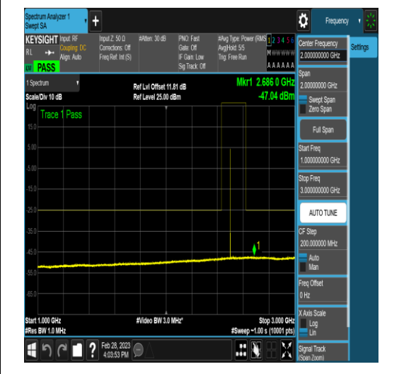
NTNV_DC_5A_n41A_PC3_30_5+60_M+L_TID16 _NS_01_1000_3000_#1
