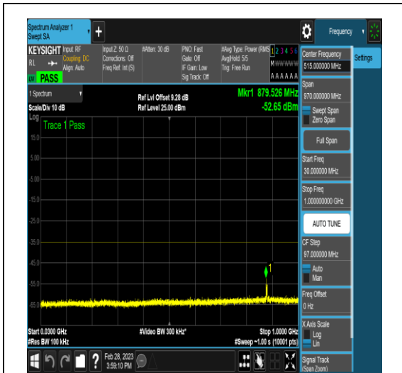
NTNV_DC_5A_n41A_PC3_30_5+60_M+L_TID5_ NS_01_30_1000_#1
