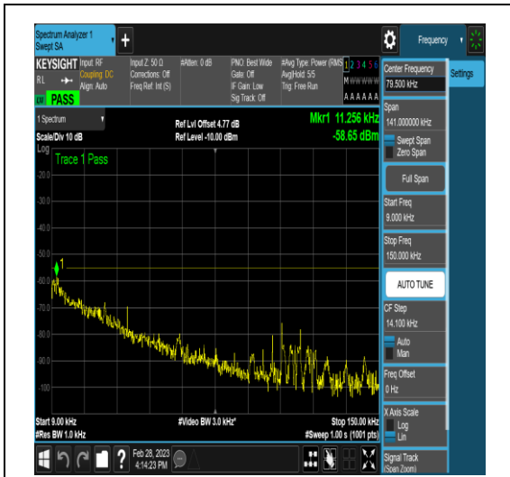
NTNV_DC_5A_n41A_PC3_30_5+60_M+M_TID6 NS_01_0.009_0.15_#1
