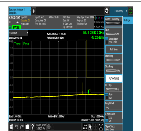
NTNV_DC_5A_n41A_PC3_30_5+60_M+L_TID5_ NS_01_1000_3000_#1
