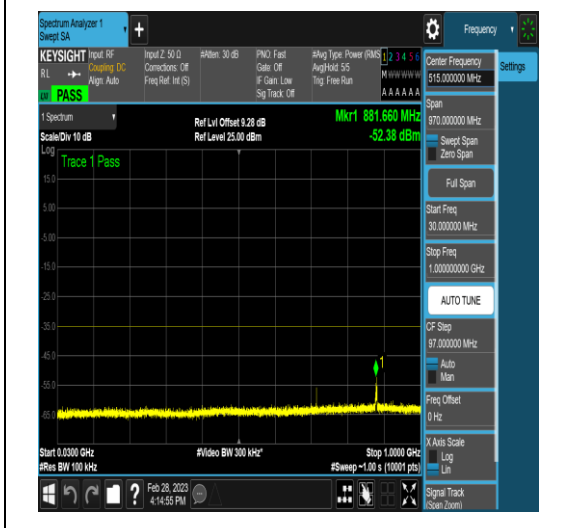
NTNV_DC_5A_n41A_PC3_30_5+60_M+M_TID6 NS_01_30_1000_#1
