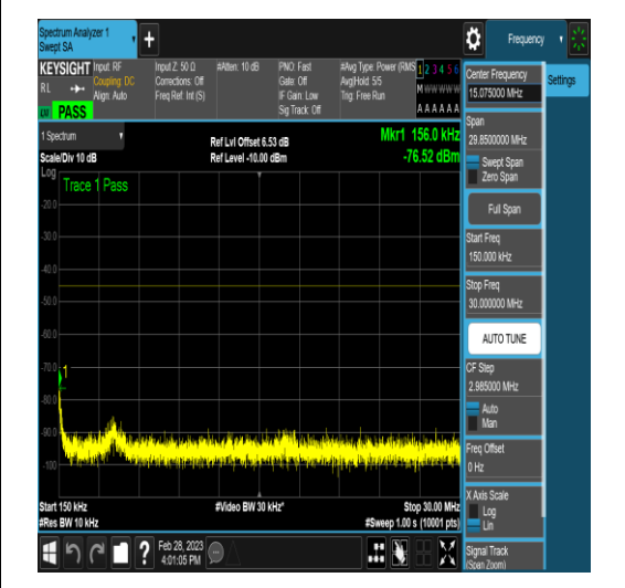
NTNV_DC_5A_n41A_PC3_30_5+60_M+L_TID5_ NS_01_12000_20000_#1
