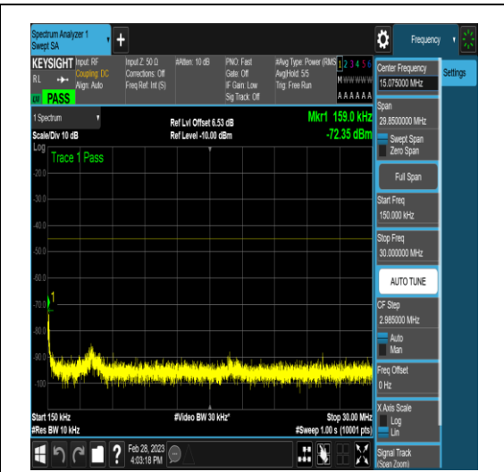
NTNV_DC_5A_n41A_PC3_30_5+60_M+L_TID16 _NS_01_0.15_30_#1
