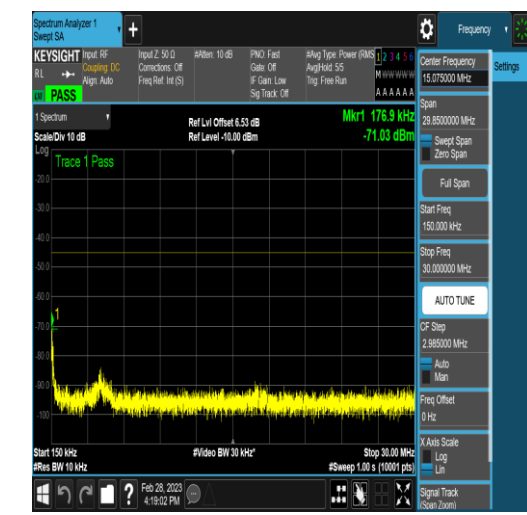
NTNV_DC_5A_n41A_PC3_30_5+60_M+M_TID17 _NS_01_0.15_30_#1
