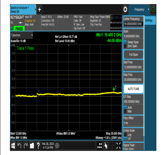
NTNV_DC_5A_n41A_PC3_30_5+60_M+M_TID4_ NS_01_12000_20000_#1
