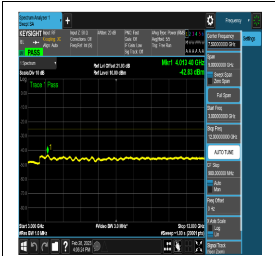
NTNV_DC_5A_n41A_PC3_30_5+60_M+L_TID17 _NS_01_3000_12000_#1
