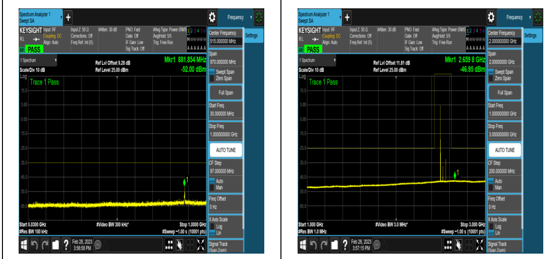
NTNV_DC_5A_n41A_PC3_30_5+60_M+L_TID4_ NS_01_0.009_0.15_#1
