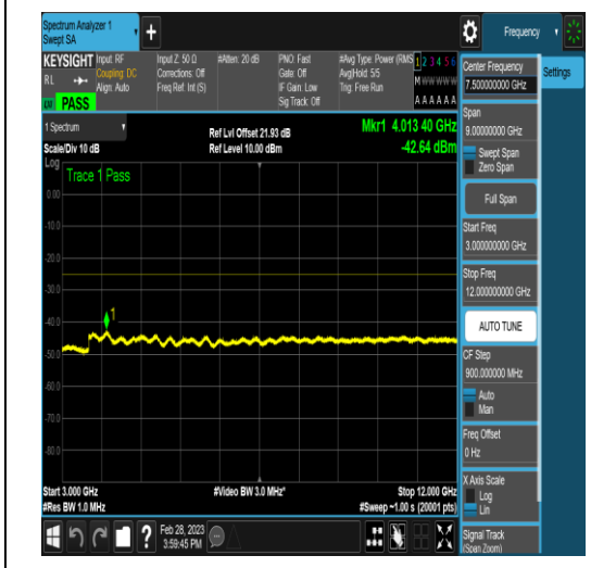
NTNV_DC_5A_n41A_PC3_30_5+60_M+L_TID5_ NS_01_3000_12000_#1
