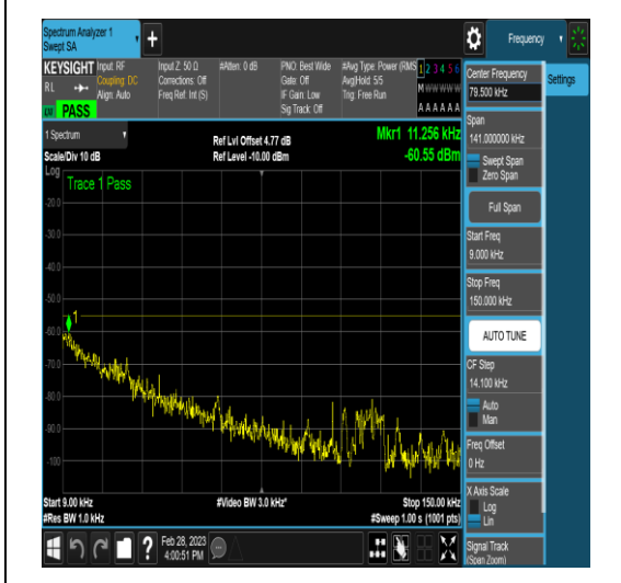
NTNV_DC_5A_n41A_PC3_30_5+60_M+L_TID5_ NS_01_3000_12000_#1
