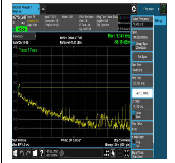
NTNV_DC_5A_n41A_PC3_30_5+60_M+L_TID18 _NS_01_0.009_0.15_#1
