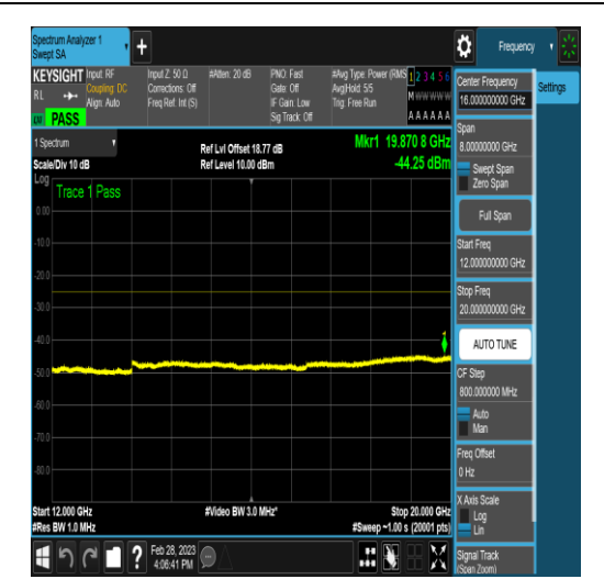
NTNV_DC_5A_n41A_PC3_30_5+60_M+L_TID17 _NS_01_12000_20000_#1
