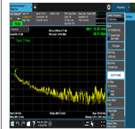
NTNV_DC_5A_n41A_PC3_30_5+60_M+M_TID17 _NS_01_0.009_0.15_#1
