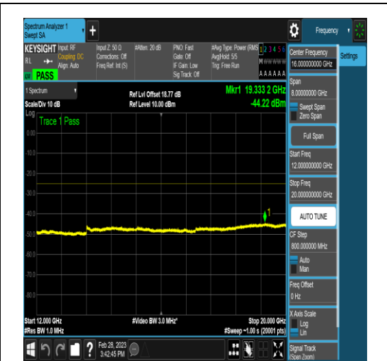
NTNV_DC_5A_n41A_PC3_30_5+40_M+H_TID4_ NS_01_12000_20000_#1
