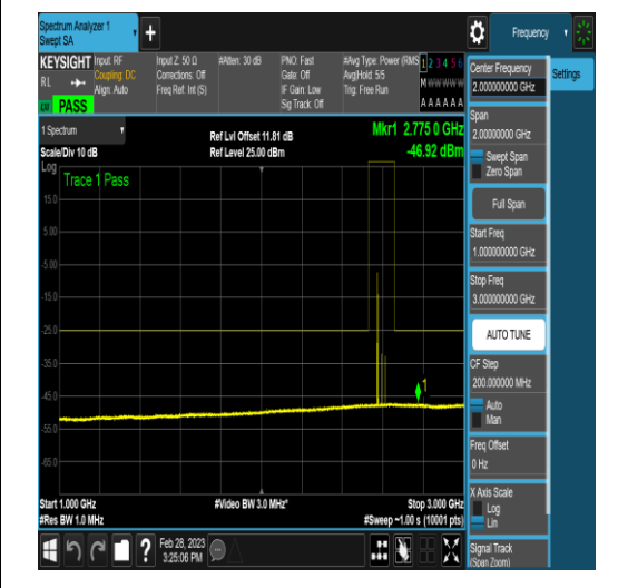
NTNV_DC_5A_n41A_PC3_30_5+40_M+M_TID4 NS_01_1000_3000_#1
