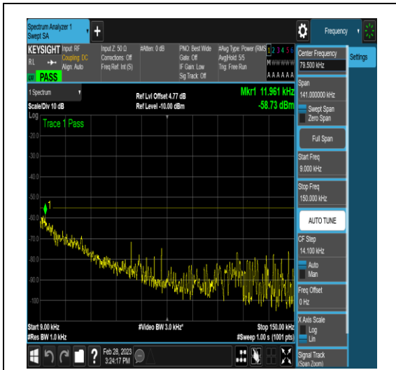
NTNV_DC_5A_n41A_PC3_30_5+40_M+M_TID4 NS_01_0.009_0.15_#1
