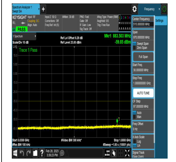
NTNV_DC_5A_n41A_PC3_30_5+40_M+M_TID18 _NS_01_30_1000_#1
