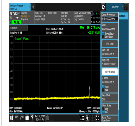
NTNV_DC_5A_n41A_PC3_30_5+40_M+M_TID4 NS_01_30_1000_#1
