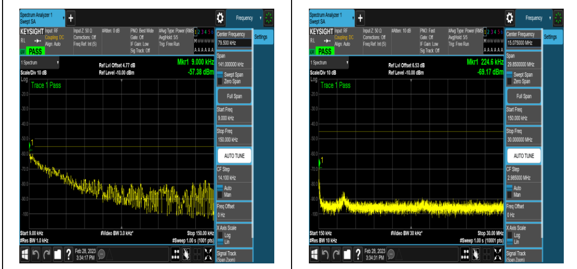
NTNV_DC_5A_n41A_PC3_30_5+40_M+M_TID16 _NS_01_3000_12000_#1
