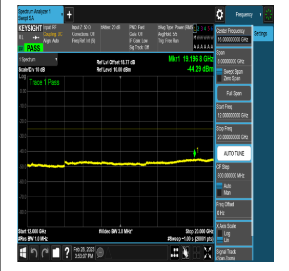
NTNV_DC_5A_n41A_PC3_30_5+40_M+H_TID17 _NS_01_1000_3000_#1
