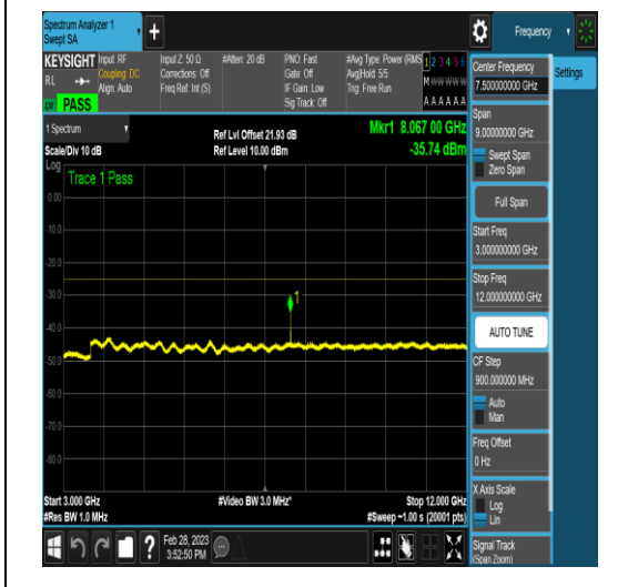
NTNV_DC_5A_n41A_PC3_30_5+40_M+H_TID17 _NS_01_30_1000_#1
