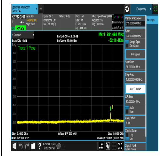
NTNV_DC_5A_n41A_PC3_30_5+40_M+M_TID6 NS_01_0.009_0.15_#1
