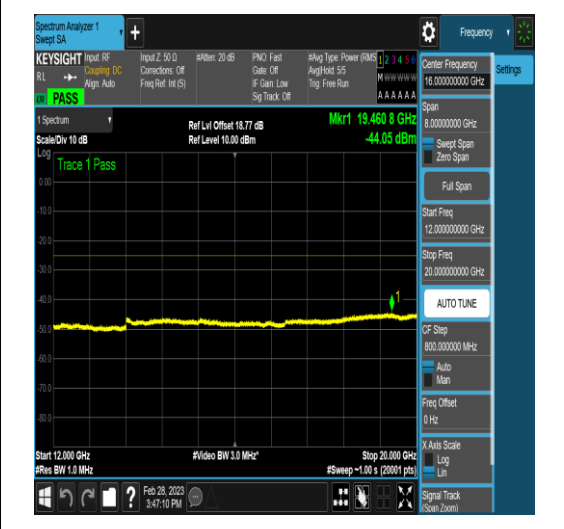
NTNV_DC_5A_n41A_PC3_30_5+40_M+H_TID6 NS_01_12000_20000_#1
