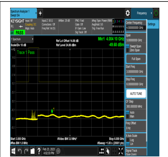
NTNV_DC_2A_n78A-3450-3550_PC3_30_5+90_ M+L_TID16_N/A_3000_6000_#1
