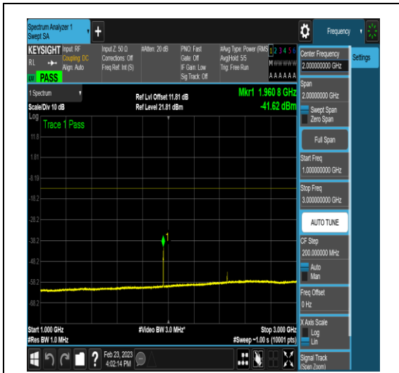
NTNV_DC_2A_n78A-3450-3550_PC3_30_5+90_ M+L_TID16_N/A_1000_3000_#1
