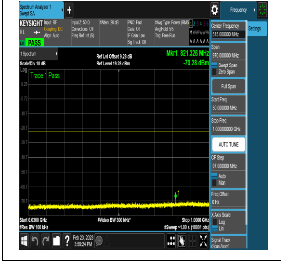
NTNV_DC_2A_n78A-3450-3550_PC3_30_5+90_ M+L_TID6_N/A_30_1000_#1
