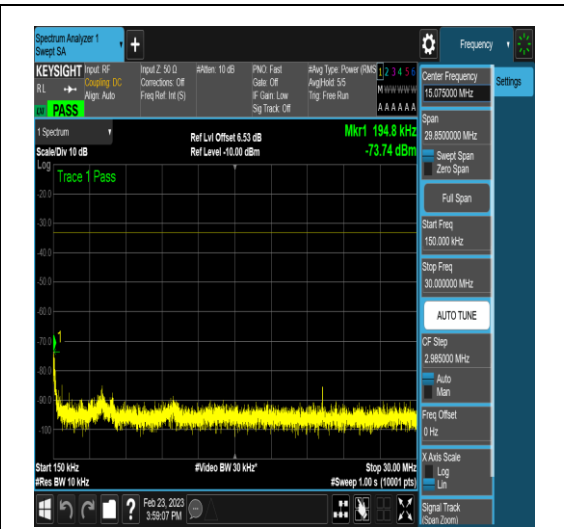
NTNV_DC_2A_n78A-3450-3550_PC3_30_5+90_ M+L_TID6_N/A_0.15_30_#1
