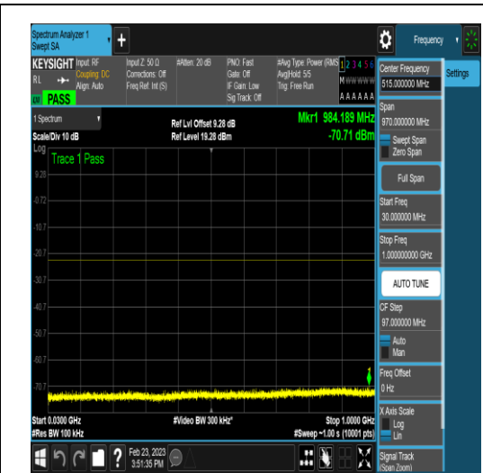
NTNV_DC_2A_n78A-3450-3550_PC3_30_5+80_ M+H_TID18_N/A_30_1000_#1
