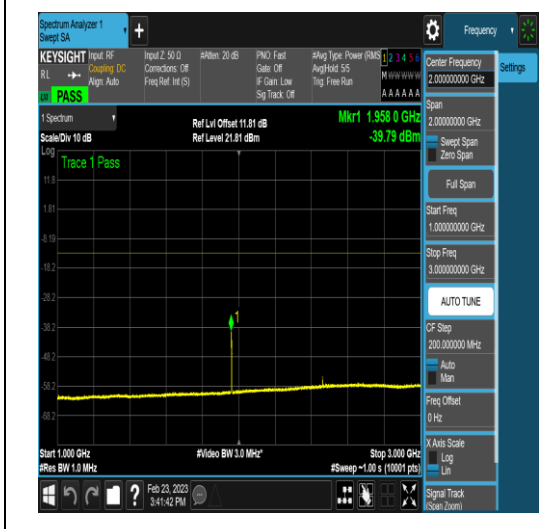
NTNV_DC_2A_n78A-3450-3550_PC3_30_5+80_ M+H_TID5_N/A_0.15_30_#1
