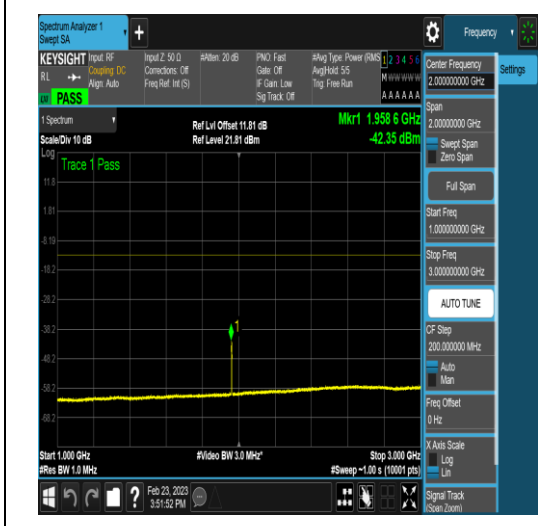
NTNV_DC_2A_n78A-3450-3550_PC3_30_5+80_ M+H_TID18_N/A_1000_3000_#1
