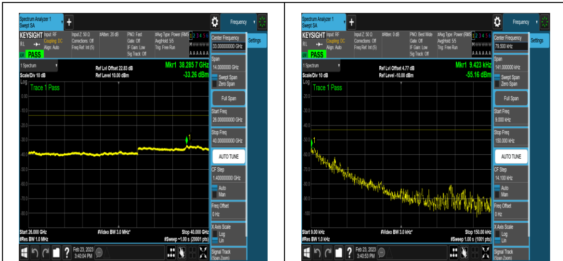
NTNV_DC_2A_n78A-3450-3550_PC3_30_5+80_ M+H_TID4_N/A_26000_40000_#1
