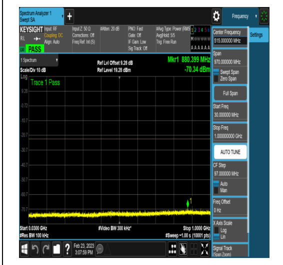
NTNV_DC_2A_n78A-3450-3550_PC3_30_5+80_ M+L_TID4_N/A_30_1000_#1
