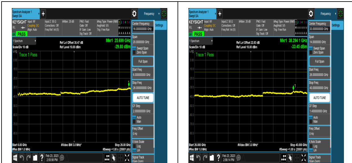
NTNV_DC_2A_n78A-3450-3550_PC3_30_5+60_ M+H_TID5_N/A_6000_26000_#1
