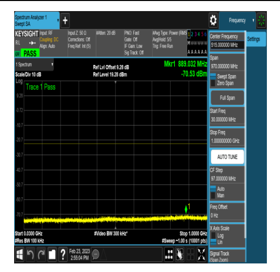
NTNV_DC_2A_n78A-3450-3550_PC3_30_5+60_ M+H_TID5_N/A_30_1000_#1
