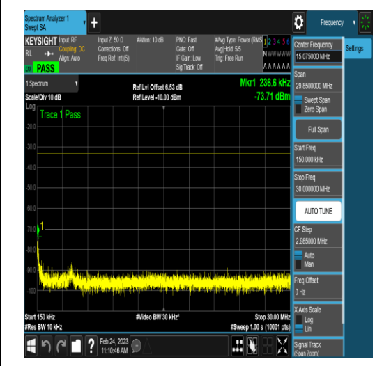
NTNV_DC_2A_n78A-3450-3550_PC3_30_5+60_ M+H_TID6_N/A_0.15_30_#1
