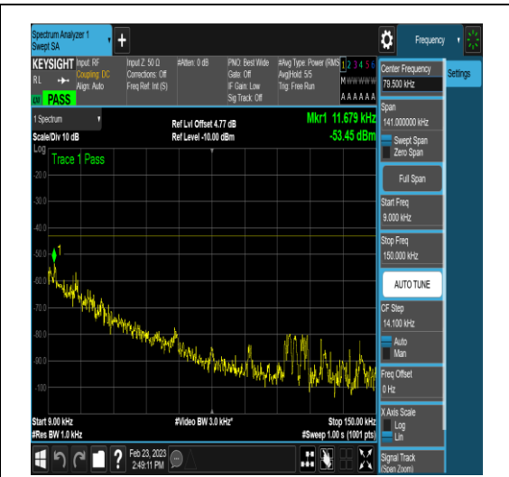
NTNV_DC_2A_n78A-3450-3550_PC3_30_5+60_ M+M_TID18_N/A_0.009_0.15_#1
