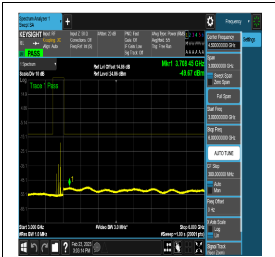
NTNV_DC_2A_n78A-3450-3550_PC3_30_5+60_ M+H_TID17_N/A_3000_6000_#1
