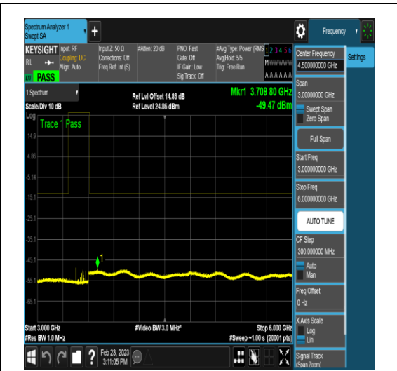
NTNV_DC_2A_n78A-3450-3550_PC3_30_5+80_ M+L_TID5_N/A_3000_6000_#1
