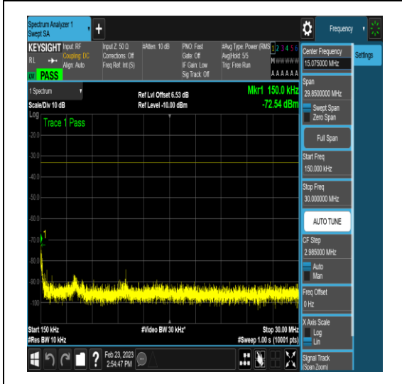
NTNV_DC_2A_n78A-3450-3550_PC3_30_5+60_ M+H_TID5_N/A_0.15_30_#1
