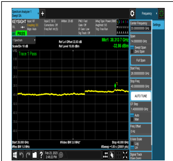
NTNV_DC_2A_n78A-3450-3550_PC3_30_5+60_ M+M_TID17_N/A_26000_40000_#1
