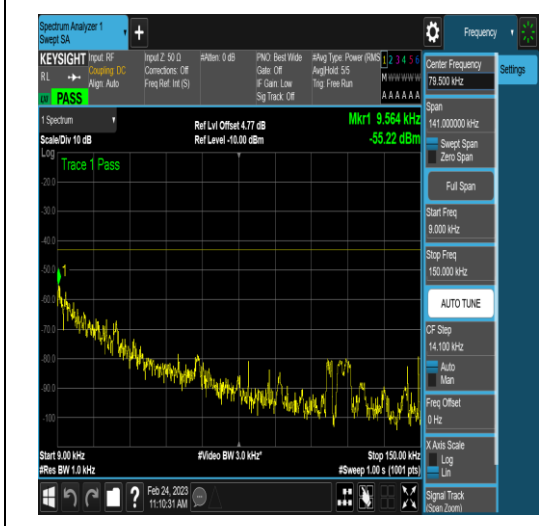
NTNV_DC_2A_n78A-3450-3550_PC3_30_5+60_ M+H_TID6_N/A_0.009_0.15_#1
