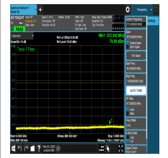
NTNV_DC_2A_n78A-3450-3550_PC3_30_5+60_ M+M_TID18_N/A_30_1000_#1
