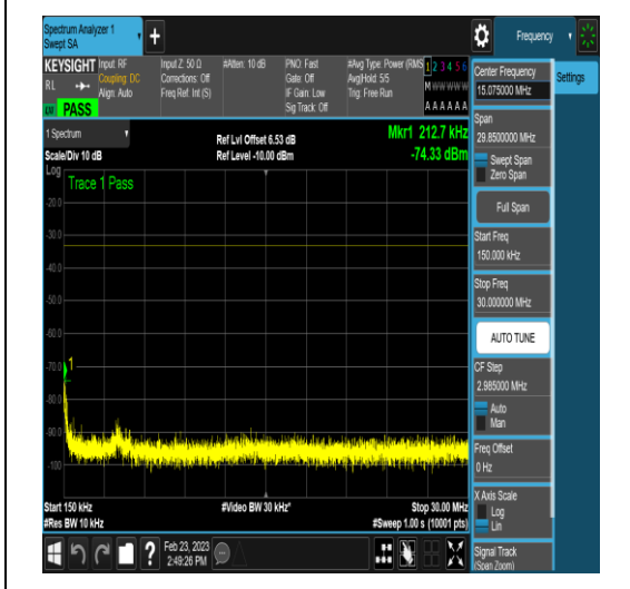
NTNV_DC_2A_n78A-3450-3550_PC3_30_5+60_ M+M_TID18_N/A_0.15_30_#1
