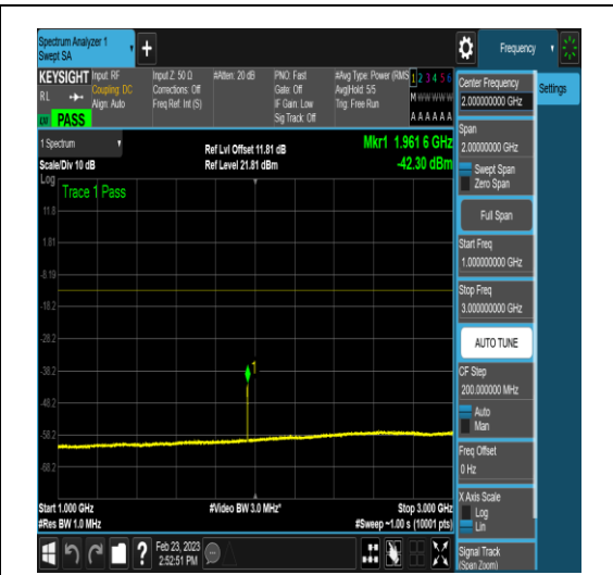
NTNV_DC_2A_n78A-3450-3550_PC3_30_5+60_ M+H_TID4_N/A_1000_3000_#1
