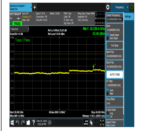
NTNV_DC_2A_n78A-3450-3550_PC3_30_5+60_ M+H_TID17_N/A_26000_40000_#1
