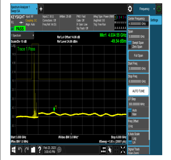
NTNV_DC_2A_n78A-3450-3550_PC3_30_5+60_ M+H_TID16_N/A_3000_6000_#1
