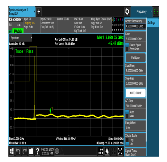
NTNV_DC_2A_n78A-3450-3550_PC3_30_5+60_ M+H_TID5_N/A_3000_6000_#1
