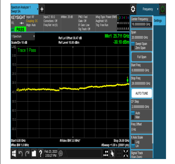
NTNV_DC_2A_n78A-3450-3550_PC3_30_5+60_ M+H_TID4_N/A_6000_26000_#1
