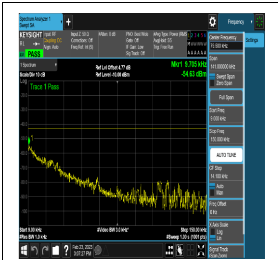
NTNV_DC_2A_n78A-3450-3550_PC3_30_5+80_ M+L_TID4_N/A_0.009_0.15_#1
