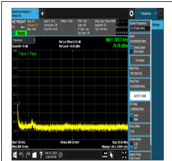
NTNV_DC_2A_n78A-3450-3550_PC3_30_5+60_ M+H_TID16_N/A_0.15_30_#1
