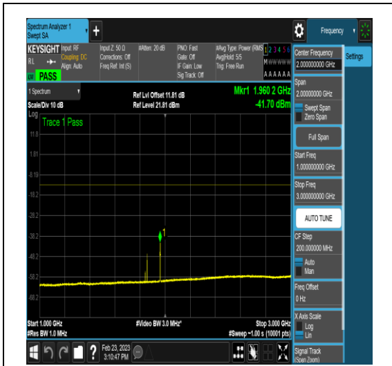
NTNV_DC_2A_n78A-3450-3550_PC3_30_5+80_ M+L_TID5_N/A_1000_3000_#1
