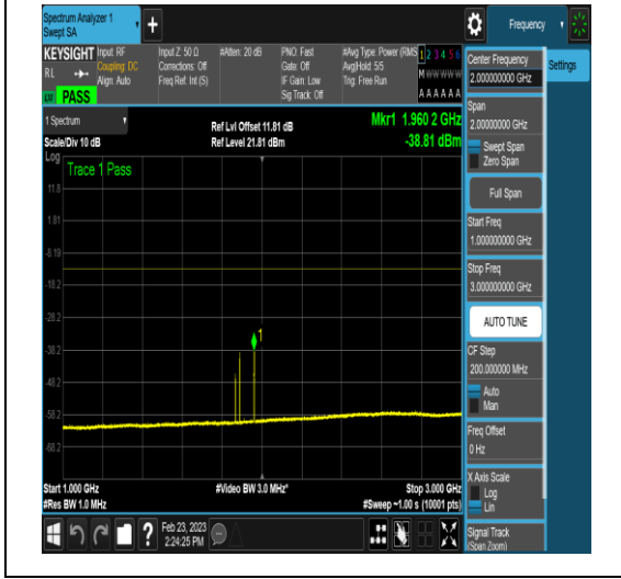
NTNV_DC_2A_n78A-3450-3550_PC3_30_5+60_ M+L_TID5_N/A_0.15_30_#1
