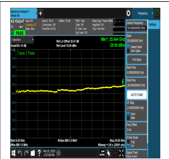
NTNV_DC_2A_n78A-3450-3550_PC3_30_5+60_ M+M_TID4_N/A_6000_26000_#1
