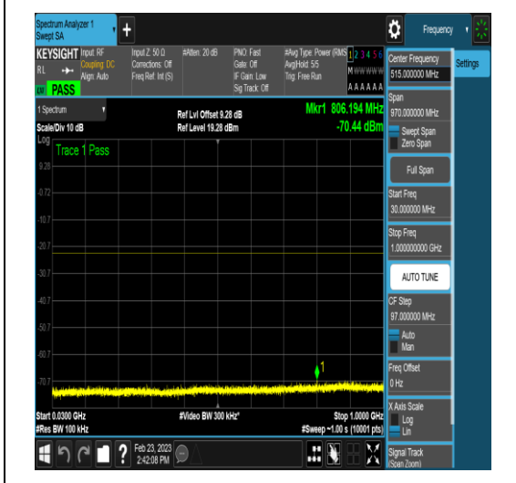
NTNV_DC_2A_n78A-3450-3550_PC3_30_5+60_ M+M_TID6_N/A_30_1000_#1
