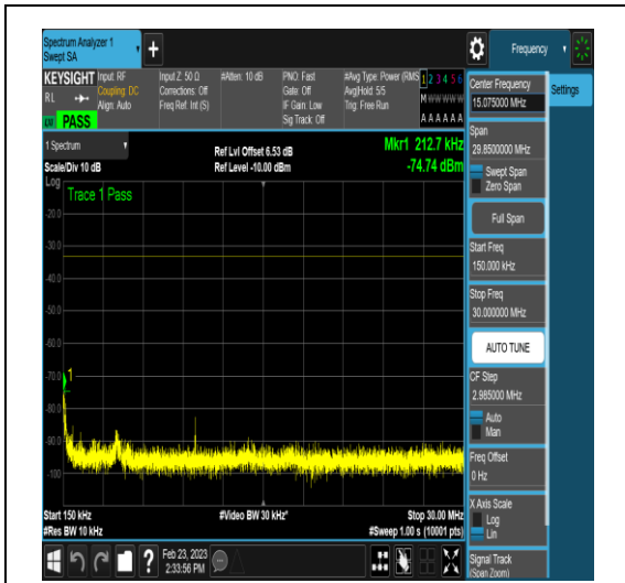
NTNV_DC_2A_n78A-3450-3550_PC3_30_5+60_ M+L_TID18_N/A_0.15_30_#1
