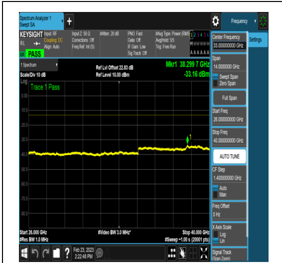
NTNV_DC_2A_n78A-3450-3550_PC3_30_5+60_ M+L_TID4_N/A_26000_40000_#1
