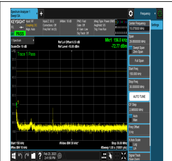
NTNV_DC_2A_n78A-3450-3550_PC3_30_5+60_ M+M_TID6_N/A_0.15_30_#1
