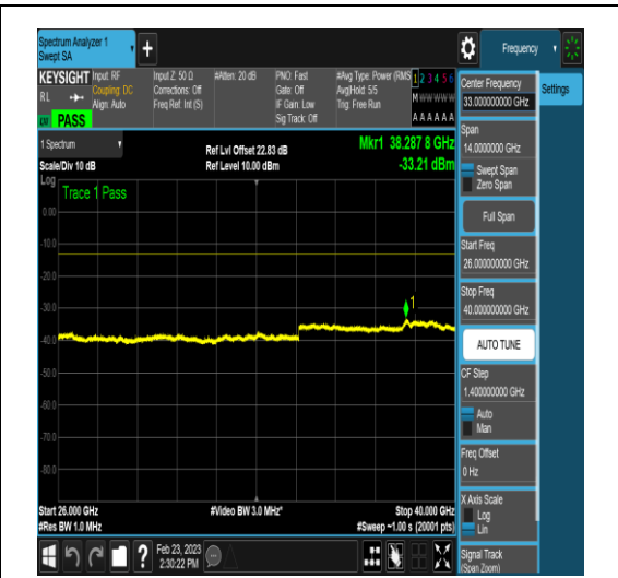
NTNV_DC_2A_n78A-3450-3550_PC3_30_5+60_ M+L_TID16_N/A_26000_40000_#1
