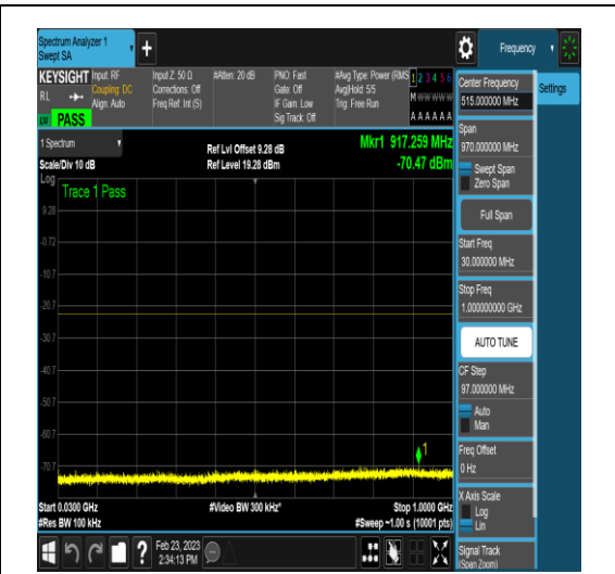
NTNV_DC_2A_n78A-3450-3550_PC3_30_5+60_ M+L_TID18_N/A_30_1000_#1
