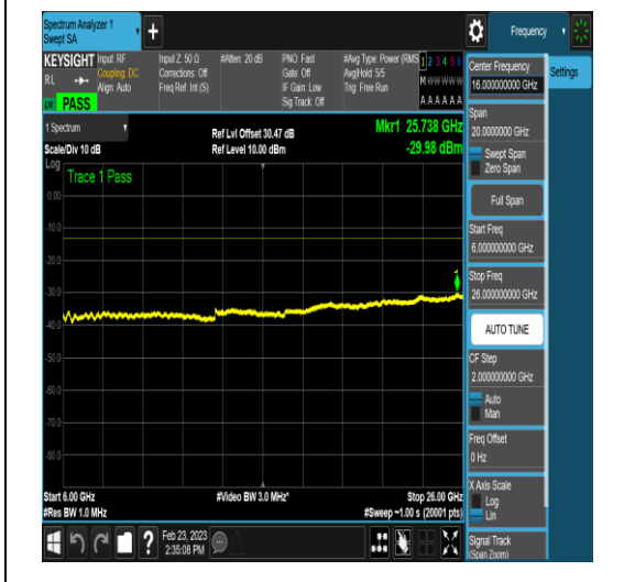
NTNV_DC_2A_n78A-3450-3550_PC3_30_5+60_ M+L_TID18_N/A_1000_3000_#1
