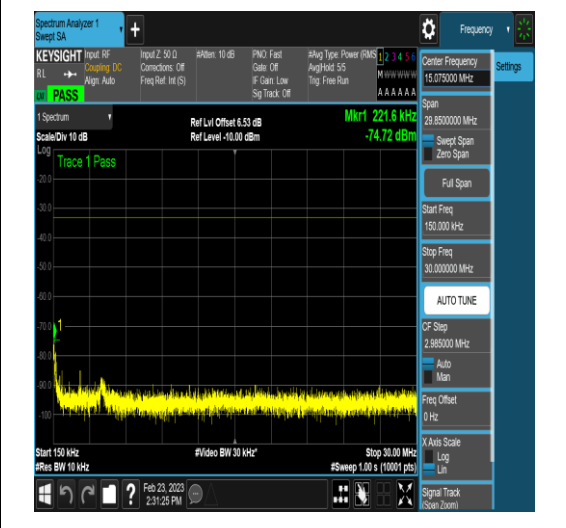
NTNV_DC_2A_n78A-3450-3550_PC3_30_5+60_ M+L_TID17_N/A_0.15_30_#1
