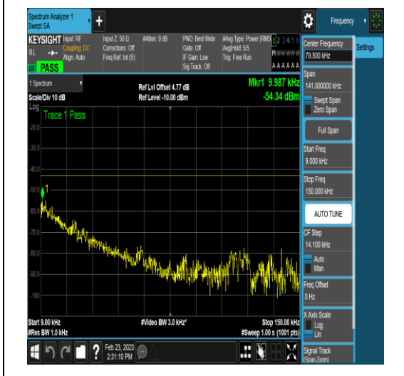
NTNV_DC_2A_n78A-3450-3550_PC3_30_5+60_ M+L_TID17_N/A_0.009_0.15_#1
