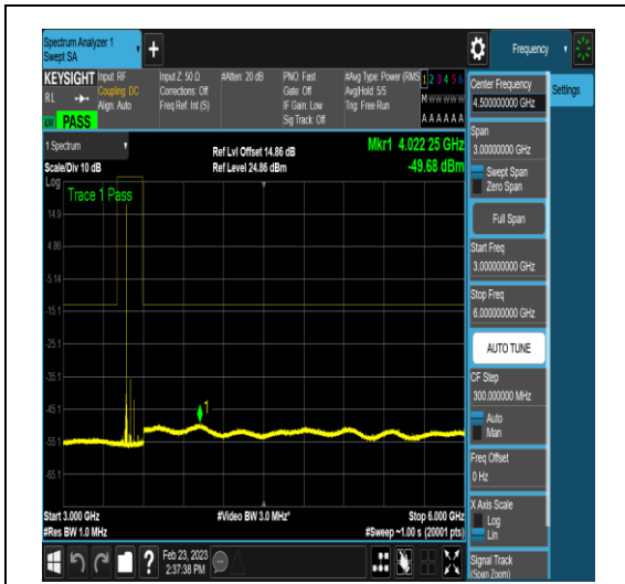
NTNV_DC_2A_n78A-3450-3550_PC3_30_5+60_ M+M_TID4_N/A_3000_6000_#1
