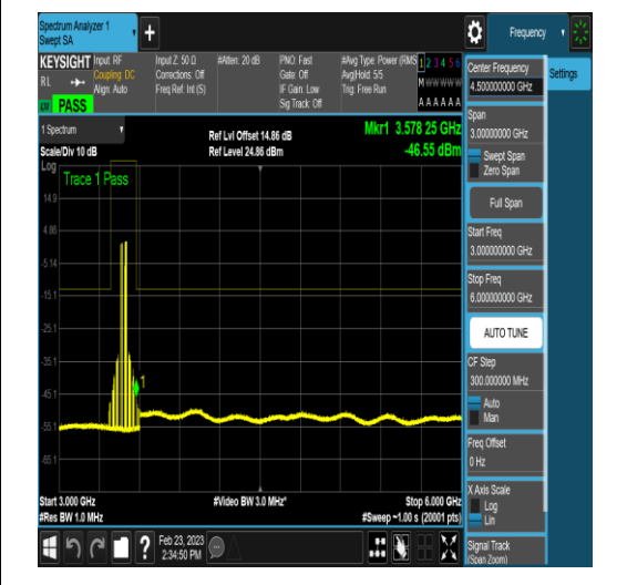
NTNV_DC_2A_n78A-3450-3550_PC3_30_5+60_ M+L_TID18_N/A_3000_6000_#1
