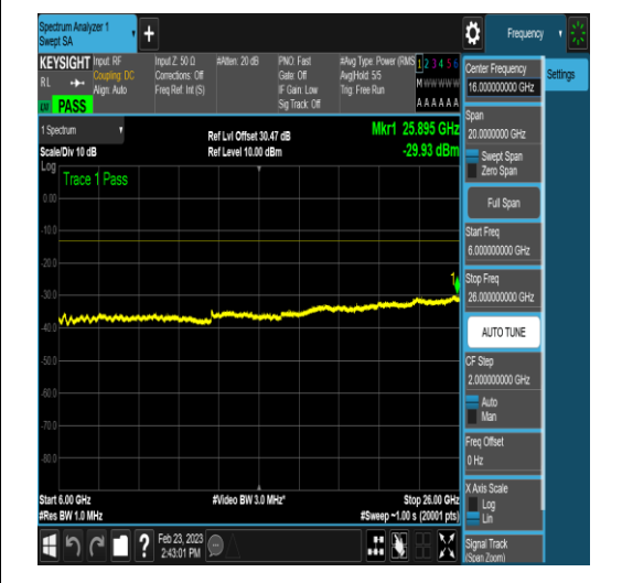
NTNV_DC_2A_n78A-3450-3550_PC3_30_5+60_ M+M_TID6_N/A_1000_3000_#1
