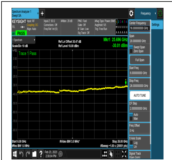
NTNV_DC_2A_n78A-3450-3550_PC3_30_5+60_ M+L_TID16_N/A_6000_26000_#1
