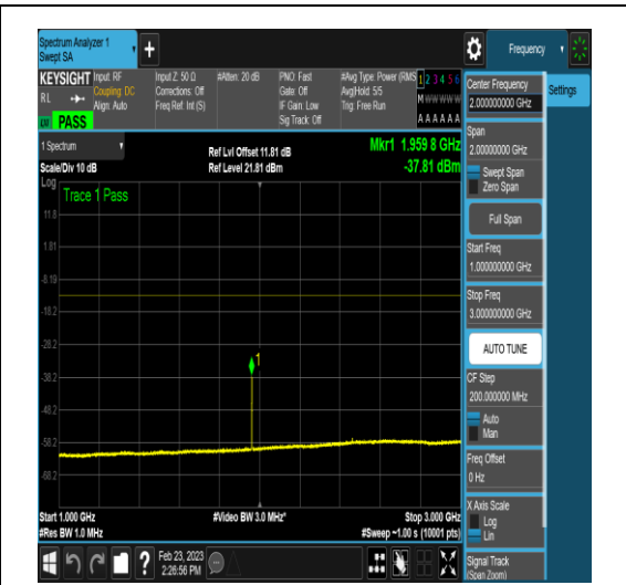
NTNV_DC_2A_n78A-3450-3550_PC3_30_5+60_ M+L_TID6_N/A_1000_3000_#1
