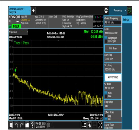
NTNV_DC_2A_n78A-3450-3550_PC3_30_5+60_ M+L_TID5_N/A_0.009_0.15_#1
