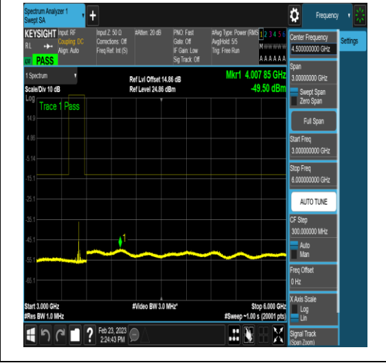
NTNV_DC_2A_n78A-3450-3550_PC3_30_5+60_ M+L_TID5_N/A_30_1000_#1
