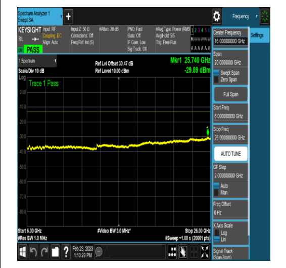
NTNV_DC_2A_n78A-3450-3550_PC3_30_5+40_ M+M_TID6_N/A_6000_26000_#1
