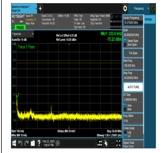
NTNV_DC_2A_n78A-3450-3550_PC3_30_5+40_ M+M_TID5_N/A_0.15_30_#1
