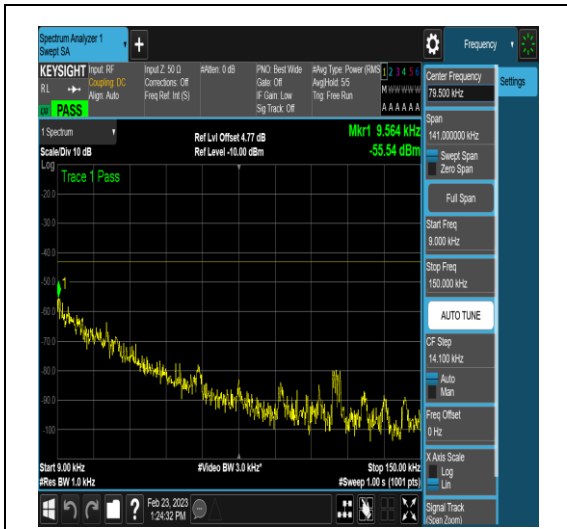
NTNV_DC_2A_n78A-3450-3550_PC3_30_5+40_ M+H_TID6_N/A_0.009_0.15_#1
