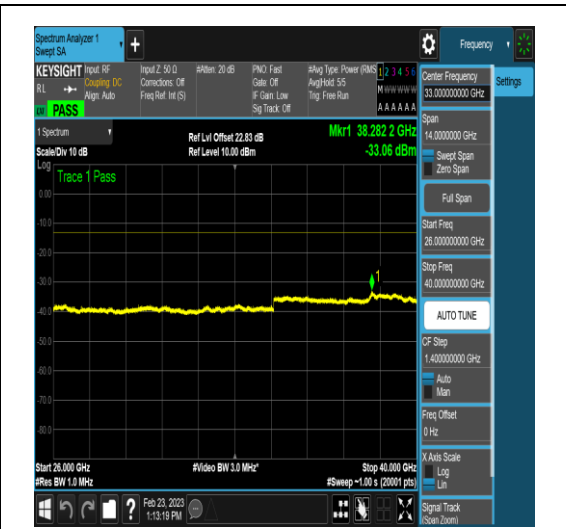
NTNV_DC_2A_n78A-3450-3550_PC3_30_5+40_ M+M_TID16_N/A_26000_40000_#1
