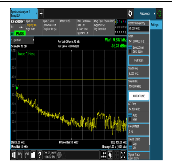
NTNV_DC_2A_n78A-3450-3550_PC3_30_5+40_ M+M_TID5_N/A_0.009_0.15_#1
