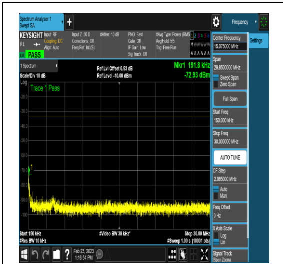
NTNV_DC_2A_n78A-3450-3550_PC3_30_5+40_ M+M_TID18_N/A_0.15_30_#1
