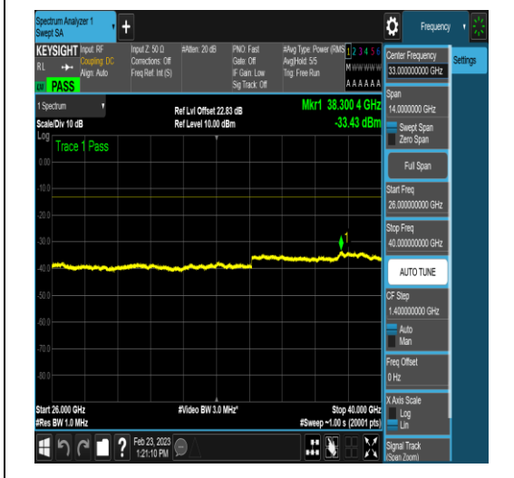
NTNV_DC_2A_n78A-3450-3550_PC3_30_5+40_ M+H_TID4_N/A_26000_40000_#1
