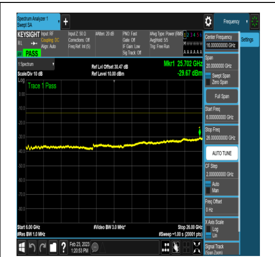
NTNV_DC_2A_n78A-3450-3550_PC3_30_5+40_ M+H_TID4_N/A_6000_26000_#1
