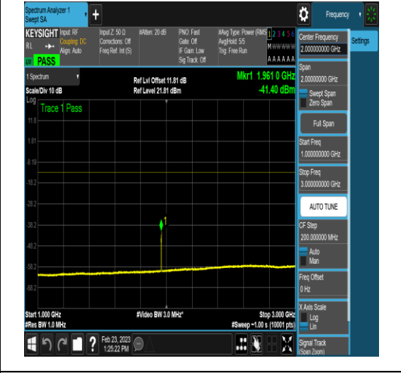
NTNV_DC_2A_n78A-3450-3550_PC3_30_5+40_ M+H_TID6_N/A_1000_3000_#1
