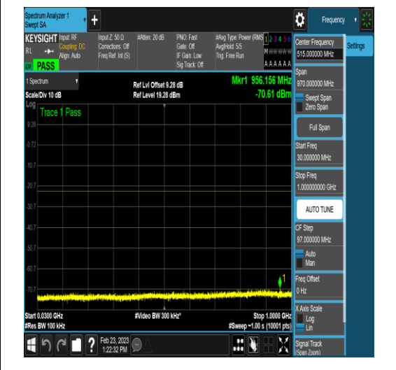
NTNV_DC_2A_n78A-3450-3550_PC3_30_5+40_ M+H_TID5_N/A_0.009_0.15_#1
