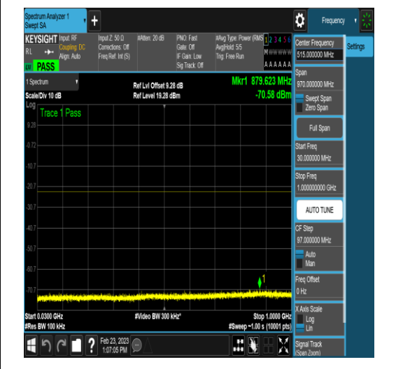
NTNV_DC_2A_n78A-3450-3550_PC3_30_5+40_ M+M_TID5_N/A_30_1000_#1
