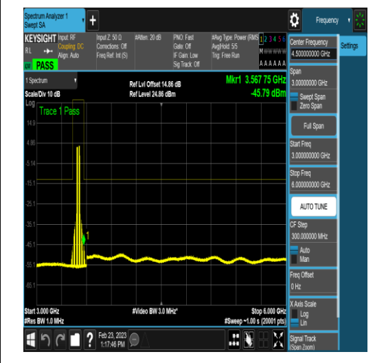
NTNV_DC_2A_n78A-3450-3550_PC3_30_5+40_ M+M_TID18_N/A_3000_6000_#1
