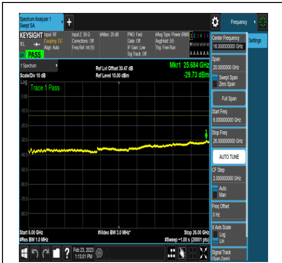
NTNV_DC_2A_n78A-3450-3550_PC3_30_5+40_ M+M_TID16_N/A_6000_26000_#1
