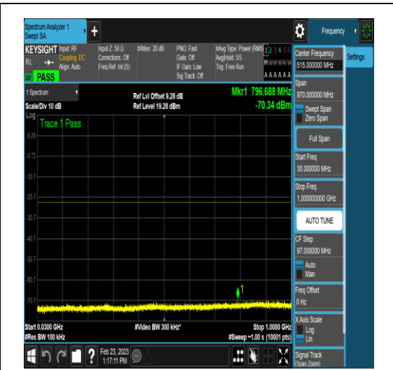
NTNV_DC_2A_n78A-3450-3550_PC3_30_5+40_ M+M_TID18_N/A_30_1000_#1
