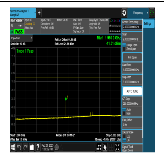
NTNV_DC_2A_n78A-3450-3550_PC3_30_5+40_ M+M_TID6_N/A_1000_3000_#1
