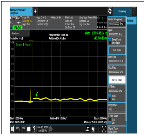
NTNV_DC_2A_n78A-3450-3550_PC3_30_5+40_ M+H_TID4_N/A_3000_6000_#1
