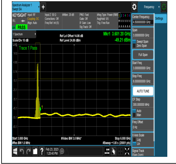
NTNV_DC_2A_n78A-3450-3550_PC3_30_5+40_ M+H_TID6_N/A_30_1000_#1
