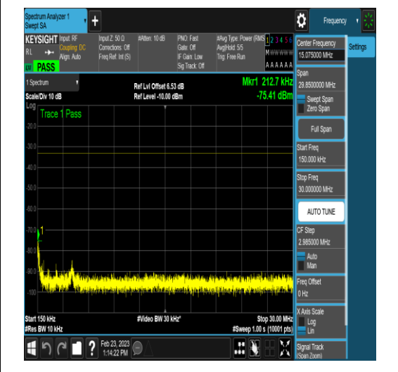
NTNV_DC_2A_n78A-3450-3550_PC3_30_5+40_ M+M_TID17_N/A_0.15_30_#1
