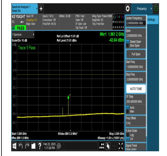
NTNV_DC_2A_n78A-3450-3550_PC3_30_5+40_ M+M_TID18_N/A_1000_3000_#1
