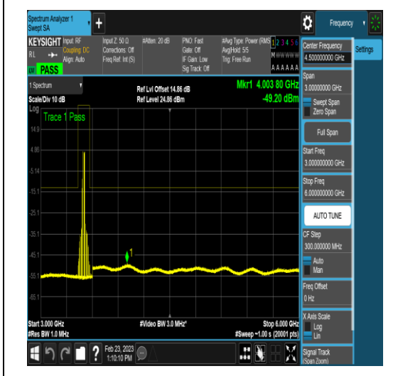
NTNV_DC_2A_n78A-3450-3550_PC3_30_5+40_ M+M_TID6_N/A_3000_6000_#1
