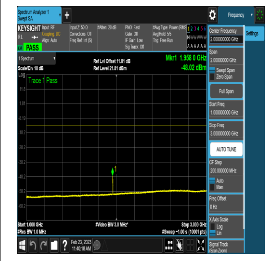
NTNV_DC_2A_n78A-3450-3550_PC3_30_5+20_ M+M_TID6_N/A_0.15_30_#1
