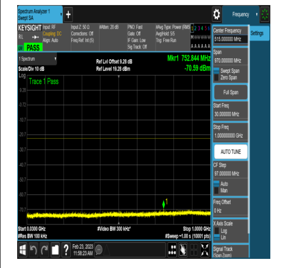
NTNV_DC_2A_n78A-3450-3550_PC3_30_5+20_ M+M_TID18_N/A_0.009_0.15_#1
