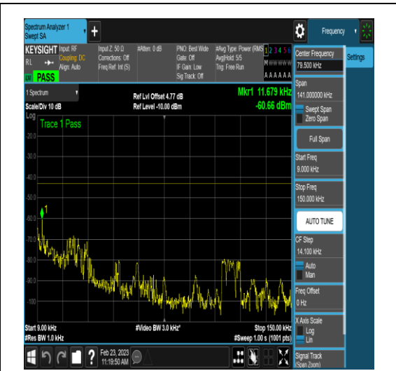
NTNV_DC_2A_n78A-3450-3550_PC3_30_5+20_ M+L_TID18_N/A_0.009_0.15_#1
