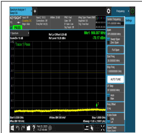
NTNV_DC_2A_n78A-3450-3550_PC3_30_5+20_ M+M_TID4_N/A_30_1000_#1
