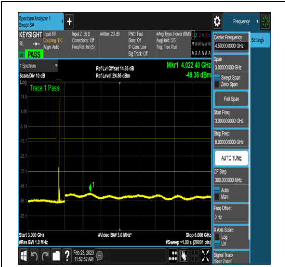
NTNV_DC_2A_n78A-3450-3550_PC3_30_5+20_ M+M_TID17_N/A_3000_6000_#1
