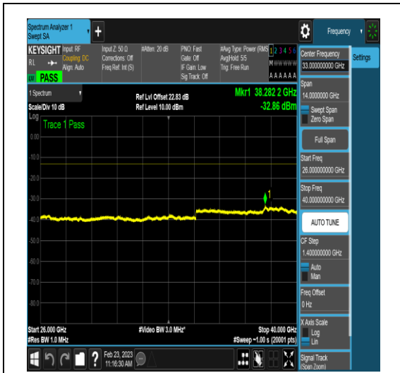
NTNV_DC_2A_n78A-3450-3550_PC3_30_5+20_ M+L_TID17_N/A_26000_40000_#1
