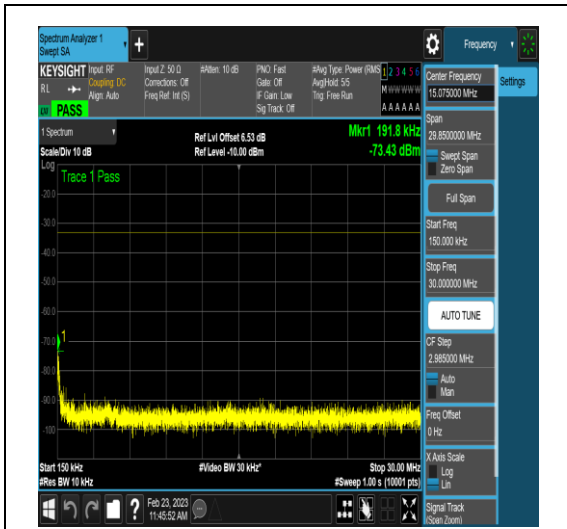
NTNV_DC_2A_n78A-3450-3550_PC3_30_5+20_ M+M_TID16_N/A_0.15_30_#1
