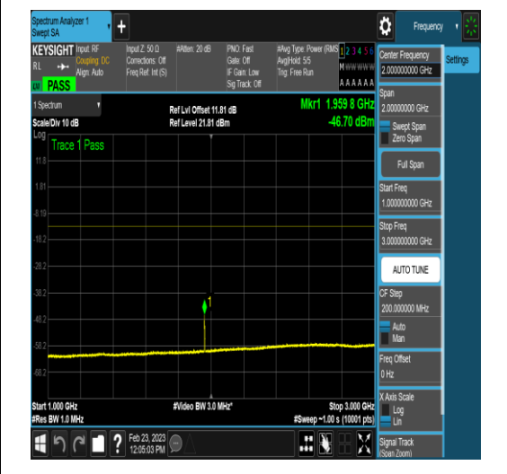
NTNV_DC_2A_n78A-3450-3550_PC3_30_5+20_ M+H_TID4_N/A_1000_3000_#1
