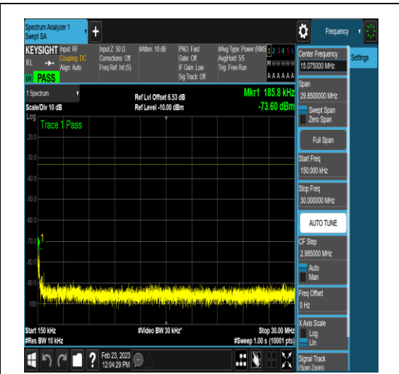
NTNV_DC_2A_n78A-3450-3550_PC3_30_5+20_ M+H_TID4_N/A_0.15_30_#1
