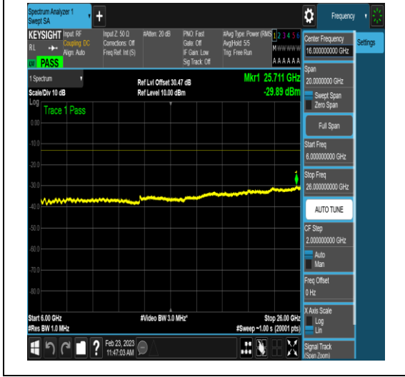
NTNV_DC_2A_n78A-3450-3550_PC3_30_5+20_ M+M_TID16_N/A_1000_3000_#1
