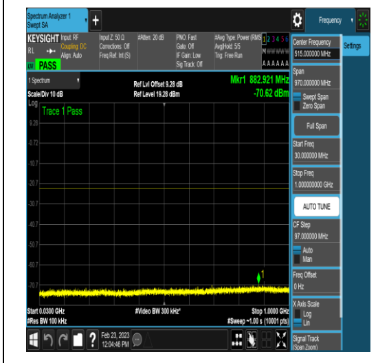
NTNV_DC_2A_n78A-3450-3550_PC3_30_5+20_ M+H_TID4_N/A_30_1000_#1
