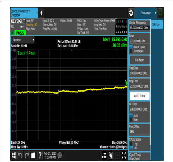
NTNV_DC_2A_n78A-3450-3550_PC3_30_5+20_ M+M_TID17_N/A_6000_26000_#1
