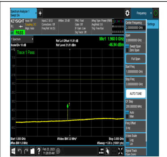
NTNV_DC_2A_n78A-3450-3550_PC3_30_5+20_ M+M_TID4_N/A_1000_3000_#1
