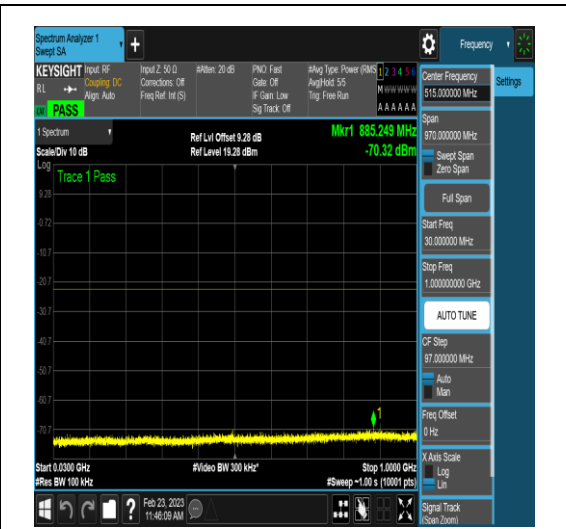
NTNV_DC_2A_n78A-3450-3550_PC3_30_5+20_ M+M_TID16_N/A_30_1000_#1
