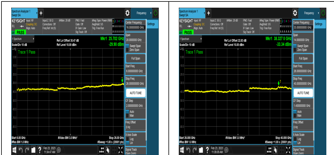
NTNV_DC_2A_n78A-3450-3550_PC3_30_5+20_ M+M_TID5_N/A_6000_26000_#1
