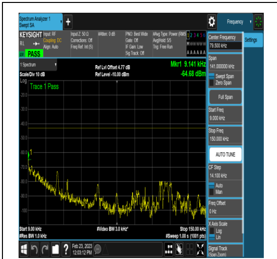
NTNV_DC_2A_n78A-3450-3550_PC3_30_5+20_ M+H_TID4_N/A_0.009_0.15_#1
