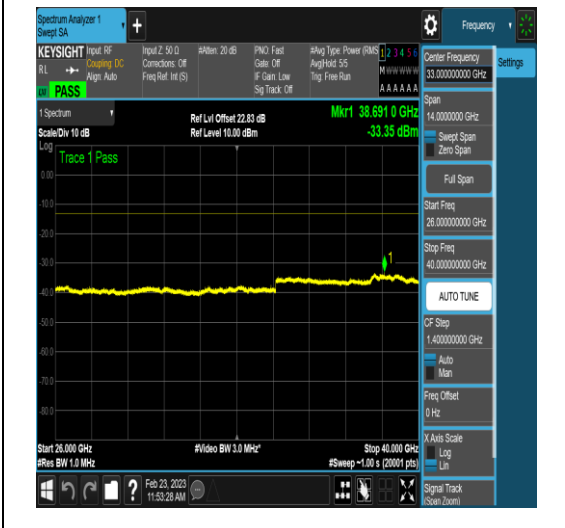
NTNV_DC_2A_n78A-3450-3550_PC3_30_5+20_ M+M_TID17_N/A_26000_40000_#1
