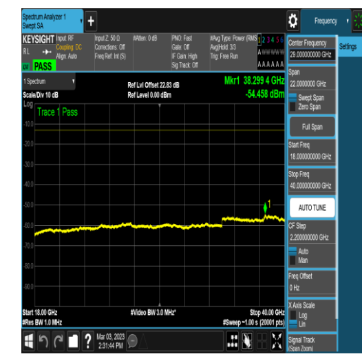
NTNV_N78-3700-3800_PC2_30_100_M_TID4_N/ A_1000_6000_#1
