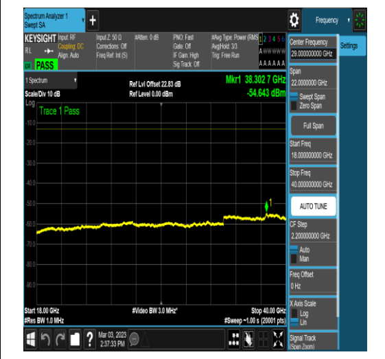
NTNV_N78-3700-3800_PC2_30_100_M_TID16_ N/A_18000_40000_#1
