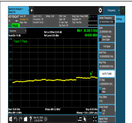
NTNV_N78-3700-3800_PC2_30_100_M_TID5_N/ A_18000_40000_#1
