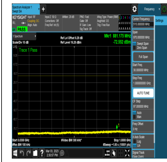
NTNV_N78-3700-3800_PC2_30_100_M_TID4_N/ A_30_1000_#1
