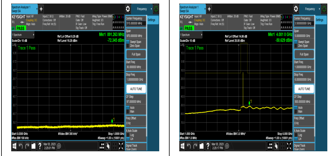
NTNV_N78-3700-3800_PC2_30_100_L_TID16_N/A_0.009_0.15_#1
