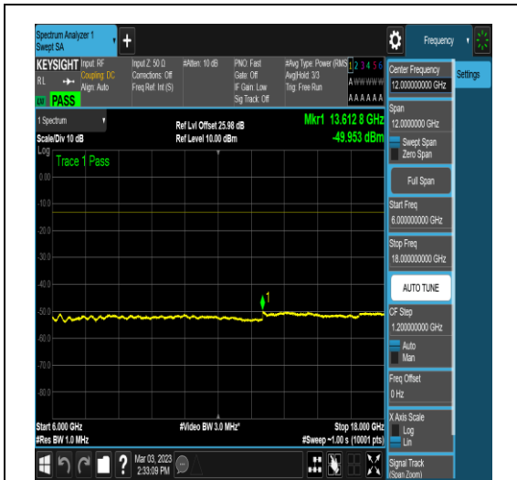
NTNV_N78-3700-3800_PC2_30_100_M_TID5_N/ A_6000_18000_#1
