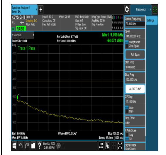
NTNV_N78-3700-3800_PC2_30_100_M_TID6_N/ A_0.009_0.15_#1
