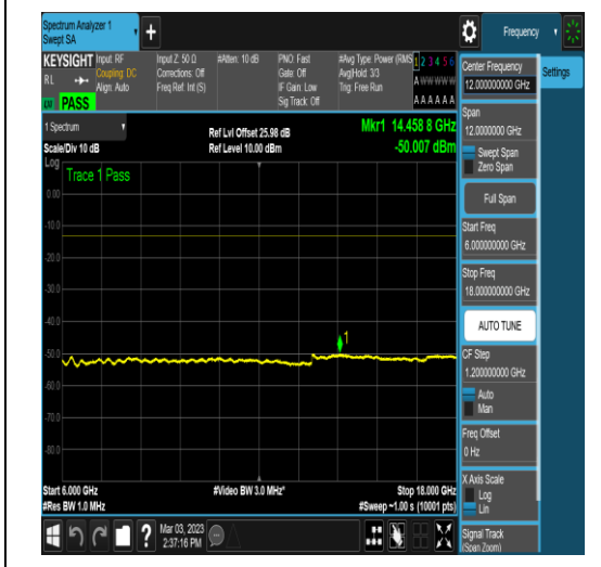
NTNV_N78-3700-3800_PC2_30_100_M_TID16_ N/A_6000_18000_#1
