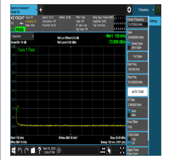
NTNV_N78-3700-3800_PC2_30_100_M_TID6_N/ A_0.15_30_#1
