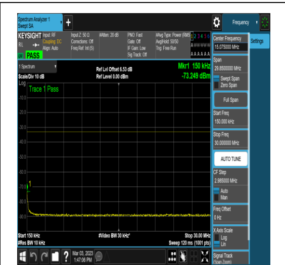
NTNV_N78-3700-3800_PC2_30_90_L_TID17_N/ A_0.15_30_#1
