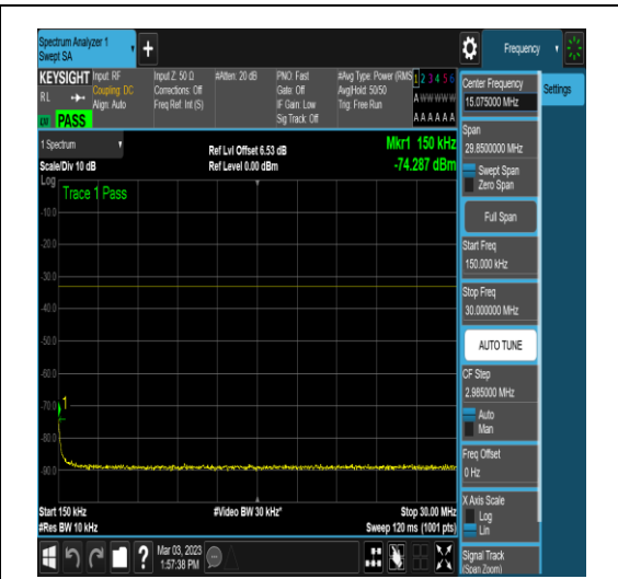
NTNV_N78-3700-3800_PC2_30_90_M_TID16_N/ A_0.15_30_#1
