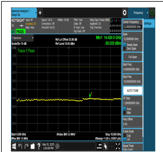
NTNV_N78-3700-3800_PC2_30_90_M_TID17_N/ A_6000_18000_#1
