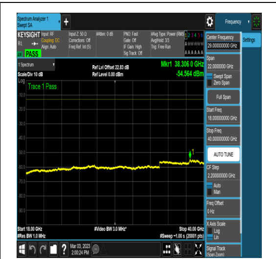
NTNV_N78-3700-3800_PC2_30_90_M_TID17_N/ A_18000_40000_#1
