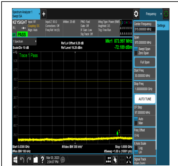
NTNV_N78-3700-3800_PC2_30_90_H_TID4_N/A _30_1000_#1
