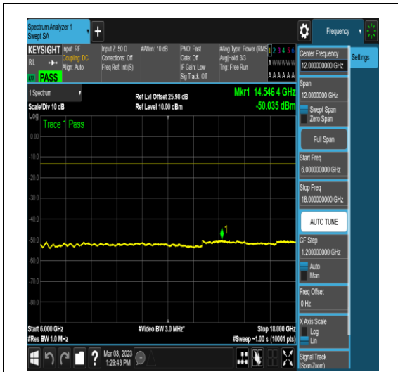
NTNV_N78-3700-3800_PC2_30_80_H_TID5_N/A _6000_18000_#1
