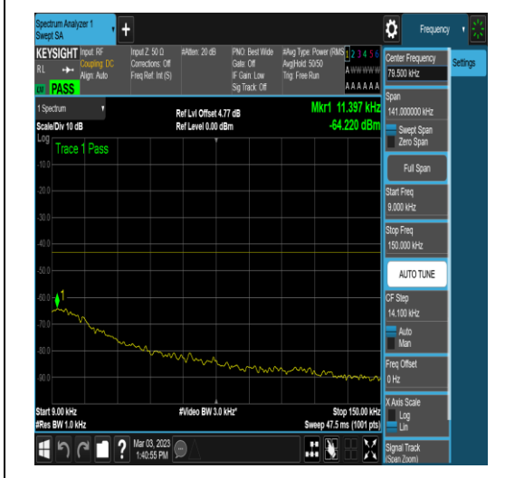
NTNV_N78-3700-3800_PC2_30_90_L_TID5_N/A _0.009_0.15_#1
