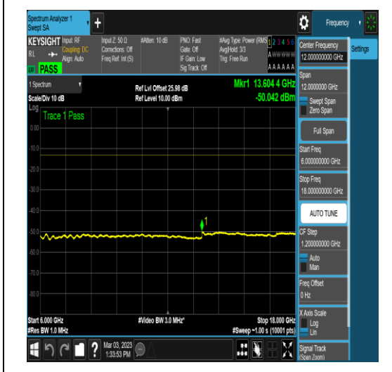
NTNV_N78-3700-3800_PC2_30_80_H_TID16_N/ A_6000_18000_#1
