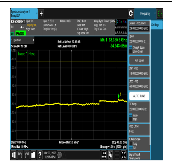
NTNV_N78-3700-3800_PC2_30_80_H_TID5_N/A _18000_40000_#1
