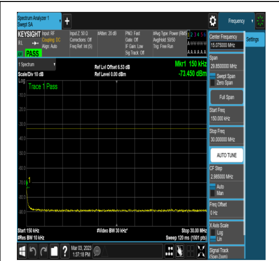
NTNV_N78-3700-3800_PC2_30_80_H_TID18_N/ A_0.15_30_#1
