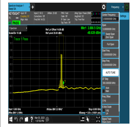
NTNV_N78-3700-3800_PC2_30_80_H_TID18_N/ A_1000_6000_#1
