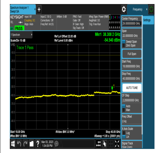
NTNV_N78-3700-3800_PC2_30_80_H_TID16_N/ A_18000_40000_#1
