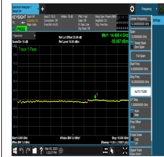
NTNV_N78-3700-3800_PC2_30_80_M_TID17_N/ A_6000_18000_#1
