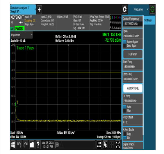
NTNV_N78-3700-3800_PC2_30_80_H_TID6_N/A _0.15_30_#1
