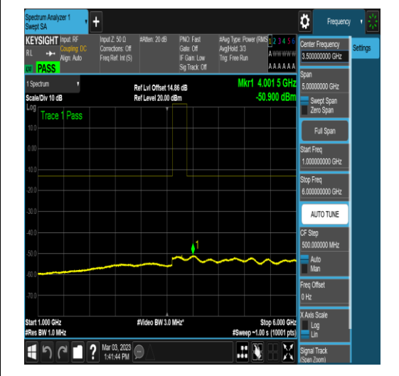
NTNV_N78-3700-3800_PC2_30_90_L_TID5_N/A _0.15_30_#1
