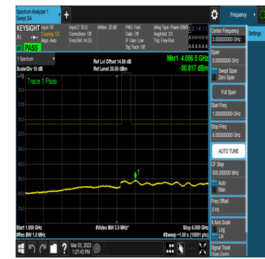
NTNV_N78-3700-3800_PC2_30_80_H_TID4_N/A _1000_6000_#1
