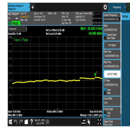
NTNV_N78-3700-3800_PC2_30_80_M_TID17_N/ A_18000_40000_#1
