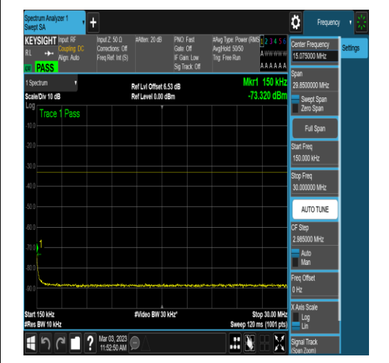
NTNV_N78-3700-3800_PC2_30_50_L_TID4_N/A_0.15_30_#1
