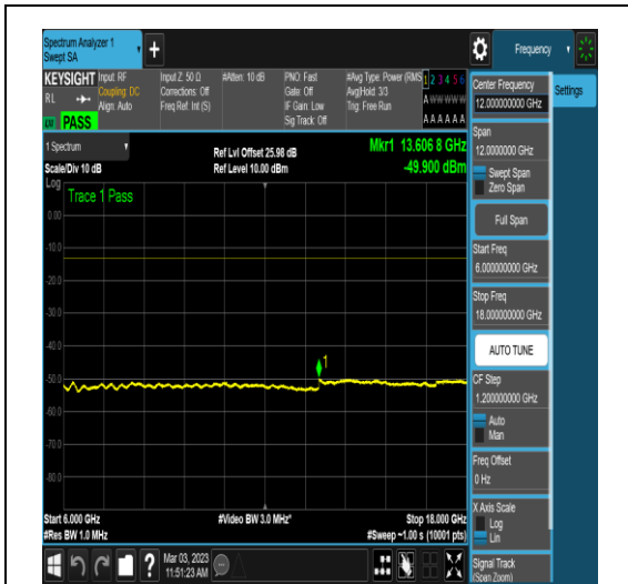
NTNV_N78-3700-3800_PC2_30_40_H_TID18_N/A_6000_18000_#1
