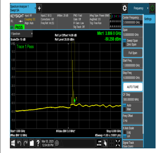
NTNV_N78-3700-3800_PC2_30_50_L_TID18_N/A_0.15_30_#1
