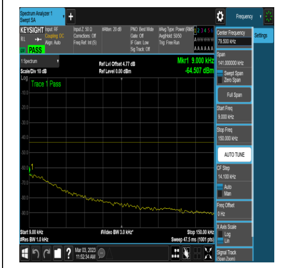
NTNV_N78-3700-3800_PC2_30_50_L_TID4_N/A_0.009_0.15_#1
