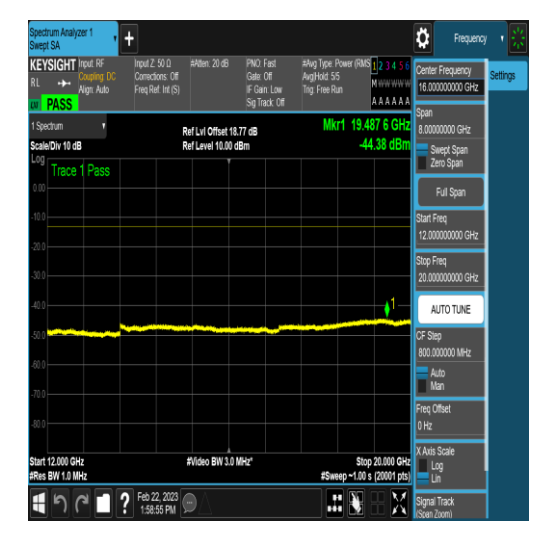
NTNV_N78-3650-3700_PC2_30_40_H_TID16_N/ A_12000_20000_#1
