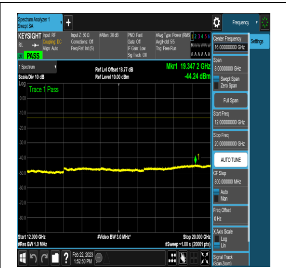
NTNV_N78-3650-3700_PC2_30_40_H_TID4_N/A _12000_20000_#1
