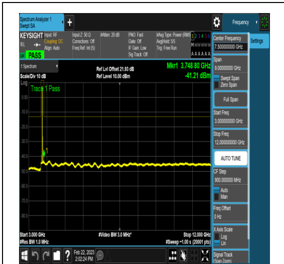
NTNV_N78-3650-3700_PC2_30_40_H_TID18_N/ A_3000_12000_#1
