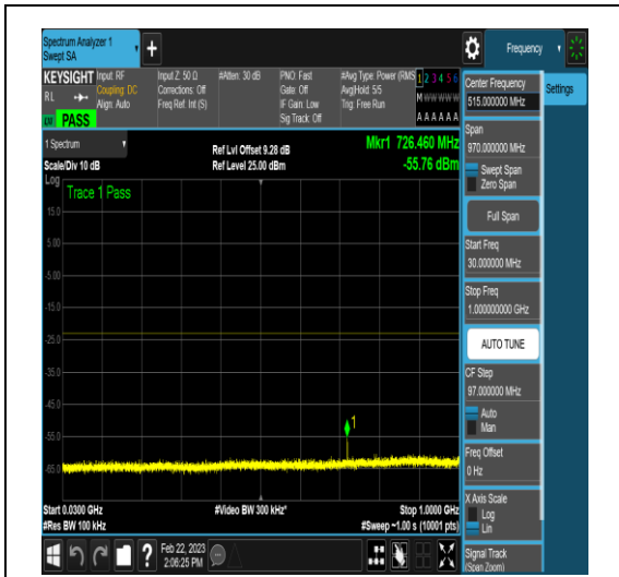
NTNV_N78-3650-3700_PC2_30_50_M_TID5_N/A _30_1000_#1
