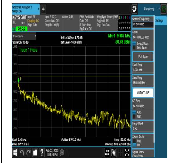
NTNV_N78-3650-3700_PC2_30_40_H_TID5_N/A _0.009_0.15_#1
