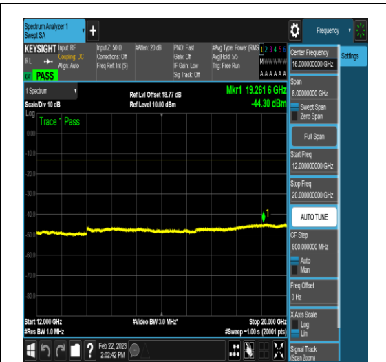
NTNV_N78-3650-3700_PC2_30_40_H_TID18_N/ A_12000_20000_#1
