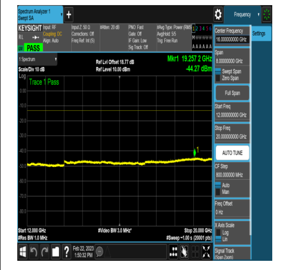
NTNV_N78-3650-3700_PC2_30_40_M_TID18_N/ A_1000_3000_#1
