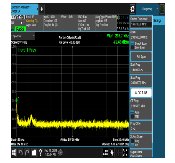
NTNV_N78-3650-3700_PC2_30_40_H_TID5_N/A _0.15_30_#1
