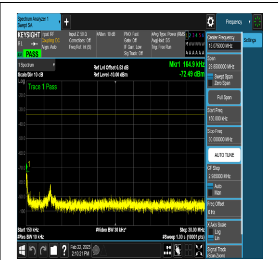
NTNV_N78-3650-3700_PC2_30_50_M_TID16_N/ A_0.15_30_#1
