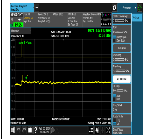
NTNV_N78-3650-3700_PC2_30_50_M_TID5_N/A _3000_12000_#1
