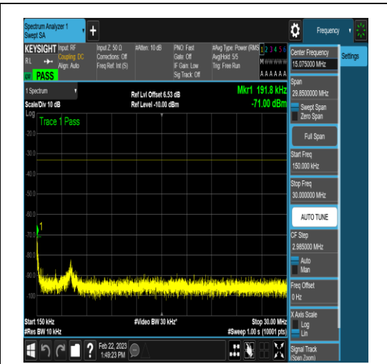
NTNV_N78-3650-3700_PC2_30_40_M_TID18_N/ A_0.15_30_#1
