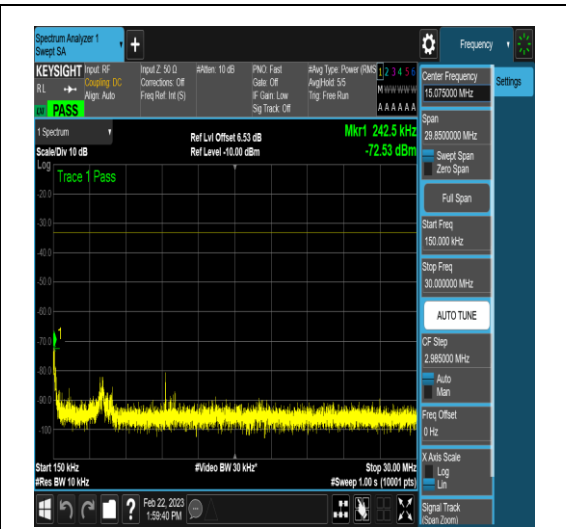
NTNV_N78-3650-3700_PC2_30_40_H_TID17_N/ A_0.15_30_#1
