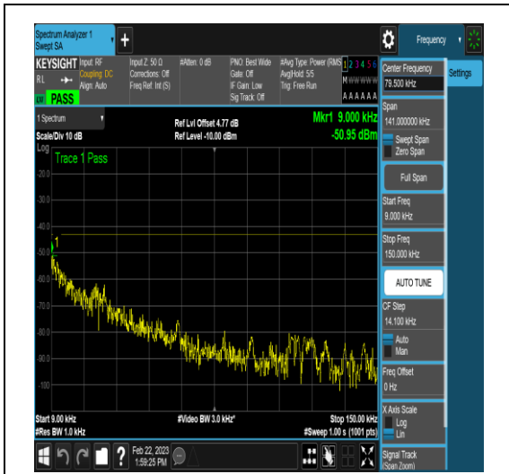
NTNV_N78-3650-3700_PC2_30_40_H_TID17_N/ A_0.009_0.15_#1
