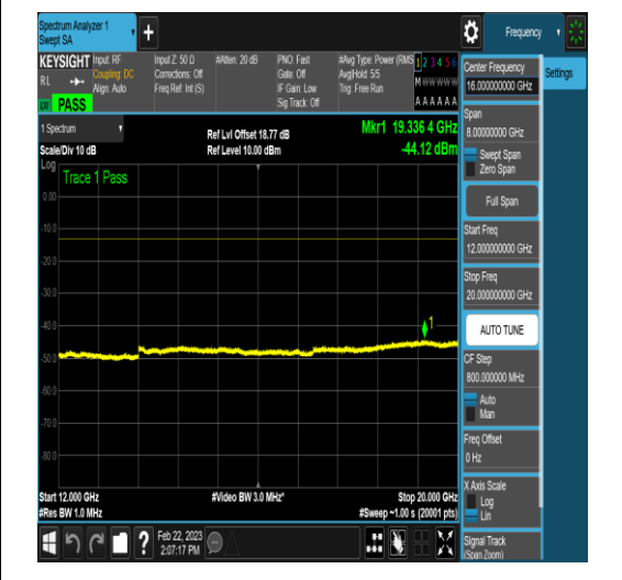
NTNV_N78-3650-3700_PC2_30_50_M_TID5_N/A _12000_20000_#1
