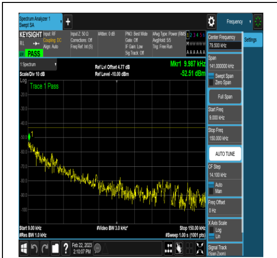
NTNV_N78-3650-3700_PC2_30_50_M_TID16_N/ A_0.009_0.15_#1
