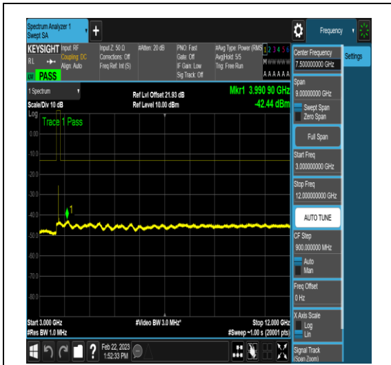
NTNV_N78-3650-3700_PC2_30_40_H_TID4_N/A _3000_12000_#1
