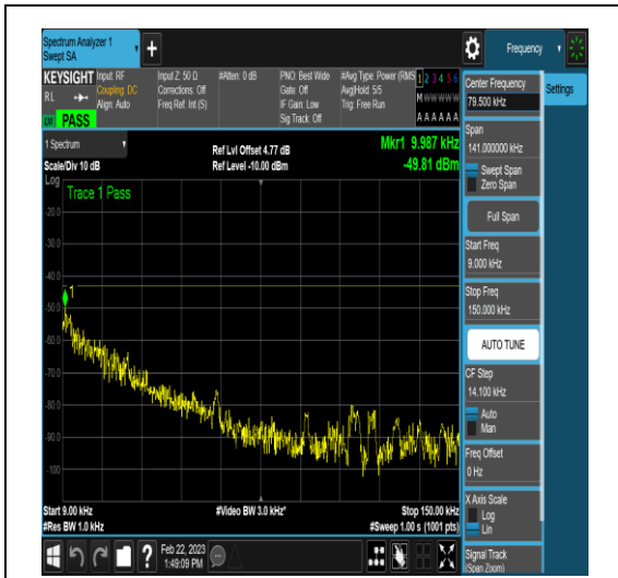
NTNV_N78-3650-3700_PC2_30_40_M_TID18_N/ A_0.009_0.15_#1
