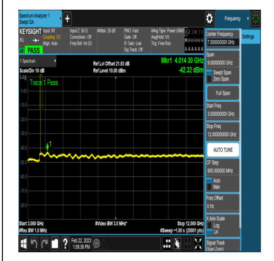
NTNV_N78-3650-3700_PC2_30_40_H_TID16_N/ A_3000_12000_#1
