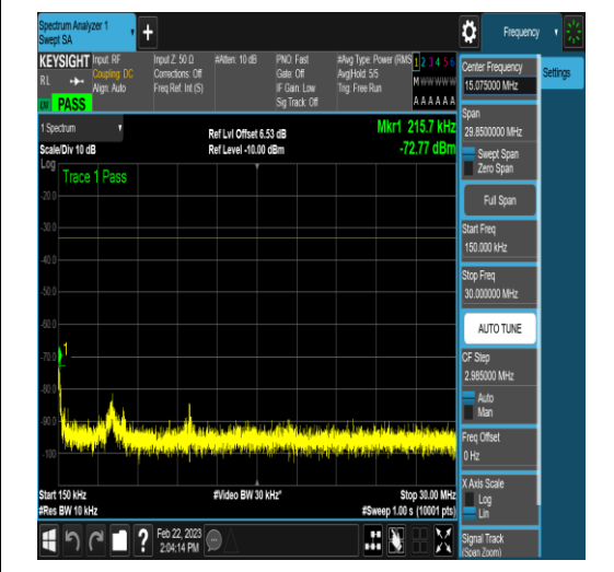
NTNV_N78-3650-3700_PC2_30_50_M_TID4_N/A _0.15_30_#1
