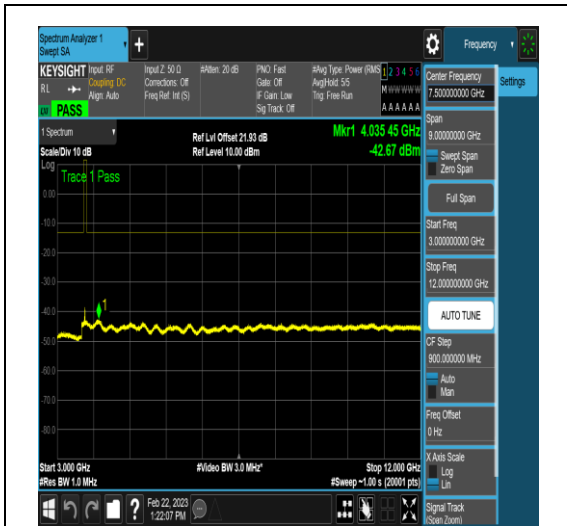
NTNV_N78-3650-3700_PC2_30_20_H_TID16_N/ A_3000_12000_#1
