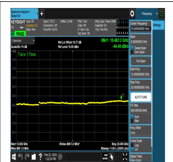
NTNV_N78-3650-3700_PC2_30_20_H_TID16_N/ A_12000_20000_#1
