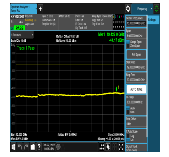
NTNV_N78-3650-3700_PC2_30_20_M_TID5_N/A _12000_20000_#1
