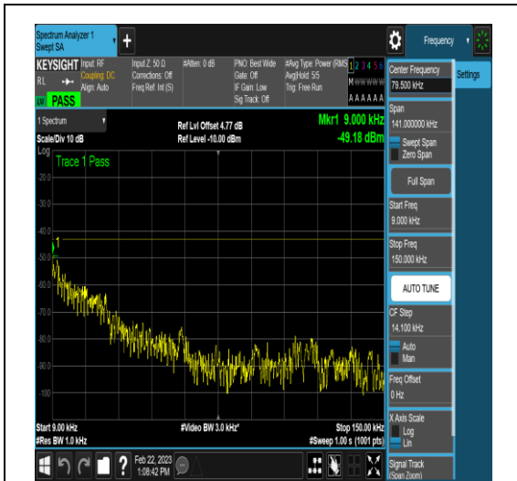
NTNV_N78-3650-3700_PC2_30_20_M_TID16_N/ A_0.009_0.15_#1
