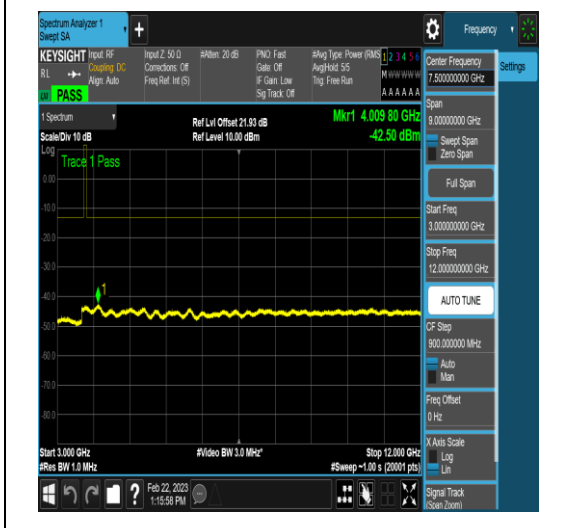
NTNV_N78-3650-3700_PC2_30_20_H_TID4_N/A _3000_12000_#1
