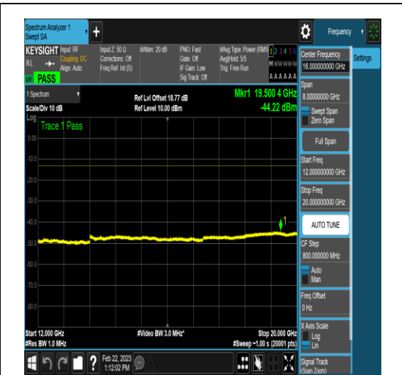
NTNV_N78-3650-3700_PC2_30_20_M_TID17_N/ A_12000_20000_#1
