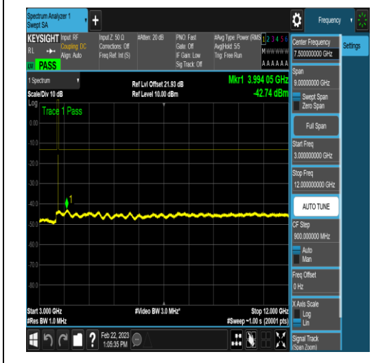
NTNV_N78-3650-3700_PC2_30_20_M_TID5_N/A _3000_12000_#1
