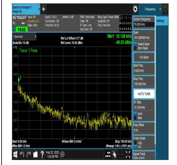
NTNV_N78-3650-3700_PC2_30_20_M_TID4_N/A_0.009_0.15_#1
