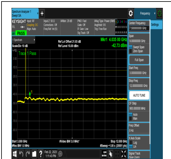
NTNV_N78-3650-3700_PC2_30_20_M_TID17_N/ A_3000_12000_#1
