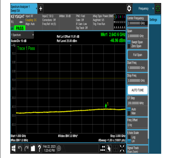
NTNV_N78-3650-3700_PC2_30_20_H_TID17_N/ A_0.15_30_#1
