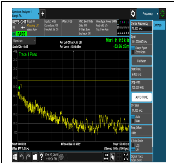
NTNV_N78-3650-3700_PC2_30_20_H_TID6_N/A _0.009_0.15_#1
