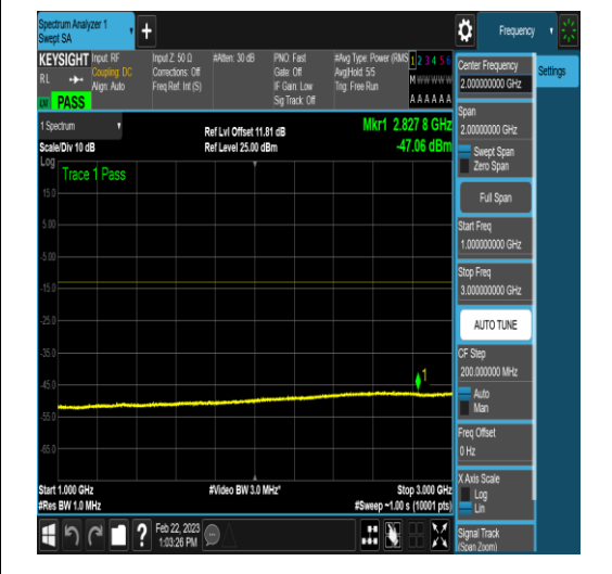
NTNV_N78-3650-3700_PC2_30_20_M_TID4_N/A_0.15_30_#1
