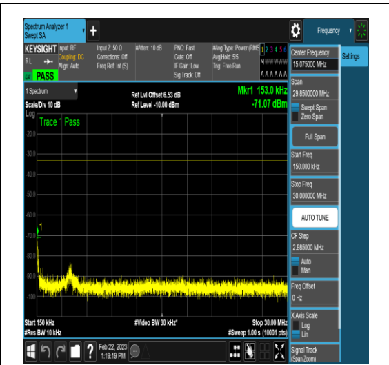
NTNV_N78-3650-3700_PC2_30_20_H_TID6_N/A _0.15_30_#1
