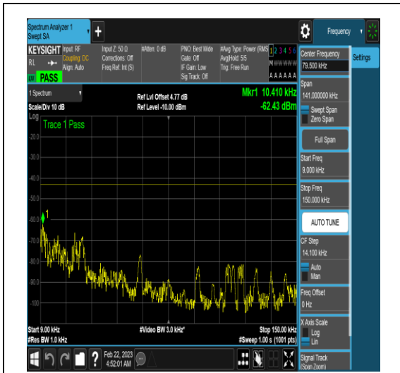
NTNV_N78-3450-3550_PC2_30_100_M_TID4_N/ A_0.009_0.15_#1
