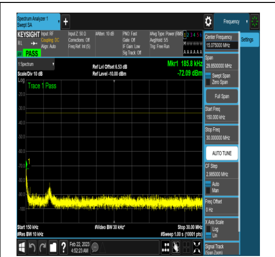
NTNV_N78-3450-3550_PC2_30_100_M_TID4_N/ A_0.15_30_#1
