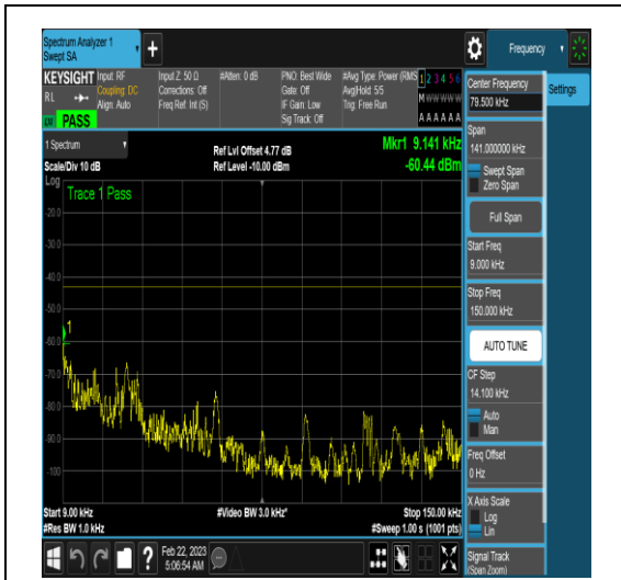
NTNV_N78-3450-3550_PC2_30_100_M_TID18_ N/A_0.009_0.15_#1
