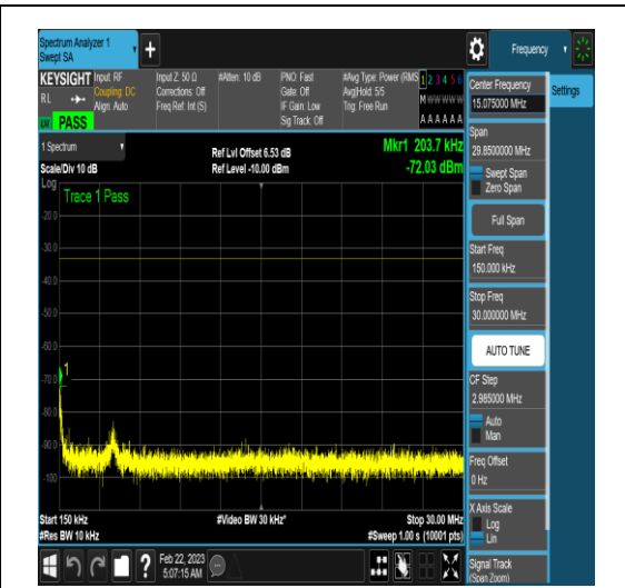
NTNV_N78-3450-3550_PC2_30_100_M_TID18_ N/A_0.15_30_#1
