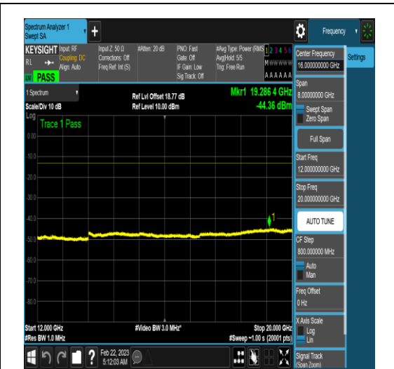
NTNV_N78-3450-3550_PC2_30_100_H_TID4_N/ A_12000_20000_#1
