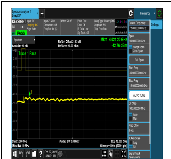
NTNV_N78-3450-3550_PC2_30_100_M_TID5_N/ A_3000_12000_#1
