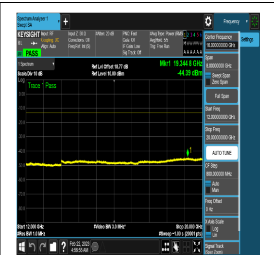
NTNV_N78-3450-3550_PC2_30_100_M_TID5_N/ A_12000_20000_#1
