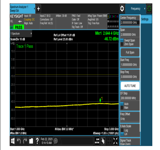
NTNV_N78-3450-3550_PC2_30_100_H_TID5_N/ A_0.15_30_#1
