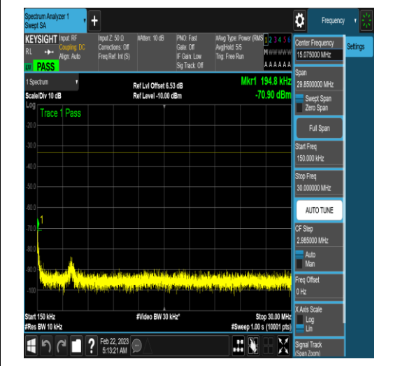
NTNV_N78-3450-3550_PC2_30_100_H_TID5_N/ A_0.15_30_#1
