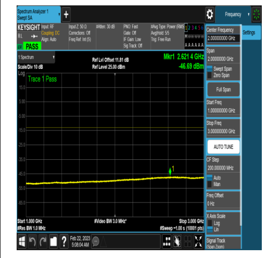
NTNV_N78-3450-3550_PC2_30_100_M_TID18_ N/A_1000_3000_#1
