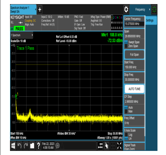
NTNV_N78-3450-3550_PC2_30_100_M_TID6_N/ A_0.15_30_#1
