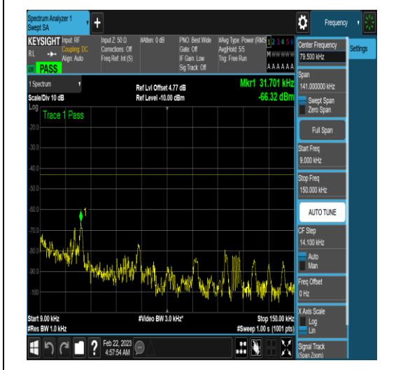
NTNV_N78-3450-3550_PC2_30_100_M_TID6_N/ A_0.009_0.15_#1
