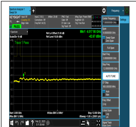
NTNV_N78-3450-3550_PC2_30_100_H_TID4_N/ A_3000_12000_#1
