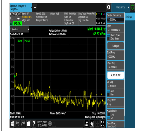
NTNV_N78-3450-3550_PC2_30_100_H_TID5_N/ A_0.009_0.15_#1
