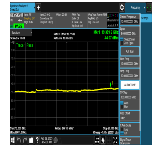
NTNV_N78-3450-3550_PC2_30_100_M_TID4_N/ A_1000_3000_#1
