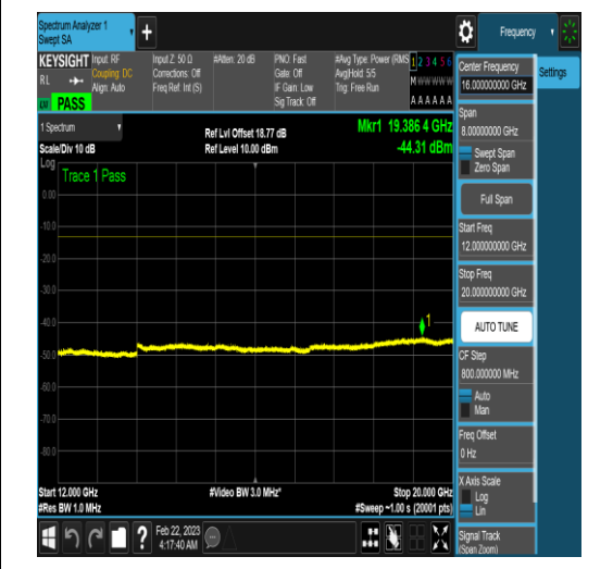
NTNV_N78-3450-3550_PC2_30_90_H_TID4_N/A _12000_20000_#1
