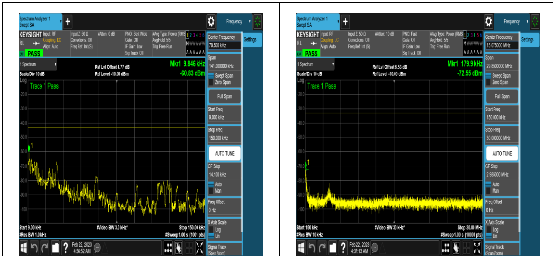
NTNV_N78-3450-3550_PC2_30_100_L_TID5_N/ A_0.009_0.15_#1
