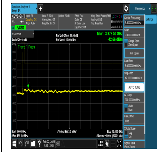
NTNV_N78-3450-3550_PC2_30_90_H_TID18_N/ A_3000_12000_#1
