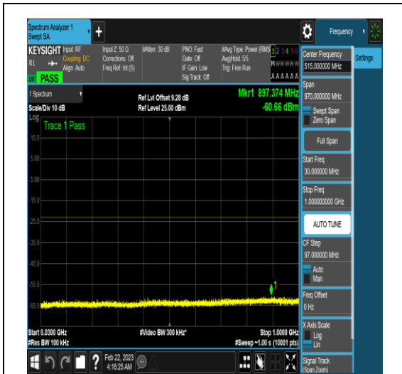
NTNV_N78-3450-3550_PC2_30_90_H_TID4_N/A _30_1000_#1
