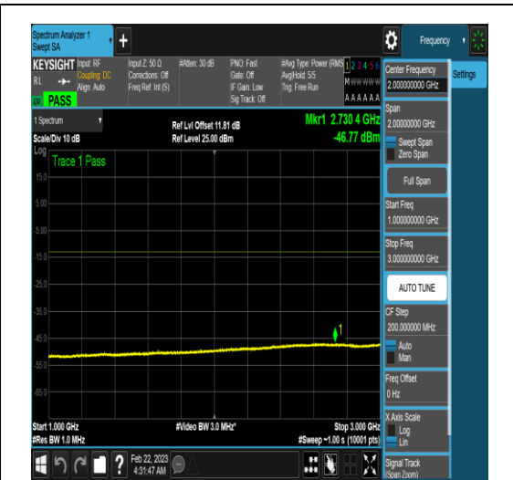
NTNV_N78-3450-3550_PC2_30_90_H_TID18_N/ A_1000_3000_#1
