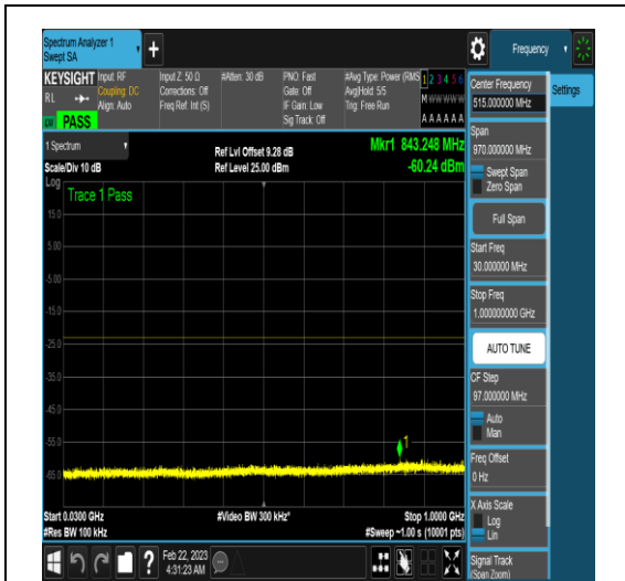
NTNV_N78-3450-3550_PC2_30_90_H_TID18_N/ A_30_1000_#1
