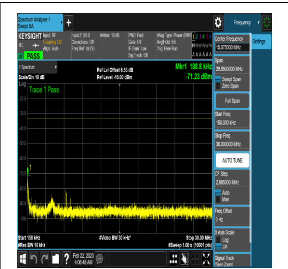
NTNV_N78-3450-3550_PC2_30_90_M_TID16_N/ A_0.15_30_#1
