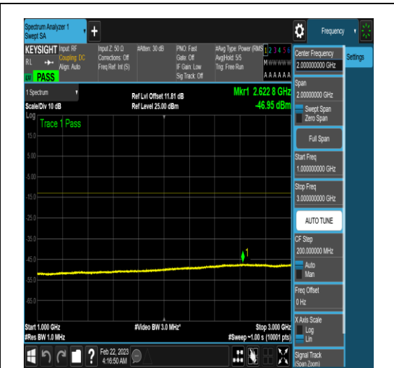
NTNV_N78-3450-3550_PC2_30_90_H_TID4_N/A _1000_3000_#1
