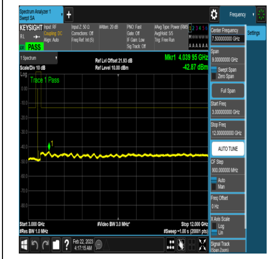
NTNV_N78-3450-3550_PC2_30_90_H_TID4_N/A _3000_12000_#1
