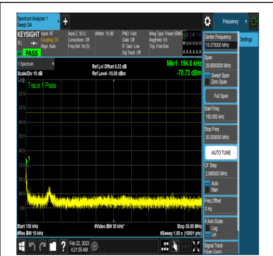
NTNV_N78-3450-3550_PC2_30_90_H_TID6_N/A _0.15_30_#1
