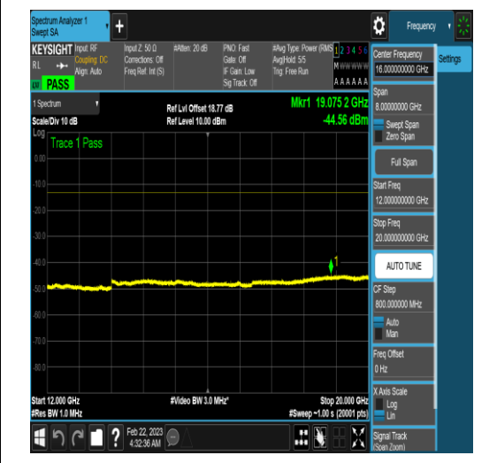
NTNV_N78-3450-3550_PC2_30_90_H_TID18_N/ A_12000_20000_#1
