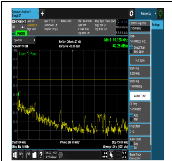
NTNV_N78-3450-3550_PC2_30_90_H_TID6_N/A _0.009_0.15_#1
