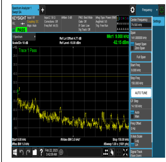
NTNV_N78-3450-3550_PC2_30_90_L_TID5_N/A _0.009_0.15_#1
