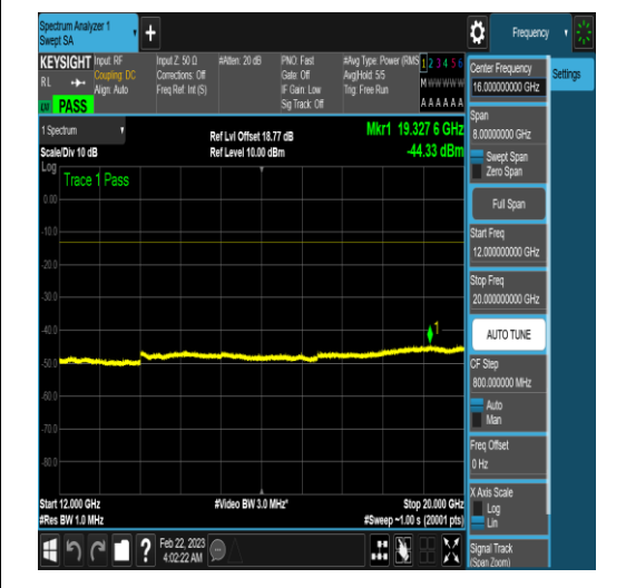
NTNV_N78-3450-3550_PC2_30_90_M_TID5_N/A _12000_20000_#1
