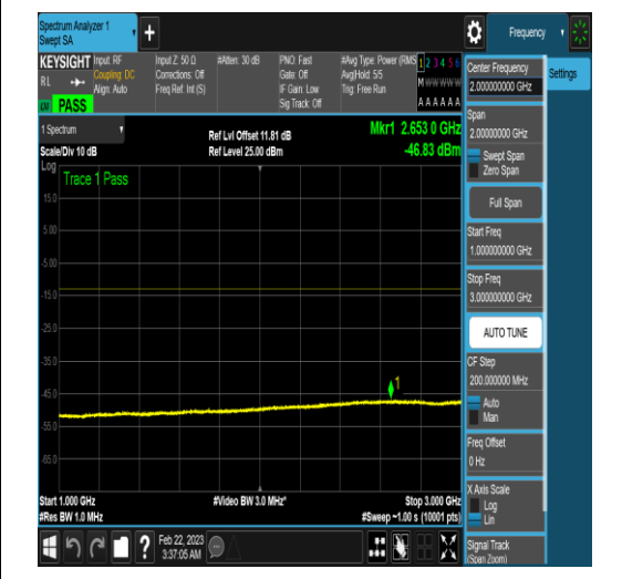
NTNV_N78-3450-3550_PC2_30_80_H_TID18_N/ A_1000_3000_#1
