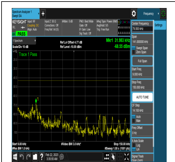
NTNV_N78-3450-3550_PC2_30_80_H_TID18_N/ A_0.009_0.15_#1
