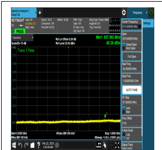
NTNV_N78-3450-3550_PC2_30_80_H_TID16_N/ A_30_1000_#1
