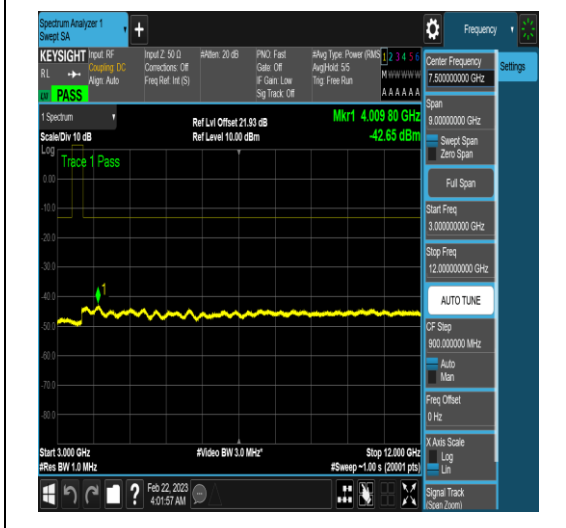
NTNV_N78-3450-3550_PC2_30_90_M_TID5_N/A _3000_12000_#1
