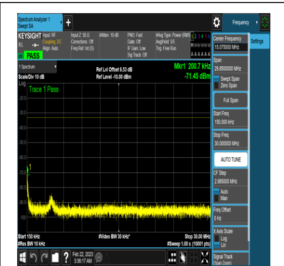
NTNV_N78-3450-3550_PC2_30_80_H_TID18_N/ A_0.15_30_#1
