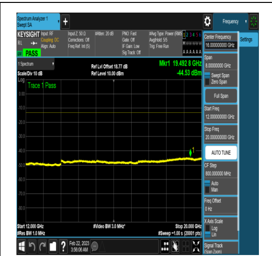
NTNV_N78-3450-3550_PC2_30_90_L_TID18_N/A_12000_20000_#1
