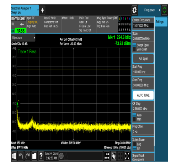
NTNV_N78-3450-3550_PC2_30_90_L_TID5_N/A _0.15_30_#1
