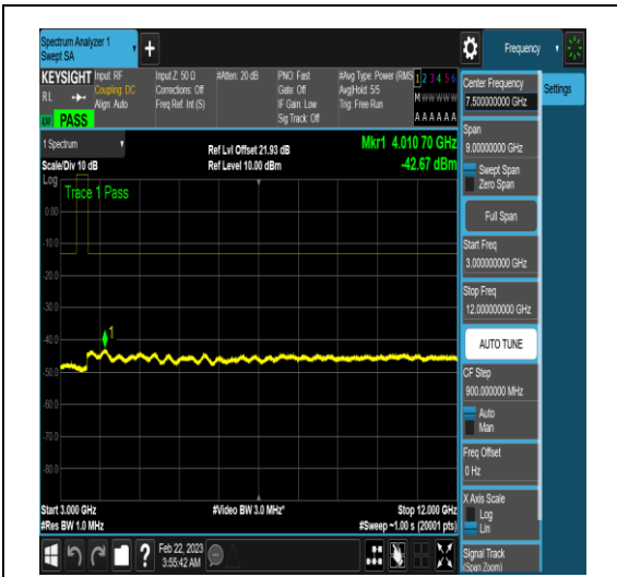
NTNV_N78-3450-3550_PC2_30_90_L_TID18_N/A_3000_12000_#1
