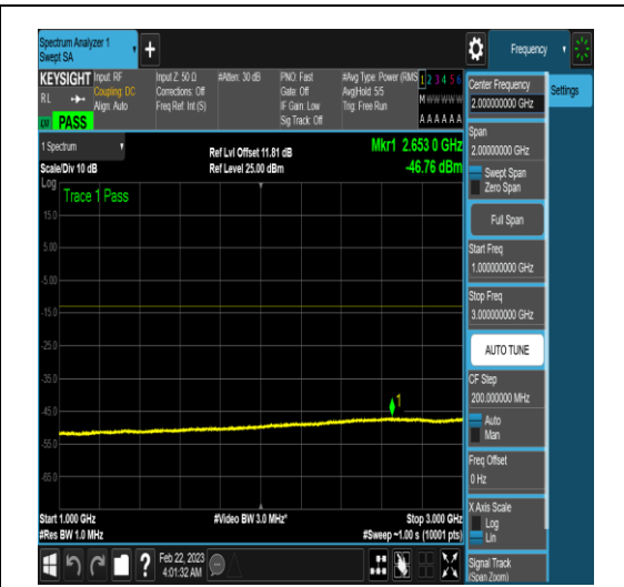
NTNV_N78-3450-3550_PC2_30_90_M_TID5_N/A _1000_3000_#1
