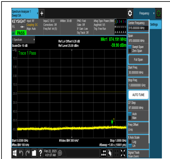
NTNV_N78-3450-3550_PC2_30_90_M_TID5_N/A _30_1000_#1
