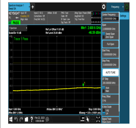
NTNV_N78-3450-3550_PC2_30_90_M_TID4_N/A_0.15_30_#1
