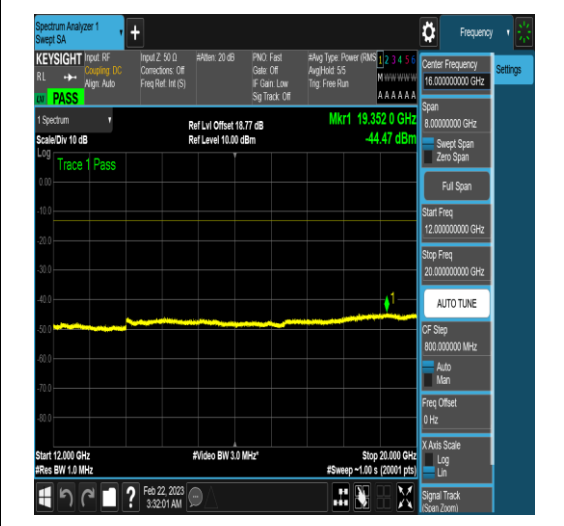
NTNV_N78-3450-3550_PC2_30_80_H_TID16_N/ A_12000_20000_#1
