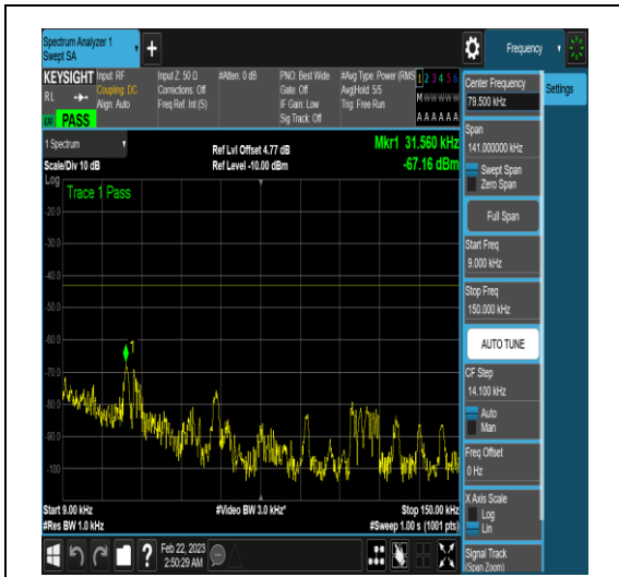
NTNV_N78-3450-3550_PC2_30_80_L_TID6_N/A _0.009_0.15_#1
