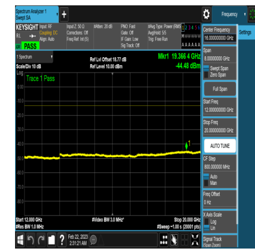
NTNV_N78-3450-3550_PC2_30_60_H_TID5_N/A _12000_20000_#1
