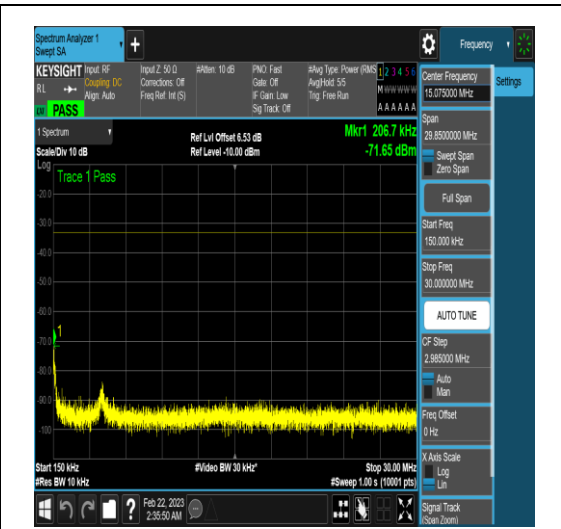
NTNV_N78-3450-3550_PC2_30_60_H_TID16_N/ A_0.15_30_#1
