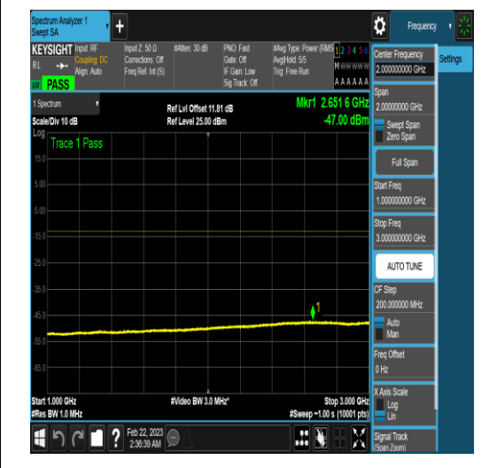
NTNV_N78-3450-3550_PC2_30_60_H_TID16_N/ A_1000_3000_#1
