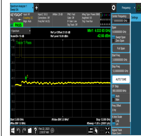
NTNV_N78-3450-3550_PC2_30_60_H_TID5_N/A _3000_12000_#1
