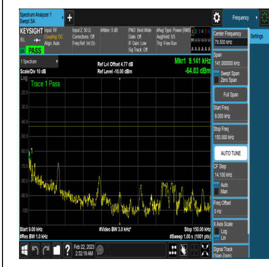
NTNV_N78-3450-3550_PC2_30_60_H_TID5_N/A _3000_12000_#1
