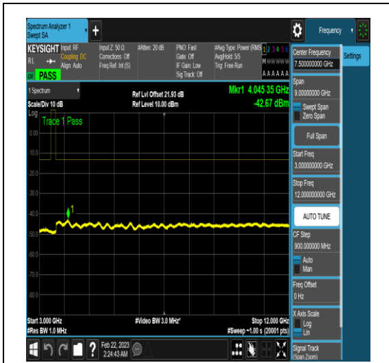
NTNV_N78-3450-3550_PC2_30_60_M_TID18_N/ A_3000_12000_#1
