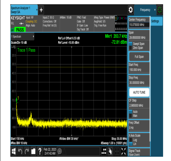
NTNV_N78-3450-3550_PC2_30_60_H_TID18_N/ A_0.15_30_#1
