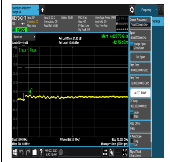
NTNV_N78-3450-3550_PC2_30_80_L_TID4_N/A _3000_12000_#1
