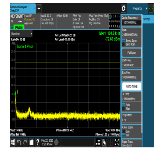
NTNV_N78-3450-3550_PC2_30_60_H_TID4_N/A _0.15_30_#1
