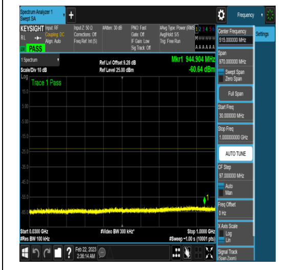
NTNV_N78-3450-3550_PC2_30_60_H_TID16_N/ A_30_1000_#1
