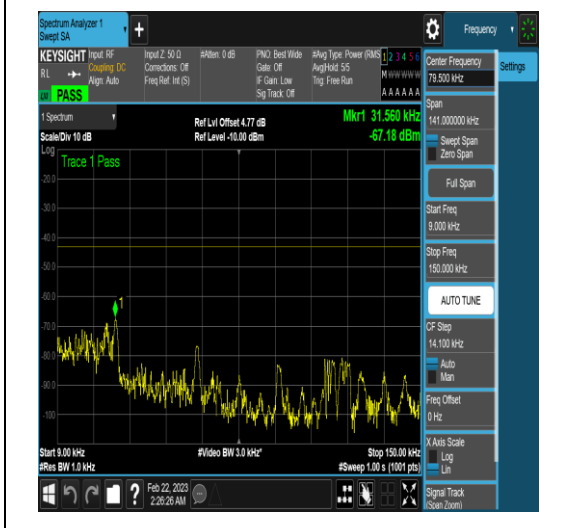
NTNV_N78-3450-3550_PC2_30_60_H_TID4_N/A _0.009_0.15_#1
