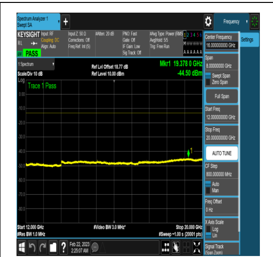
NTNV_N78-3450-3550_PC2_30_60_M_TID18_N/ A_12000_20000_#1
