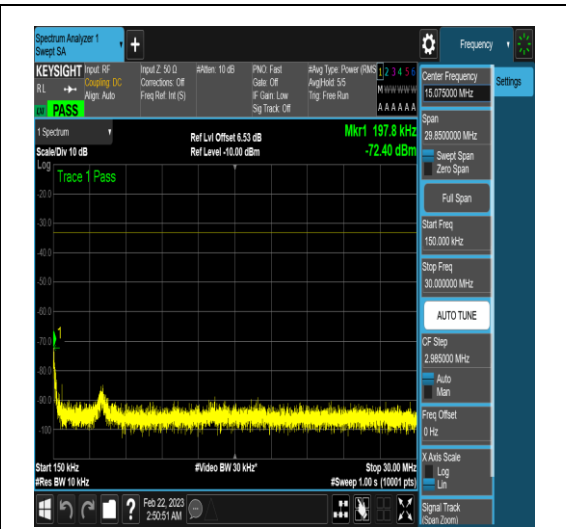
NTNV_N78-3450-3550_PC2_30_80_L_TID6_N/A _0.15_30_#1
