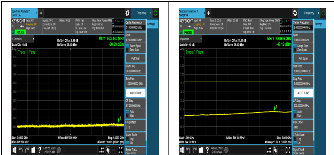
NTNV_N78-3450-3550_PC2_30_60_H_TID5_N/A _30_1000_#1
