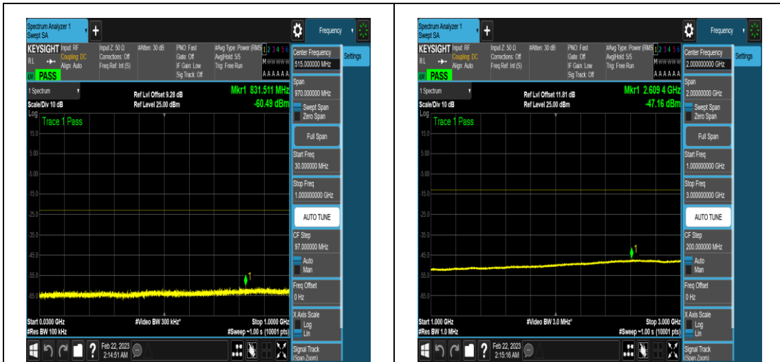
NTNV_N78-3450-3550_PC2_30_60_M_TID6_N/A _30_1000_#1
