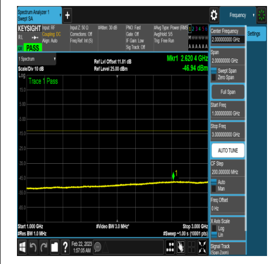
NTNV_N78-3450-3550_PC2_30_60_L_TID6_N/A _0.15_30_#1
