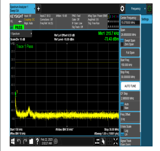
NTNV_N78-3450-3550_PC2_30_60_L_TID16_N/ A_12000_20000_#1
