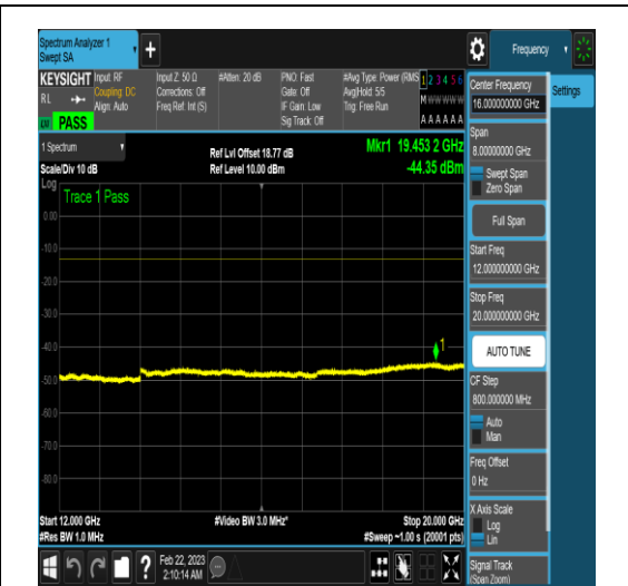
NTNV_N78-3450-3550_PC2_30_60_M_TID4_N/A _12000_20000_#1
