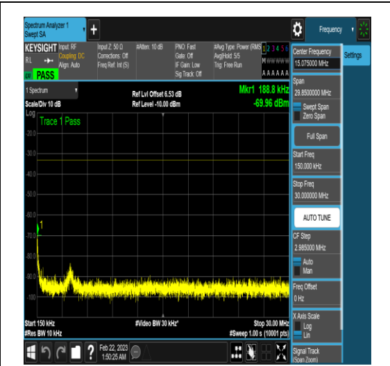
NTNV_N78-3450-3550_PC2_30_60_L_TID4_N/A _0.15_30_#1
