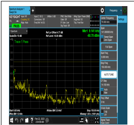
NTNV_N78-3450-3550_PC2_30_60_L_TID18_N/ A_0.009_0.15_#1
