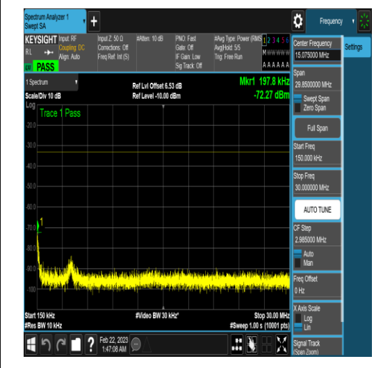
NTNV_N78-3450-3550_PC2_30_50_H_TID17_N/ A_12000_20000_#1
