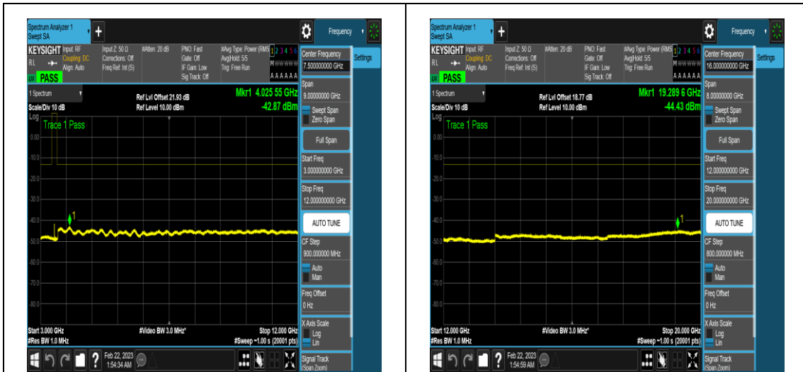
NTNV_N78-3450-3550_PC2_30_60_L_TID5_N/A _3000_12000_#1
