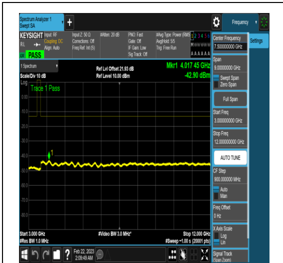
NTNV_N78-3450-3550_PC2_30_60_M_TID4_N/A _3000_12000_#1
