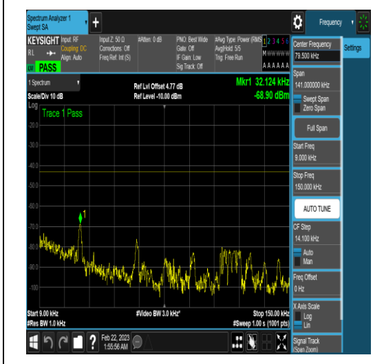
NTNV_N78-3450-3550_PC2_30_60_L_TID6_N/A _0.009_0.15_#1
