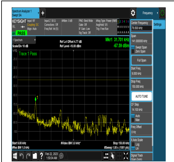
NTNV_N78-3450-3550_PC2_30_60_L_TID4_N/A _0.009_0.15_#1
