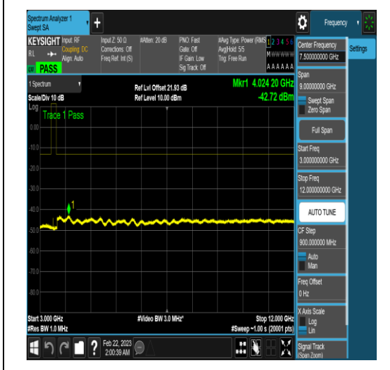
NTNV_N78-3450-3550_PC2_30_60_L_TID16_N/ A_3000_12000_#1
