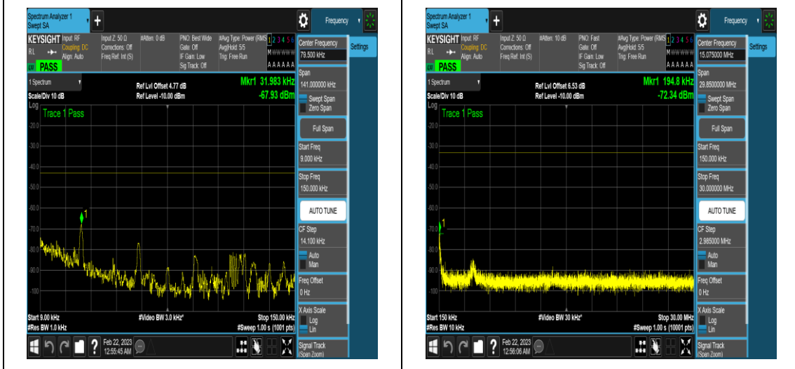
NTNV_N78-3450-3550_PC2_30_50_L_TID4_N/A_0.009_0.15_#1 NTNV_N78-3450-3550_PC2_30_50_L_TID4_N/A_0.15_30_#1
