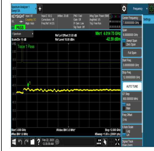
NTNV_N78-3450-3550_PC2_30_40_M_TID18_N/ A_30_1000_#1
