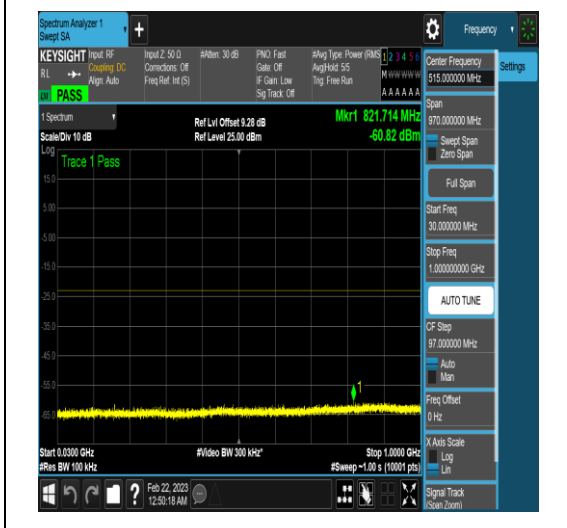
NTNV_N78-3450-3550_PC2_30_40_H_TID17_N/ A_30_1000_#1
