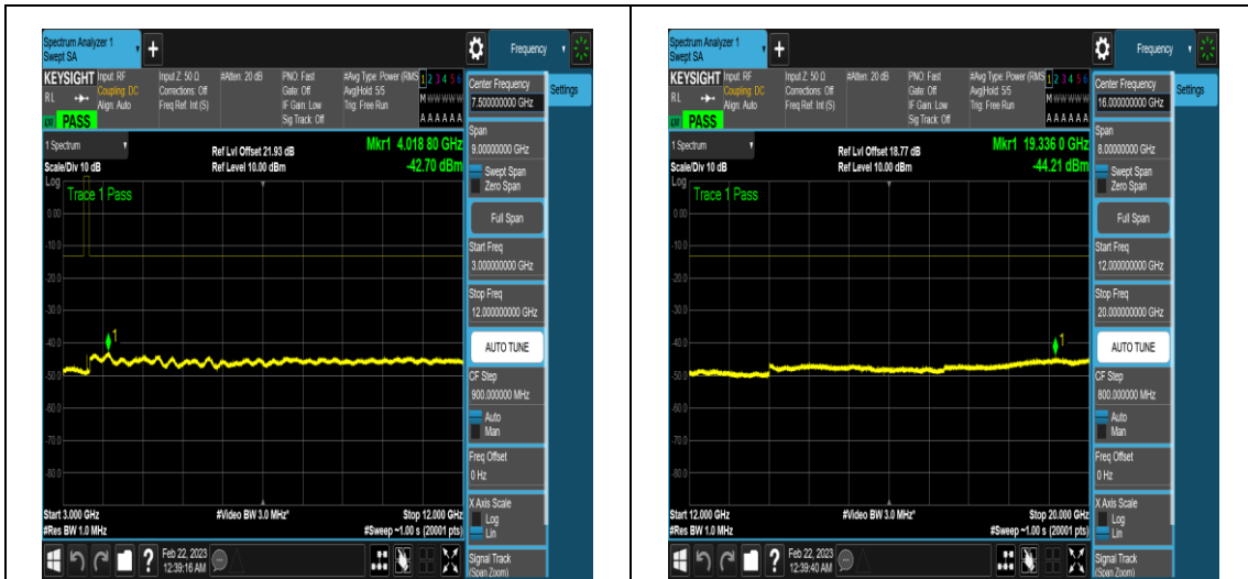
NTNV_N78-3450-3550_PC2_30_40_H_TID4_N/A _3000_12000_#1
