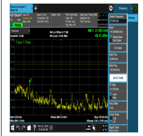
NTNV_N78-3450-3550_PC2_30_40_H_TID5_N/A _0.009_0.15_#1
