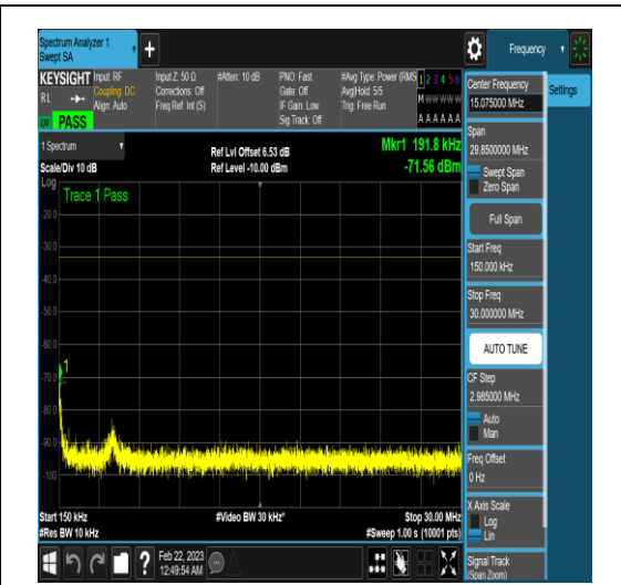
NTNV_N78-3450-3550_PC2_30_40_H_TID17_N/ A_0.15_30_#1
