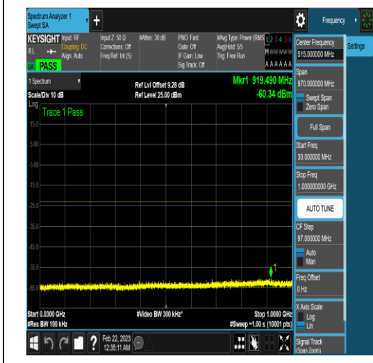
NTNV_N78-3450-3550_PC2_30_40_M_TID18_N/ A_30_1000_#1
