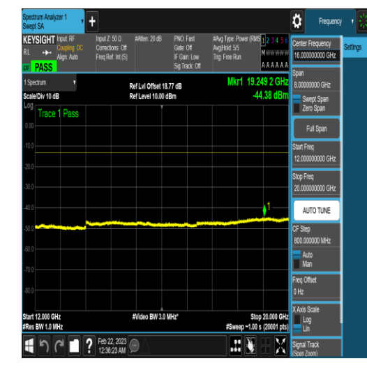
NTNV_N78-3450-3550_PC2_30_40_M_TID18_N/ A_1000_3000_#1
