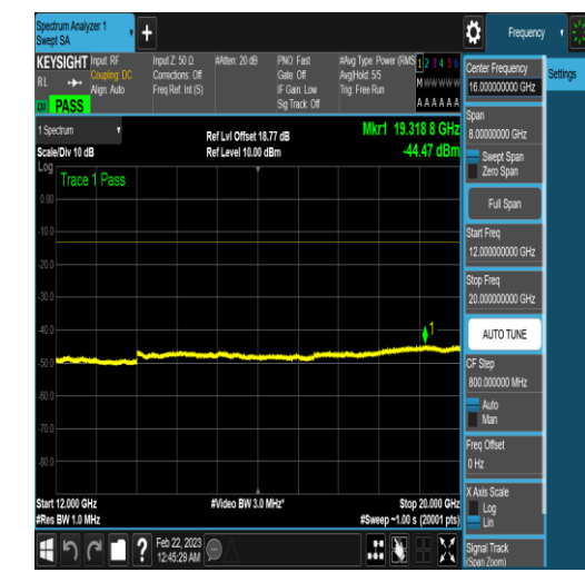
NTNV_N78-3450-3550_PC2_30_40_H_TID6_N/A _12000_20000_#1
