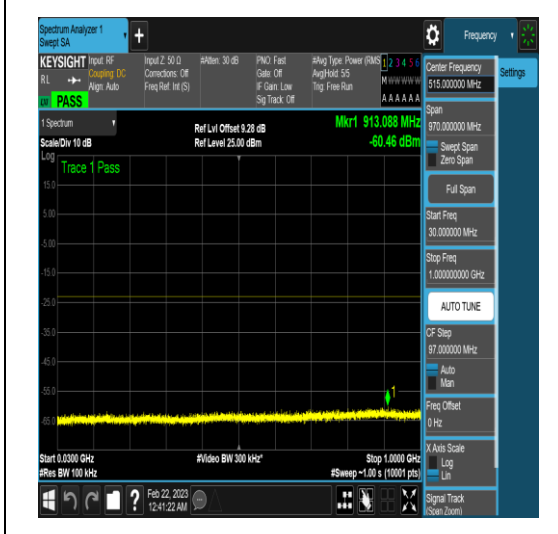
NTNV_N78-3450-3550_PC2_30_40_H_TID5_N/A _0.009_0.15_#1
