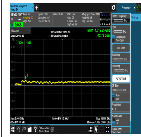
NTNV_N78-3450-3550_PC2_30_40_H_TID6_N/A _3000_12000_#1
