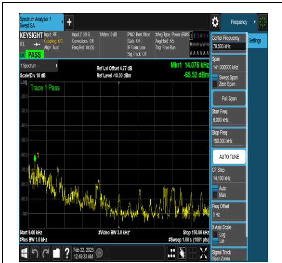
NTNV_N78-3450-3550_PC2_30_40_H_TID17_N/ A_0.009_0.15_#1
