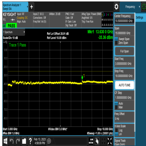
NTNV_N41_PC2_30_100_M_TID24_N/A_3000_1 8000_#1
