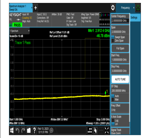
NTNV_N41_PC2_30_100_H_TID18_N/A_1000_3000_#1
