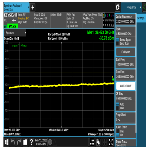
NTNV_N41_PC2_30_100_M_TID9_N/A_18000_2 6500_#1
