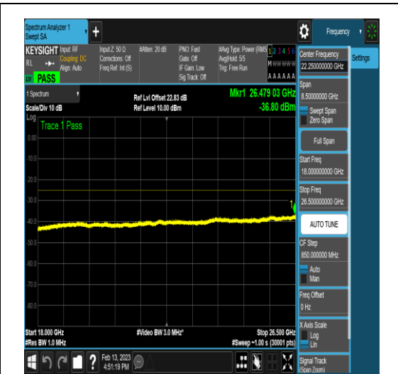
NTNV_N41_PC2_30_100_M_TID12_N/A_18000_1 26500_#1
