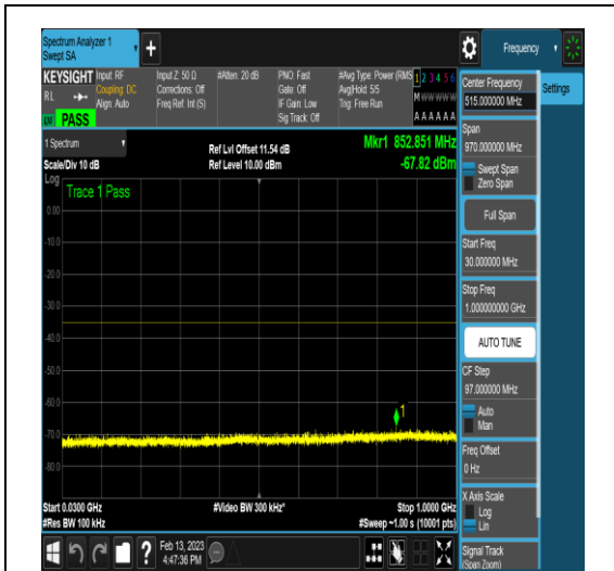
NTNV_N41_PC2_30_100_M_TID6_N/A_30_1000_#1
