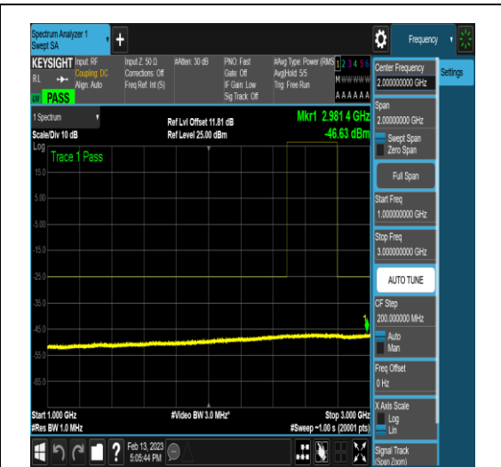
NTNV_N41_PC2_30_100_H_TID9_N/A_1000_3000_#1
