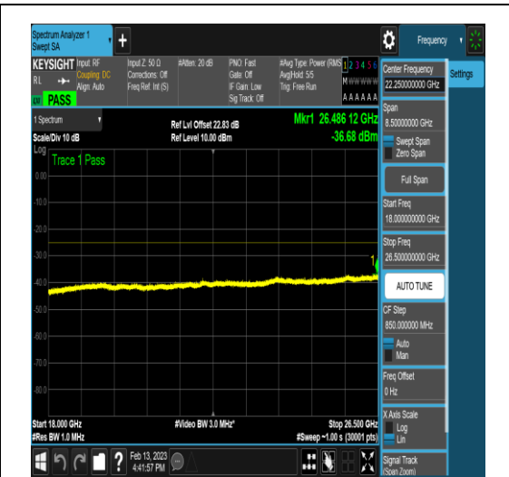
NTNV_N41_PC2_30_100_L_TID24_N/A_18000_1 26500_#1
