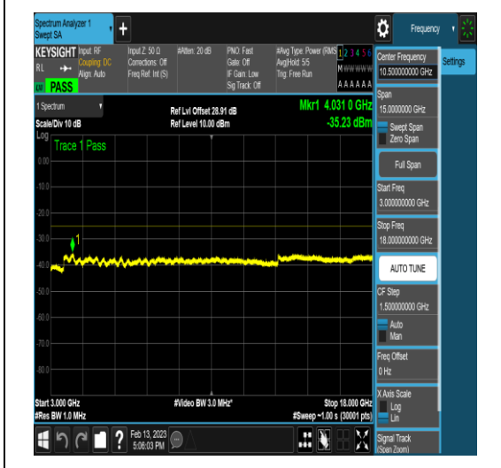
NTNV_N41_PC2_30_100_H_TID9_N/A_3000_18000_#1
