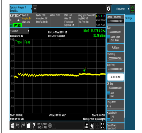
NTNV_N41_PC2_30_100_L_TID27_N/A_30_100_0_#1
