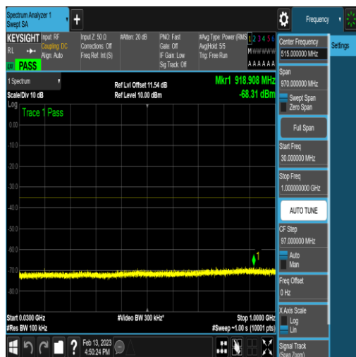
NTNV_N41_PC2_30_100_M_TID12_N/A_30_100 0_#1
