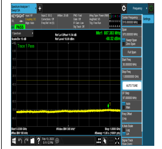
NTNV_N41_PC2_30_100_H_TID18_N/A_30_100_0_#1
