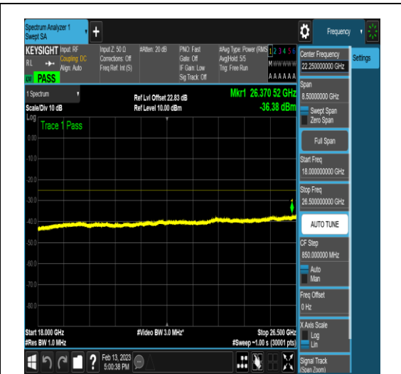
NTNV_N41_PC2_30_100_M_TID27_N/A_18000_26500_#1
