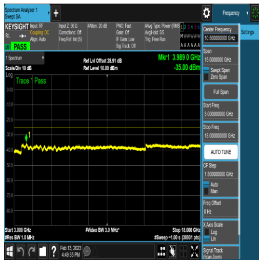
NTNV_N41_PC2_30_100_M_TID9_N/A_3000_18 000_#1
