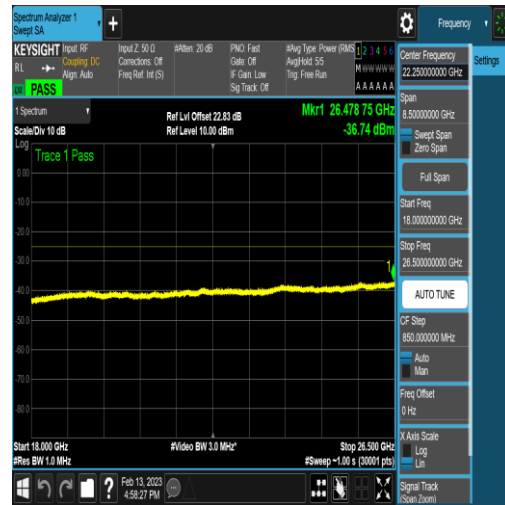
NTNV_N41_PC2_30_100_M_TID24_N/A_18000_26500_#1
