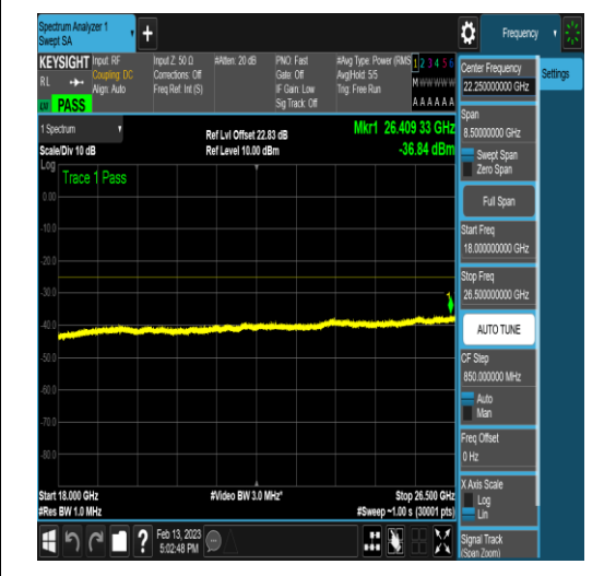
NTNV_N41_PC2_30_100_H_TID3_N/A_1000_3000_#1
