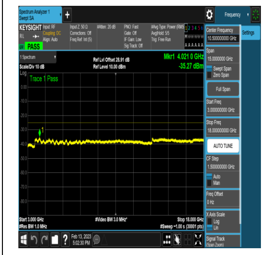
NTNV_N41_PC2_30_100_H_TID3_N/A_30_1000_#1
