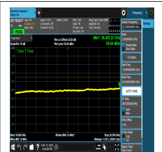
NTNV_N41_PC2_30_100_H_TID15_N/A_18000_26500_#1
