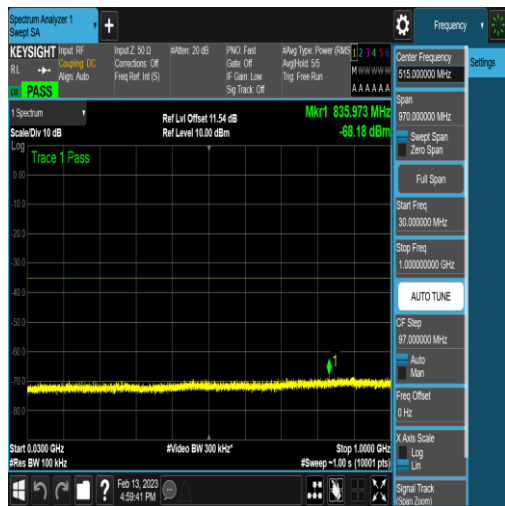
NTNV_N41_PC2_30_100_M_TID27_N/A_30_100 0_#1
