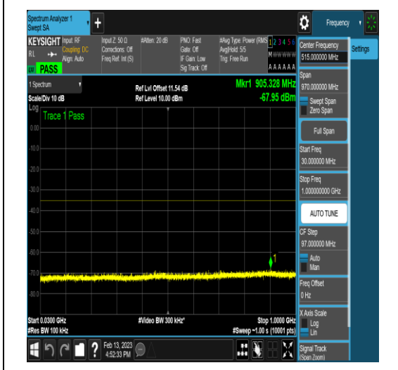
NTNV_N41_PC2_30_100_M_TID15_N/A_30_100_0_#1
