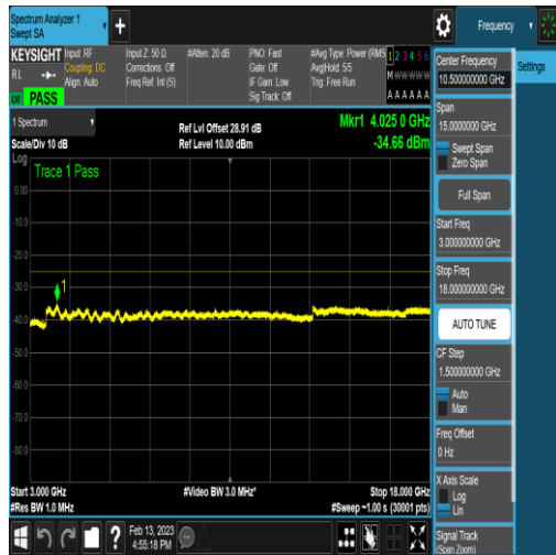
NTNV_N41_PC2_30_100_M_TID18_N/A_3000_18000_#1
