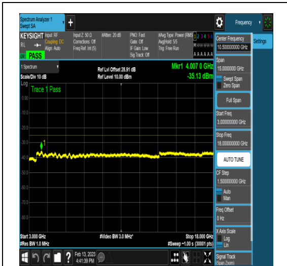
NTNV_N41_PC2_30_100_L_TID24_N/A_3000_1 8000_#1
