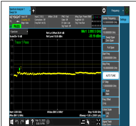
NTNV_N41_PC2_30_100_M_TID27_N/A_3000_1 8000_#1
