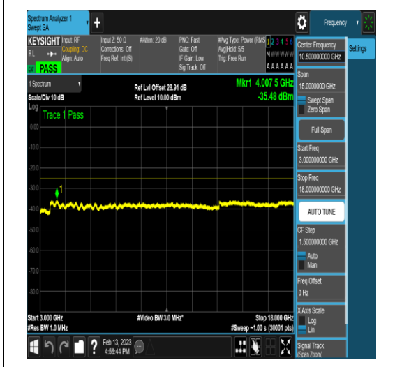
NTNV_N41_PC2_30_100_M_TID21_N/A_3000_1 8000_#1
