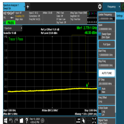
NTNV_N41_PC2_30_100_M_TID12_N/A_1000_3 000_#1
