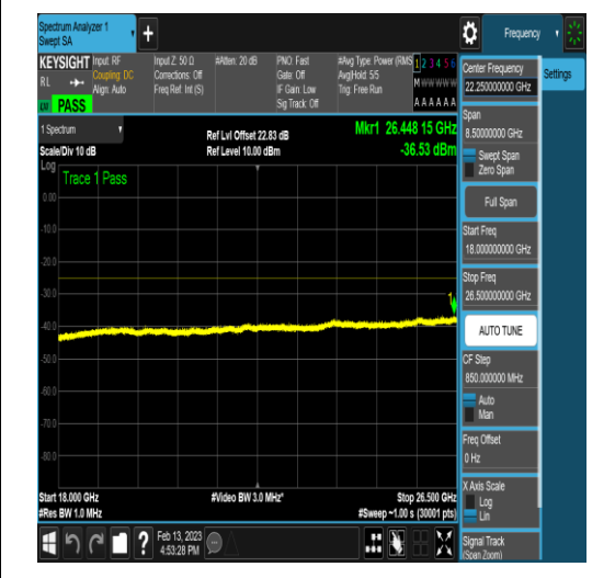
NTNV_N41_PC2_30_100_M_TID15_N/A_1000_3_000_#1
