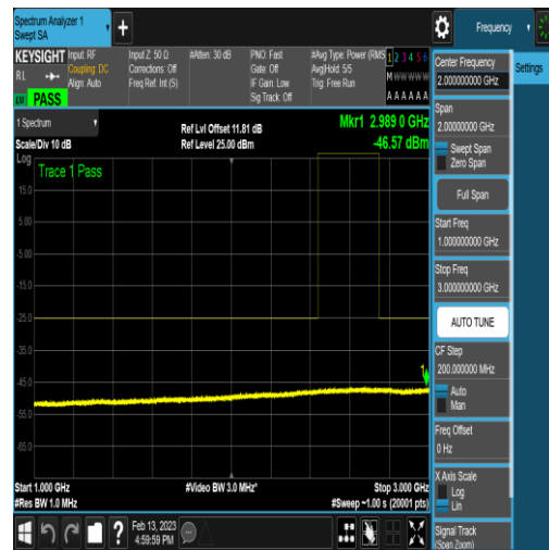
NTNV_N41_PC2_30_100_M_TID27_N/A_1000_3 000_#1
