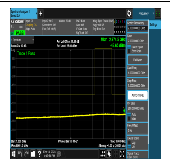
NTNV_N41_PC2_30_100_M_TID6_N/A_1000_3000_#1
