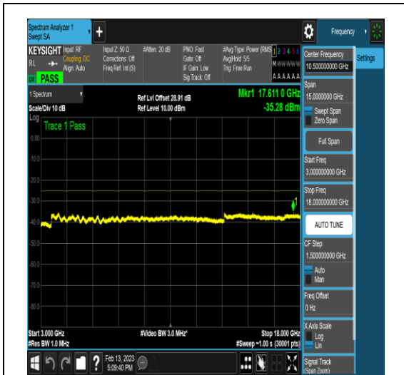
NTNV_N41_PC2_30_100_H_TID15_N/A_3000_1 8000_#1
