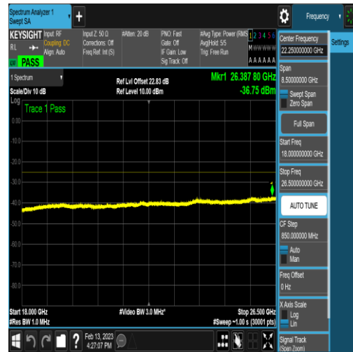
NTNV_N41_PC2_30_60_H_TID27_N/A_18000_2 6500_#1
