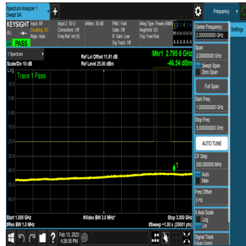
NTNV_N41_PC2_30_60_H_TID27_N/A_1000_30 00_#1
