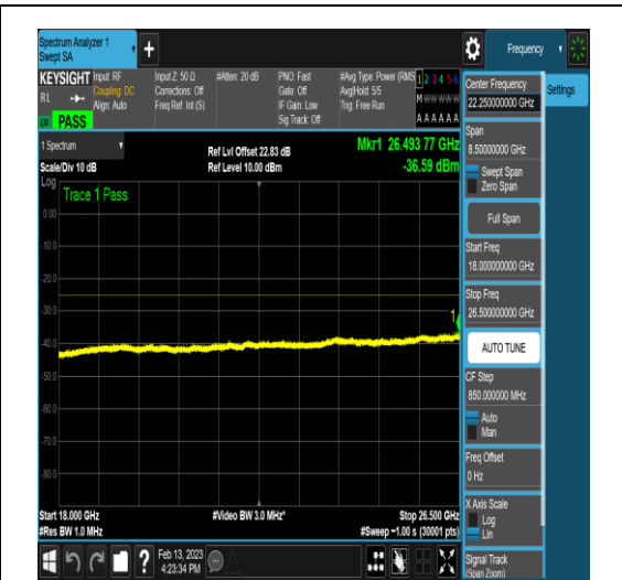
NTNV_N41_PC2_30_60_H_TID21_N/A_18000_26500_#1
