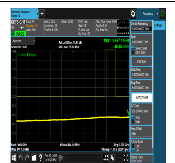
NTNV_N41_PC2_30_60_H_TID15_N/A_1000_3000_#1
