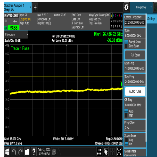
NTNV_N41_PC2_30_60_H_TID18_N/A_18000_2 6500_#1
