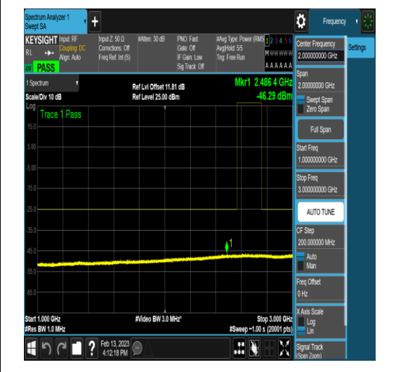
NTNV_N41_PC2_30_60_M_TID27_N/A_1000_3000_#1
