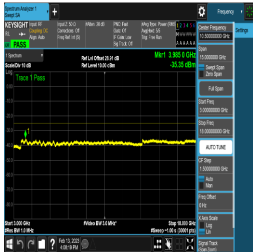
NTNV_N41_PC2_30_60_M_TID24_N/A_3000_18 000_#1
