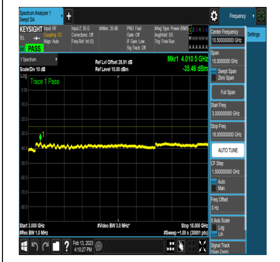
NTNV_N41_PC2_30_60_M_TID27_N/A_3000_18000_#1
