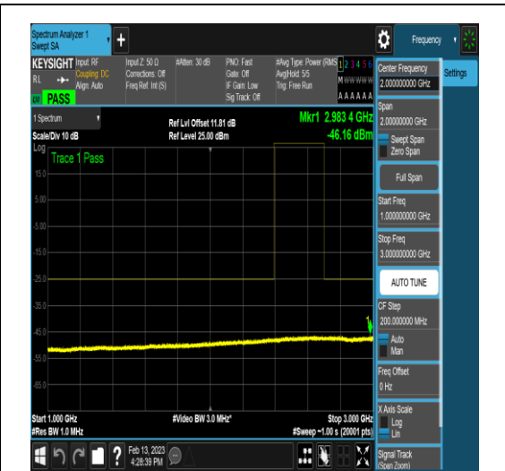
NTNV_N41_PC2_30_100_L_TID3_N/A_1000_3000_#1
