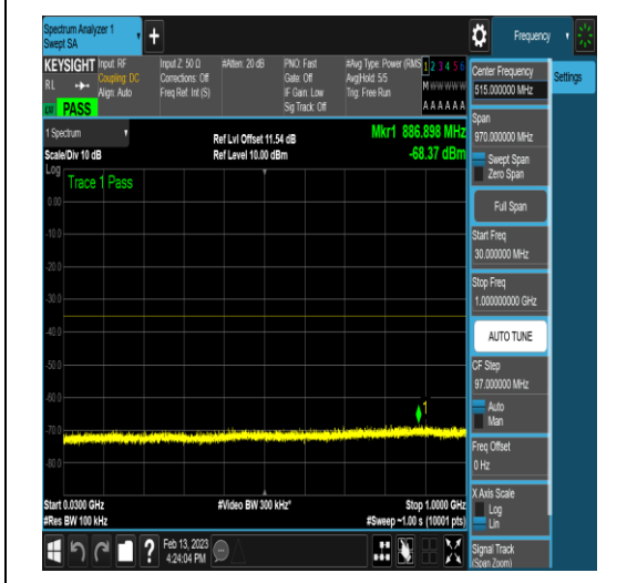
NTNV_N41_PC2_30_60_H_TID24_N/A_30_1000_#1
