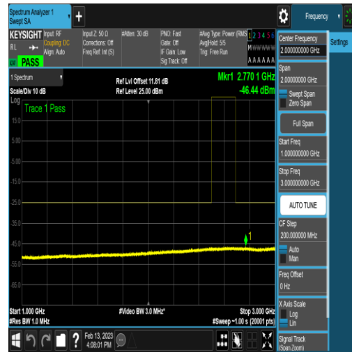
NTNV_N41_PC2_30_60_M_TID24_N/A_1000_30 00_#1
