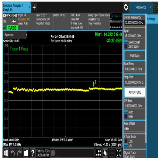
NTNV_N41_PC2_30_60_H_TID27_N/A_3000_18 000_#1
