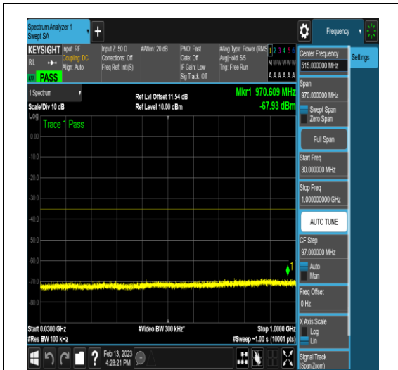
NTNV_N41_PC2_30_100_L_TID3_N/A_30_1000_#1
