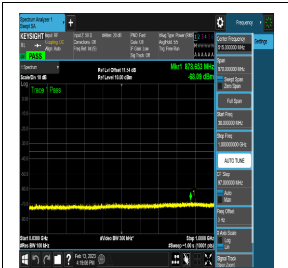
NTNV_N41_PC2_30_60_H_TID15_N/A_30_1000_#1
