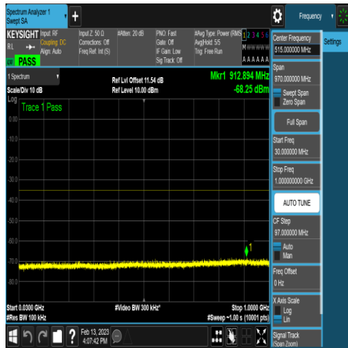
NTNV_N41_PC2_30_60_M_TID24_N/A_30_1000 _#1
