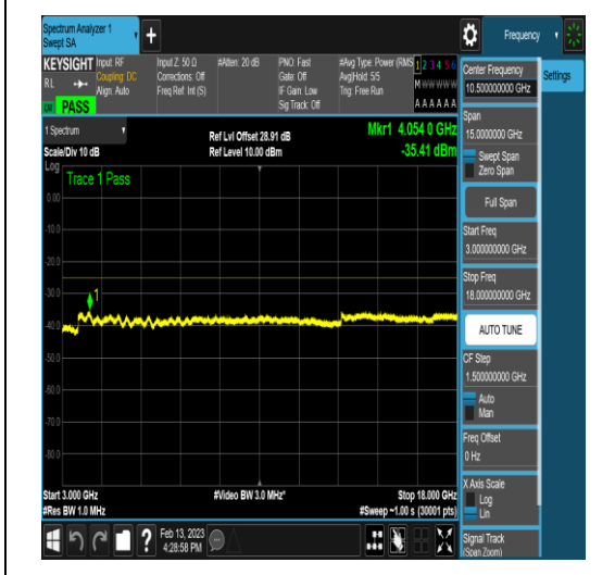
NTNV_N41_PC2_30_100_L_TID3_N/A_3000_18000_#1
