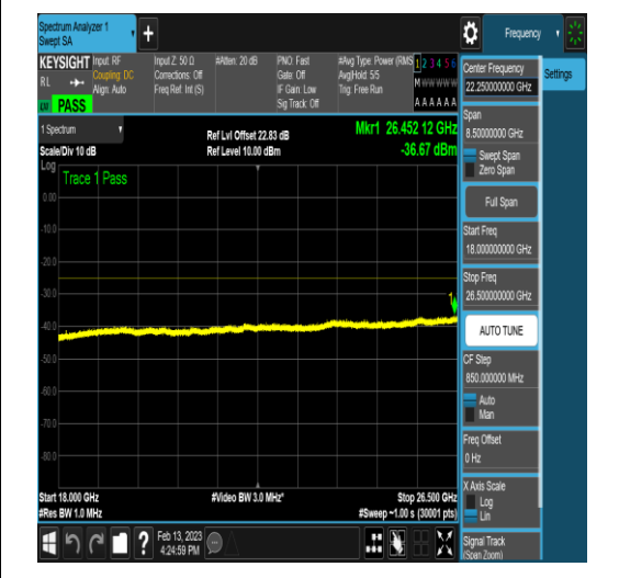
NTNV_N41_PC2_30_60_H_TID24_N/A_1000_3000_#1
