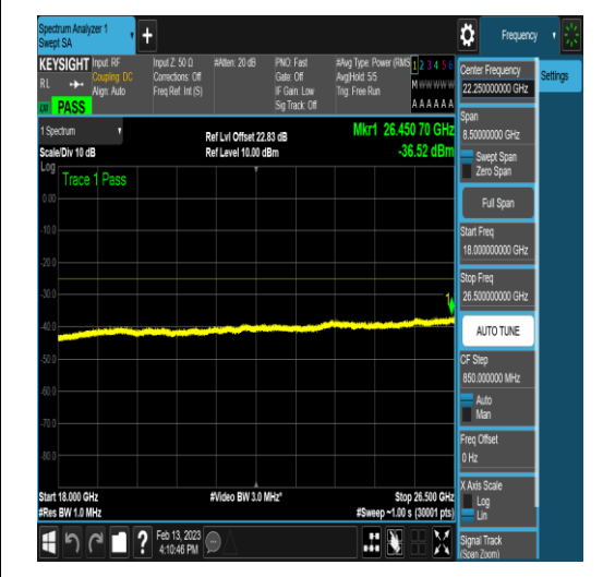
NTNV_N41_PC2_30_60_M_TID27_N/A_18000_26500_#1
