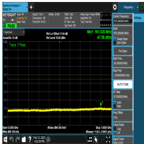
NTNV_N41_PC2_30_60_H_TID21_N/A_30_1000 _#1
