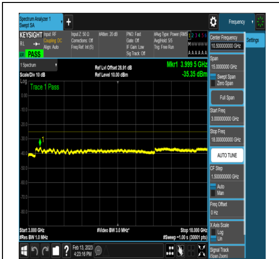
NTNV_N41_PC2_30_60_H_TID21_N/A_3000_18000_#1
