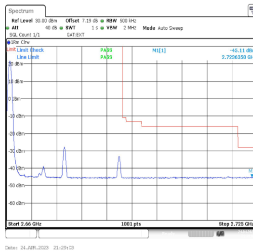
41-41_41-41_15MHz-15MHz_64QAM@64QAM-64QAM@64QAM_39725-39875_75RB#0@75RB#0-75RB#0@75RB#0
