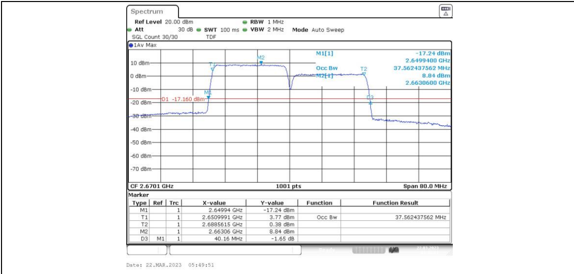
41-41-20MHz-20MHz-16QAM-16QAM-39750-39948-100RB#0-100RB#0
