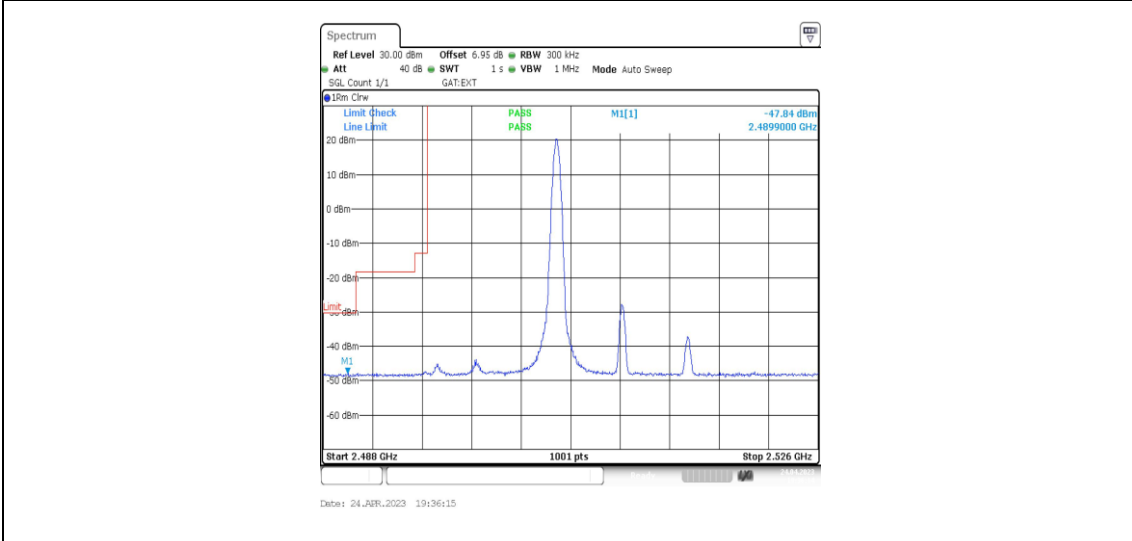
41-41_41-41_10MHz-20MHz_16QAM@16QAM-16QAM@16QAM_39705-39849_1RB#49@50RB#0-0 RB#0@100RB#0
