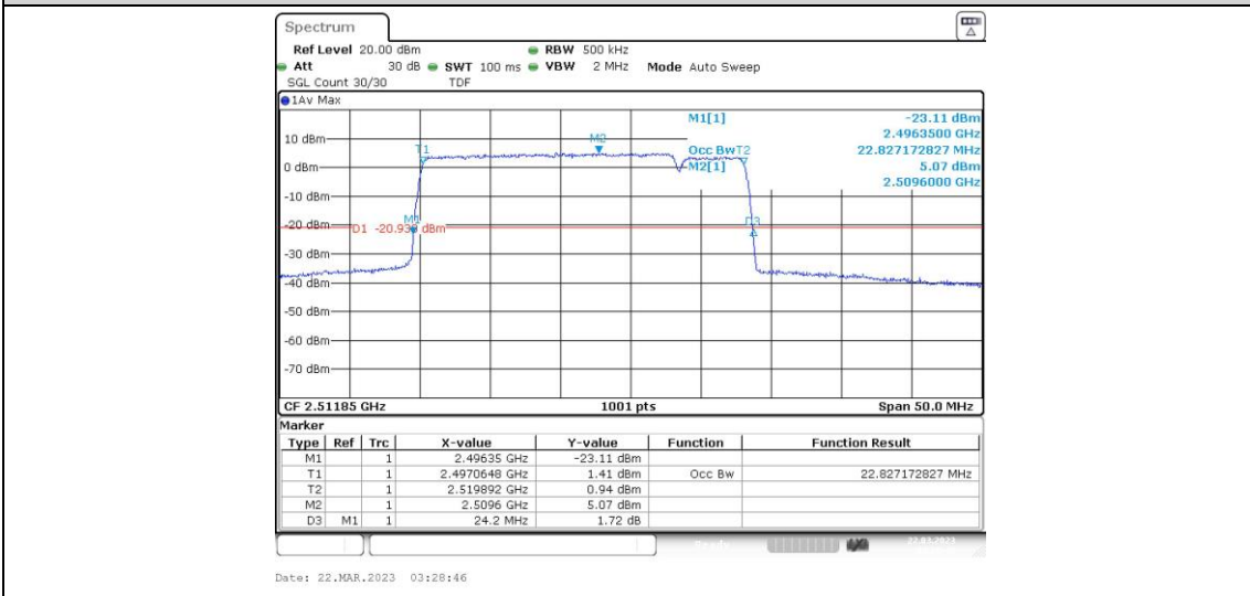
41-41-20MHz-5MHz-64QAM-64QAM-40595-40712-100RB#0-25RB#0
