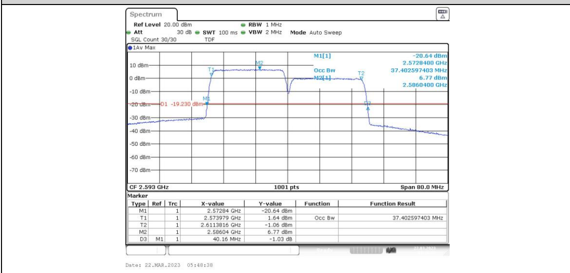
41-41-20MHz-20MHz-16QAM-16QAM-41292-41490-100RB#0-100RB#0
