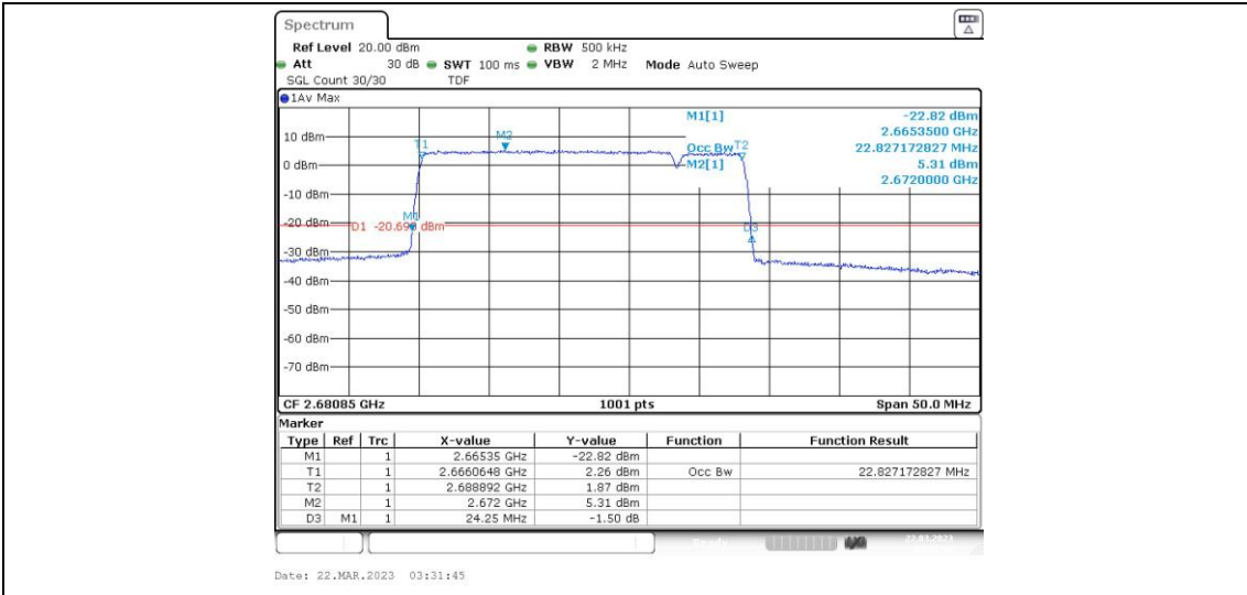
41-41-20MHz-5MHz-64QAM-64QAM-39750-39867-100RB#0-25RB#0
