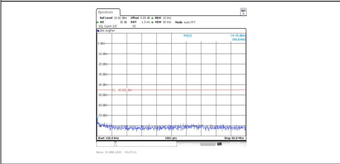
38-38-20MHz-20MHz-64QAM-64QAM-37901-38099-1RB#0-0RB#0-0.15~30MHz
