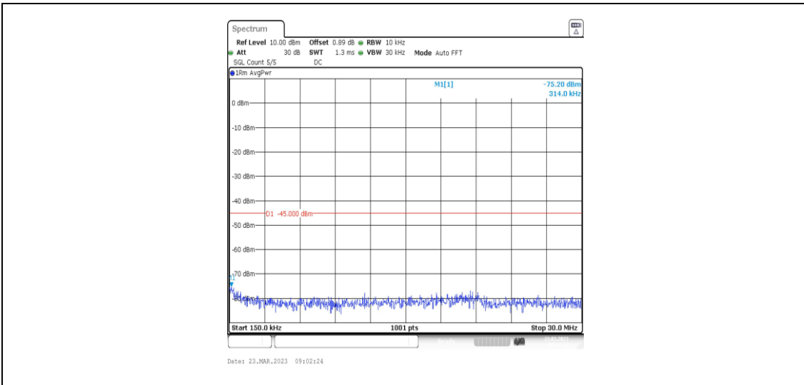
38-38-20MHz-20MHz-16QAM-16QAM-37952-38150-1RB#0-ORB#0-0.15~30MHz
