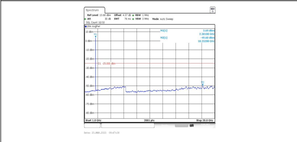
38-38-20MHz-20MHz-64QAM-64QAM-37901-38099-1RB#0-ORB#0-1000~20000MHz
