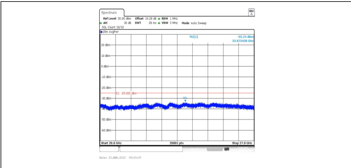
38-38-20MHz-20MHz-16QAM-16QAM-37952-38150-1RB#0-0RB#0-20000~27000MHz
