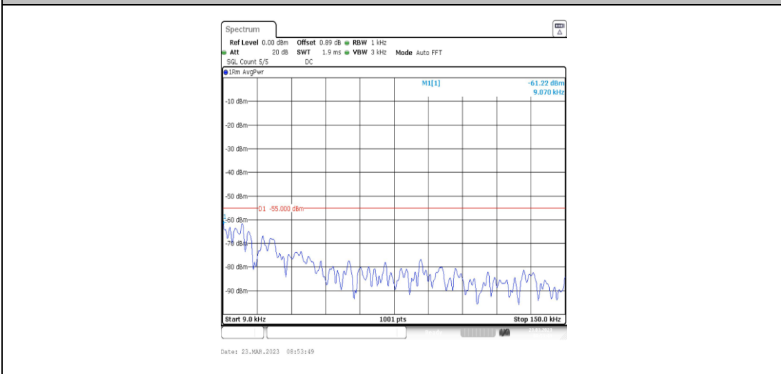
38-38-20MHz-20MHz-16QAM-16QAM-37901-38099-1RB#0-1RB#99-0.009~0.15MHz
