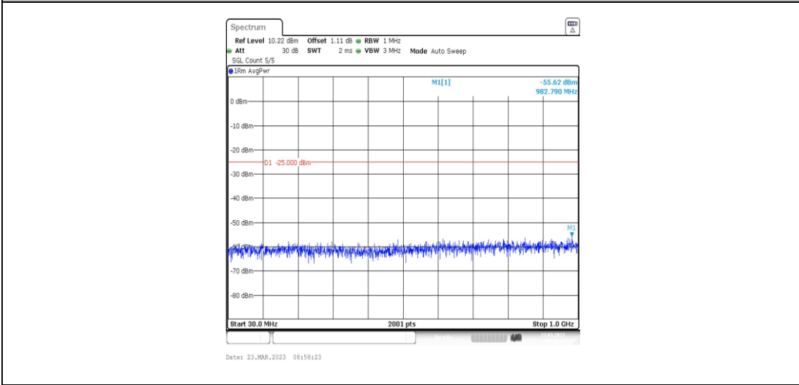
38-38-20MHz-20MHz-16QAM-16QAM-37901-38099-100RB#0-100RB#0-30~1000MHz
