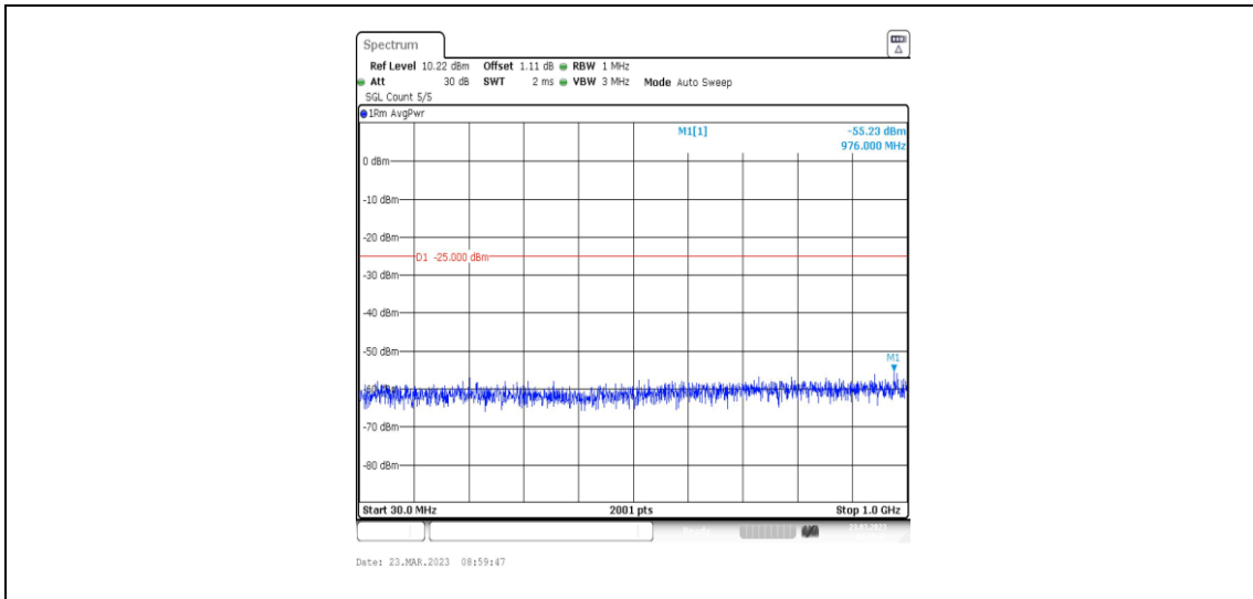
38-38-20MHz-20MHz-64QAM-64QAM-37901-38099-100RB#0-100RB#0-30~1000MHz
