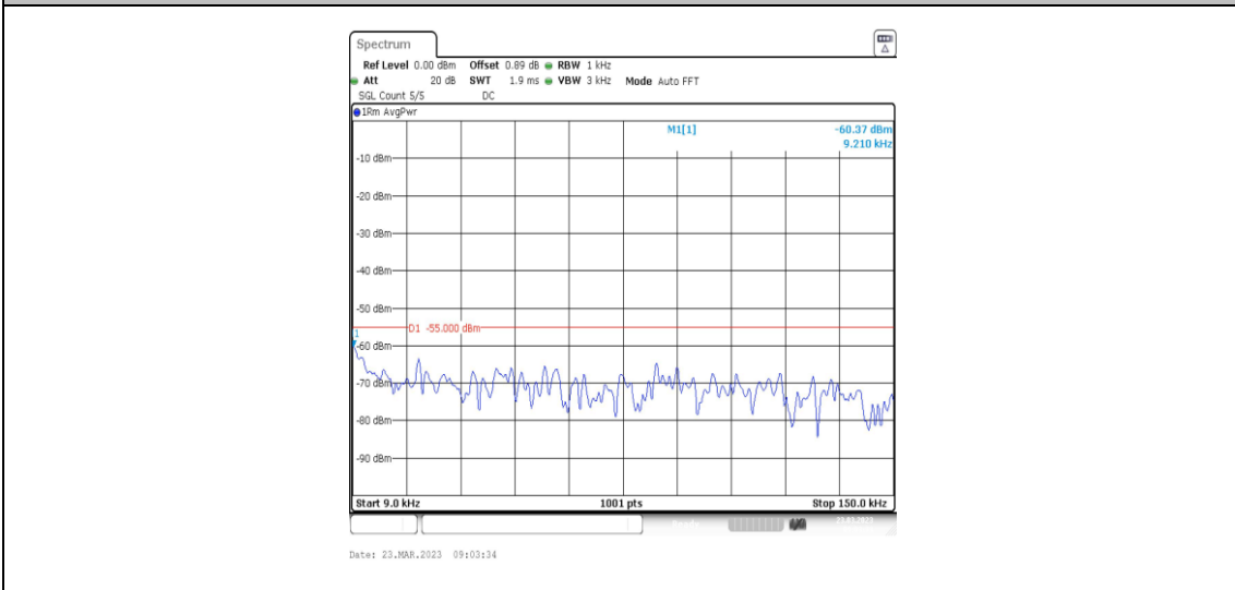
38-38-20MHz-20MHz-64QAM-64QAM-37952-38150-1RB#0-0RB#0-0.009~0.15MHz
