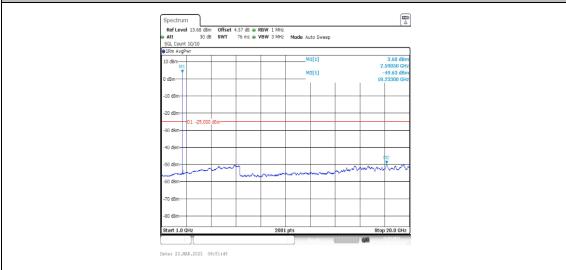
38-38-20MHz-20MHz-64QAM-64QAM-37901-38099-1RB#99-0RB#0-1000~20000MHz
