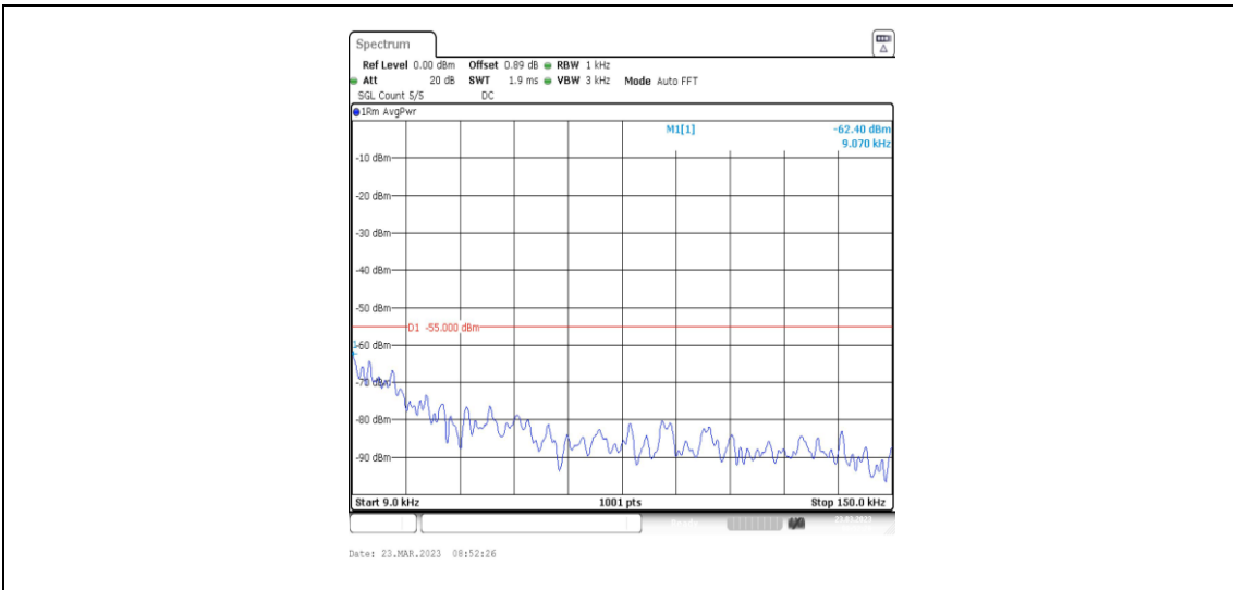
38-38-20MHz-20MHz-QPSK-QPSK-37901-38099-1RB#0-1RB#99-0.009~0.15MHz
