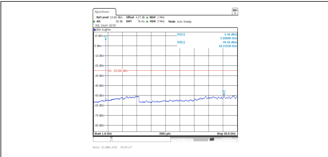
38-38-20MHz-20MHz-QPSK-QPSK-37952-38150-1RB#99-ORB#0-1000~20000MHz
