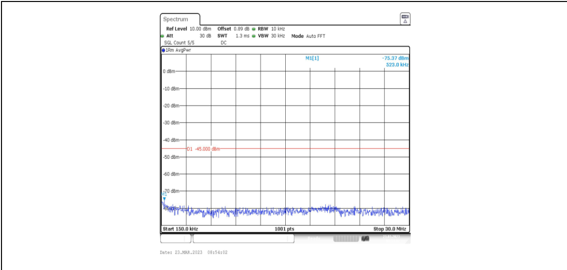
38-38-20MHz-20MHz-16QAM-16QAM-37901-38099-1RB#0-1RB#99-0.15~30MHz
