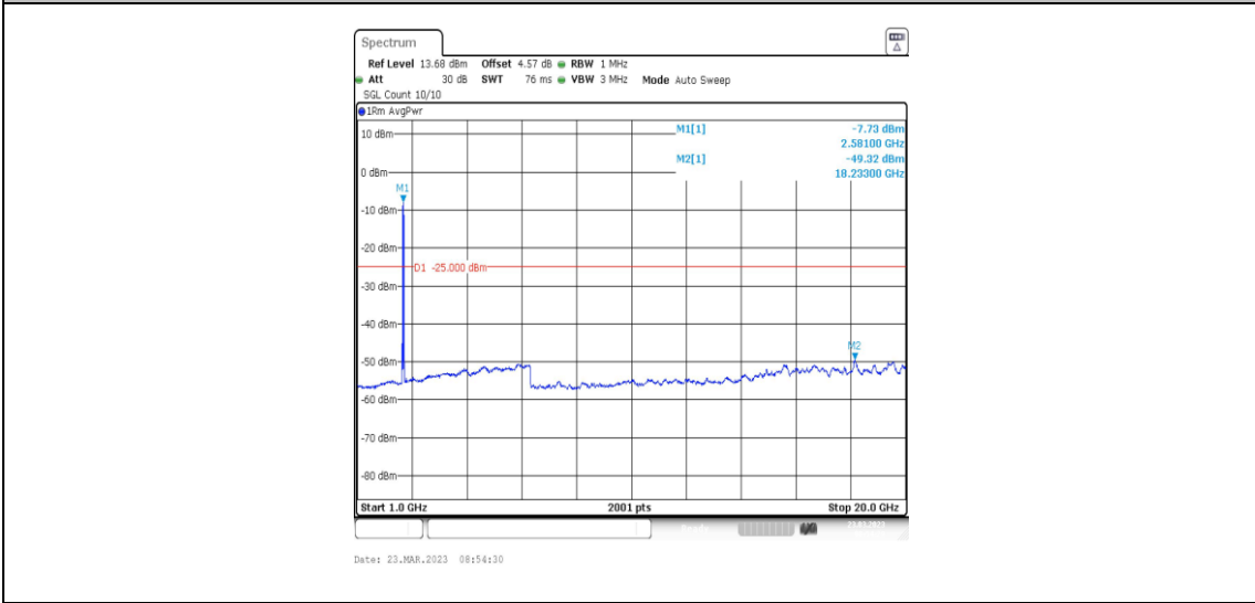
38-38-20MHz-20MHz-16QAM-16QAM-37901-38099-1RB#0-1RB#99-1000~20000MHz
