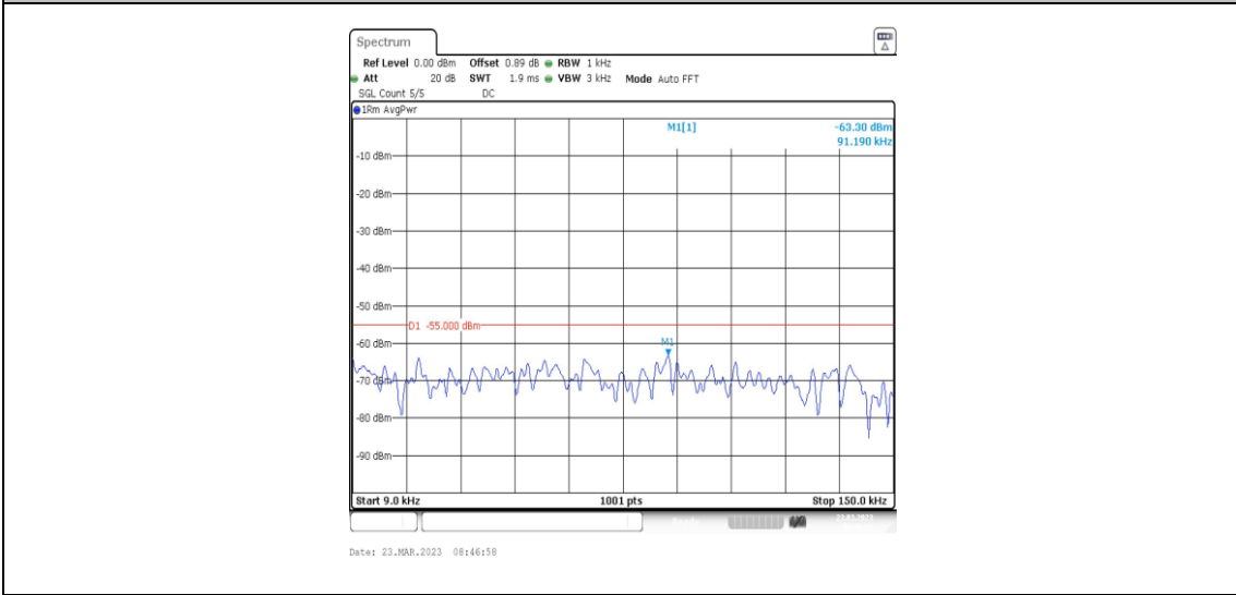
38-38-20MHz-20MHz-64QAM-64QAM-37901-38099-1RB#0-0RB#0-0.009~0.15MHz
