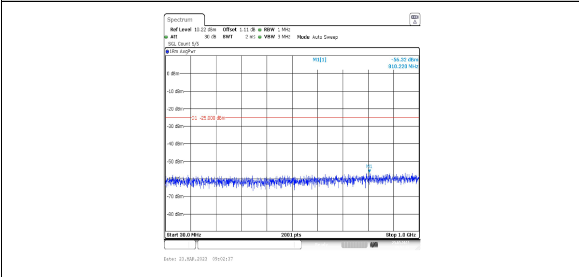
38-38-20MHz-20MHz-16QAM-16QAM-37952-38150-1RB#0-ORB#0-30~1000MHz
