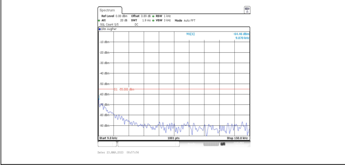
38-38-20MHz-20MHz-16QAM-16QAM-37901-38099-100RB#0-100RB#0-0.009~0.15MHz
