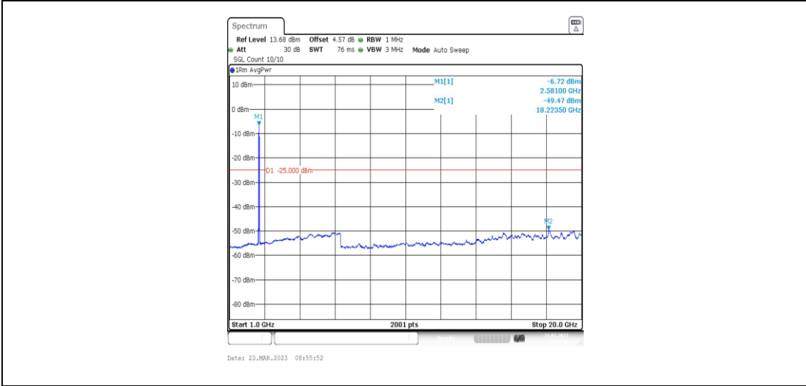
38-38-20MHz-20MHz-64QAM-64QAM-37901-38099-1RB#0-1RB#99-1000~20000MHz
