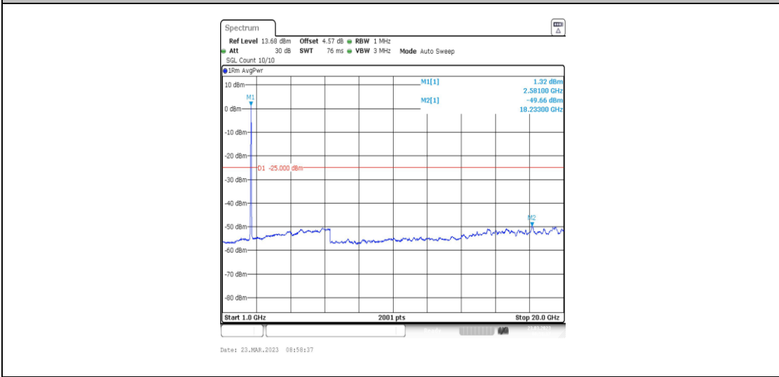
38-38-20MHz-20MHz-16QAM-16QAM-37901-38099-100RB#0-100RB#0-1000~20000MHz
