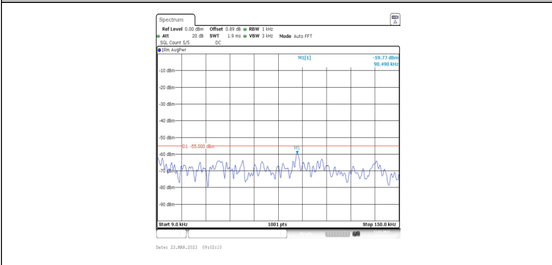
38-38-20MHz-20MHz-16QAM-16QAM-37952-38150-1RB#0-0RB#0-0.009~0.15MHz
