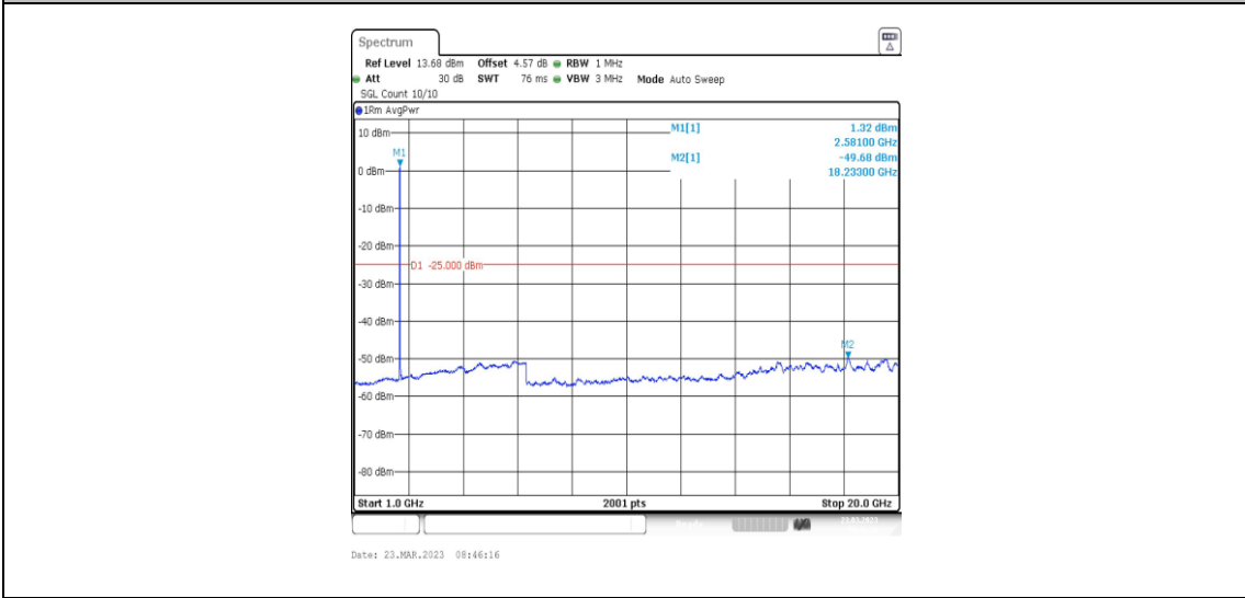
38-38-20MHz-20MHz-16QAM-16QAM-37901-38099-1RB#0-ORB#0-1000~20000MHz
