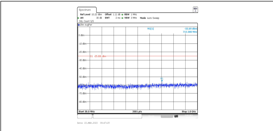
38-38-20MHz-20MHz-64QAM-64QAM-37901-38099-1RB#0-ORB#0-30~1000MHz
