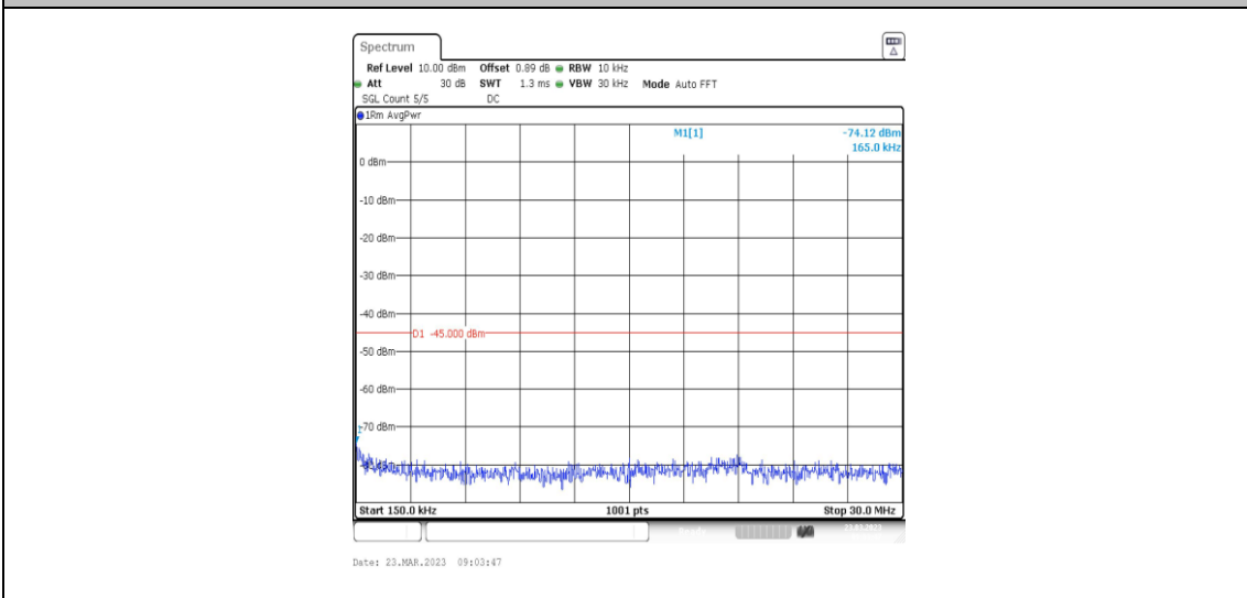
38-38-20MHz-20MHz-64QAM-64QAM-37952-38150-1RB#0-0RB#0-0.15~30MHz
