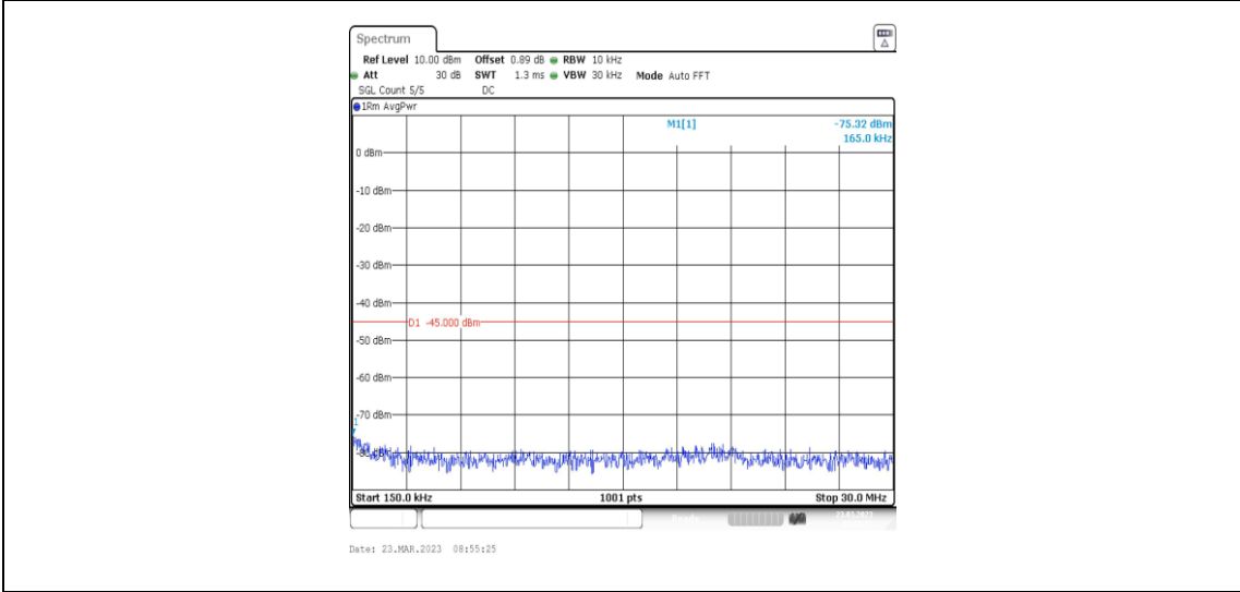
38-38-20MHz-20MHz-64QAM-64QAM-37901-38099-1RB#0-1RB#99-0.15~30MHz
