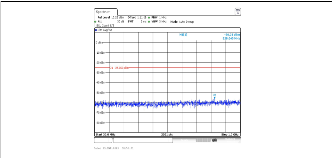
38-38-20MHz-20MHz-64QAM-64QAM-37901-38099-1RB#99-0RB#0-30~1000MHz
