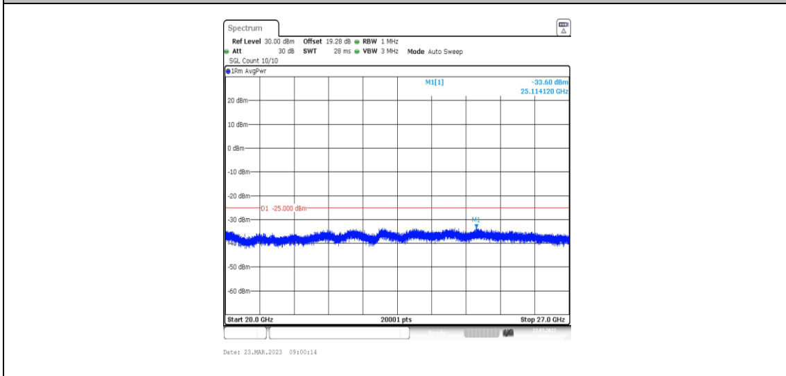
38-38-20MHz-20MHz-64QAM-64QAM-37901-38099-100RB#0-100RB#0-20000~27000MHz
