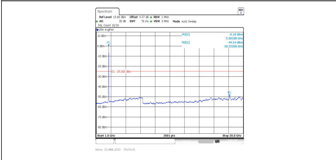
38-38-20MHz-20MHz-64QAM-64QAM-37901-38099-100RB#0-100RB#0-1000~20000MHz
