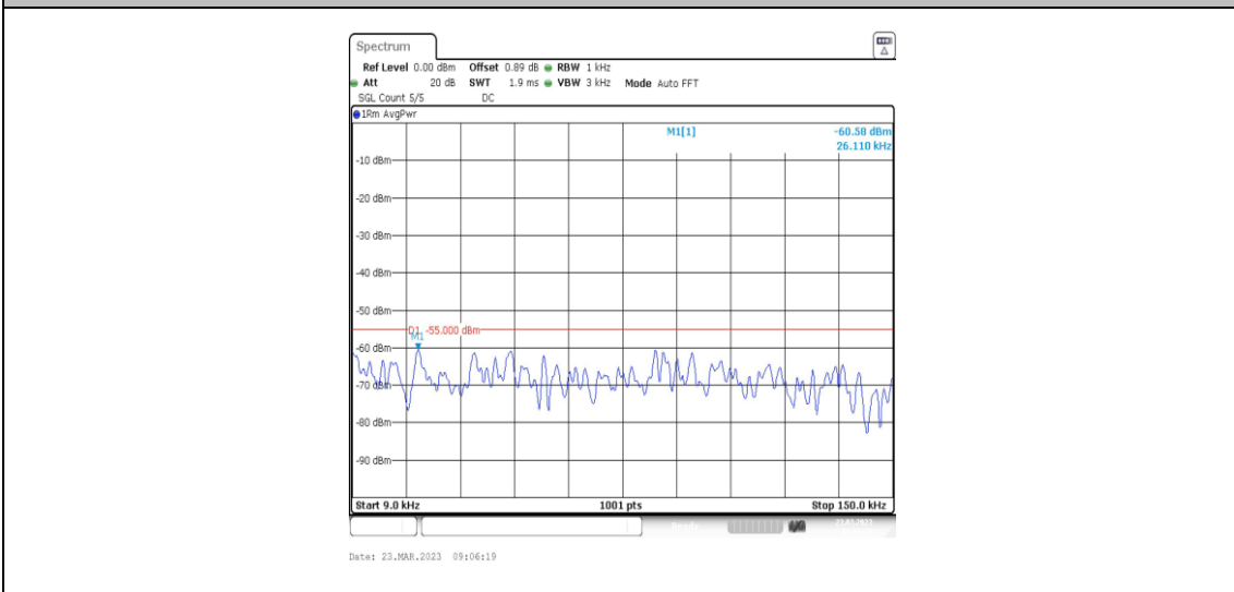
38-38-20MHz-20MHz-16QAM-16QAM-37952-38150-1RB#99-ORB#0-0.009~0.15MHz
