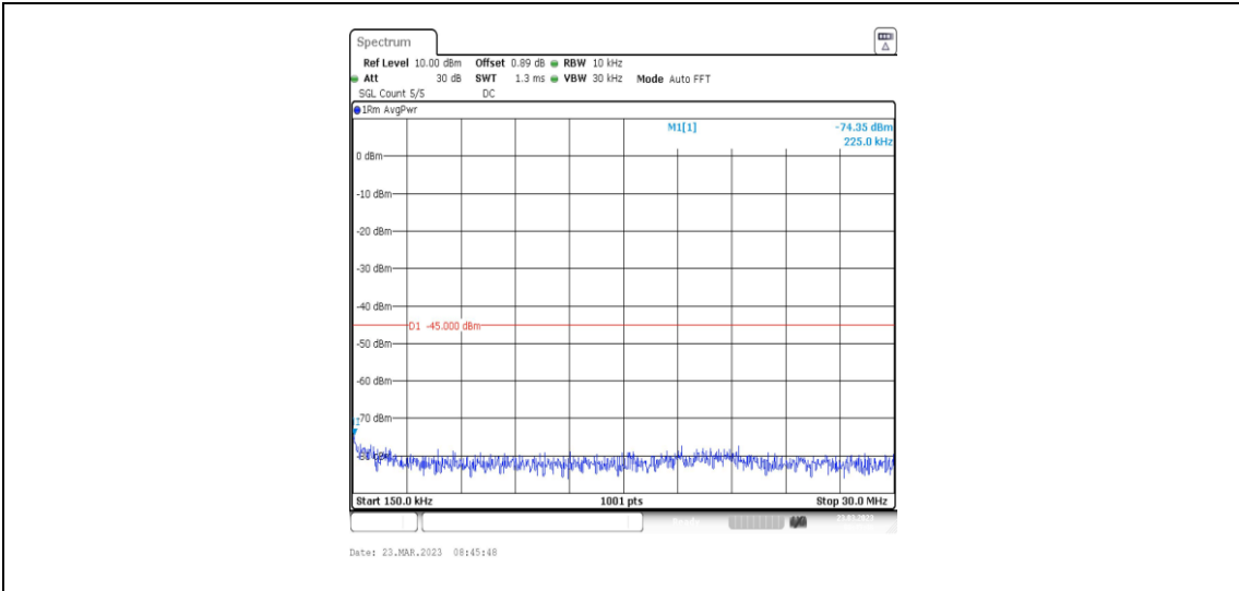
38-38-20MHz-20MHz-16QAM-16QAM-37901-38099-1RB#0-ORB#0-0.15~30MHz
