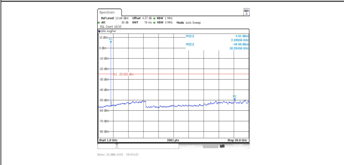
38-38-20MHz-20MHz-16QAM-16QAM-37901-38099-1RB#99-0RB#0-1000~20000MHz
