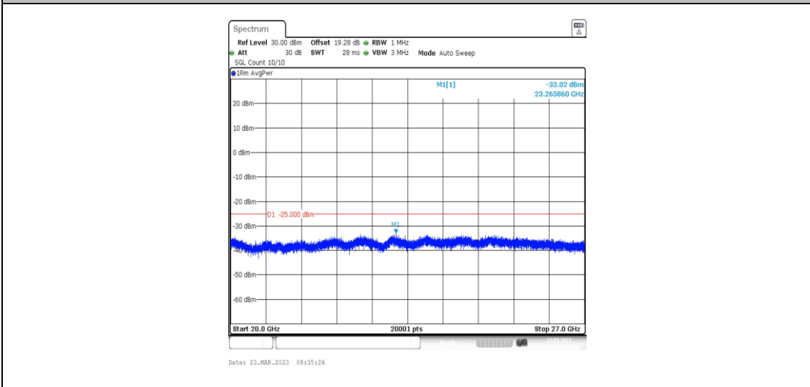
38-38-20MHz-20MHz-64QAM-64QAM-37850-38048-1RB#99-0RB#0-20000~27000MHz
