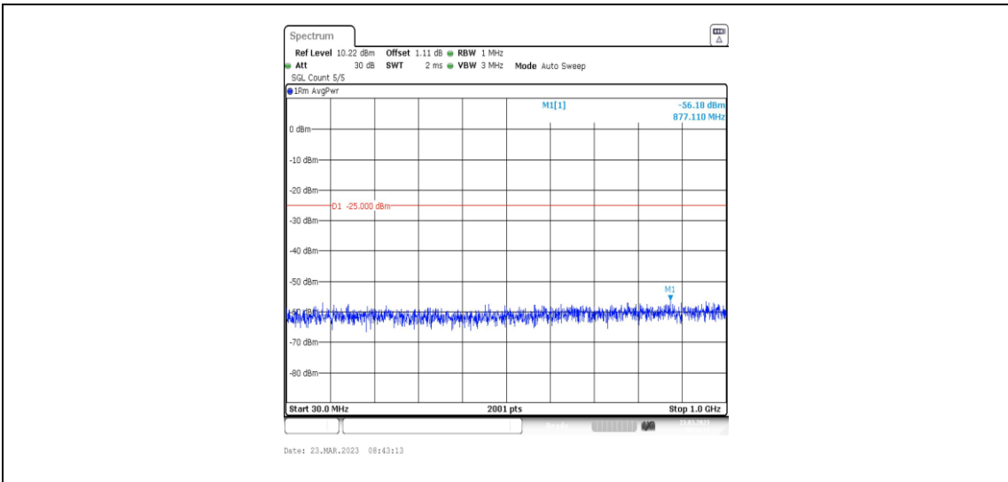
38-38-20MHz-20MHz-64QAM-64QAM-37850-38048-100RB#0-100RB#0-30~1000MHz
