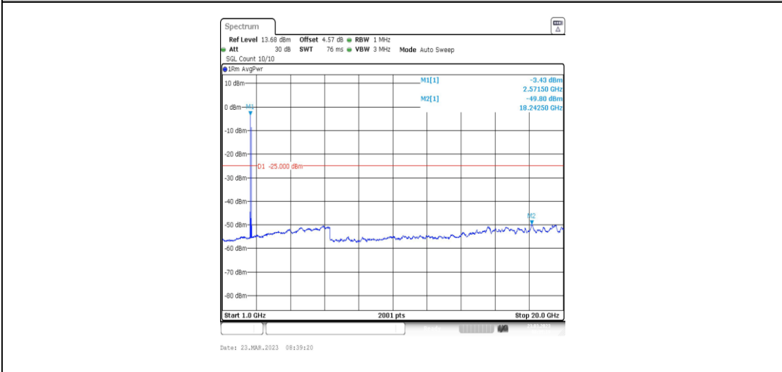
38-38-20MHz-20MHz-64QAM-64QAM-37850-38048-1RB#0-1RB#99-1000~20000MHz
