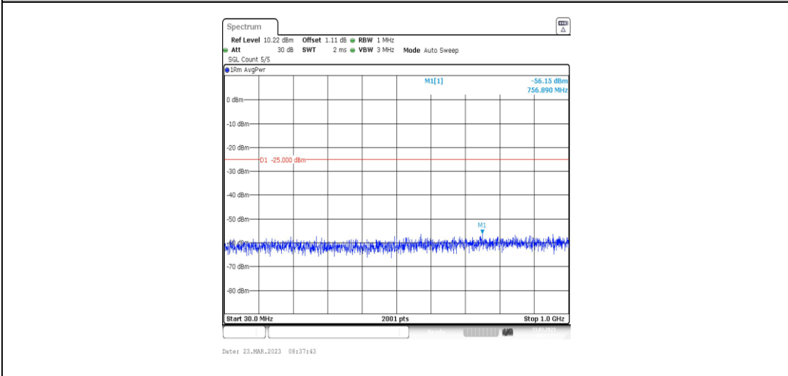
38-38-20MHz-20MHz-16QAM-16QAM-37850-38048-1RB#0-1RB#99-30~1000MHz
