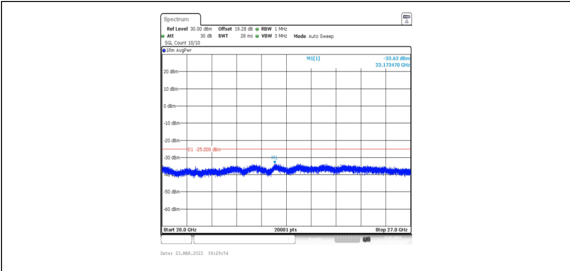
38-38-20MHz-20MHz-16QAM-16QAM-37850-38048-1RB#0-0RB#0-20000~27000MHz
