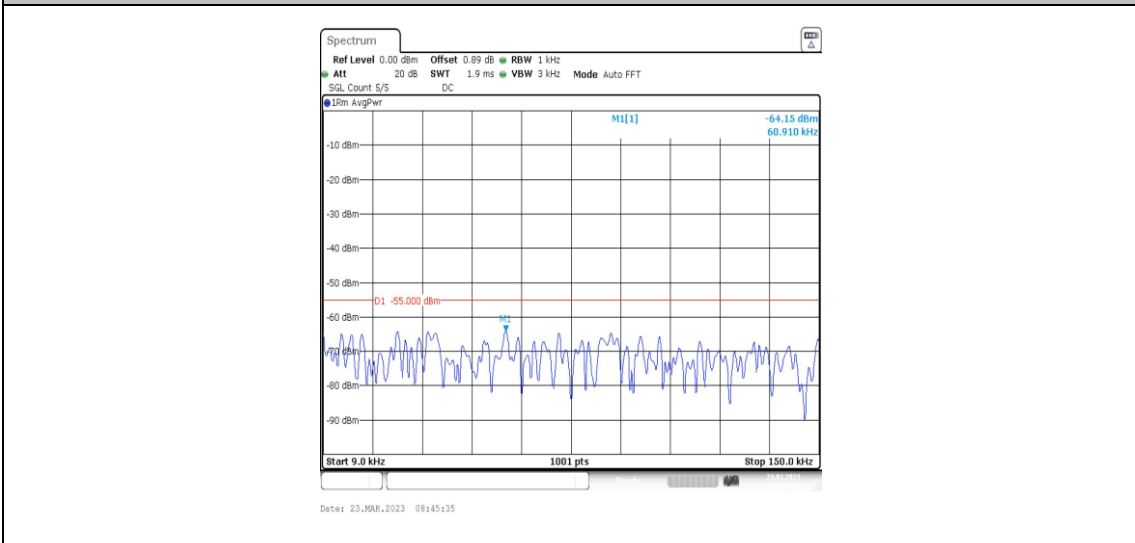
38-38-20MHz-20MHz-16QAM-16QAM-37901-38099-1RB#0-0RB#0-0.009~0.15MHz
