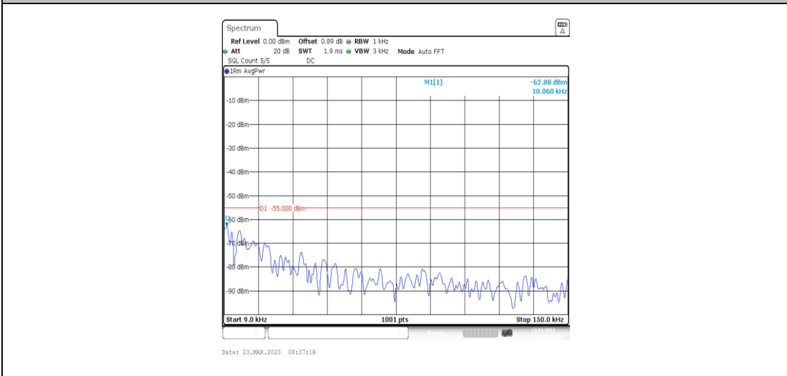
38-38-20MHz-20MHz-16QAM-16QAM-37850-38048-1RB#0-1RB#99-0.009~0.15MHz
