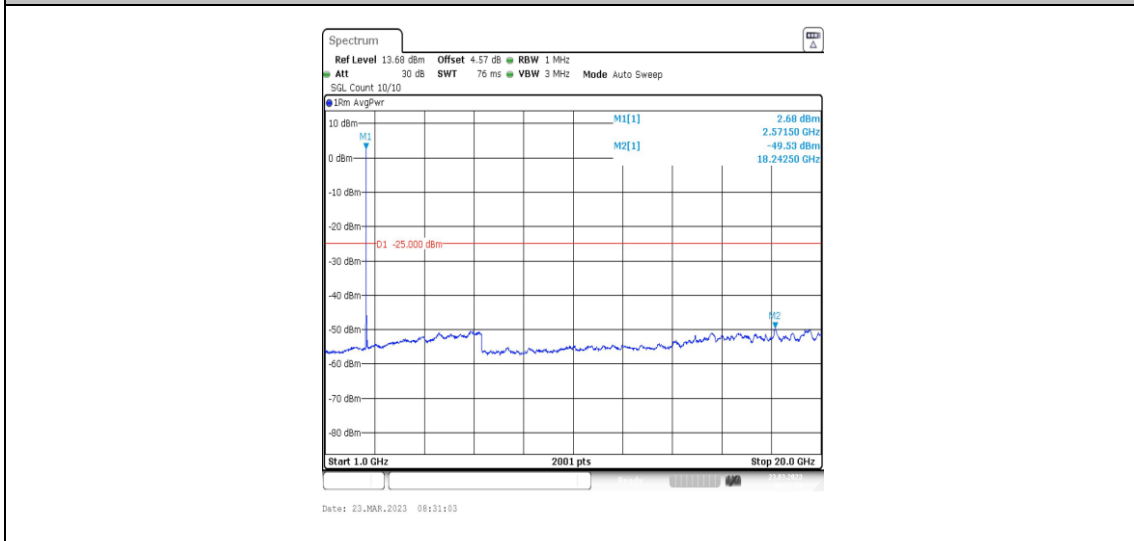
38-38-20MHz-20MHz-64QAM-64QAM-37850-38048-1RB#0-ORB#0-1000~20000MHz
