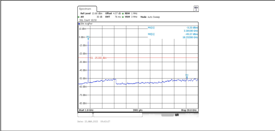
38-38-20MHz-20MHz-64QAM-64QAM-37850-38048-100RB#0-100RB#0-1000~20000MHz
