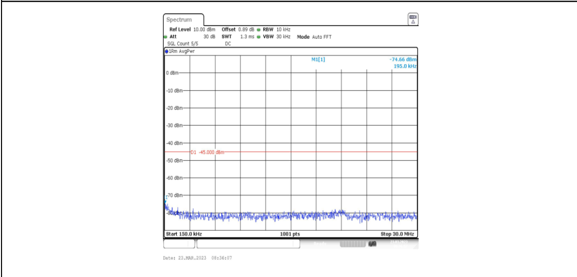
38-38-20MHz-20MHz-QPSK-QPSK-37850-38048-1RB#0-1RB#99-0.15~30MHz
