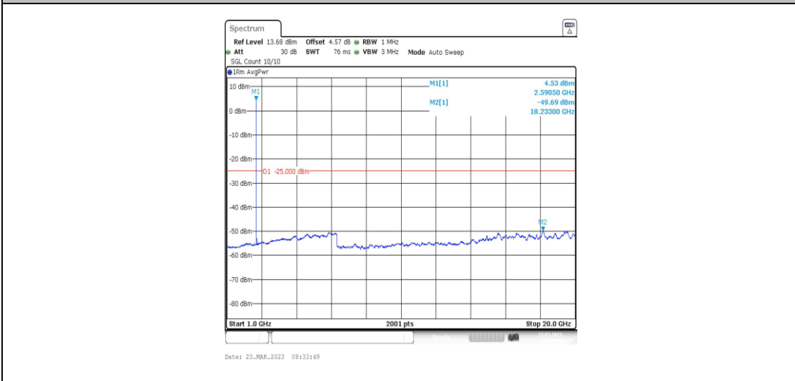
38-38-20MHz-20MHz-16QAM-16QAM-37850-38048-1RB#99-0RB#0-1000~20000MHz
