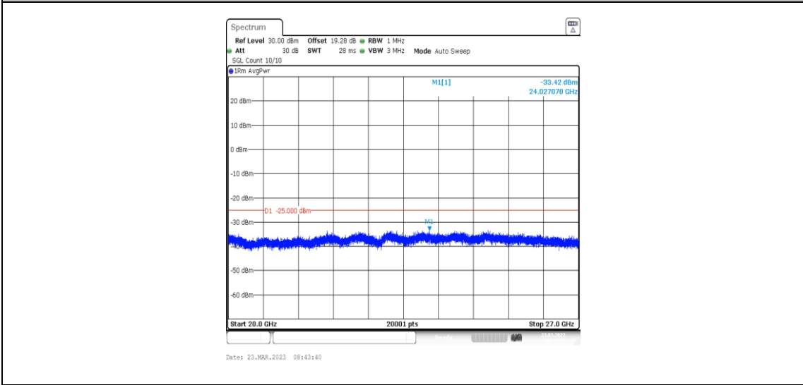
38-38-20MHz-20MHz-64QAM-64QAM-37850-38048-100RB#0-100RB#0-20000~27000MHz
