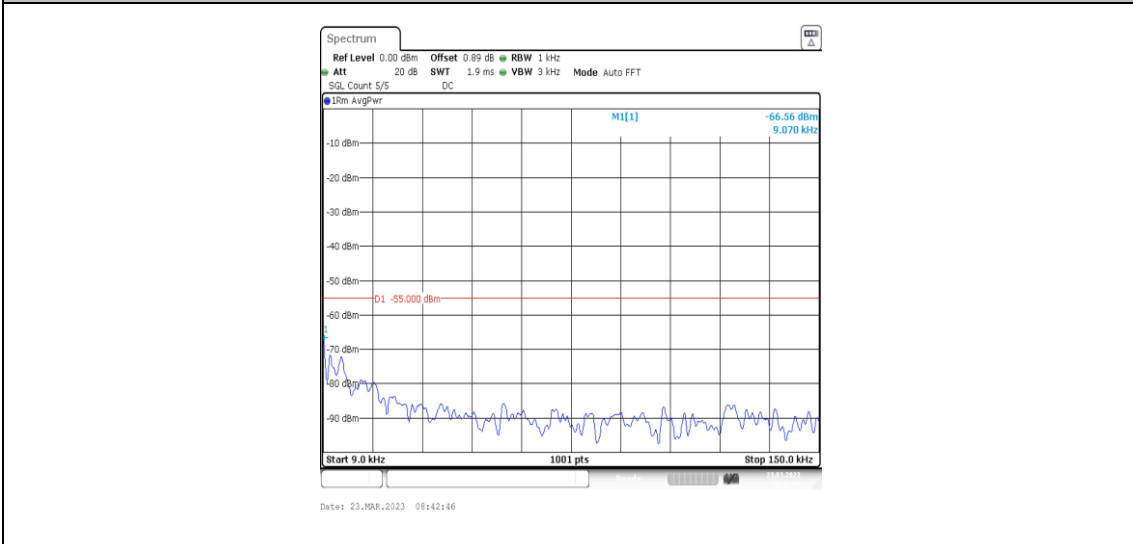
38-38-20MHz-20MHz-64QAM-64QAM-37850-38048-100RB#0-100RB#0-0.009~0.15MHz
