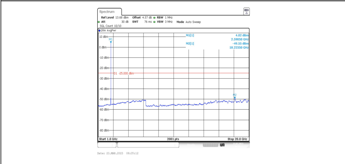
38-38-20MHz-20MHz-64QAM-64QAM-37850-38048-1RB#99-0RB#0-1000~20000MHz
