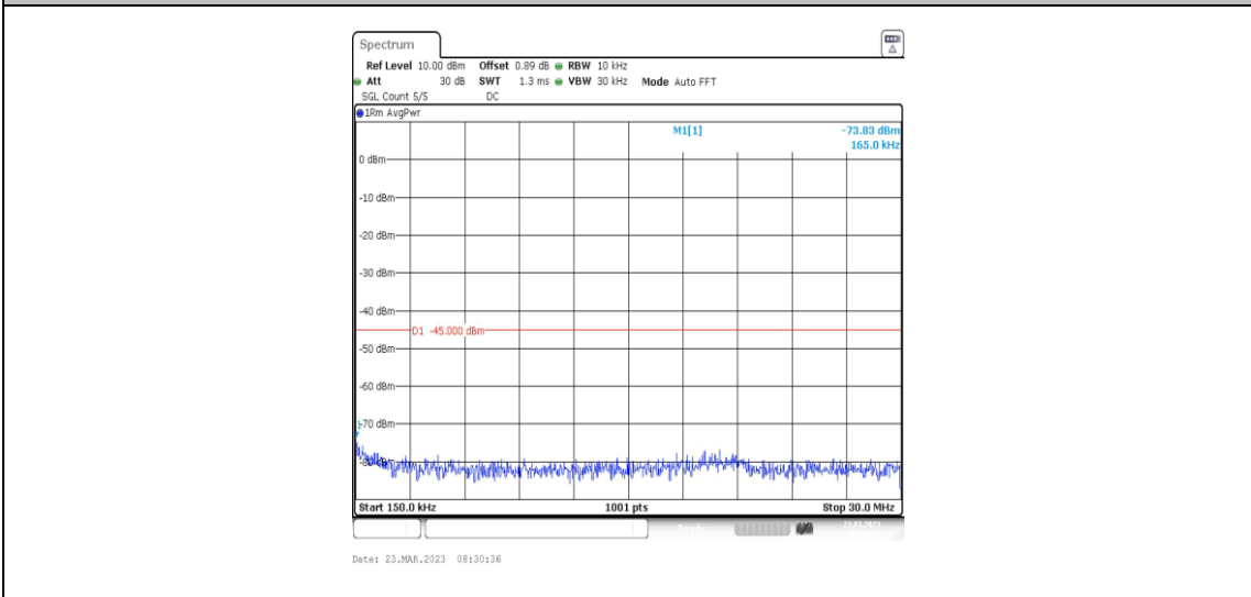
38-38-20MHz-20MHz-64QAM-64QAM-37850-38048-1RB#0-0RB#0-0.15~30MHz
