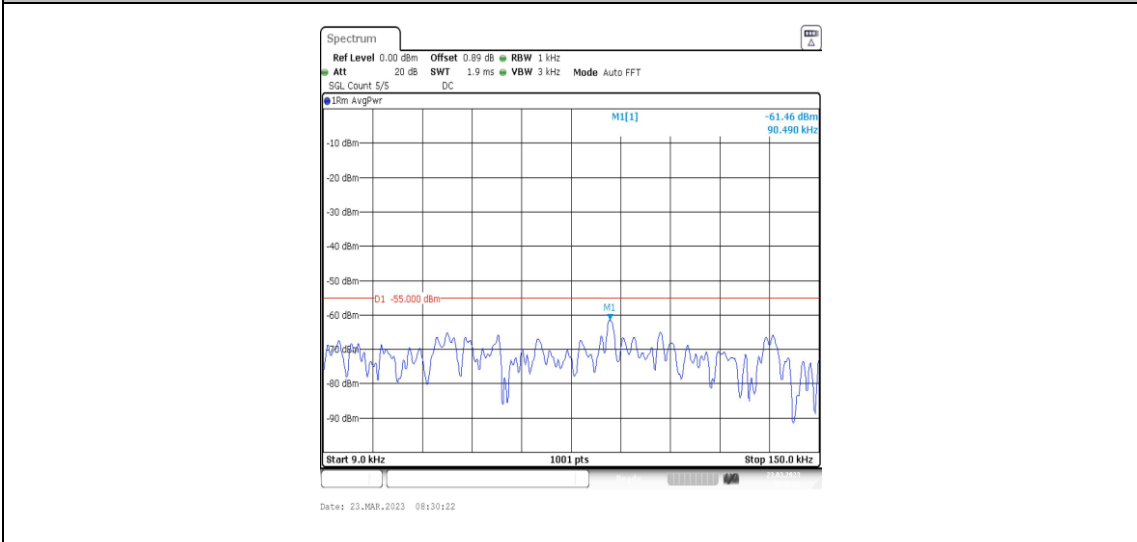
38-38-20MHz-20MHz-64QAM-64QAM-37850-38048-1RB#0-0RB#0-0.009~0.15MHz
