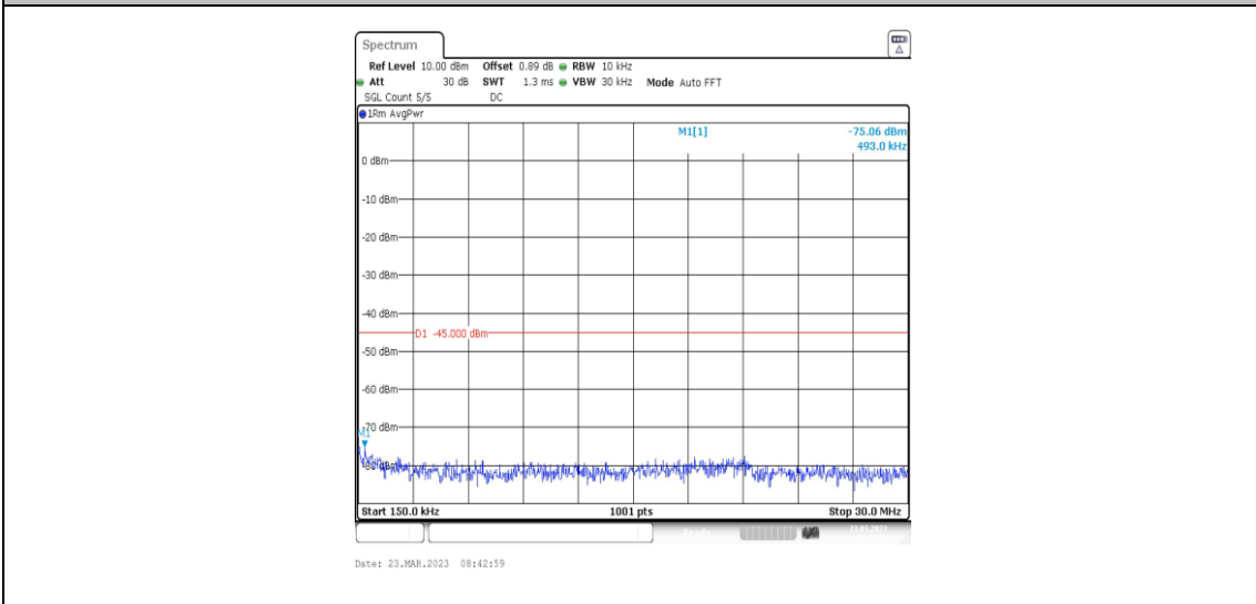
38-38-20MHz-20MHz-64QAM-64QAM-37850-38048-100RB#0-100RB#0-0.15~30MHz
