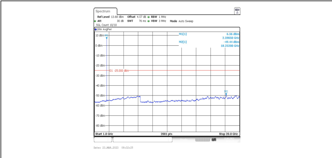
38-38-20MHz-20MHz-QPSK-QPSK-37850-38048-1RB#99-ORB#0-1000~20000MHz
