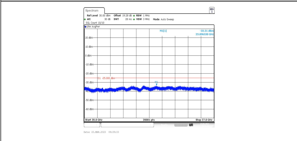
38-38-20MHz-20MHz-64QAM-64QAM-37850-38048-1RB#0-1RB#99-20000~27000MHz
