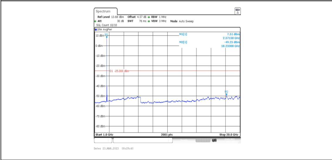
38-38-20MHz-20MHz-16QAM-16QAM-37850-38048-1RB#0-ORB#0-1000~20000MHz
