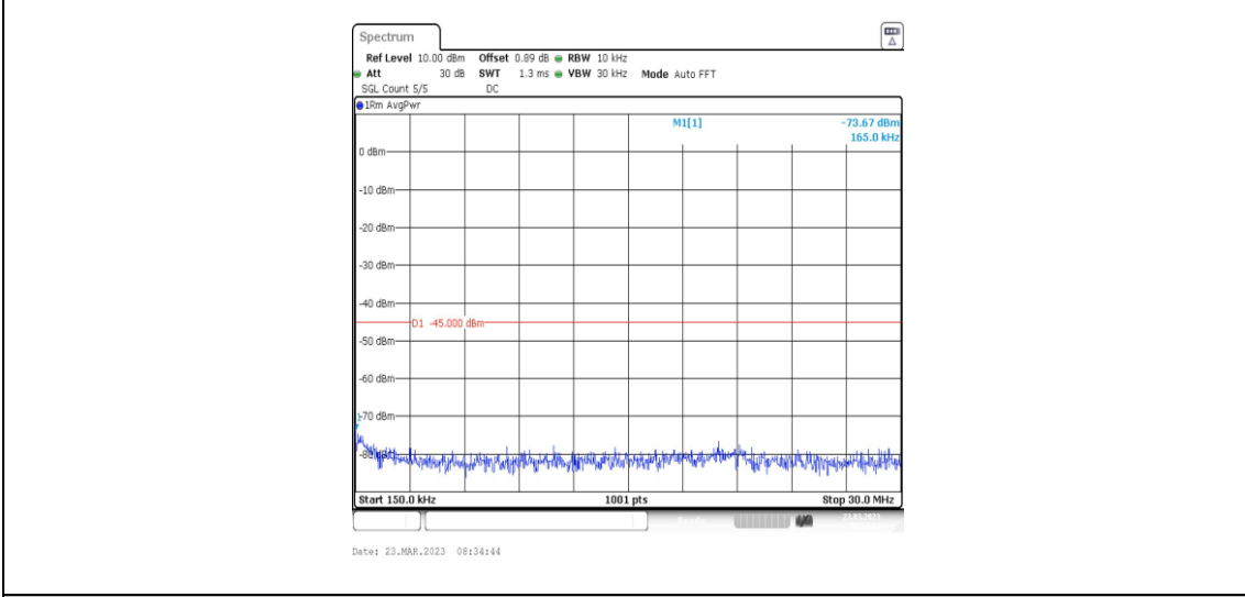
38-38-20MHz-20MHz-64QAM-64QAM-37850-38048-1RB#99-0RB#0-0.15~30MHz
