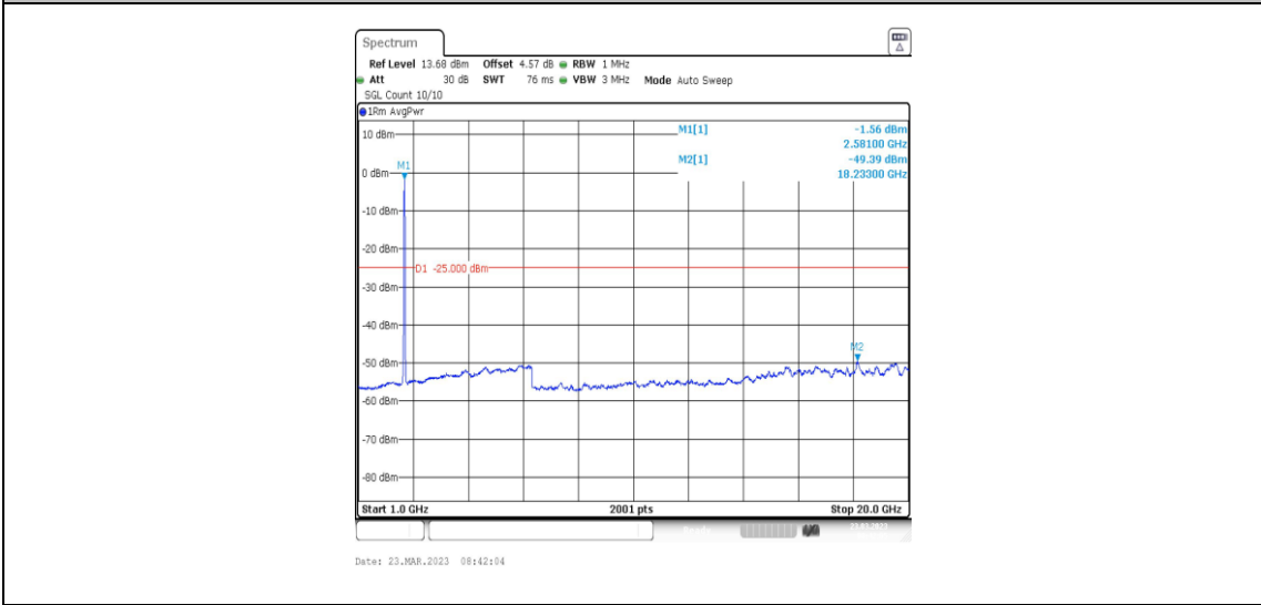
38-38-20MHz-20MHz-16QAM-16QAM-37850-38048-100RB#0-100RB#0-1000~20000MHz
