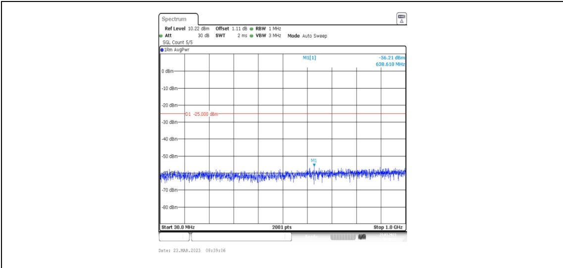
38-38-20MHz-20MHz-64QAM-64QAM-37850-38048-1RB#0-1RB#99-30~1000MHz
