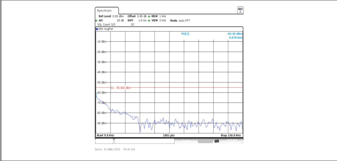
38-38-20MHz-20MHz-16QAM-16QAM-37850-38048-100RB#0-100RB#0-0.009~0.15MHz
