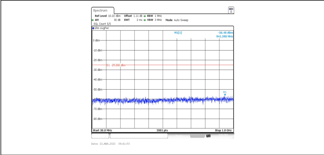
38-38-20MHz-20MHz-16QAM-16QAM-37850-38048-100RB#0-100RB#0-30~1000MHz
