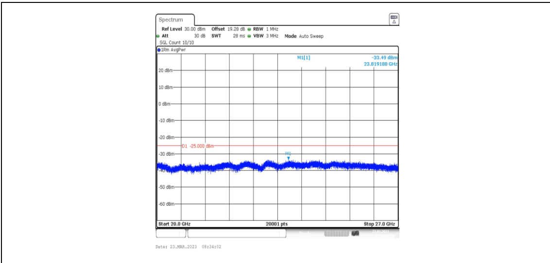
38-38-20MHz-20MHz-16QAM-16QAM-37850-38048-1RB#99-0RB#0-20000~27000MHz
