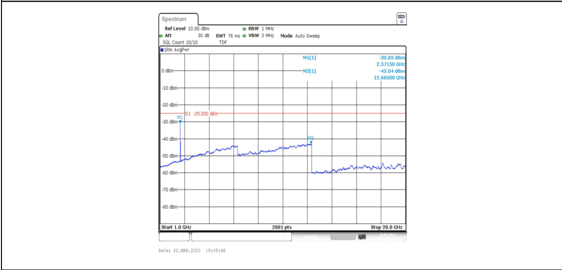
38-38-15MHz-15MHz-16QAM-16QAM-37825-37975-1RB#0-1RB#74-1000~20000MHz
