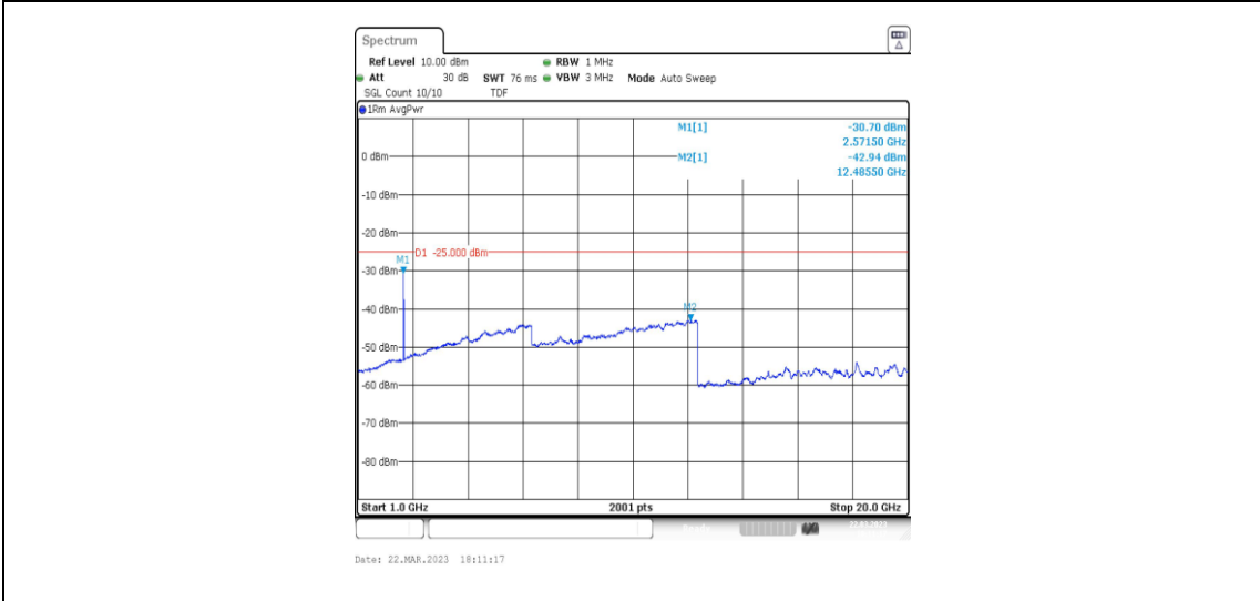
38-38-15MHz-15MHz-64QAM-64QAM-37825-37975-1RB#0-1RB#74-1000~20000MHz
