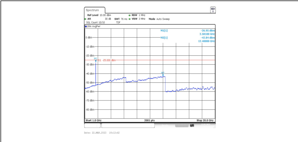
38-38-15MHz-15MHz-QPSK-QPSK-37825-37975-75RB#0-75RB#0-1000~20000MHz
