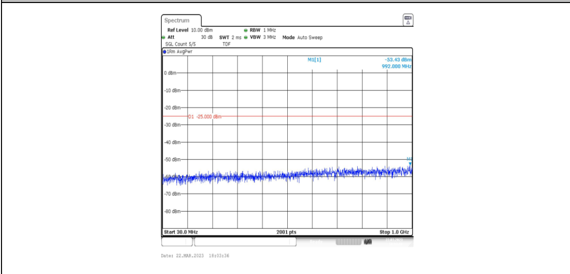
38-38-15MHz-15MHz-QPSK-QPSK-37825-37975-1RB#74-0RB#0-30~1000MHz
