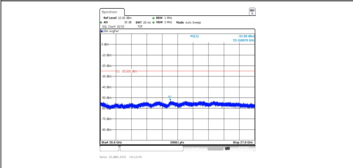
38-38-15MHz-15MHz-QPSK-QPSK-37825-37975-75RB#0-75RB#0-20000~27000MHz
