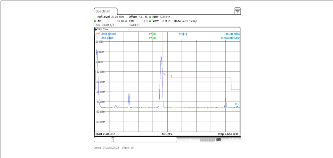
38-38_38-38_20MHz-20MHz_QPSK@QPSK-QPSK@QPSK_37952-38150_1RB#0@100RB#0-1RB#99 @100RB#0
