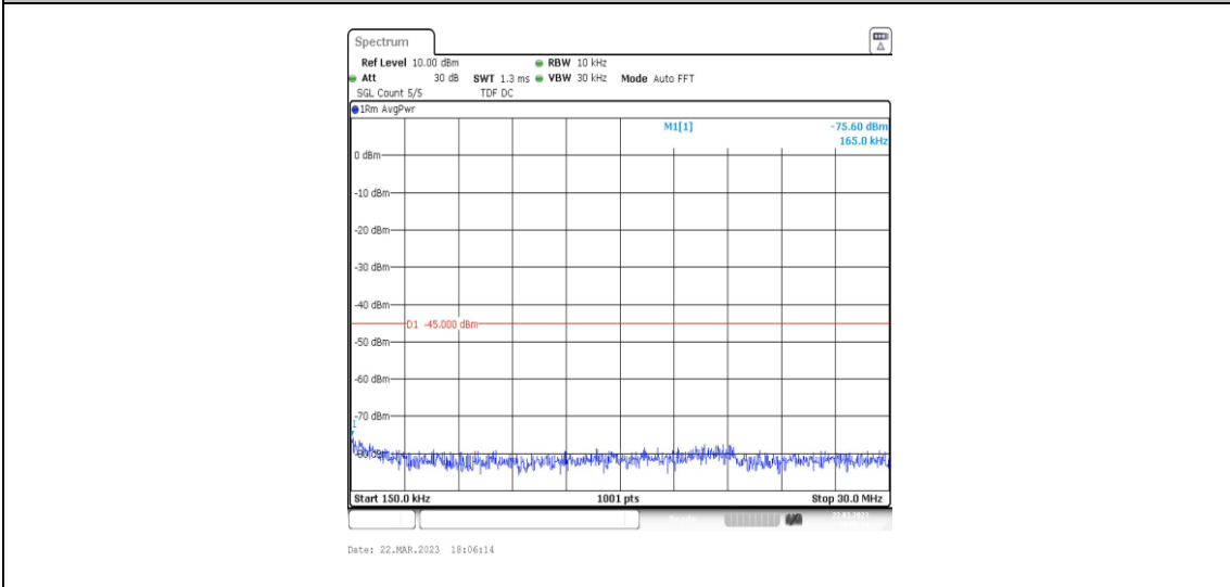
38-38-15MHz-15MHz-64QAM-64QAM-37825-37975-1RB#74-0RB#0-0.15~30MHz
