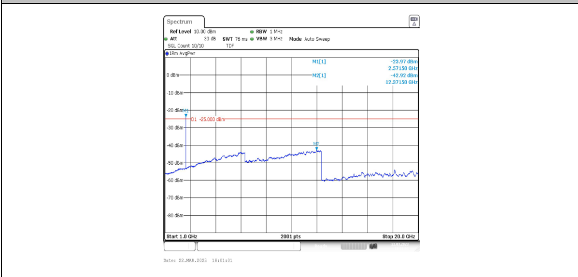
38-38-15MHz-15MHz-16QAM-16QAM-37825-37975-1RB#0-ORB#0-1000~20000MHz
