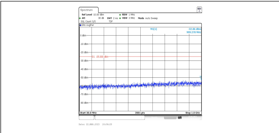
38-38-15MHz-15MHz-64QAM-64QAM-37825-37975-1RB#74-0RB#0-30~1000MHz
