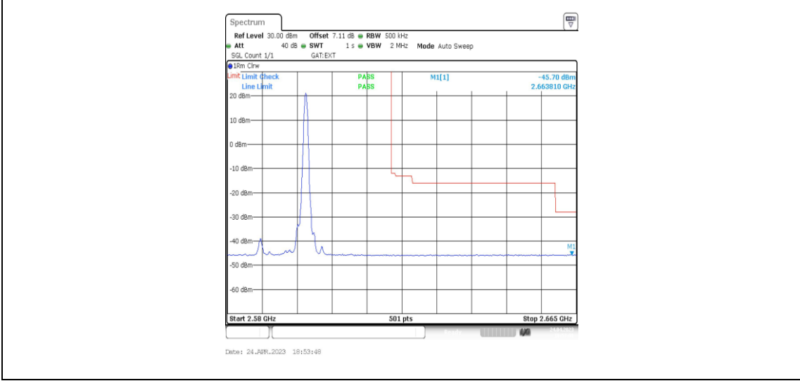
38-38_38-38_20MHz-20MHz_64QAM@64QAM-64QAM@64QAM_37952-38150_1RB#0@100RB#0-0 RB#0@100RB#0
