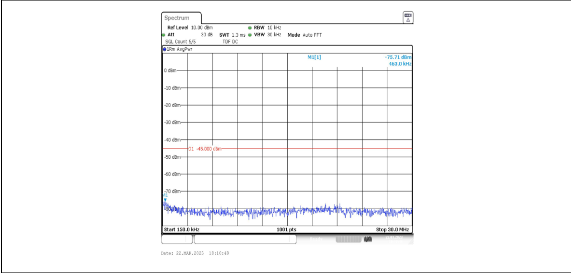
38-38-15MHz-15MHz-64QAM-64QAM-37825-37975-1RB#0-1RB#74-0.15~30MHz
