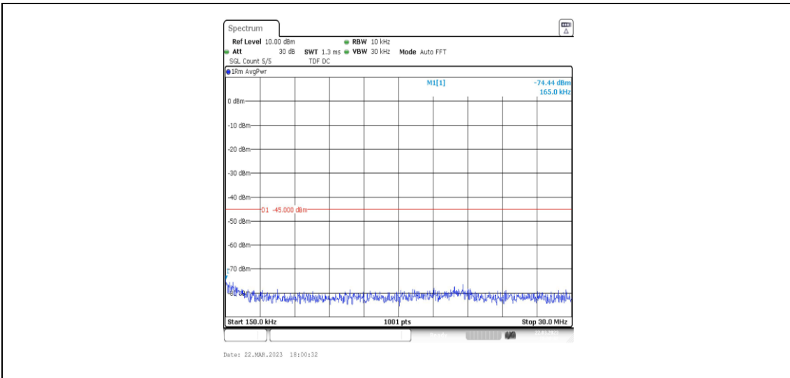
38-38-15MHz-15MHz-16QAM-16QAM-37825-37975-1RB#0-ORB#0-0.15~30MHz
