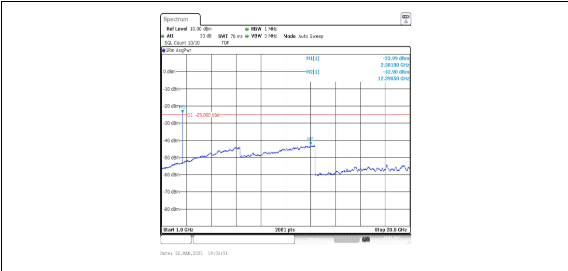
38-38-15MHz-15MHz-QPSK-QPSK-37825-37975-1RB#74-0RB#0-1000~20000MHz
