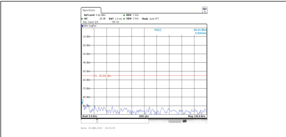
38-38-15MHz-15MHz-QPSK-QPSK-37825-37975-1RB#74-0RB#0-0.009~0.15MHz
