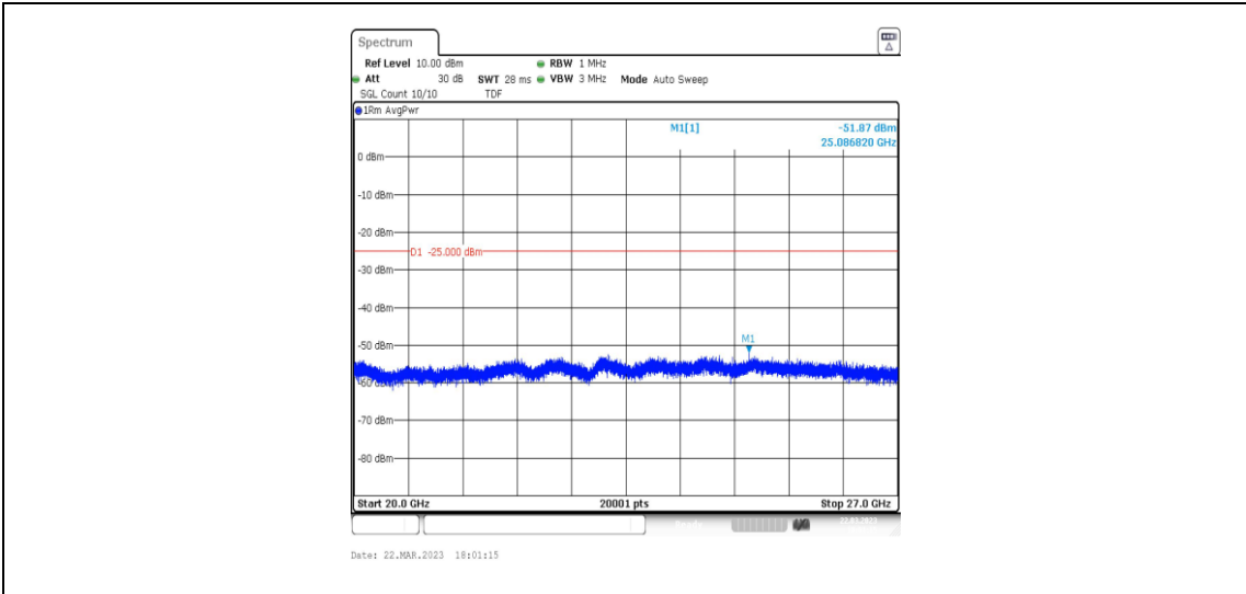
38-38-15MHz-15MHz-16QAM-16QAM-37825-37975-1RB#0-0RB#0-20000~27000MHz
