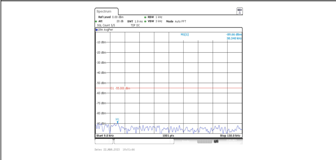
38-38-15MHz-15MHz-64QAM-64QAM-37825-37975-1RB#0-0RB#0-0.009~0.15MHz
