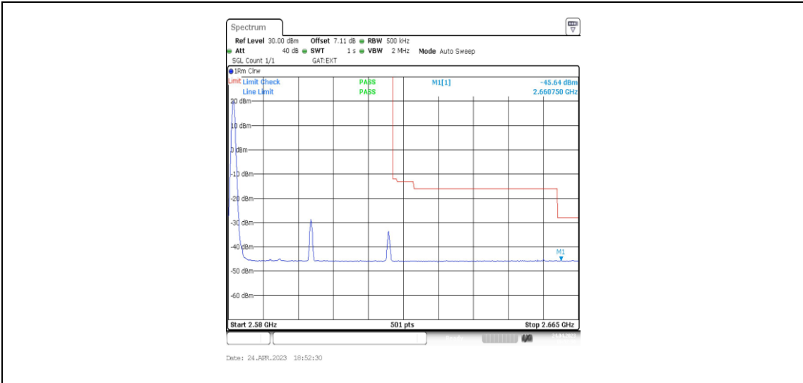
38-38_38-38_20MHz-20MHz_16QAM@16QAM-16QAM@16QAM_37952-38150_1RB#0@100RB#0-0 RB#0@100RB#0
