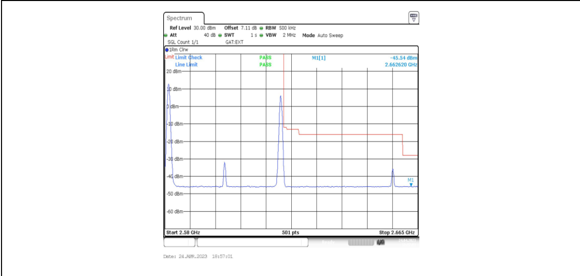
38-38_38-38_20MHz-20MHz_16QAM@16QAM-16QAM@16QAM_37952-38150_1RB#0@100RB#0-1RB#99@100RB#0
