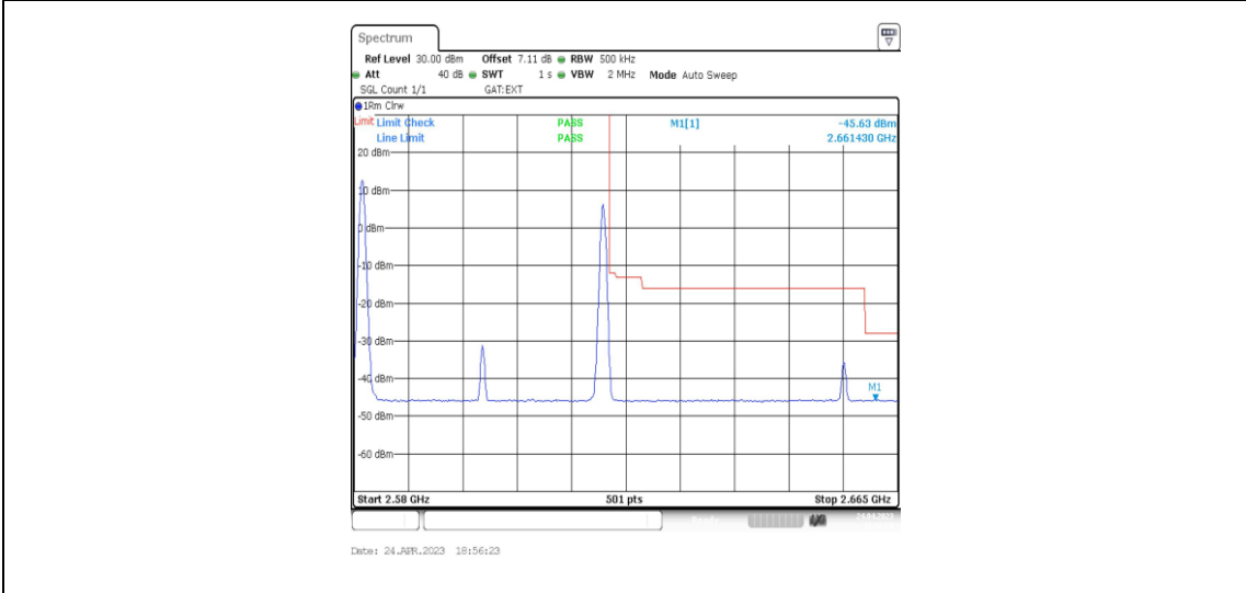
38-38_38-38_20MHz-20MHz_16QAM@16QAM-16QAM@16QAM_37952-38150_1RB#0@100RB#0-1RB#99@100RB#0
