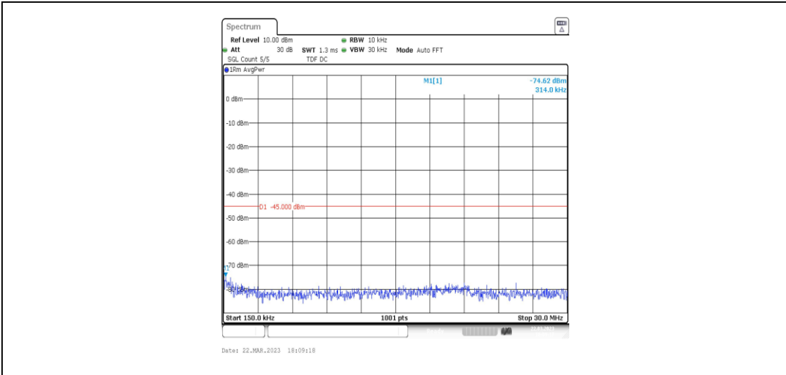
38-38-15MHz-15MHz-16QAM-16QAM-37825-37975-1RB#0-1RB#74-0.15~30MHz
