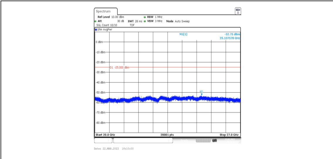
38-38-15MHz-15MHz-16QAM-16QAM-37825-37975-1RB#0-1RB#74-20000~27000MHz
