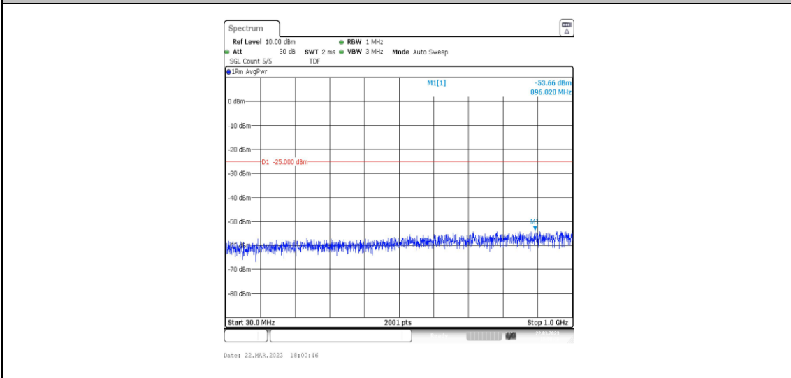
38-38-15MHz-15MHz-16QAM-16QAM-37825-37975-1RB#0-ORB#0-30~1000MHz
