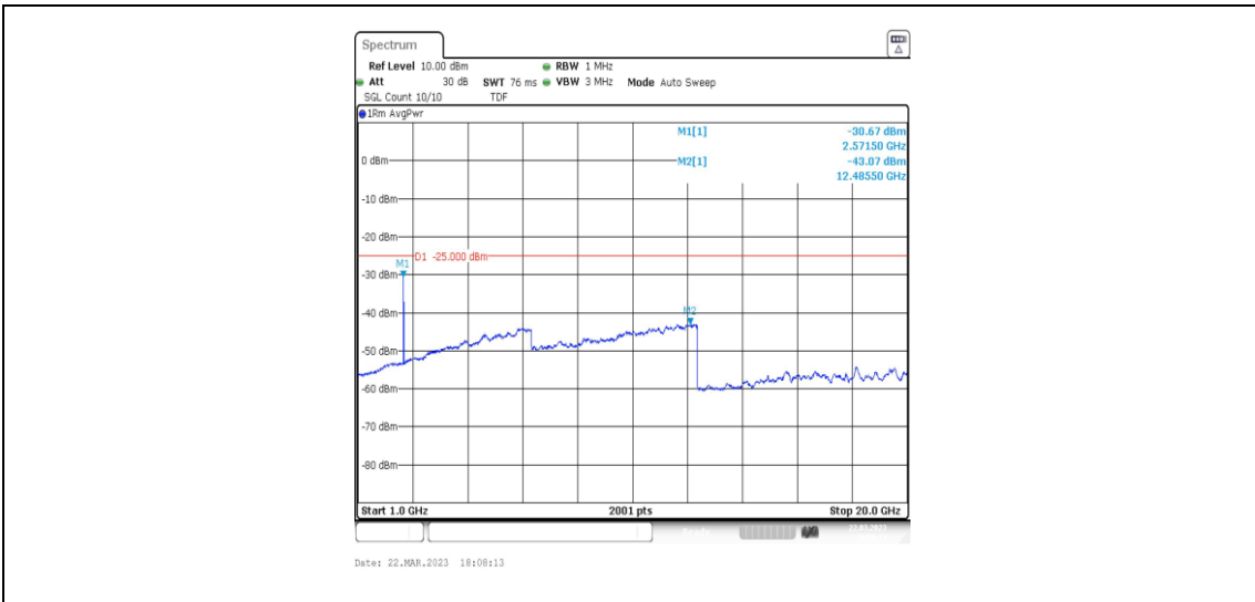
38-38-15MHz-15MHz-QPSK-QPSK-37825-37975-1RB#0-1RB#74-1000~20000MHz
