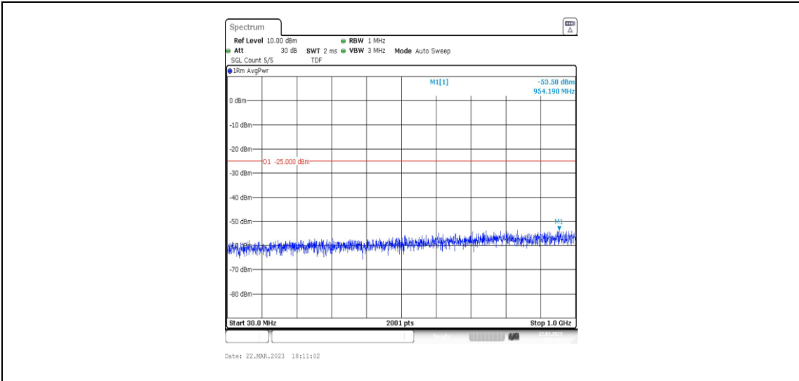
38-38-15MHz-15MHz-64QAM-64QAM-37825-37975-1RB#0-1RB#74-30~1000MHz
