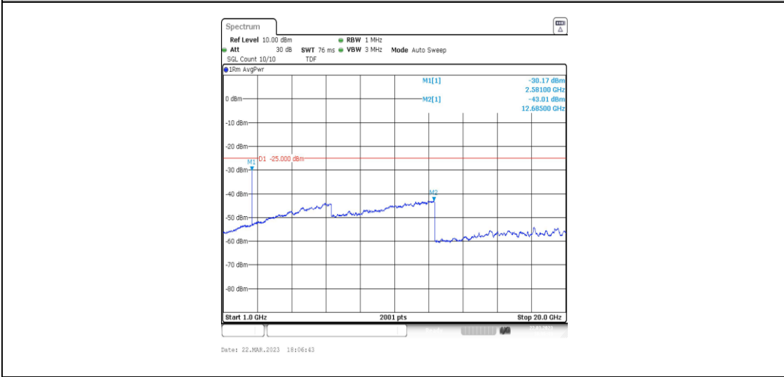
38-38-15MHz-15MHz-64QAM-64QAM-37825-37975-1RB#74-0RB#0-1000~20000MHz
