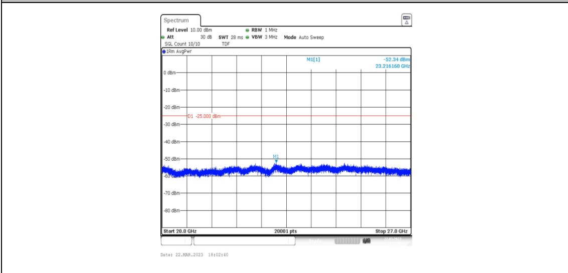
38-38-15MHz-15MHz-64QAM-64QAM-37825-37975-1RB#0-0RB#0-20000~27000MHz
