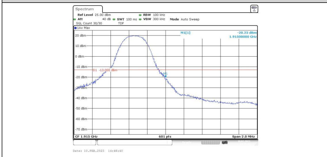
Band25-5MHz-QPSK-26665-25RB#0
