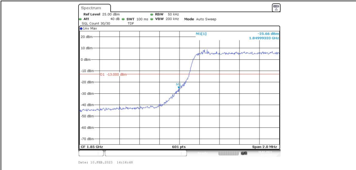
Band25-3MHz-QPSK-26675-1RB#0
