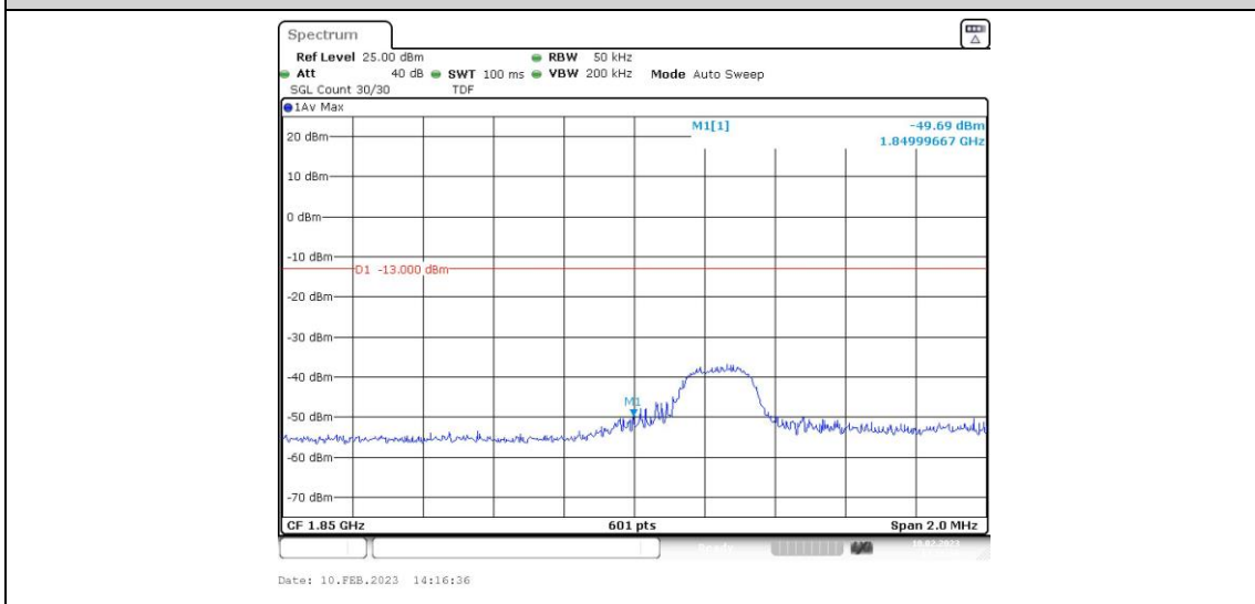
Band25-3MHz-16QAM-26055-15RB#0
