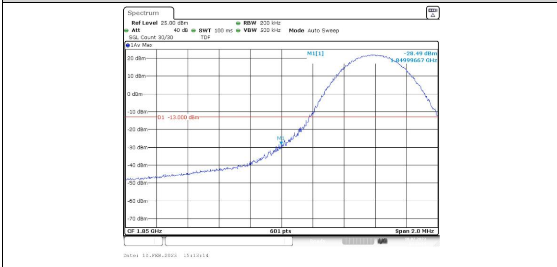
Band25-10MHz-QPSK-26090-1RB#49
