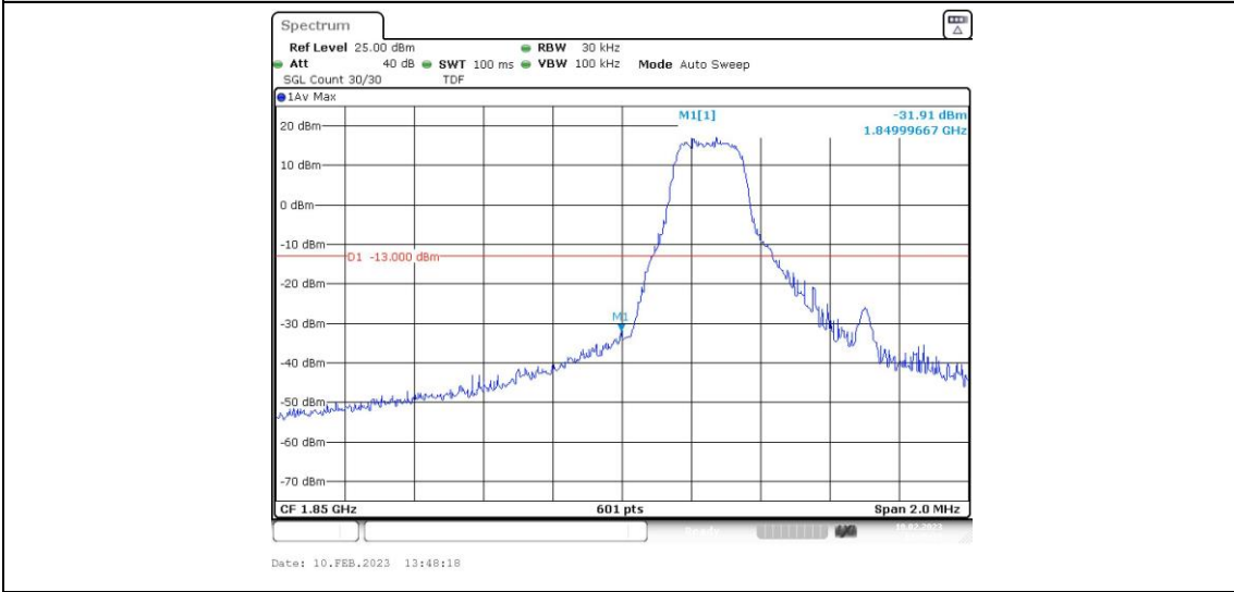
Band25-1.4MHz-16QAM-26047-1RB#5
