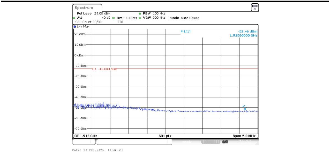
Band25-5MHz-16QAM-26665-1RB#24
