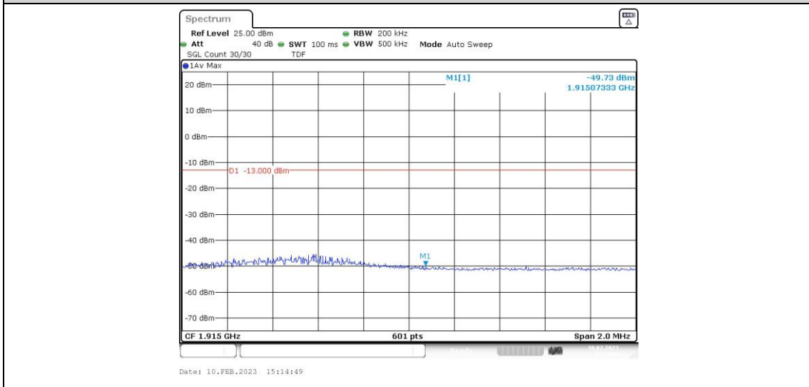
Band25-10MHz-16QAM-26640-1RB#49
