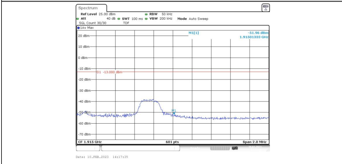
Band25-3MHz-16QAM-26675-1RB#14
