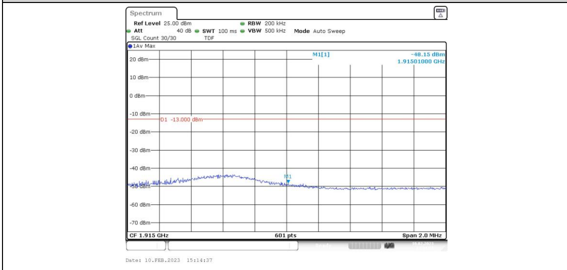
Band25-10MHz-QPSK-26640-1RB#49
