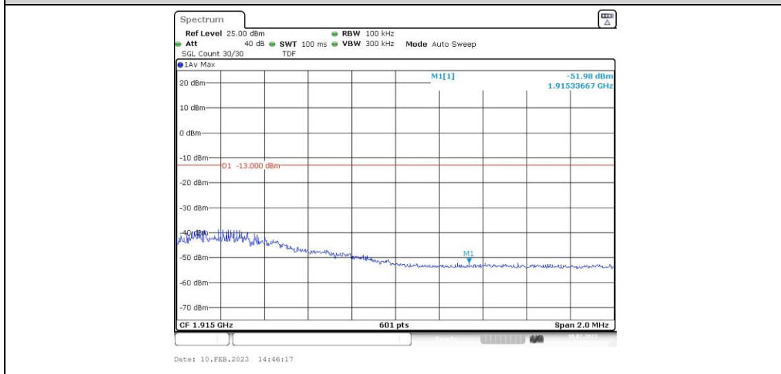
Band25-5MHz-QPSK-26665-1RB#24
