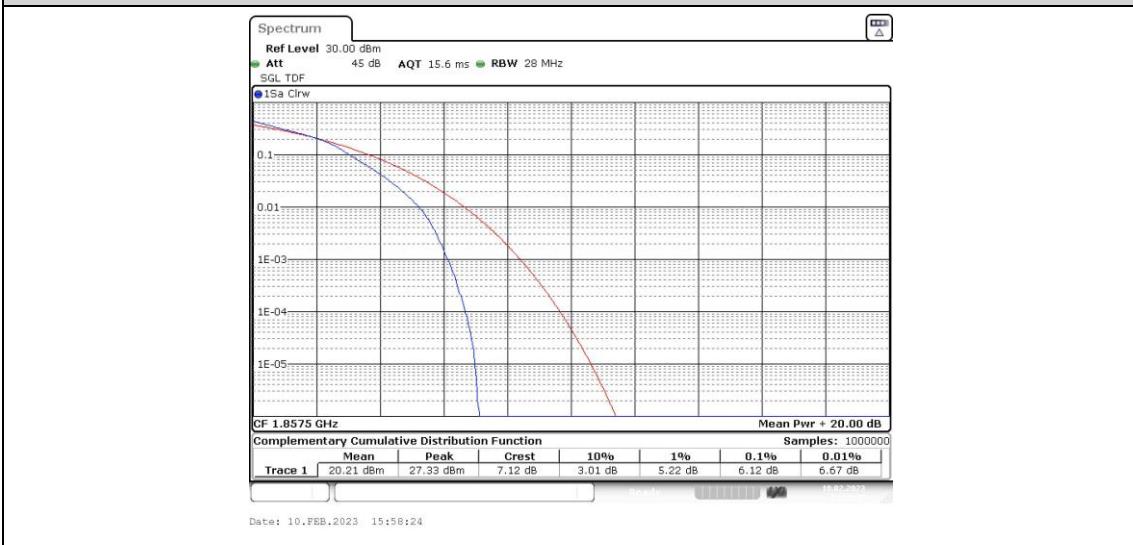
Band25-15MHz-16QAM-26365-1RB#0
