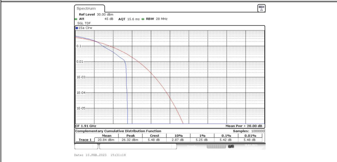
Band25-10MHz-16QAM-26640-50RB#0
