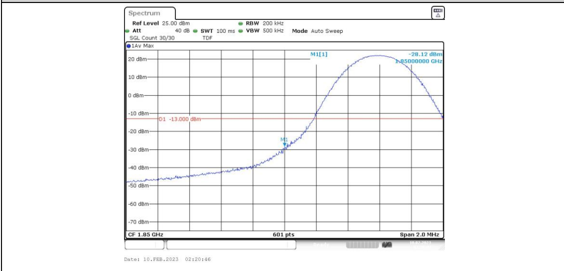
Band2-10MHz-QPSK-18650-1RB#49
