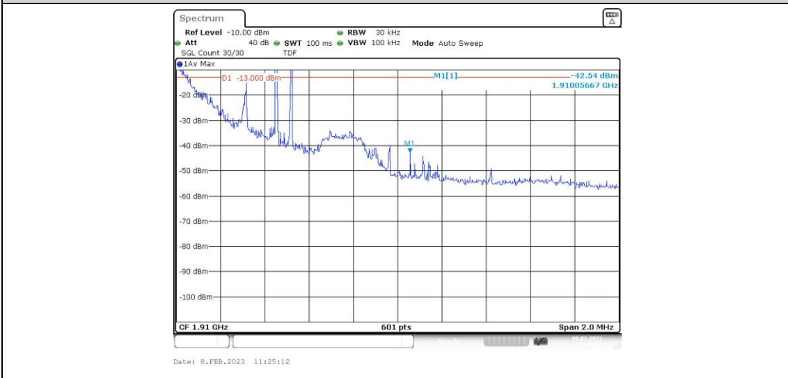
Band2-1.4MHz-QPSK-19193-1RB#5
