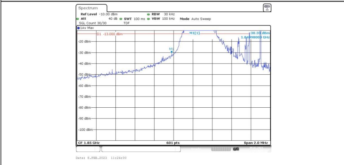
Band2-1.4MHz-16QAM-18607-1RB#5
