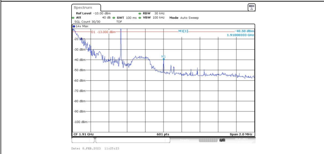
Band2-1.4MHz-16QAM-19193-1RB#5
