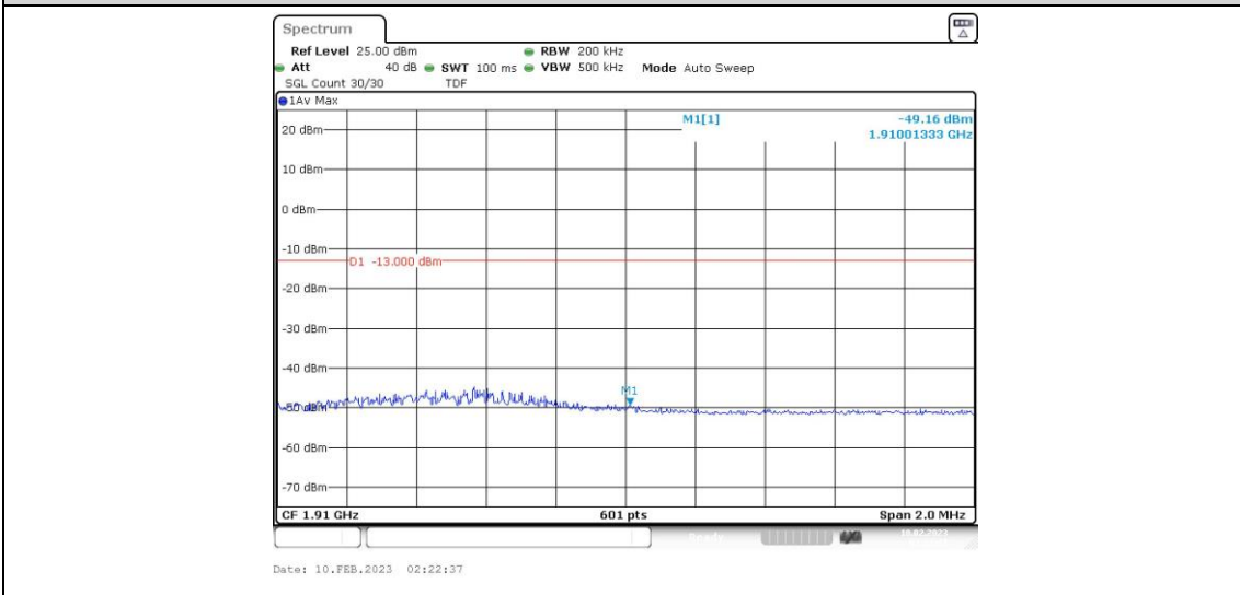
Band2-10MHz-16QAM-19150-1RB#49
