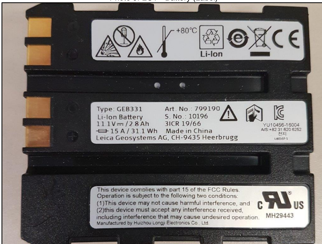
Photo 9: EUT - Battery (Label)
