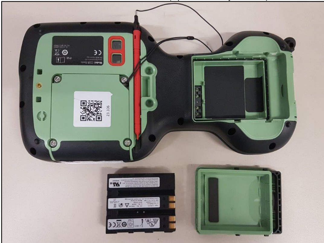
Photo 8: EUT - Battery (Label)
