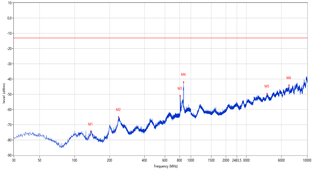
RSE Test case_CE FCC PART22&24&27_FCC LTE B5&12&13&26
